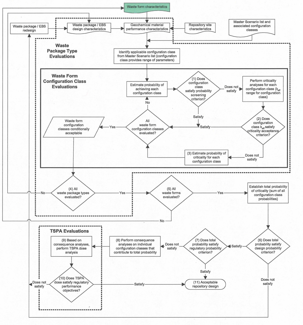
Figure 1. Disposal Criticality Analysis Methodology
