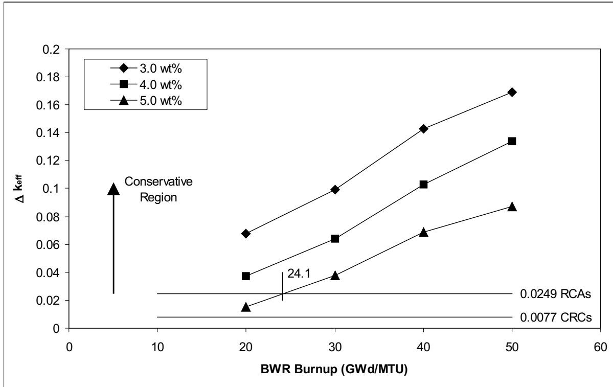
Figure 15. BWR \Delta k_{eff} Values for Bounding versus Nominal Parameters
