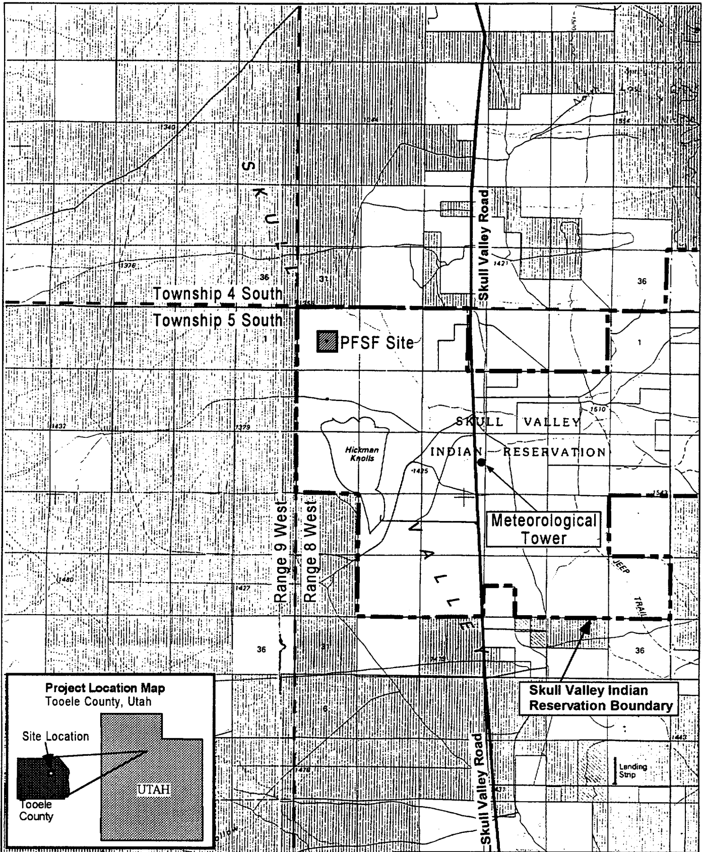
FIGURE 2.3-6 METEOROLOGICAL TOWER LOCATION RELATIVE TO THE PFSF SITE PRIVATE FUEL STORAGE FACILITY SAFETY ANALYSIS REPORT
