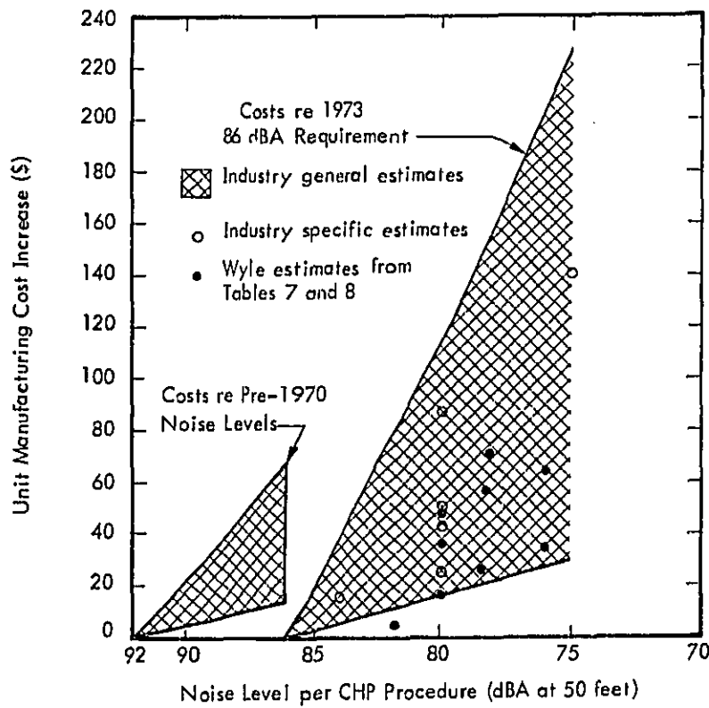
Figure 13. Estimated Noise Reduction Costs for Motorcycles >200 cc
