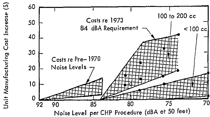
Figure 12. Estimated Noise Reduction Costs for Motor-Driven Cycles <200 cc
