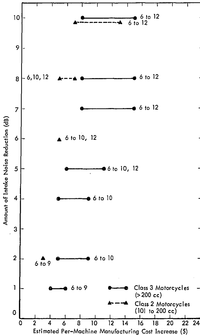
Figure 10. Estimated Costs for Reduction of Motorcycle Intake Noise
