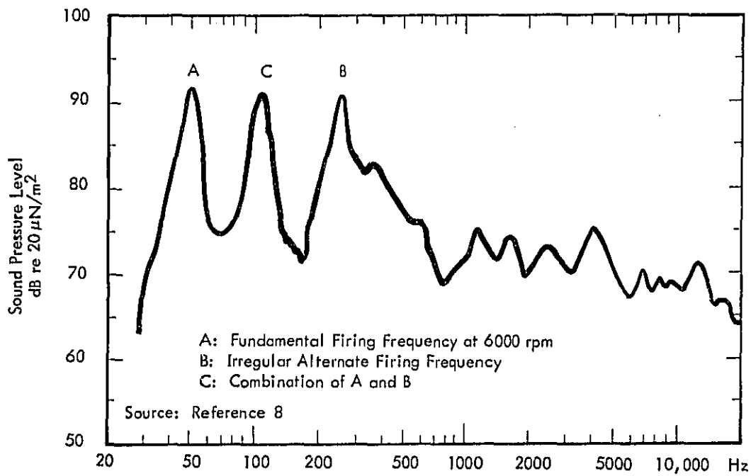
Figure 7. Narrow Band Exhaust Noise Spectrum for >200 cc Muffled Four-Cycle Twin Cylinder Motorcycle - See Text
