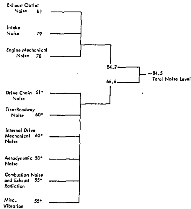
Figure 6. Typical Component Contributions to Total Noise Level When Measured per California Highway Patrol Procedures (dBA at 50 feet) for Typical 1973 Model Motorcycles > 200 cc
