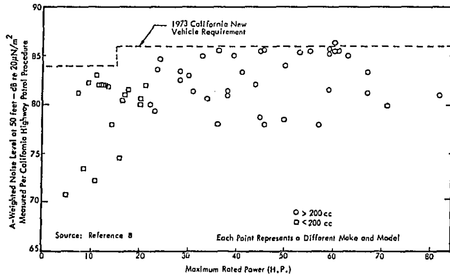
Figure 3. Noise Levels of 1973 Model Motorcycles
