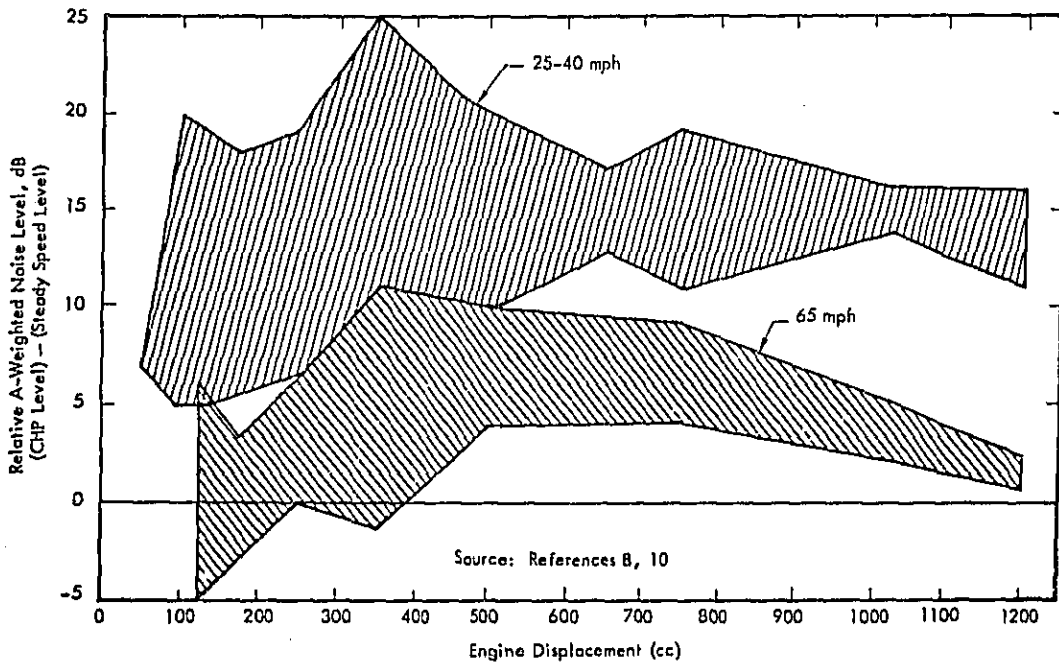
Figure 5. Difference Between CHP Method Acceleration and Steady Speed Noise Levels for 1973 Model Motorcycles
