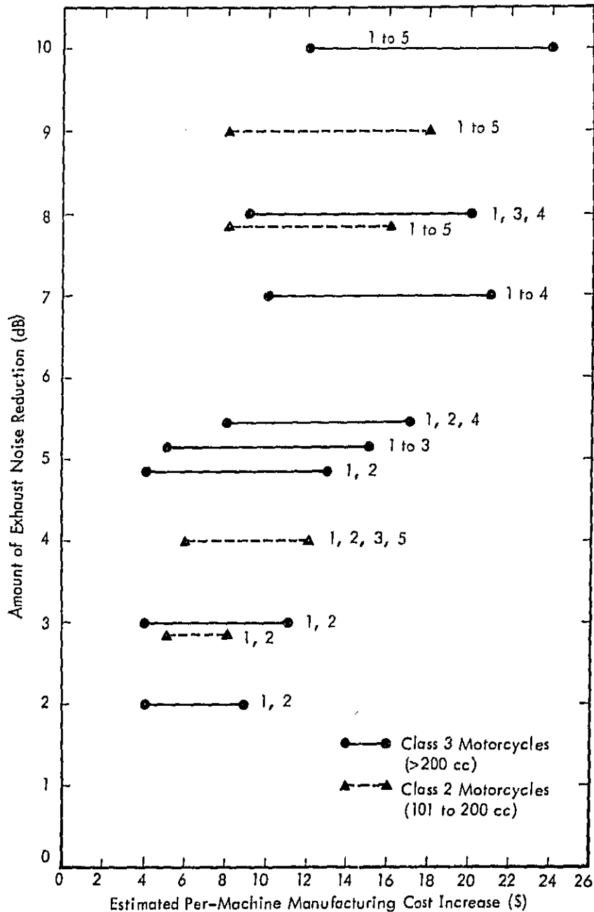
Figure 9. Estimated Costs for Reduction of Motorcycle Exhaust Noise
