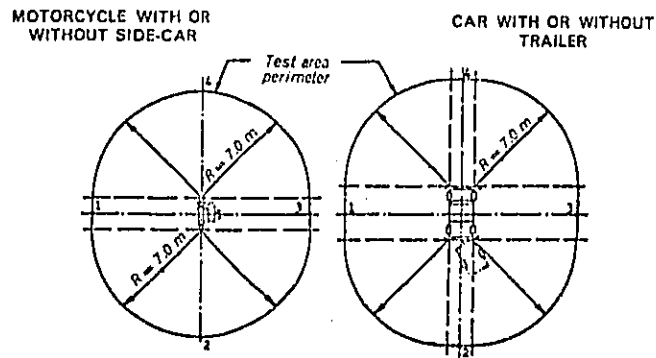
Fig. 2. — Measuring positions for measurement with stationary vehicles
