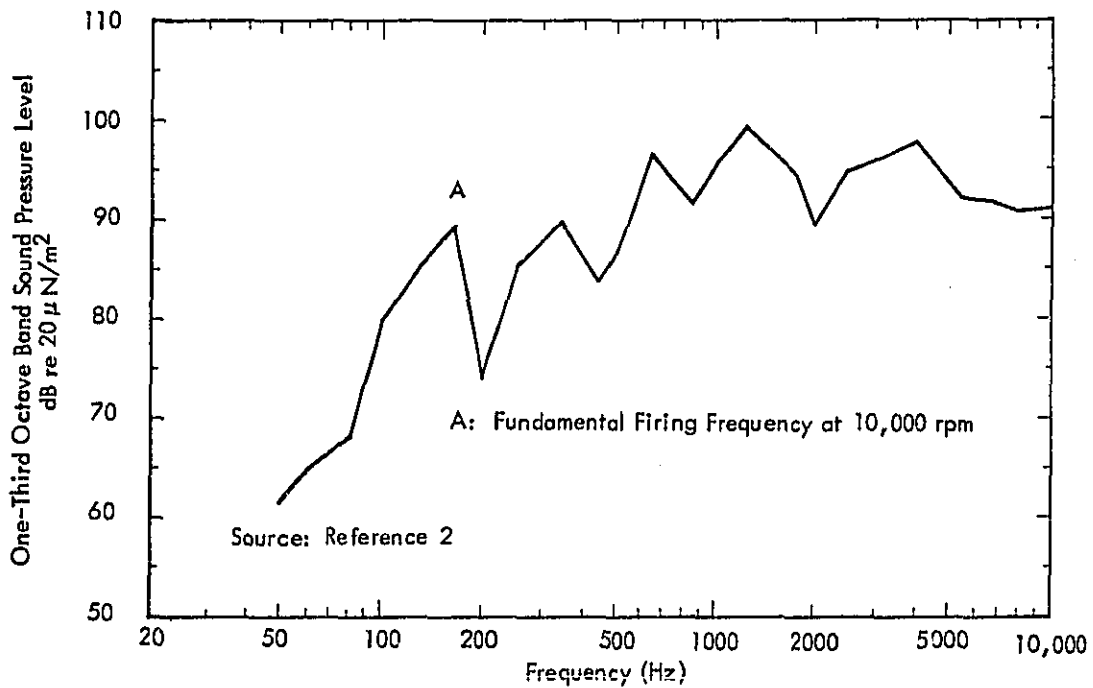
Figure 8. Passby Noise Spectrum for <200 cc Unmuffled Two-Cycle Single Cylinder Motorcycle - See Text
