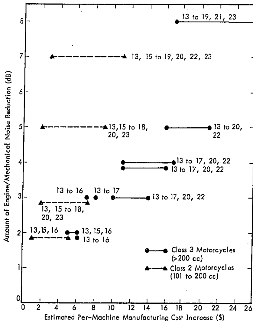
Figure 11. Estimated Costs for Reduction of Motorcycle Engine/Mechanical Noise
