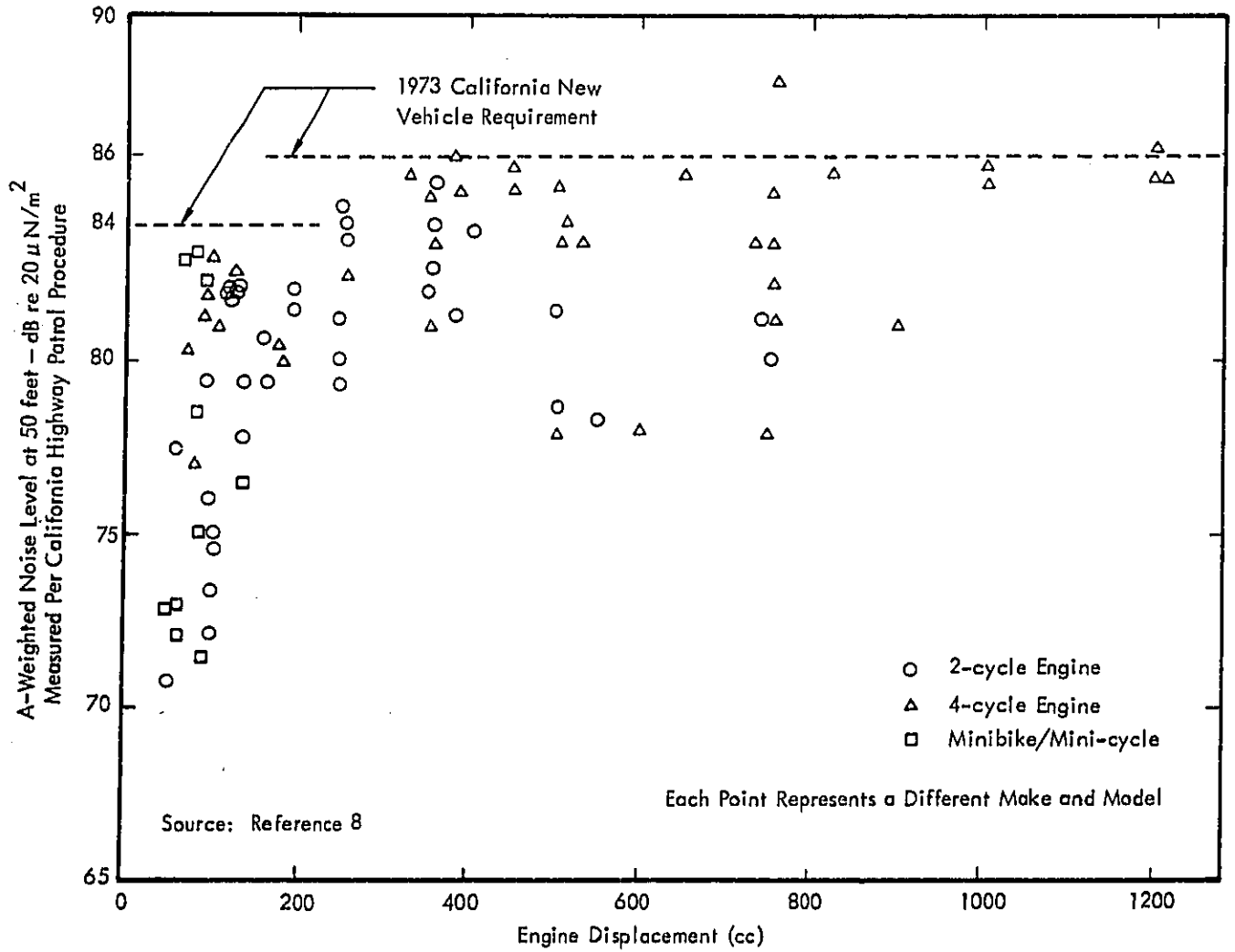
Figure 2. Noise Levels of 1973 Model Motorcycles
