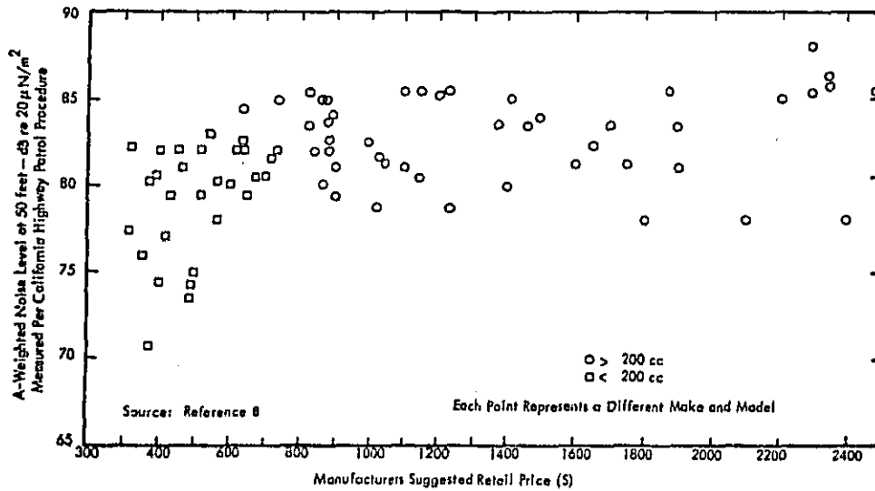
Figure 4. Noise Levels of 1973 Model Motorcycles
