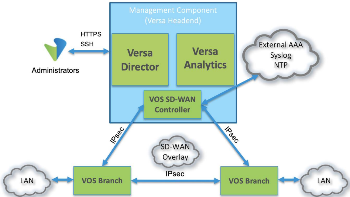
Figure 1: Versa solution
