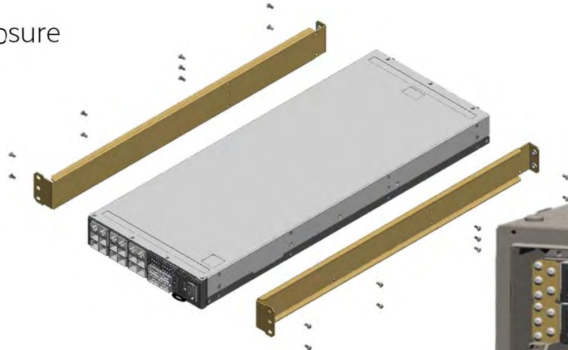
HPE StoreFabric Switch with rail kit
