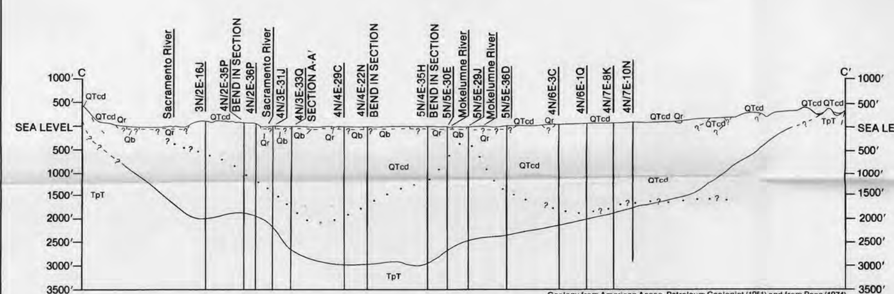
Geologic section C - C', Sacramento Valley, California (See Plate 1 for location of section)
