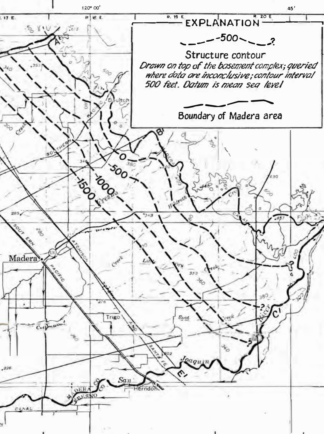
CONTOURS ON BASEMENT COMPLEX
