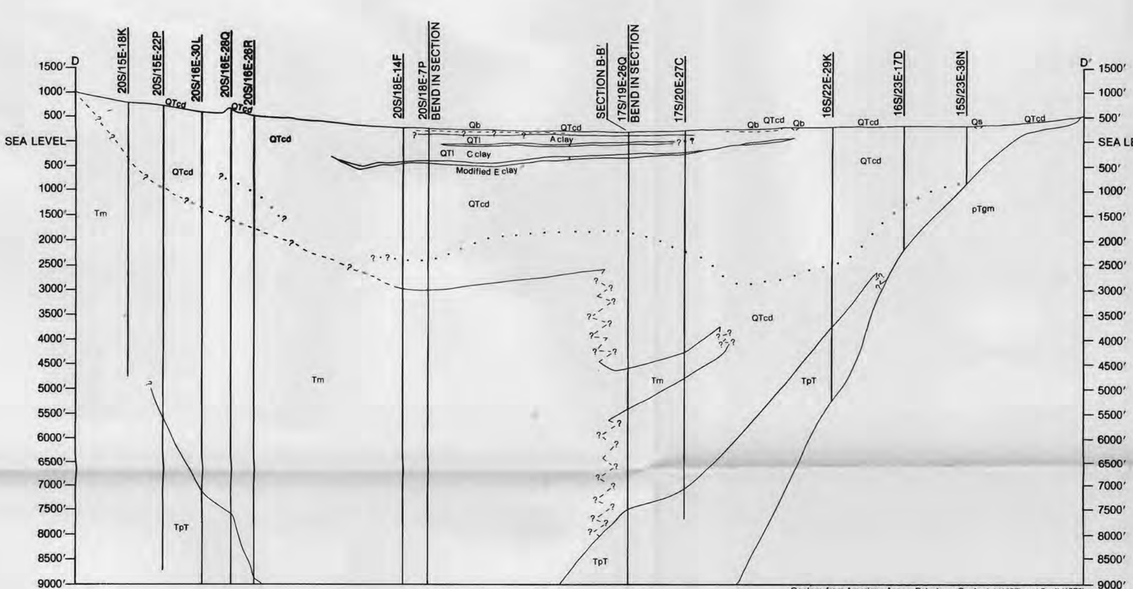
Geologic section D - D', San Joaquin Valley, California (See Plate 2 for location of section)
