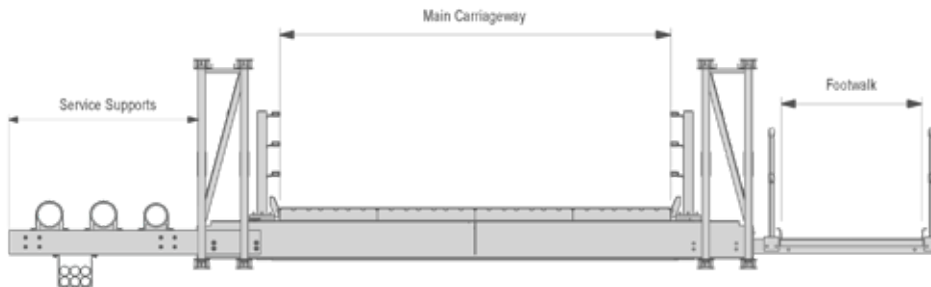
Carriageway, Footwalk and Service Truss
