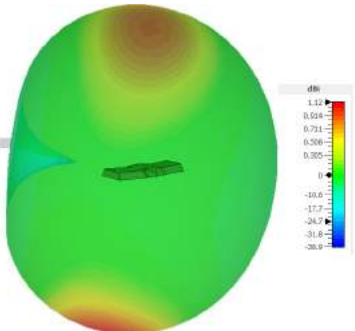
3D Pattern Element 2 (1800MHz)
