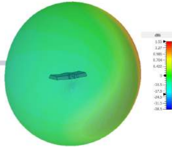
3D Pattern Element 1 (850MHz)
