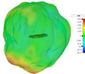
3D Pattern Element 2 (7100MHz)
