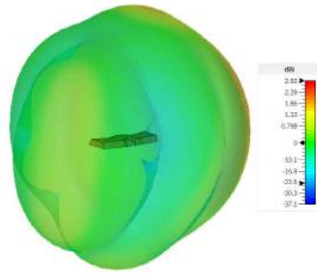
3D Pattern Element 1 (7100MHz)
