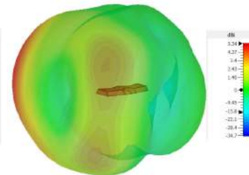
3D Pattern Element 2 (3500MHz)
