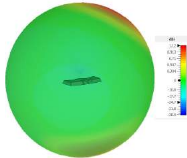
3D Pattern Element 1 (2600MHz)
