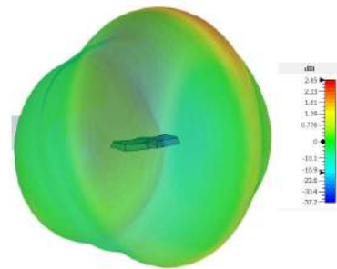
3D Pattern Element 1 (2600MHz)
