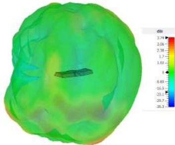
3D Pattern Element 1 (7100MHz)
