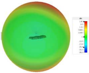
3D Pattern Element 1 (1800MHz)
