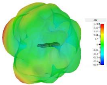
3D Pattern Element 2 (5400MHz)
