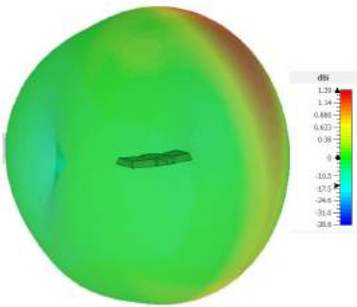
3D Pattern Element 1 (1800MHz)
