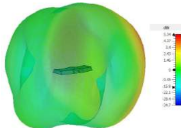
3D Pattern Element 1 (3500MHz)
