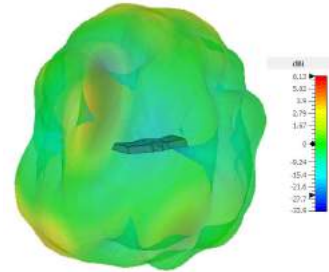
3D Pattern Element 1 (5400MHz)
