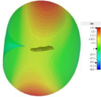
3D Pattern Element 2 (850MHz)
