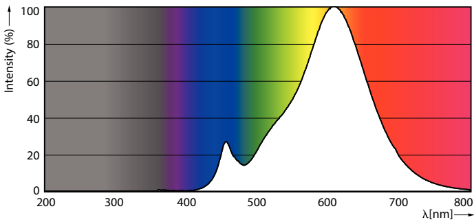
Spectral Power Distribution Colour - LEDClassic 35W G93 E27 825 100-240 ND LA
