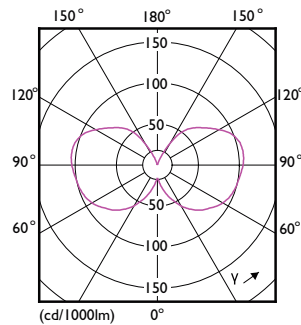
Light Distribution Diagram - LEDClassic 35W G93 E27 825 100-240 ND LA
