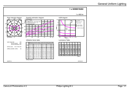
General uniform lighting - LEDClassic 35W G93 E27 825 100-240 ND LA
