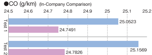
● CO (g/km) (In-Company Comparison)
