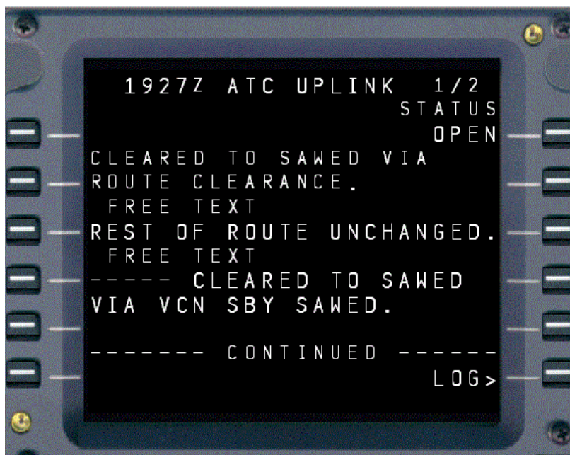
Figure 6 – UM79 Route Clearance and Supplementary Route Free Text (B737 MCDU Test Bench – FAA Tech Center)
