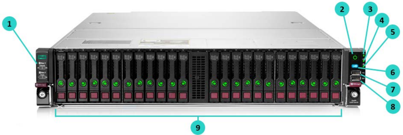
48 SFF Front View
