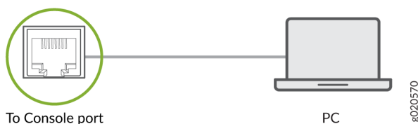
Figure 32: Connect the ACX7024 or ACX7024X Router Directly to a Management Console
