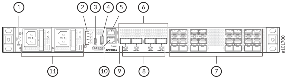
Figure 4: Front View of an AC-Powered ACX7024 Router
