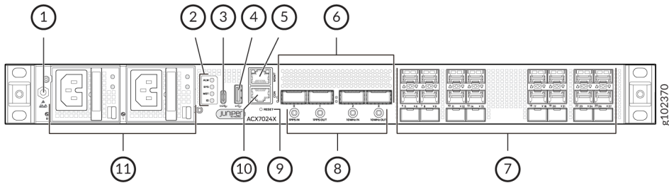
Figure 7: Front View of an AC-Powered ACX7024X Router
