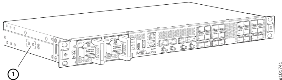
Figure 26: Grounding Point on the ACX7024 and ACX7024X Routers
