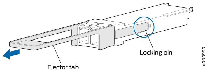
Figure 43: QSFP28 Transceiver
