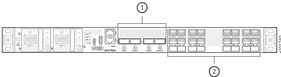
Figure 12: ACX7024 and ACX7024X Port Panel
