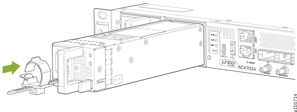
Figure 35: Install an AC PSM in an ACX7024 or ACX7024X Router
