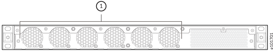
Figure 6: Rear View of an ACX7024 Router
