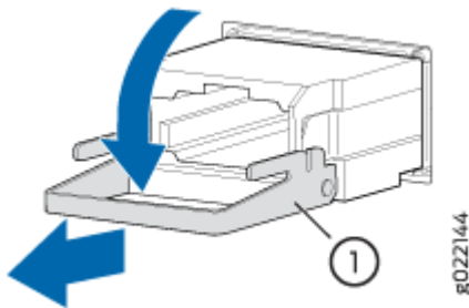
Figure 41: Remove a QSFP+ transceiver
