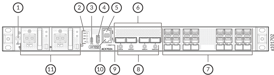
Figure 5: Front View of a DC-Powered ACX7024 Router
