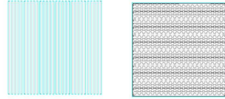
Figure 3. Design of 3D-printed parts according to the direct shear box, a. SolidWorks design, b. different layers of sample generated in slicing software, direction of Grooves Respected to Shear Loading (°): 90, Depth (mm) × Width (mm): 1 × 1
