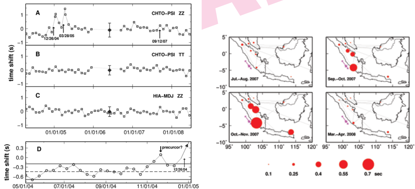
Time shifts of various station pairs, relative to reference stack of all time periods. (A-C) Rayleigh wave for CHTO-PSI from vertical (Z) component correlation (A), Love wave for CHTO-PSI from tangential (T) component correlation (B), and a stable reference pair HIA-MDJ outside Sumatra region in northeast China (C).
