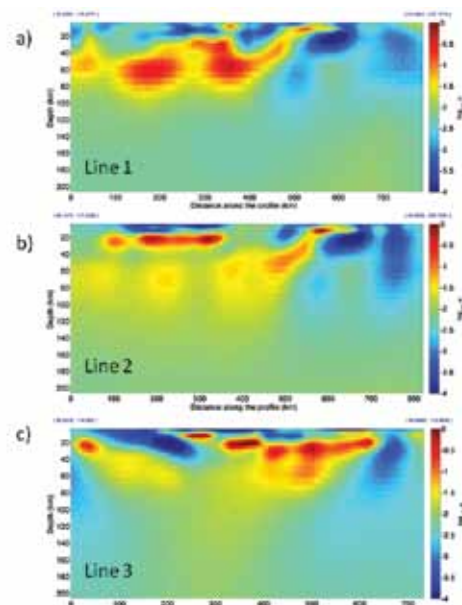
Electrical conductivity transects across the Snake River Plain (see Figure 1).
