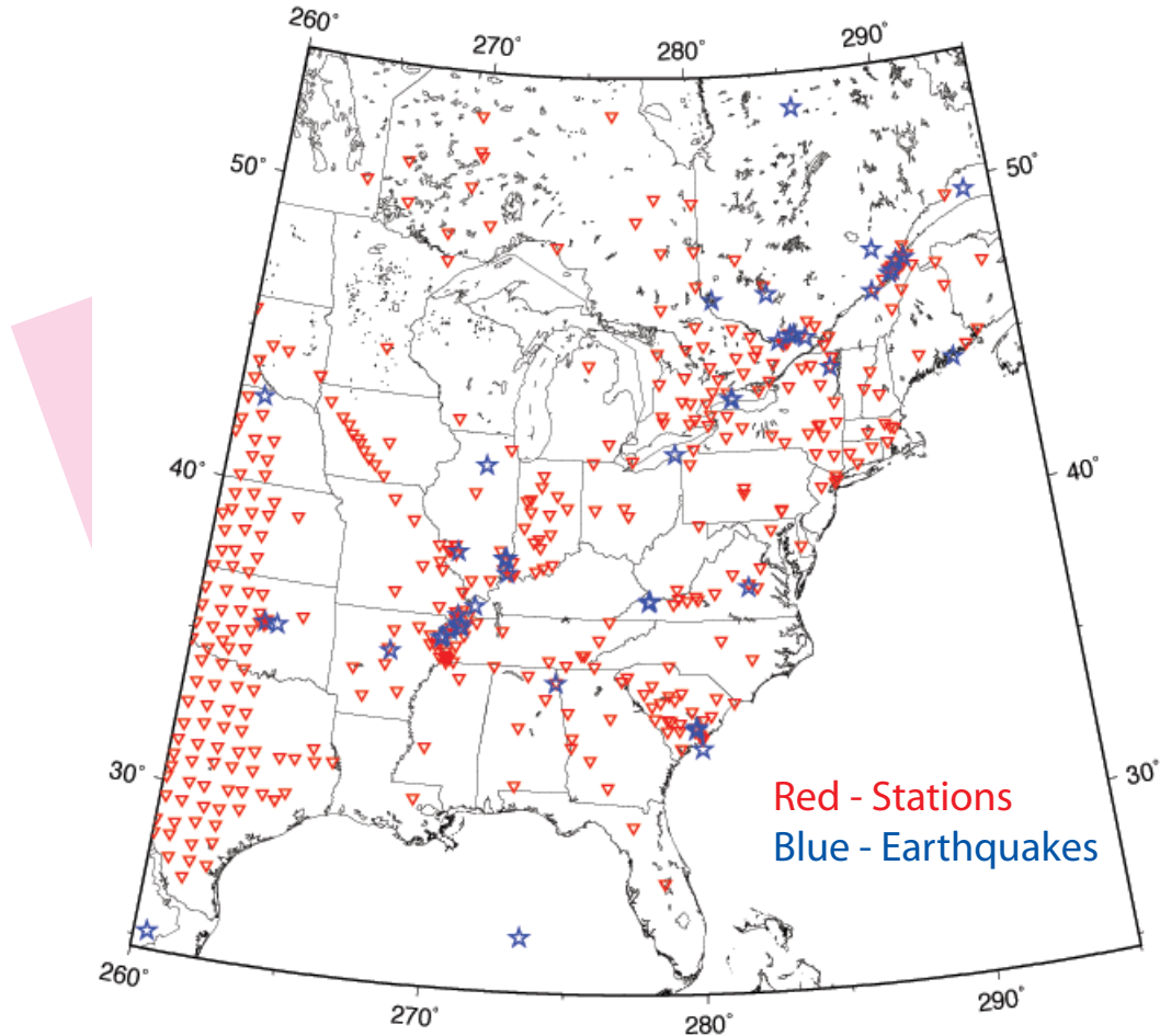
The stations and earthquakes used in the NGA East project so far.
