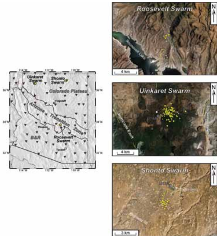
Figure Captions: Left: Locations of three earthquake swarms investigated as part of this study (yellow circles), USArray Transportable Array stations (red triangles), and the geologic/physiographic provinces of Arizona. Right Column: Google Earth screen captures of events from USArray ANF monthly archives (white circles), new events located as part of this study (yellow circles), and USArray TA stations (blue circles). Top Right: Roosevelt Swarm - 62 detections from 6/21/2007 to 6/28/2007 with 20 located events (3+ stations). Mag = 1.6 to 2.5 ml; Avg Depth = 3.8 km; Peak Activity = 10 events/hour. Middle Right: Uinkaret Swarm: 345 detections from 12/4/2007 to 12/17/2007 with 20 located events (3+ stations). Mag = 0.7 to 3.2 ml; Avg Depth = 13.5 km; Peak Activity = 18 events/hour. Bottom Right: Shonto Swarm: 172 detections from 8/29/2008 to 9/29/2008 with 34 located events (3+ stations). Mag = 0.8 to 2.8 ml; Avg Depth = 5.8 km; Peak Activity = 6 events/hour.
