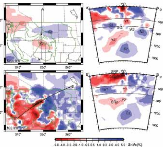
Figure 2. Great-circle cross sections of the velocity structure under the Yellowstone Caldera (YC) and the eastern Snake River Plain (SRP). The black dot and 0° represent the location of the Yellowstone Caldera and the mid-point of the great circle arc. In the cross-section views, each grid along the arc represents 1°. Labels S1, S2, N2, SG identify the same subduction structure as in Sigloch et al. [2008] and Tian et al. [2009].
