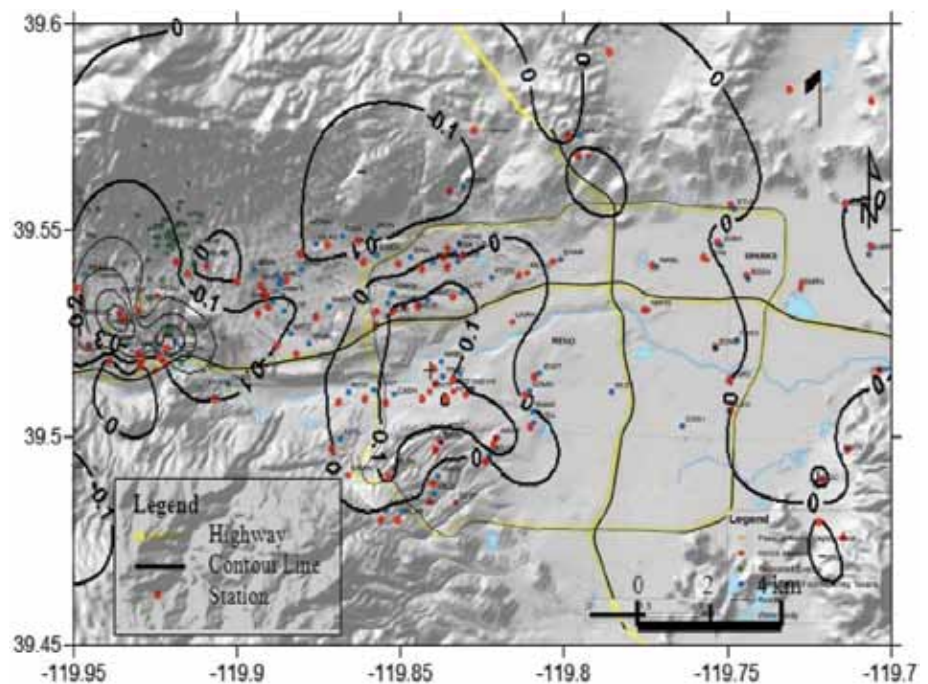
Location of deployed USArray Flexible Array Texan seismographs (red and blue) along with station time-delay contours calculated using both the permanent and portable stations.
