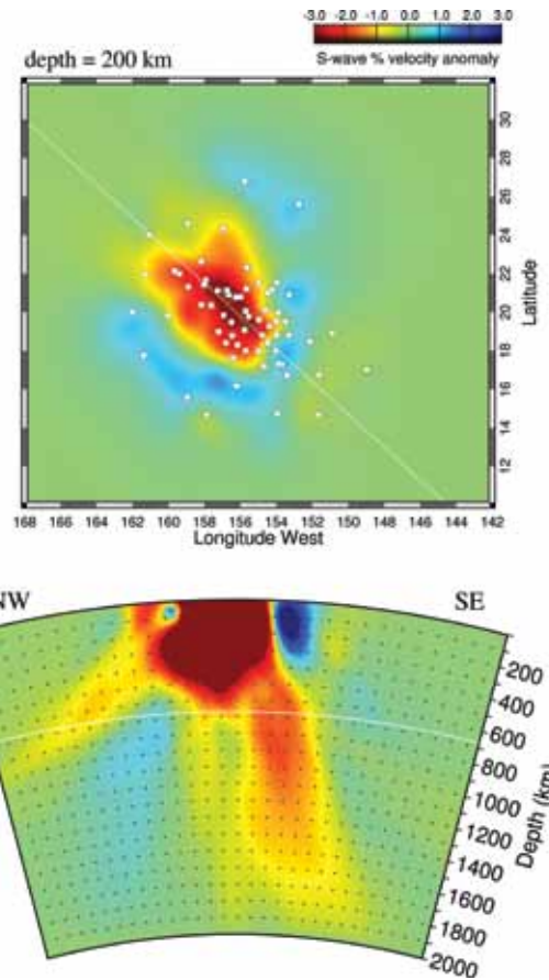
Top plot: Upper mantle shear-wave velocity heterogeneity at 200 km depth. Station locations are indicated by squares. The scale is given at the upper right and ranges \pm 3\% . Bottom plot: Vertical cross section. The scale ranges over \pm 1\% .
