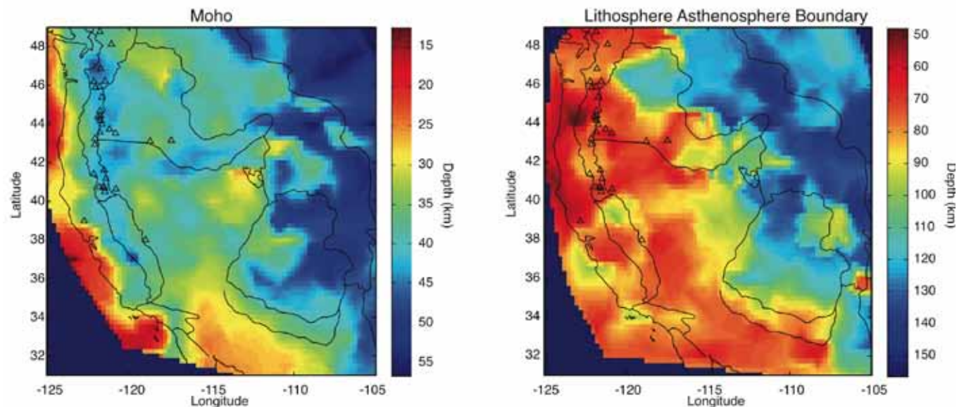
Maps of Moho (left) and LAB (right) in the western U.S. determined from a combination of SdP and PdS receiver functions. The Moho depths have been spot checked against some active source results, the LAB depths against some surface wave inversion results, both with very good agreement.
