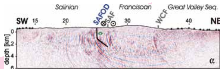
Steep-dip prestack depth migrated image. The shots used to produce the image are indicated on top. The section was normalized for subsurface coverage.
