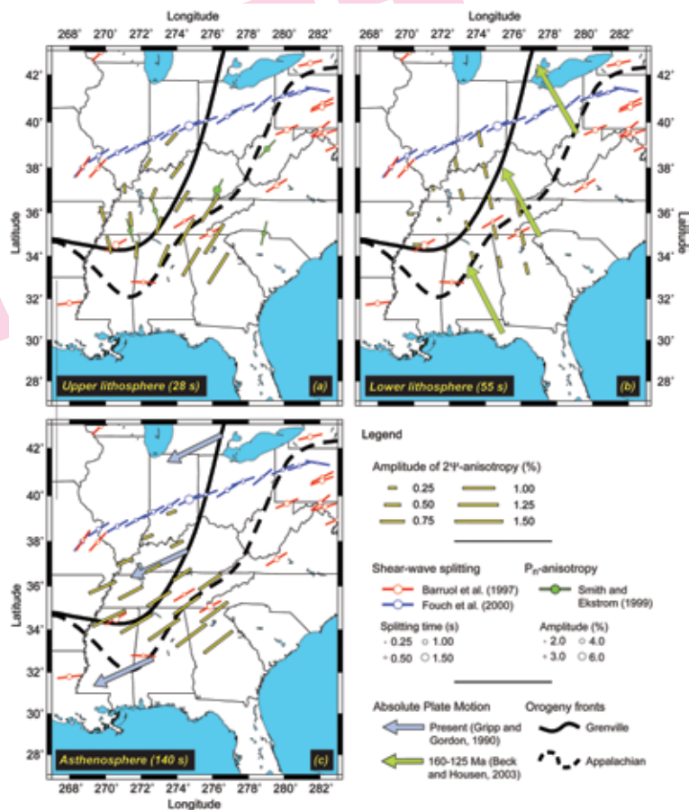
Rayleigh wave azimuthal anisotropy (yellow bars) at 28, 55, and 140 s. The orientation and size of the bar show the direction of fastest propagation of Rayleigh waves at the period and the amplitude of the anisotropy, respectively. Also plotted are main tectonic boundaries, past and present absolute plate motion, and previous anisotropy measurements. (a) At 28 s, the Rayleigh-wave fast-propagation direction beneath orogenic provinces is roughly parallel to the Grenville and Appalachian fronts, as well as to Pn fast-propagation direction. (b) At 55 s, the fast-propagation azimuth is close to the direction of the NNW drift of the North American plate during the Mesozoic. (c) At 140 s, the fast-propagation direction is parallel to the current absolute plate motion, as well as to most fast-propagation directions inferred from shear-wave splitting observations in the area.
