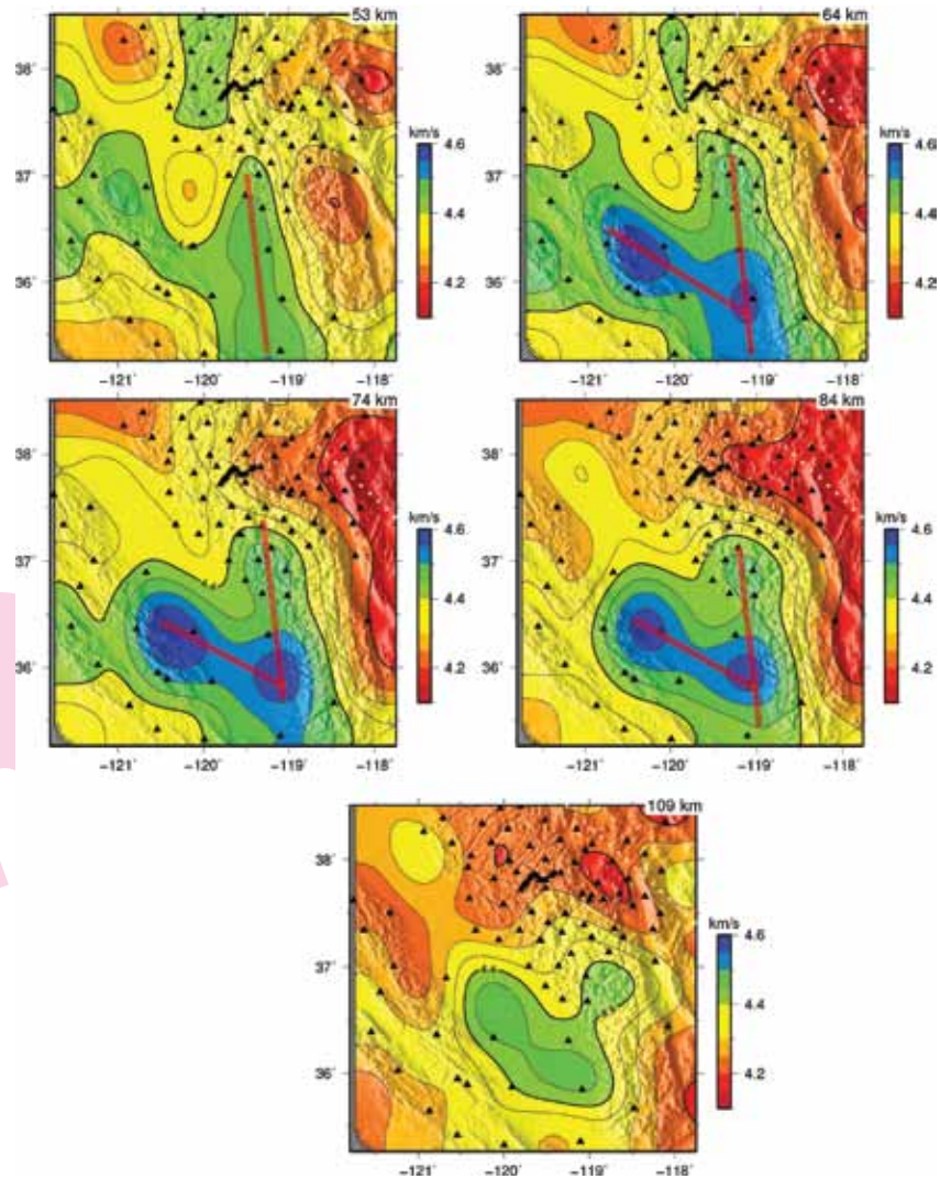
Shear velocity image from inversion of ambient and earthquake Rayleigh wave dispersion measurements using SNEP and Transportable array data.
