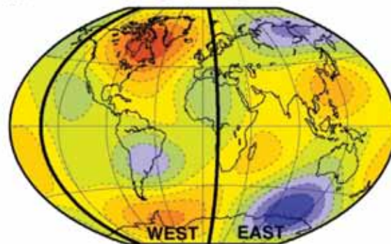
(B) Cross-coupling splitting function 16S5 - 17S4
