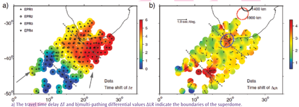
a) The travel time delay \Delta T and b) multi-pathing differential values \Delta LR indicate the boundaries of the superdome.
