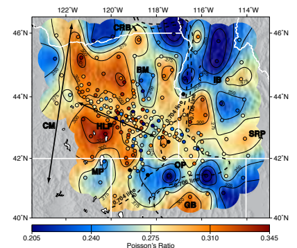
Figure 3: Map of Poisson's ratios derived from H-k stacking analysis. Smoothing parameters and geological/geochemical features are the same as in figure 1. Black solid lines denote 0.025 contours.
