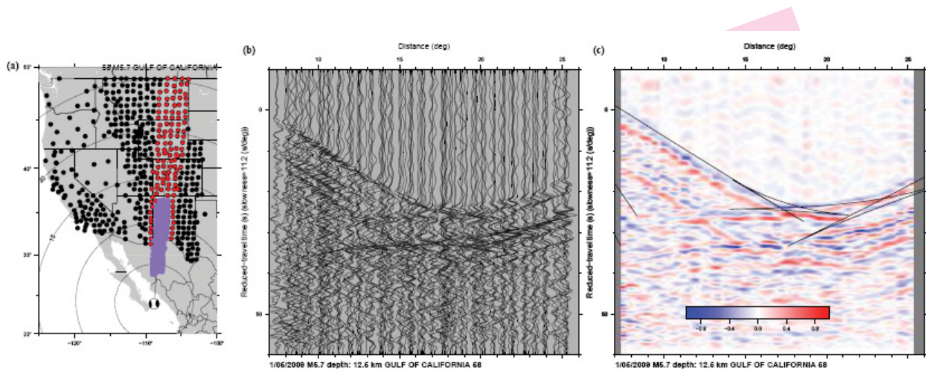
Baja California earthquake P-wave recorded by the Transportable array.
