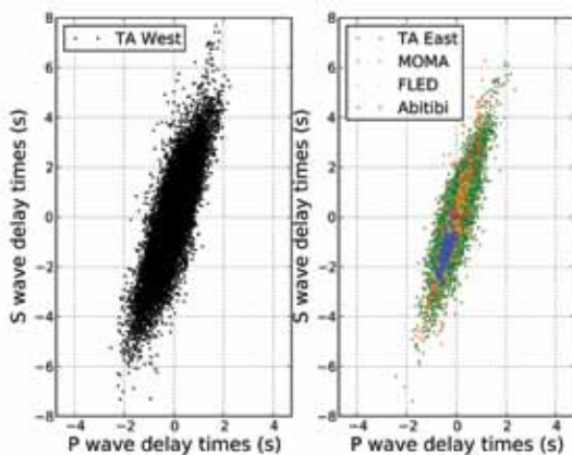
Figure 1: Station average S relative delay times for the two groups of stations west and east of the Rocky Mountains, respectively.
