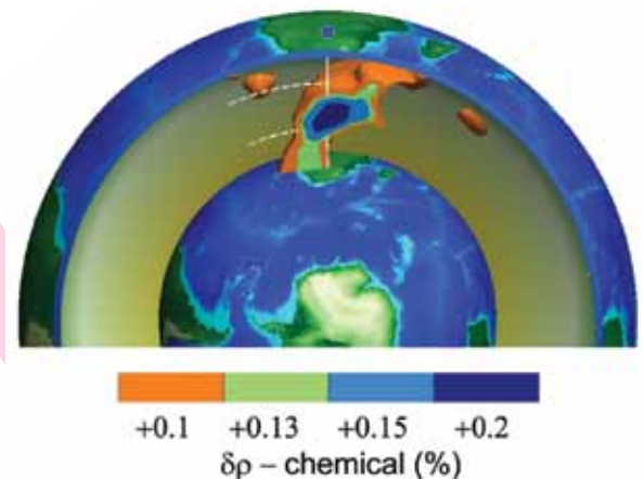
To fit geodynamic data with the thermal model shown in figure 1 additional density anomalies are needed as shown here. The "Africa Superplume" is unique in the required high chemical density anomaly needed to fit the geodynamic data.
