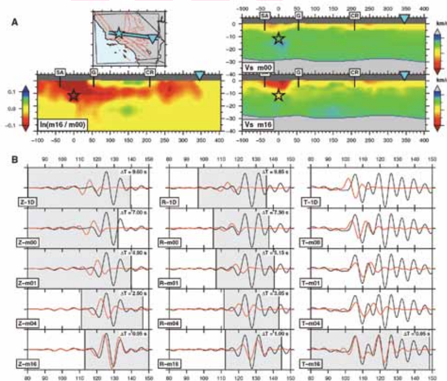
Iterative improvement of a three-component seismic seismogram. (A) Cross section of the V_s tomographic models for a path from a Mw 4.5 earthquake (star) on the White Wolf fault to station DAN (triangle) in the eastern Mojave Desert. Upper right is the initial 3D model, m00; lower right is the final 3D model, m16; and lower left is the difference between the two, \ln(m16/m00) . Faults labeled for reference are San Andreas (SA), Garlock (G), and Camp Rock (CR). (B) Iterative three-component seismic waveform fits to data for models m00, m01, m04, and m16. Also shown are synthetic seismograms computed for a standard 1D model. Synthetic seismograms (red) and recorded seismograms (black), filtered over the period range 6 to 30 s. Left column, vertical component (Z); center column, radial component (R); right column, transverse component (T). Inset "DT" label indicates the time shift between the two windowed records that provides the maximum cross-correlation.
