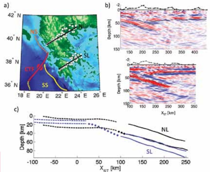
Figure 1: a) Map of study area showing location of southern segment (SS) and northern segment of western Hellenic subduction zone separated by the Cephalonia transform fault (CTF). White circles denote station locations for NL and SL deployments. b) Images of perturbation in S-wave velocity for SL (top) and NL (bottom) at -5% to +5% (red to blue). Solid lines delineate top and bottom of low-velocity layer, and the Moho of overriding plate. X-axis is horizontal distance perpendicular to strike measured from the intersection of SL with the trench of southern segment (solid yellow line in a). c) Comparison of subducted crusts imaged from marine seismics (dashed) and this study (solid) for NL (black) and SL (blue), with dots showing smooth interpolation.
