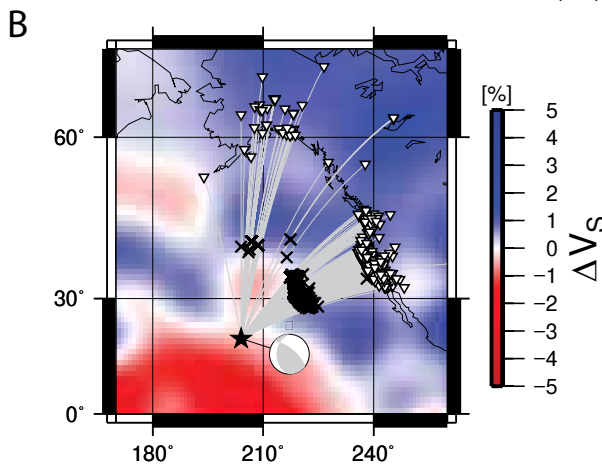
A) Seismic section (ground velocity) of the recorded aftershock recorded at the Southern California seismic network. Data have been bandpass filtered with corner frequencies of 0.7 Hz and 2 Hz. Data have been aligned on the theoretical PcP arrival for IASP91. Theoretical arrival times for several body waves are marked. B) Map of source (star) and receiver (inverted triangle) combination. PcP CMB reflection points are marked by crosses. Background shows S-wave seismic velocities from a tomographic model (Ritsema and van Heijst, 2002). Great circle paths are marked as thin grey lines and the double couple solution for the earthquake is also given.
