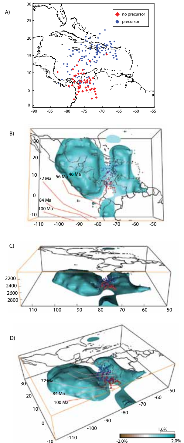
A) Map of the Caribbean region showing the calculated points of ray paths exiting the core and entering the mantle. Blue circles indicate the events with precursors, with a good (> 5) signal to noise ratio and red diamonds indicate the events with no evident precursor, which also have a good (> 5) signal to noise ratio. B-D) Tomographic images of the lower mantle (Grand, 2002) with isosurfaces of 1.6% shear velocity perturbation and greater. The exit points are also plotted with the images showing the localization of the scatterers and their relationship to the surrounding high velocities. The red lines (and ages) are the estimated Farallon plate boundaries from plate and kinematic reconstructions between 100 and 46 Ma (Pindell et al. , 2005).
