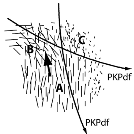
A schematic representation of three distinct anisotropic domains in the IC where the strength and orientation of fast crystallographic axes are shown as straight lines. Two different PKPpdf ray paths are shown sampling different domains. "A" represents a semi-constant anisotropic domain with a predominant alignment of fast anisotropic axes; "B" is a transitional domain with a mixed orientation of fast anisotropic axes, and "C" is an isotropic or a weakly anisotropic domain. The arrow in the middle represents the net direction of the fast axis of anisotropy.
