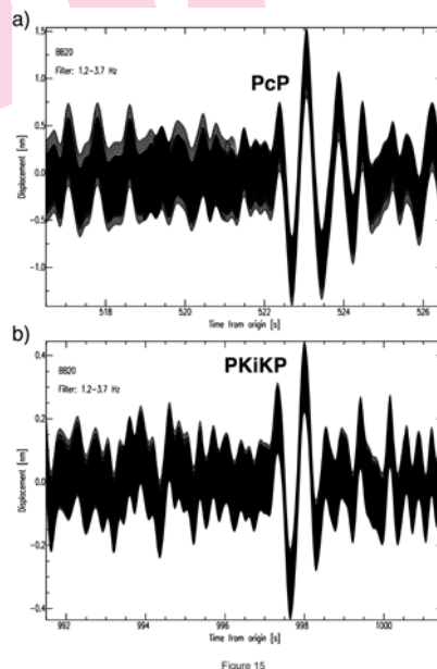
Figure 15 The subtraction of bandpass-filtered (1.2-3.7 Hz) seismic noise preceding the PKiKP waves from the PKiKP-wave signal recorded at station BB20 for the same event. 500 consecutive, 14 second long sliding windows of noise time series are calculated by shifting the time series by 1 sample toward earlier time and are then subtracted from the bandpass-filtered PKiKP-wave signal. Only 10 seconds of the time series are shown for clarity. Compare with Figure 1.
