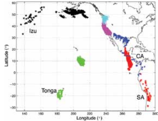
Map of PcP data stacking configurations; earthquake epicenters (stars), recording stations in western North America (triangles), and PcP midpoints (small dots). The red, blue, green, and black colour earthquakes and midpoints are the South America (SA), Central America (CA), Tonga, and Izu data sets, respectively. The CA events were recorded by University of Washington short period stations (cyan triangles), all other data sets incorporate broadband and short-period data from the TriNet, SCSN and NCSN networks (magenta triangles). All data shown have been screened to ensure a stable PcP detection in individual event stacks. About a third (half) of the Tonga (Izu) data are a screened subset of the data used by Revenaugh and Meyer (1997).
