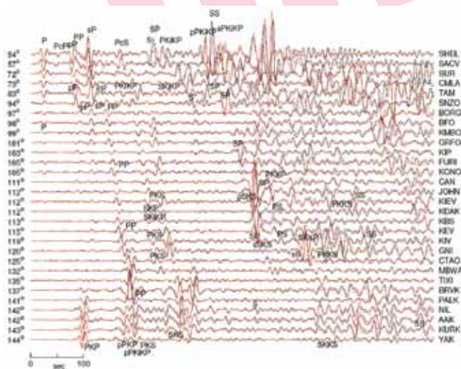
Vertical component record section comparing data (black) and SEM synthetics (red) for the September 3, 2008, Mw = 6.3 Santiago del Estero, Argentina earthquake, which occurred at a depth of 571 km. The records are aligned on the P wave, plotted as a function of epicentral distance, and bandpass filtered between 17 s and 60 s. Major seismicological body wave arrivals are labeled. Epicentral distance is plotted to the left of each set of traces, and FDSN station identification codes are plotted to the right.
