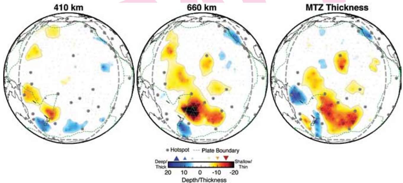
Topography maps for discontinuity depths and transition zone thickness in our Pacific study region. The depths are plotted relative to average values of 418 km, 656 km, and an average transition zone thickness of 242 km.
