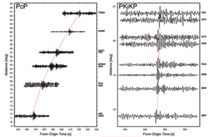
Selected PcP (left) and PKiKP (right) observations for the mb=5.7 earthquake located northwest of Kuril Islands and dated 02/07/2001. The broadband velocigrams are band-pass filtered between 1 and 3 Hz. The theoretical travel time prediction of PcP and PKiKP from the ak135 model is shown by solid line. The scales for PcP and PKiKP records are different to account for the space and changing slowness across the range of selected stations.
