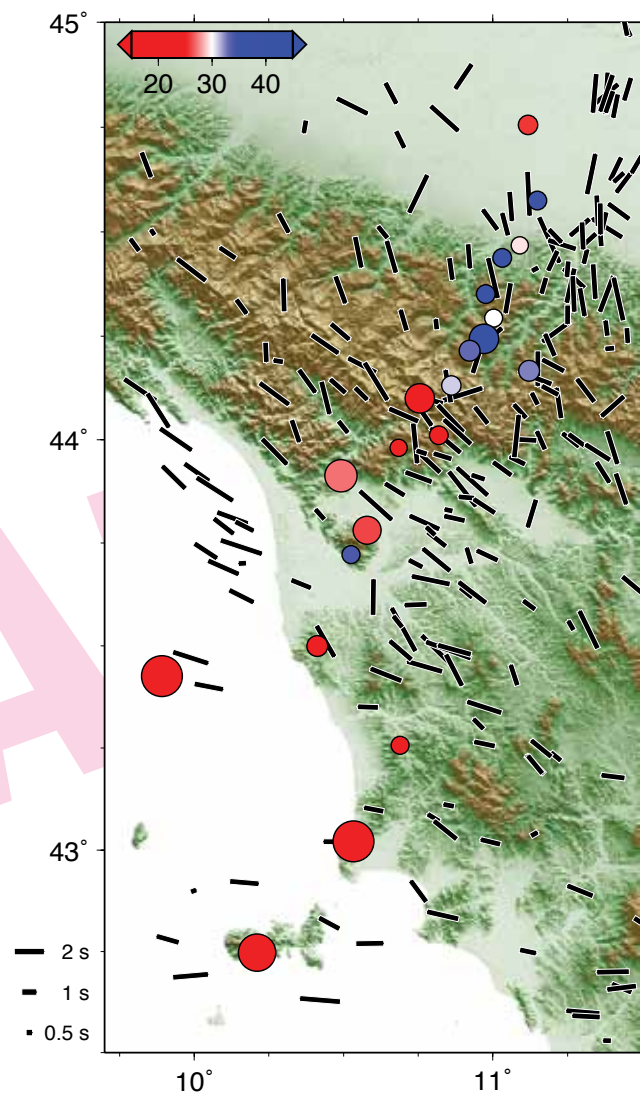
A topographic map illustrates a spatial coincidence of changes in inferred crustal thickness values (circles with depth-scaled color) and observed fast polarization directions of split shear waves (black bars). Circle size is proportional to confidence in the result (largest are most certain). Splitting observations are scaled with delay and aligned with the fast polarization. Both types of observations change dramatically across the highest part of the Apennines.
