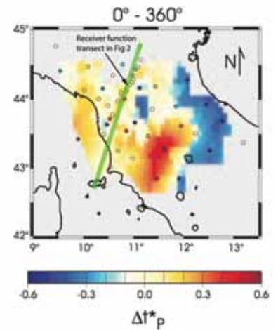
Figure 1. Spatial distribution of \Delta t^* , an estimate for seismic attenuation based on the high-frequency rolloff of P body-wave spectra recorded in Central Italy by the RETREAT deployment. The map interpolates the average \Delta t^* estimates at each station. The average \Delta t^* values at stations are shown as colored circles. The green line locates the receiver-function transect of Figure 2.
