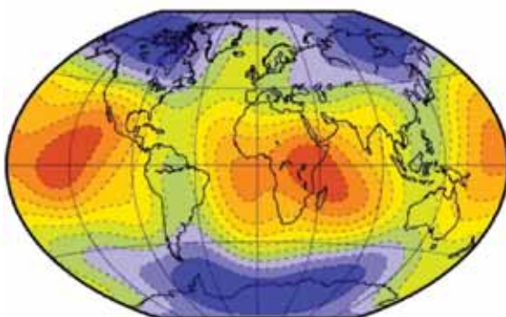
(A) Self-coupling splitting function 16S5
