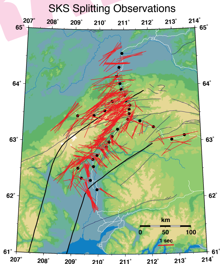
Figure. Compilation of SKS splitting results. Each measurement is plotted as a red line parallel to the fast direction, with length proportional to the delay time. The observations are plotted at the 100 km depth projection of the ray, in order to demonstrate the back-azimuthal pattern. Locations of seismic stations from the BEAAR experiment are shown by the black dots. Thick black lines show contours to slab seismicity (50 and 100 km). Thin dark lines show active faults, and white lines show roads.
