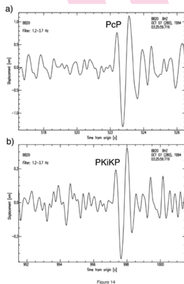
Figure 14 Bandpass-filtered ground displacements recorded at station BB20 using an optimal filter of 1.2-3.7 Hz for a nuclear event in China. Clear observations with similar waveforms of the PcP and PKiKP waves are visible.
