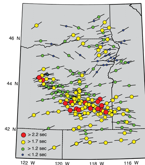
Map of average shear wave splitting parameters in the High Lava Plains and surrounding regions. Estimates were obtained by a simple average of the highest-quality measurements at each station. The symbols are color-coded by the magnitude of the delay time, as indicated by the legend at bottom left.
