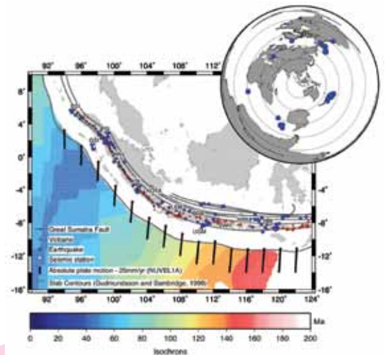
Map showing stations and events used in this study. White inverted triangles mark stations, blue circles show earthquakes (local events on main map, teleseismic events on top right map). Also shown are quaternary volcanoes (red triangle), absolute plate motions (Gripp and Gordon (1990), black arrows), slab contours at 100 km depth intervals (Gudmundsson and Sambridge, 1998), the Great Sumatra Fault, and Isochrons (Müller et al., 1997).
