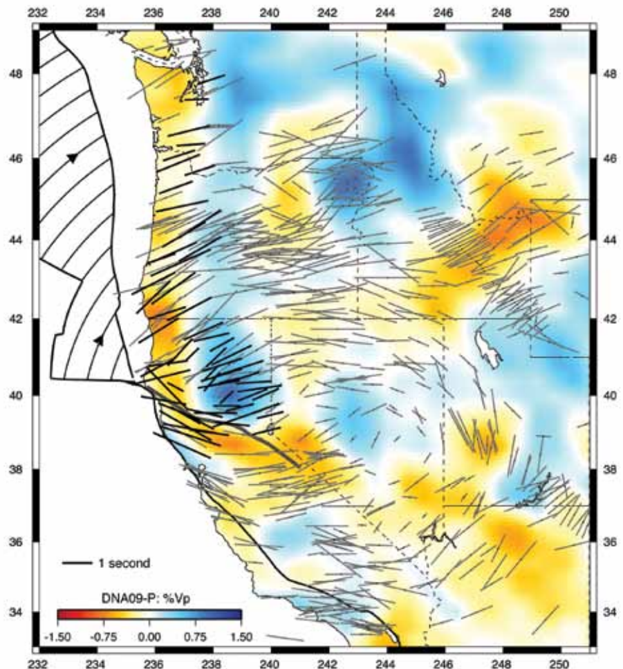
Figure. Regional splitting pattern overlain on the vertically averaged upper mantle velocity anomaly. Our splitting results are shown in black and those of previous studies are in grey (Long et al., 2009; Wang et al., 2008; West et al., 2009; Zandt and Humphreys, 2008 and references therein). The splitting pattern is shown to be uniform trench-normal throughout Cascadia. The velocity anomaly shown is a vertical average of the velocity anomaly from the DNA09 P-wave model over the 100-400km depth range (Obrebski et al., 2010). The slab is imaged as the north-south high velocity feature. The splitting measurements rotate around the southern end of the slab. Curved black lines on the G-JdF plate represent the direction of its absolute plate motion.
