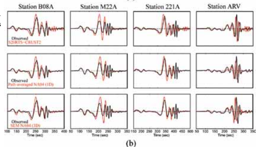
(a) The Nevada Earthquake (Mw 6.0) indicated as a star was recorded at over 400 broadband stations in USArray indicated as triangles. Some stations are surrounded by red circles where observed waveforms are obtained to be compared with synthetics. (b) Comparison between observed waveforms and several synthetics at stations surrounded by red circles in (a).
