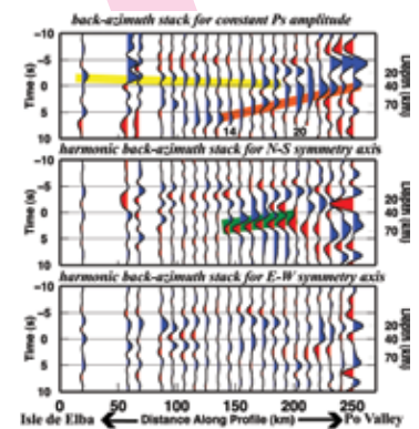
Figure 2. RF data-set along cross-Apennines transect, stacked with constant, \cos\phi (N-S) and \sin\phi (E-W) back-azimuth weighting. Blue and red pulses indicate positive and negative Ps converted-wave amplitudes, respectively. Colored stripes highlight the main features: yellow for the Tyrrhenian Moho, orange for Adriatic Moho and green for the layer atop the Apennines slab. The Y-axis shows RF delay time (depth), in s (km) referenced to a stacking-migration target at 40-km depth, so that pulses at negative delay time correspond to interfaces shallower than 40 km.
