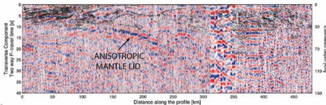
Superposition of line-drawing reflection section of Cook et al. (1999) upon transverse component receiver function. Note teleseismic signature of anisotropic mantle lid that parallels reflections from subducted crust.
