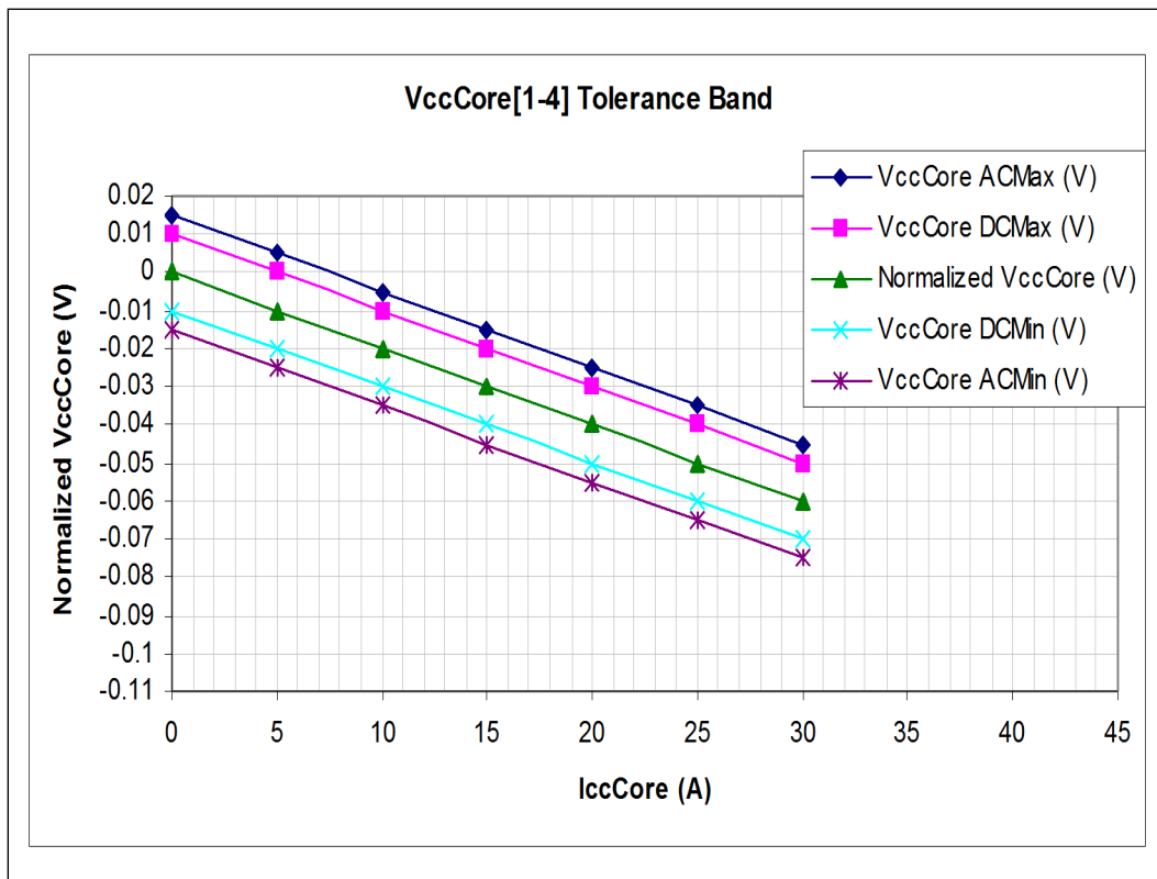
Figure 2-15. V CC CORE Load Line for the Intel® Itanium® Processor 9500 and 9700 Series
