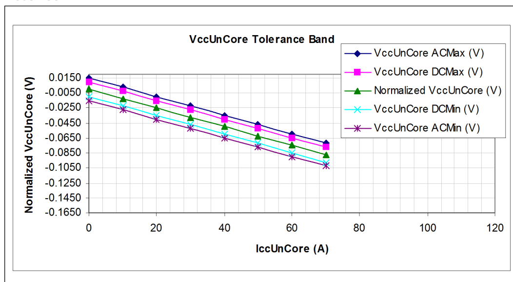
Figure 2-14. V CCUNCORE Load Line for the Intel® Itanium® Processor 9500 and 9700 Series
