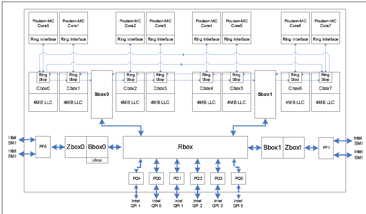
Figure 1-2. Intel® Itanium® Processor 9500 and 9700 Series Processor Block Diagram
