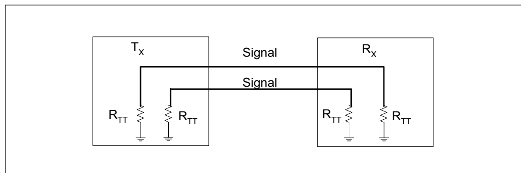
Figure 2-1. Active ODT for a Differential Link Example
