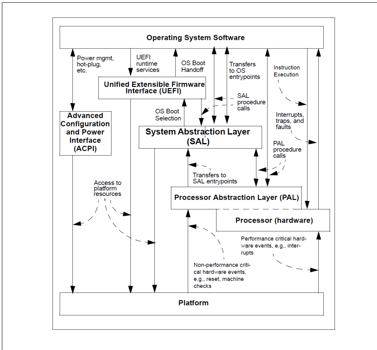
Figure 1-3. Intel® Itanium® Processor 9500 and 9700 Series Firmware Diagram
