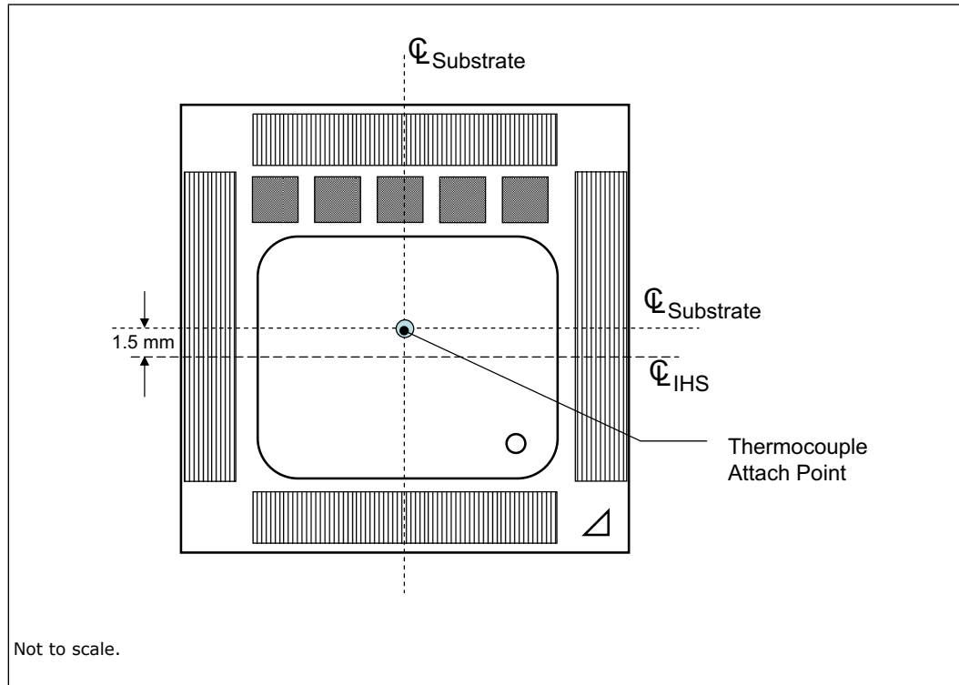
Figure 5-2. Intel® Itanium® Processor 9300, 9500 and 9700 Series Package Thermocouple Location
