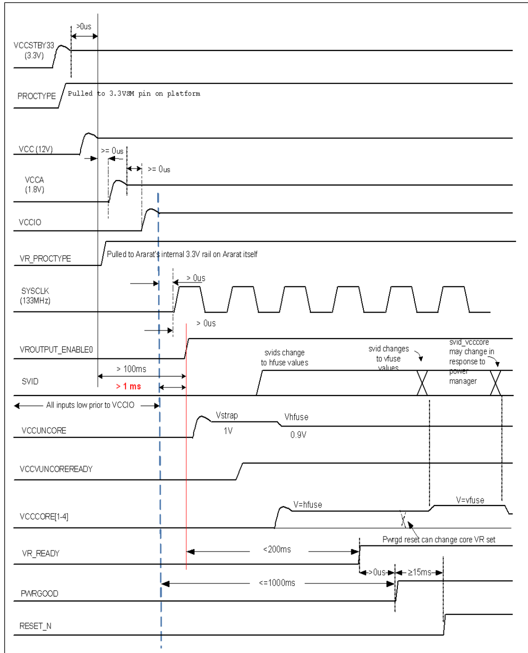
Figure 2-18. Supported Power-up Sequence Timing Requirements for Intel® Itanium® Processor 9500 and 9700 Series
