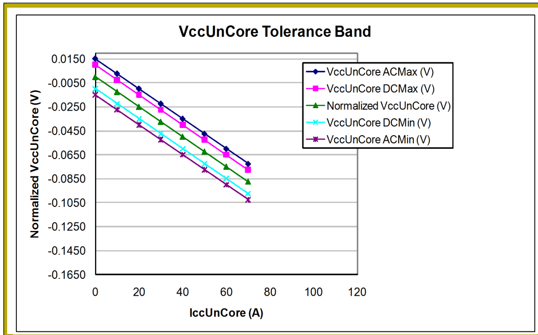
Figure 2-13. V CCUNCORE Static and Transient Tolerance for the Intel® Itanium® Processor 9500 and 9700 Series
