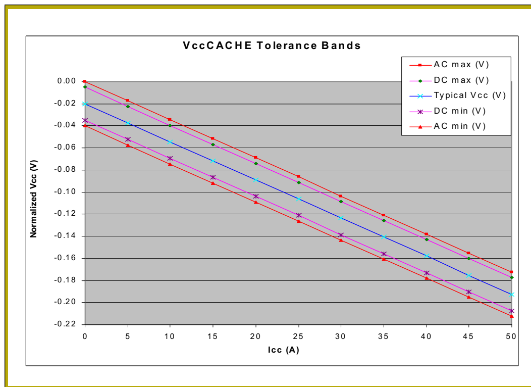
Figure 2-12. V_{CCACHE} Static and Transient Tolerance for Intel® Itanium® Processor 9300 Series
