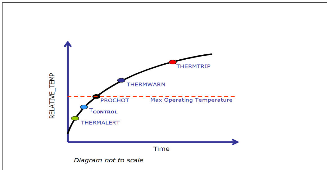
Figure 5-1. Intel® Itanium® Processor 9300, 9500 and 9700 Series’ Thermal States
