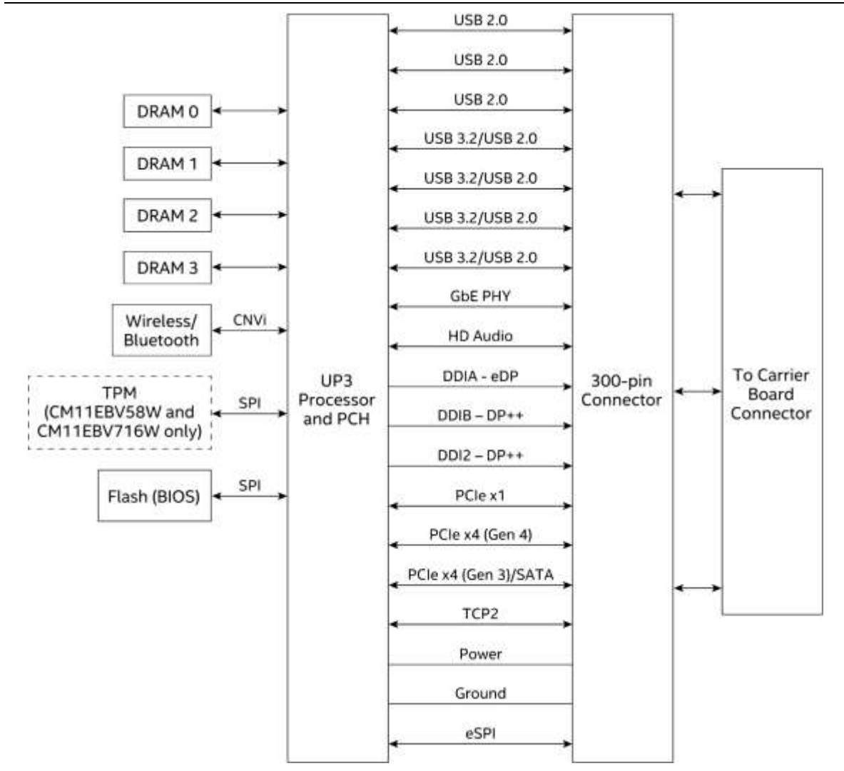
Figure 1. Block Diagram
