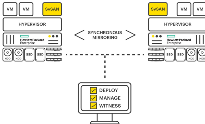
Figure 2 StorMagic SvSAN cluster on HPE servers
