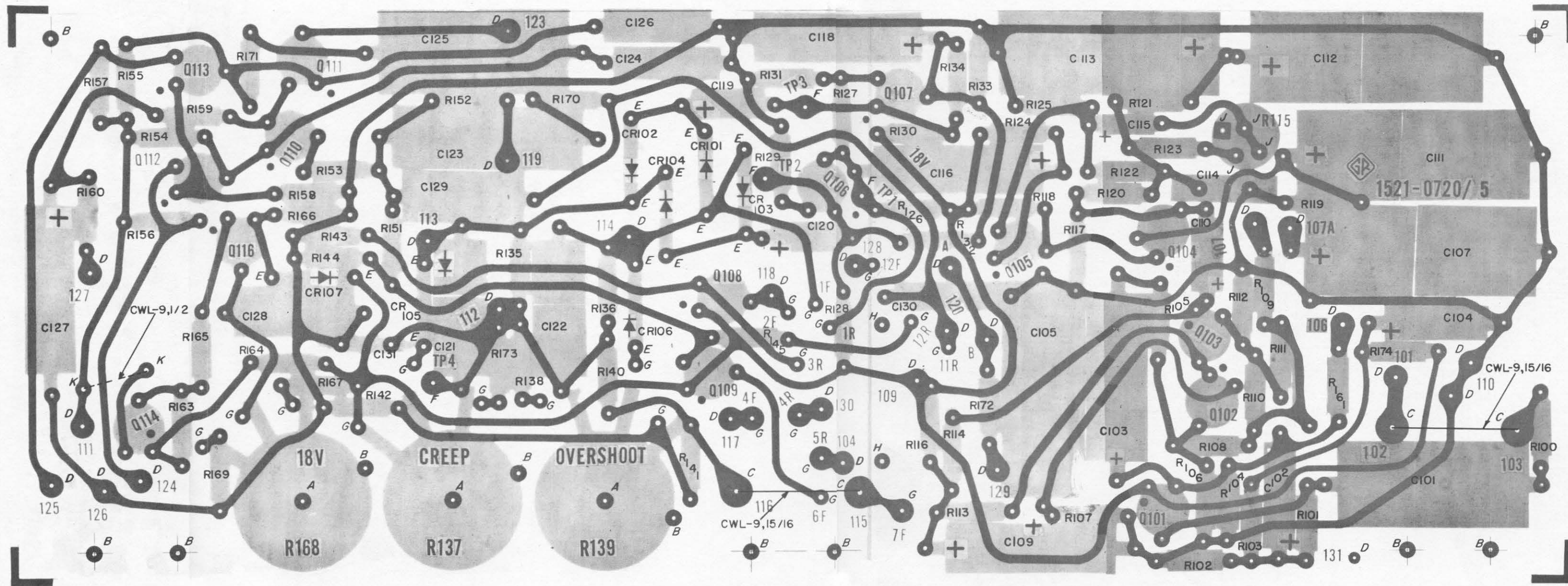
Figure 6.7. Etched-board assembly for the Type 1521-B Graphic Level Recorder (P/N 1521-2721).
