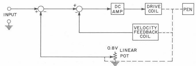
Figure 4.2. Block diagram of servo loop for dc recording.
