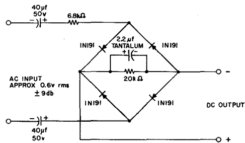
Figure 5.13. Detector circuit diagram.
