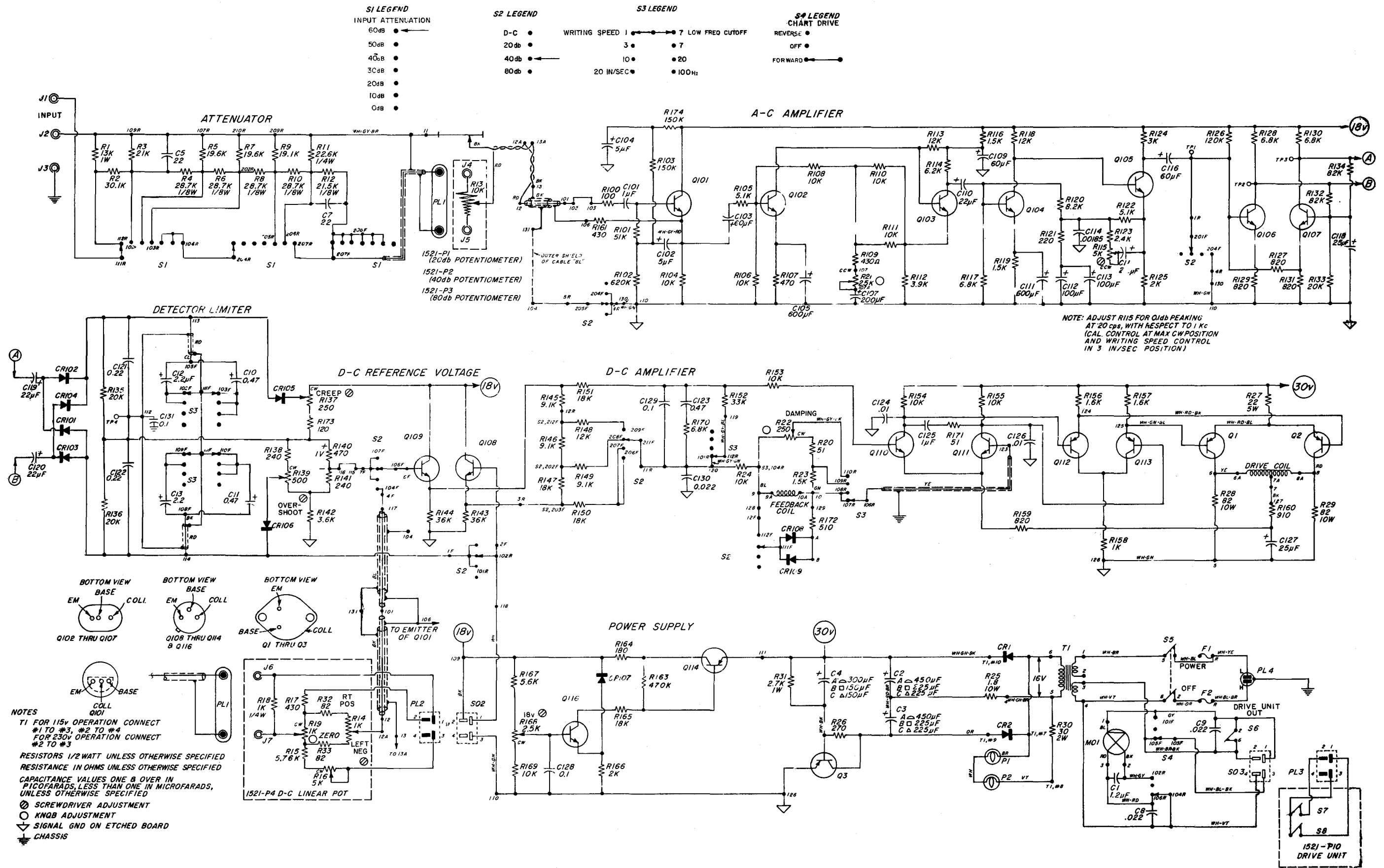
Figure 6.8. Schematic diagram for Type 1521-B Graphic Level Recorder.
