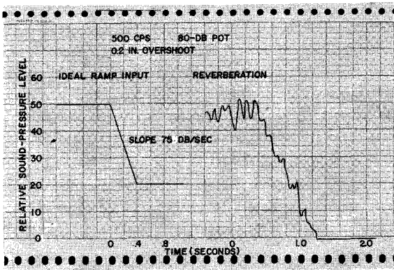
Figure 4.3. Recording of ramp-type input.
