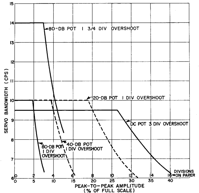
Figure 4.9. Servo bandwidth vs amplitude of excursions.
