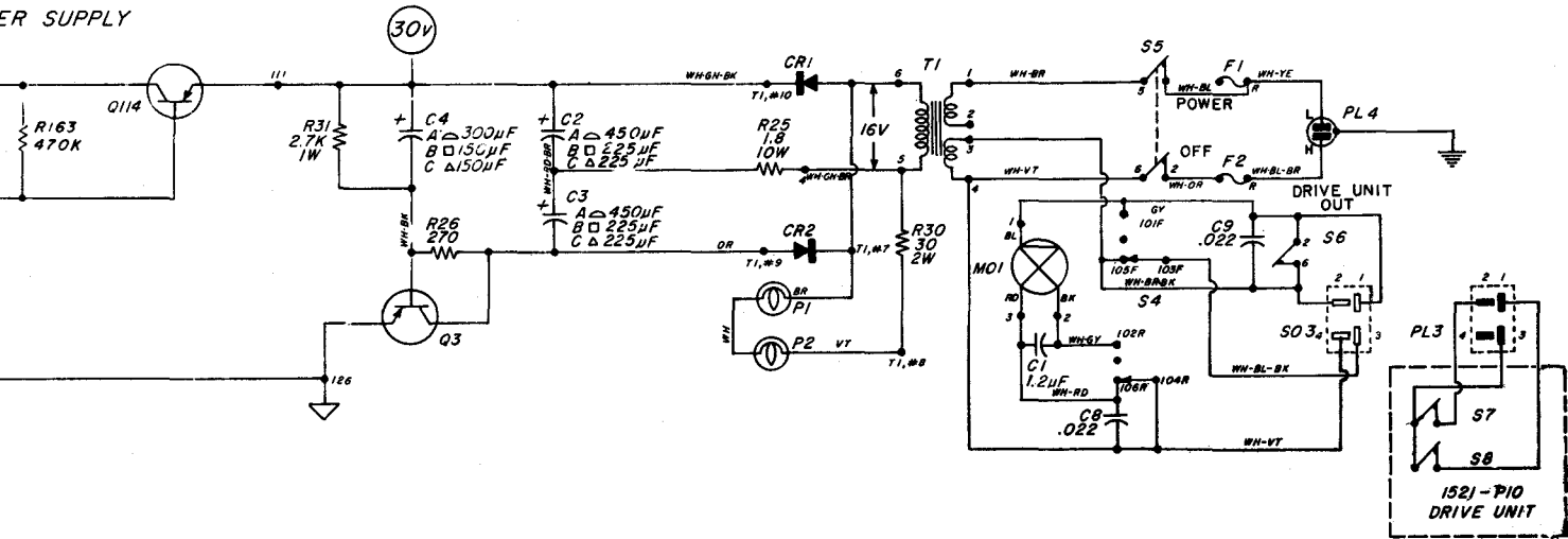
Figure 6.8. Schematic diagram for Type 1521-B Graphic Level Recorder.
