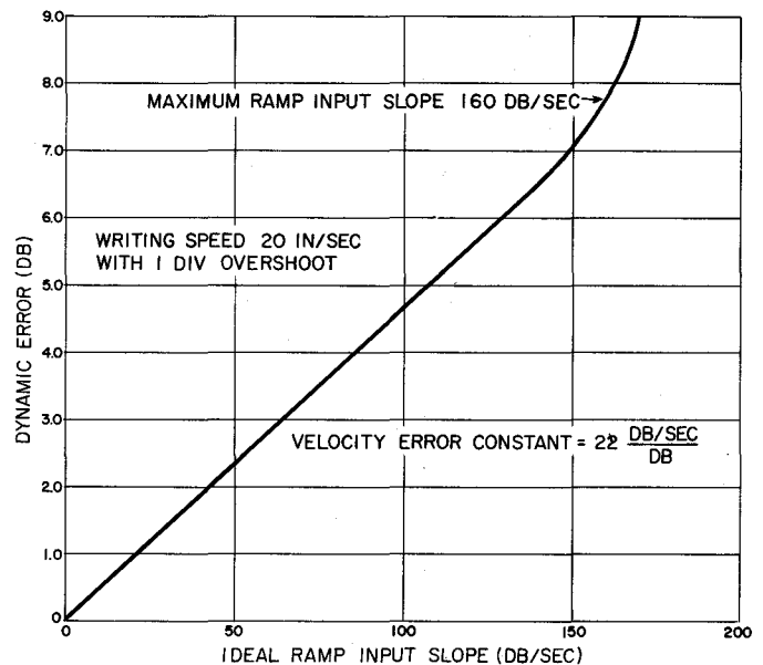
Figure 4.5. Dynamic error for 20-, 40-, and 80-db potentiometers.
