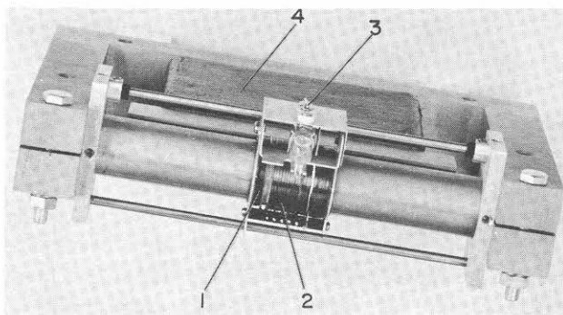
Figure 4.1. View of magnetic structure and pen motor.
