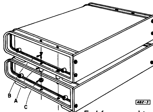
End frame stacking diagram
