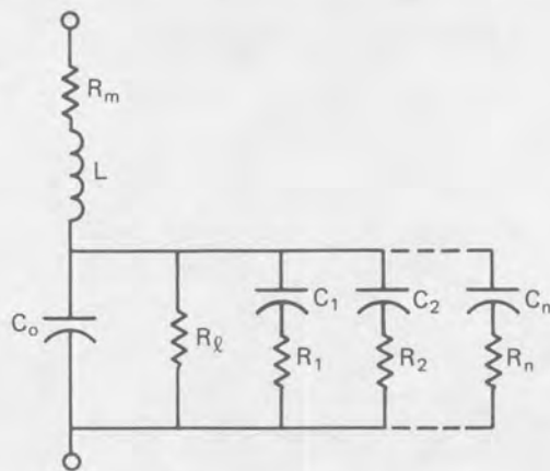
Figure 1. A capacitor equivalent circuit.
