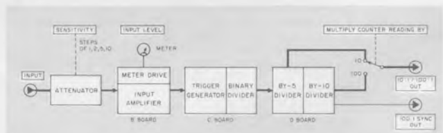
Two frequency-divider circuits allow an output that is one-tenth the input frequency or one-hundredth of it.
