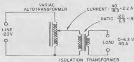
Figure 6. Low-voltage output.
