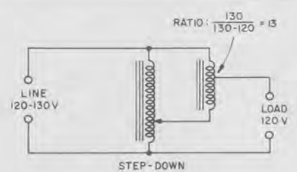
Figure 8. Step-down circuit for high line voltage
