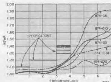
Typical and specified SWR
