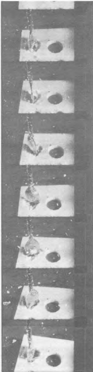
The 1540 is a valuable, economical, high-speed photographic tool. This sequence follows the action of a 2000-rpm wood bit going through a piece of particle board.
