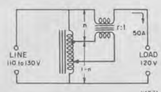
Figure 11. Constant-voltage output.
