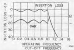
Typical insertion loss and SWR:
