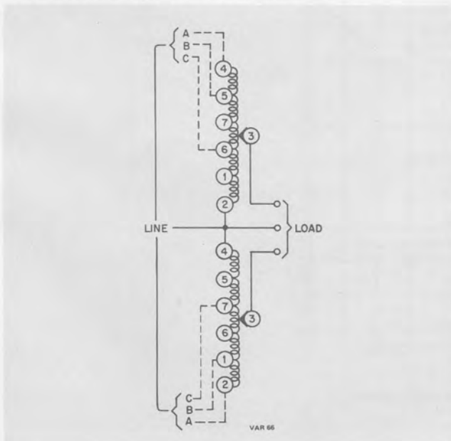
Three phase, two gang; open delta.
