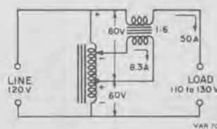
Figure 10. Overtension output.
