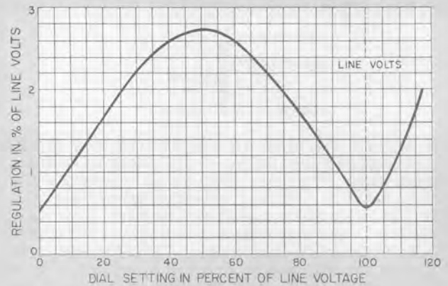
Typical regulation curve with normal rated current.
