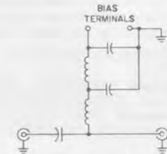
Schematic Diagram of 874-FBL
