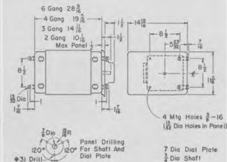
Dimensions Ganged Cased Types W30G2M, W30G3M, W30G4M, W30G6M, W30HG2M, W30HG3M, W30HG4M, and W30HG6M
