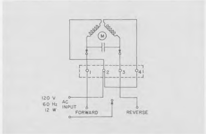
Schematic diagram of motor circuit
