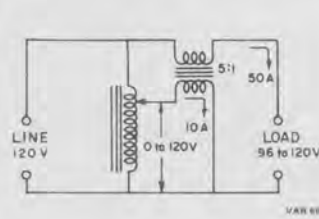
Figure 7. Line-voltage output.
