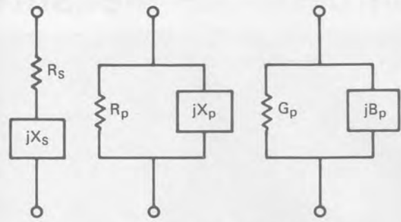
Figure 1. Series and parallel components of impedance.
