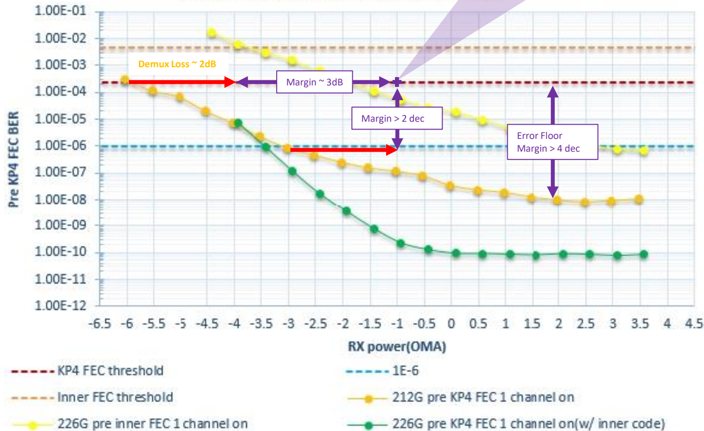
212G vs 226G lane2 BER curve
