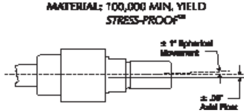
Standard AC Coupler AC250 - AC5000
