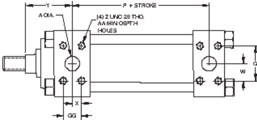
FLANGE PORT (3000 PSI Rating) (available on 'H' Series only)
