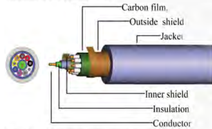
DX0109A Spiral shield leadwire
