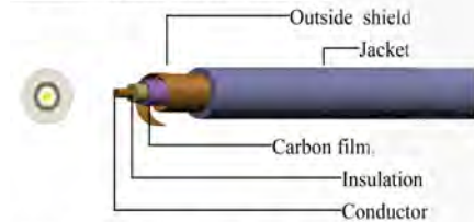
DX0281A Dibrillation cable
