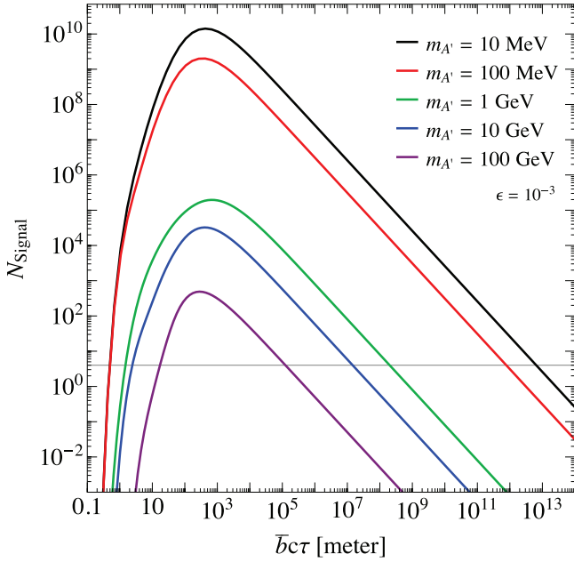
Figure 62. Projections at MATHUSLA for the case that the dark photon decays to two LLP's. The number of signal is presented in terms of b\bar{c}\tau of the LLP for different dark photon masses. Here, \epsilon = 10^{-3} is used, and N_{\text{Signal}} is proportional to \epsilon^2 . For m_{A'} = 10\text{MeV} and m_{A'} = 100\text{MeV} , the dominant dark photon production process is meson decay, and bremsstrahlung of dark photon for higher masses. The grid line is for N_{\text{Signal}} = 4 . \bar{b} 's from the numerical simulations are \bar{b} = 1.7m_\pi/m_{\text{LLP}} for m_{A'} = 10\text{MeV} and m_{A'} = 100\text{MeV} , \bar{b} = 2.0m_{A'}/m_{\text{LLP}} for m_{A'} = 1\text{GeV} , \bar{b} = 0.80m_{A'}/m_{\text{LLP}} for m_{A'} = 10\text{GeV} , and \bar{b} = 0.45m_{A'}/m_{\text{LLP}} for m_{A'} = 100\text{GeV} . This estimate assumes the 200\text{ m} \times 200\text{ m} \times 20\text{ m} benchmark geometry of figure 1.
