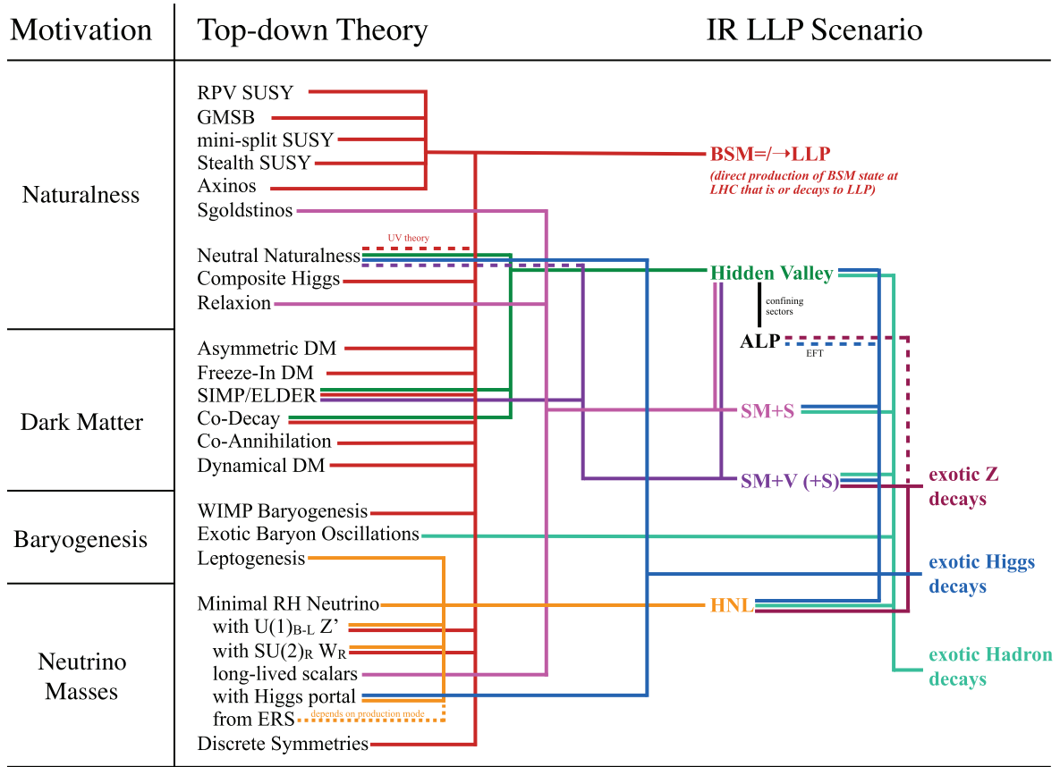
Figure 72. Qualitative overview of the top-down theory motivations for neutral LLPs discussed in this document, with colored lines (from left to right) indicating which IR LLP scenario they motivate at the LHC. Some of the IR LLP scenarios or simplified models in turn motivate specific signatures like exotic Higgs decays. We stress that these top-down theories are not the only motivations for the IR scenarios or simplified models shown here: hidden valleys, exotic Higgs decays, etc, are also motivated in their own right on generic, bottom-up grounds.
