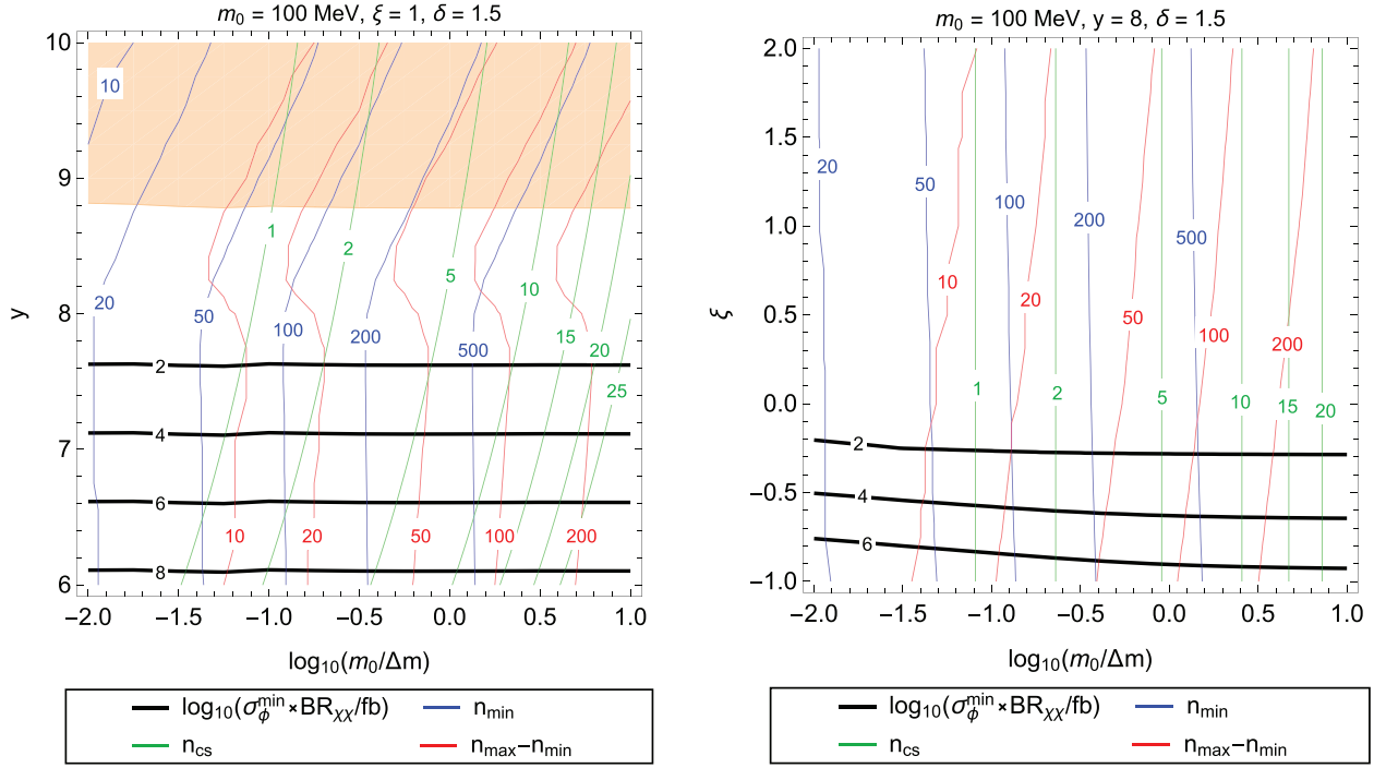
Figure 33. The reach of MATHUSLA within the DDM parameter space for the benchmark values m_0 = 100 MeV and \delta = 1.5 . Black curves indicate contours of \sigma_\phi^{\min} \text{BR}_{\chi\chi} , while blue, red, and green curves indicate contours of n_{\min} , n_{\max} - n_{\min} , and n_{\text{cs}} , respectively. Likewise, the orange shading indicates the region of DDM parameter space in which at least one of the ensemble constituents \chi_n has a characteristic decay length \beta\gamma c\tau_{\min} < 1 m. As discussed in the text, the region with m_0/\Delta m \gtrsim 0.1 , 7.5 \lesssim y \lesssim 8.8 , and \xi \gtrsim -0.3 is a particular ‘sweet spot’ in which multiple light states within the DDM ensemble comprise the present-day dark matter while numerous heavier states within the same ensemble can lead to an observable signal at MATHUSLA. This estimate assumes the 200 \text{ m} \times 200 \text{ m} \times 20 \text{ m} benchmark geometry of figure 1.
