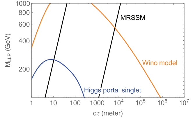
Figure 35. MATHUSLA reach for the models described in section 6.1.3 for long-lived particle masses M_{LLP} = 0.1\text{--}1 TeV and decay lengths c\tau > m for 14 TeV HL-LHC, computed using the analytical approximations outlined in section 3.1.1. (Regions between the solid lines give N_{obs} > 4 in MATHUSLA.) Note that these models give successful baryogenesis inside the full parameter space shown. The MRSSM reach projection assumes Bino LLP production in the decay of a 1.8 TeV gluino. The Higgs portal singlet projection is shown for c_H v / \Lambda_H = 0.5 . This estimate assumes the 200 \text{ m} \times 200 \text{ m} \times 20 \text{ m} benchmark geometry of figure 1.
