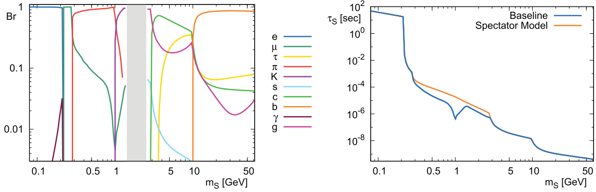
Figure 51. Left: Branching ratios of the scalar S in our baseline decay model. See text for details. Right: Scalar S lifetime of our baseline model and the spectator model for the mixing angle \theta = 10^{-6} .
