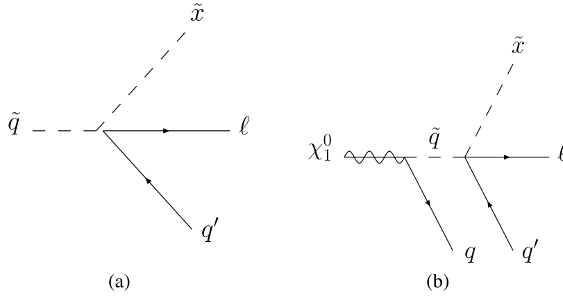
Figure 27. Left: 3-body decay of a squark LOSP directly through the interaction of equation (102), and Right: 4-body decay of a neutralino LOSP through an off-shell squark for qld^c models. Here, the quark flavors q and q' are generically different. \tilde{x} denotes the scalar component of the ADM supermultiplet X . Decay of a slepton LOSP and a neutralino LOSP through an off-shell squark is also given by the same diagrams trading a squark and a lepton with a slepton and a quark, respectively. Figure from [320].
