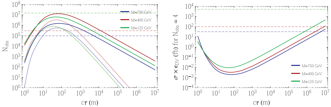
Figure 48. Left: Number of expected events in MATHUSLA with at least one (two) vertices are shown in the dark (light) lines for our three benchmark models. For the M = 400 GeV and M = 750 GeV, we assumed a cross-section equal to that of a standard model Higgs boson with this mass [580]. The 125 GeV curve assumes production in exotic Higgs decays with branching fraction 10%. Also shown is the maximum number of events allowed by the expected mono-jet limits (dashed lines). Right: MATHUSLA exclusion potential (solid), compared to the projected mono-jet limits (dashed). This estimate assumes the 200 \text{ m} \times 200 \text{ m} \times 20 \text{ m} benchmark geometry of figure 1.
