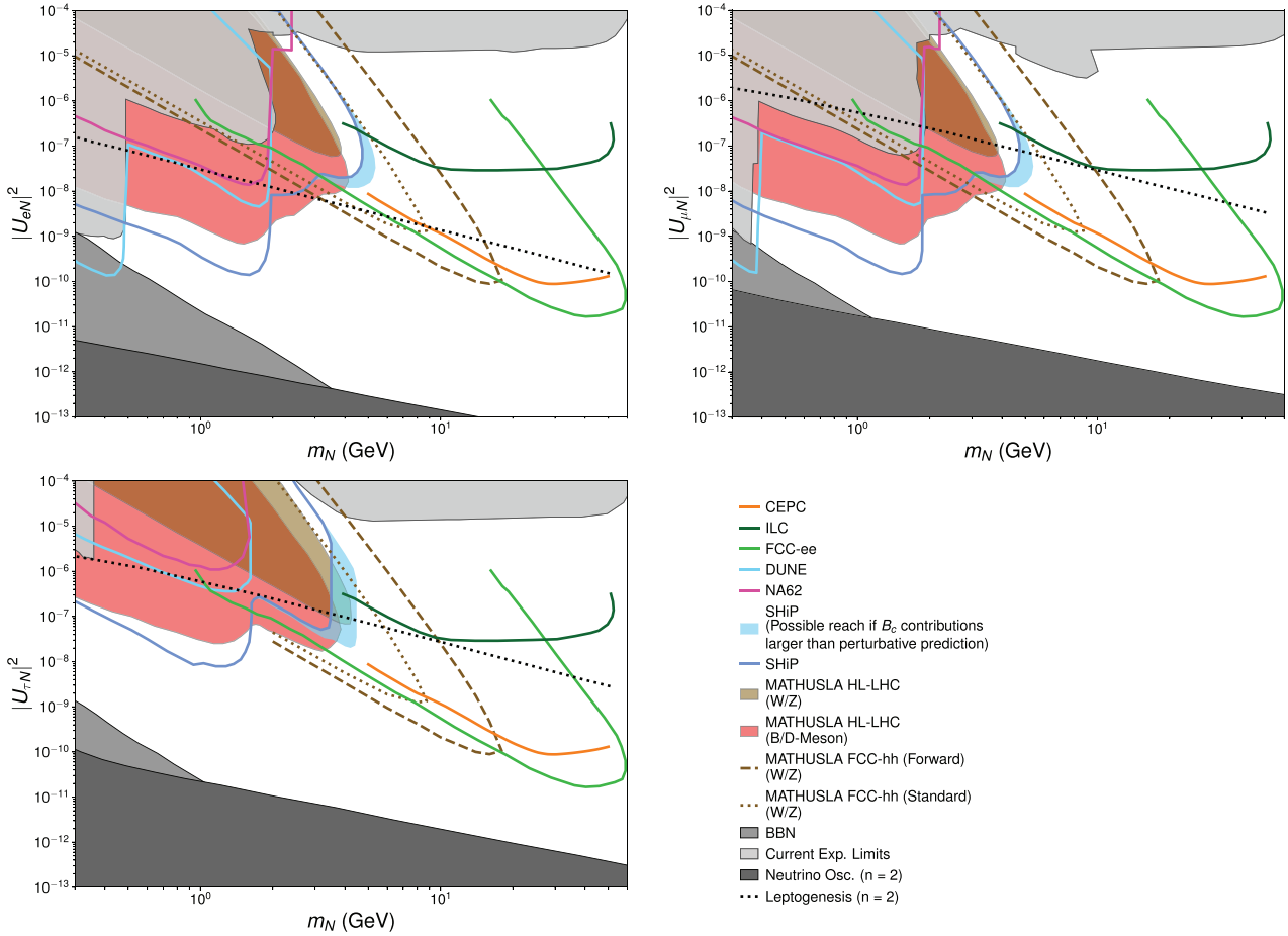
Figure 38. Projected sensitivity (4 events) in the (m_N, |U_{\alpha N}|^2) plane to sterile neutrinos, N , produced in W/Z decays at FCC-hh for MATHUSLA ‘standard’ benchmark surface version (dotted brown) and ‘forward’ version (dashed brown), see table 3 and figure 1, for \alpha = e (top-left), \alpha = \mu (top-right) and \alpha = \tau (bottom-left, only shown for m_N > 2 GeV, see text for details). Also shown are the MATHUSLA sensitivities for HL-LHC from figure 37, as well as the projected future sensitivity of various facilities: SHiP [2], FCC-ee [460], CEPC [435, 461], ILC [435, 461], NA62 [455] (see also [454]), and DUNE [502]. For the projected sensitivity of FASER, see [503], and for comparisons to other proposed LLP detectors see [2]. The light blue shaded region indicates the uncertainty in the SHiP reach due to B_c production, with \sigma(B_c)/\sigma(B) set to the LHC value at its outer boundary. The present limits on (m_N, |U_{\alpha N}|^2) from figure 37 are shown as a light-grey region. The region excluded from primordial nucleosynthesis (BBN) is shown in medium-grey. The upper limit on |U_{\alpha N}|^2 from viable leptogenesis for the minimal case n = 2 (assuming normal neutrino mass hierarchy, see [430]) and the lower exclusion on |U_{\alpha N}|^2 from the active neutrino oscillation data for the minimal case n = 2 (for normal neutrino mass hierarchy, see [430]) are respectively shown as a black dotted line and a dark-grey region. For n = 3 , the leptogenesis region extends up to the present DELPHI bounds [444, 480].
