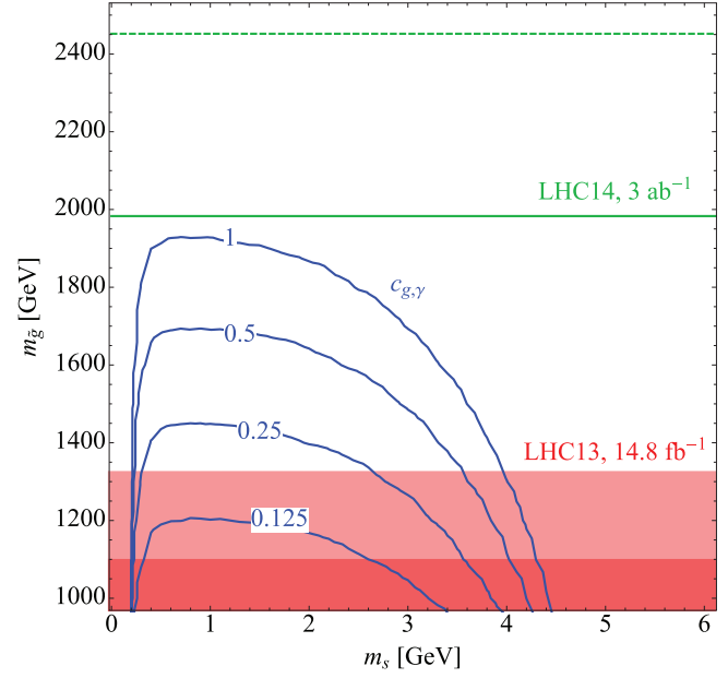
Figure 21. MATHUSLA discovery potential for Stealth SUSY. The signal arises in gluino pair production events (gluino mass is on the vertical axis), and the observed decay is a light saxion (mass on the horizontal axis) decaying to two gluons or photons. Blue curves are the reach (corresponding to 4 detected events) for various values of c_g and c_\gamma defined in equation (38). As the saxion mass approaches the axino mass (fixed here to 5 GeV), the axino begins to decay invisibly to an axion and a gravitino. Conversely, as the saxion mass falls below the two-pion threshold, the visible branching fraction of the saxion quickly becomes negligible, with the decay proceeding predominantly to a pair of axions. The red shaded regions show the current LHC exclusions for gluinos decaying to singlinos from the ATLAS RPV search [214]. The projected discovery reach at HL-LHC with 3 \text{ ab}^{-1} is shown in green. The dashed green line and lighter red region are estimated discovery and exclusion curves, respectively, with the solid green line and darker red region corresponding to an efficiency reduced by 50%, shown here as a rough guide to possible systematic error in recasting. Note that even in the event of a positive signal at the HL-LHC, MATHUSLA would be required to discover the long-lived axino produced in the event. This estimate assumes the 200 \text{ m} \times 200 \text{ m} \times 20 \text{ m} benchmark geometry of figure 1.
