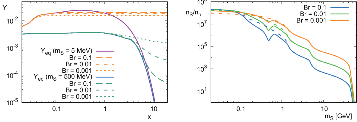
Figure 52. Left: Temperature evolution ( x = m/T ) of the Y_S intermediate abundance for m_S = 5\text{MeV} and 500\text{MeV} for the three benchmark higgs branching ratios. Right: Metastable abundance of S prior to its decay normalized over the baryon density. Values shown for Br(h \rightarrow SS) = 10^{-1}, 10^{-2} and 10^{-3} . The dashed lines correspond to the perturbative spectator model.
