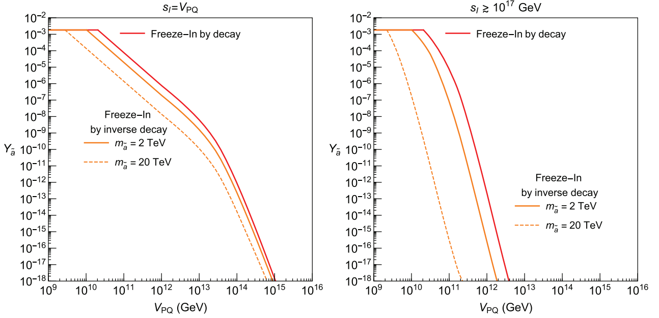
Figure 30. The axino yield from neutralino decays to SM and \tilde{a} (red) for m_{\tilde{a}} \ll 1 TeV, and neutralino inverse decays ( \tilde{\chi}^0 + \text{SM} \rightarrow \tilde{a} , orange) for m_{\tilde{a}} = 2 and 20 TeV. In both panels, 2M_1 = M_2 = \mu = 1 TeV, m_s = 500 GeV, \tan \beta = 2 , q_\mu = 2 , and \mathcal{D} = 4 ; while s_I = V_{\text{PQ}} ( M_* \gtrsim 10^{17} GeV) for the left (right) panel. Figure taken from [15].
