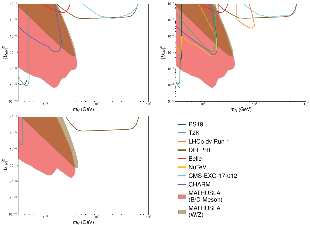
Figure 37. Projected MATHUSLA sensitivity (assuming the 200\text{ m} \times 200\text{ m} \times 20\text{ m} benchmark geometry of figure 1) in the (m_N, |U_{\alpha N}|^2) plane to sterile neutrinos, N , produced in W/Z decays (brown regions) and in B/D -meson decays (light red region) for \alpha = e (top-left), \alpha = \mu (top-right) and \alpha = \tau (bottom-left). See [487] for the assumed sterile neutrino lifetime and production rate in meson decays. Also shown are the present exclusion limits (solid lines) at 90% C.L. from Belle (as given in the Erratum) [488] (red), PS191 [489] (using the reinterpretation from [469]) (dark-green), T2K [490] (gray-blue), CHARM [491] (blue), NuTeV [492, 493] (yellow; the dashed line shows the decrease in sensitivity due to the short-lived nature of N , as taken from [488]), NA3 [494] (purple), BEBC [495] (light green), and at 95% C.L. from DELPHI [496] (brown), LHCb (using the reinterpretation from [452] of the displaced vertex search in [497]) (orange) and \sqrt{s} = 13\text{ TeV} CMS [415] (cyan).
