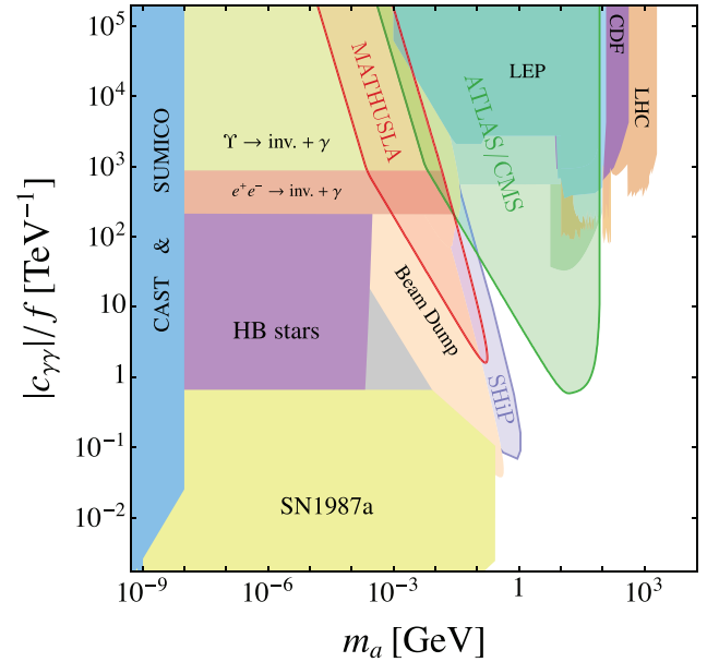
Figure 71. Projected reach in searches for Z \rightarrow a\gamma \rightarrow 3\gamma decays with ATLAS/CMS (green) and MATHUSLA (red, assuming the 200 \text{ m} \times 200 \text{ m} \times 20 \text{ m} benchmark geometry of figure 1) with \sqrt{s} = 14 \text{ TeV} center-of-mass energy and 3000 \text{ fb}^{-1} integrated luminosity.
