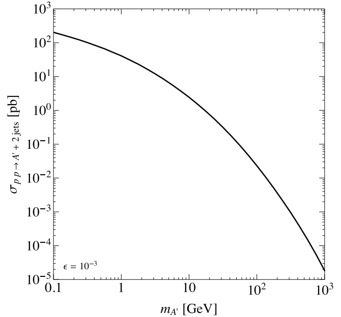
Figure 61. Cross-sections for the bremsstrahlung of dark photon at LHC in terms of dark photon mass. Here, \epsilon = 10^{-3} is chosen, and the cross-section is proportional to \epsilon^2 .
