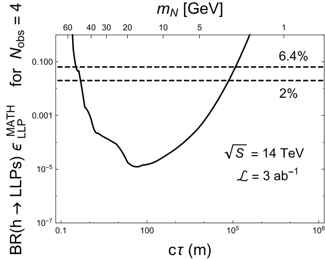
Figure 44. Sensitivity estimate for the MATHUSLA detector at the HL-LHC (assuming the 200 \text{ m} \times 200 \text{ m} \times 20 \text{ m} benchmark geometry of figure 1) for the process pp \rightarrow h \rightarrow \sum NN . We have assumed a diagonal Dirac neutrino mass matrix and m_{\nu_i} = 0.1 \text{ eV} to fix the RH neutrino lifetime. The cross-section required to see four events has been normalised to the detection efficiency \epsilon_{\text{LLP}}^{\text{MATH}} for a displaced vertex. The 2% and 6.4% lines are representative of possible \text{Br}(h \rightarrow \text{invis}) exclusions achievable by the HL-LHC, see sections 3.2.1 and 8.2.
