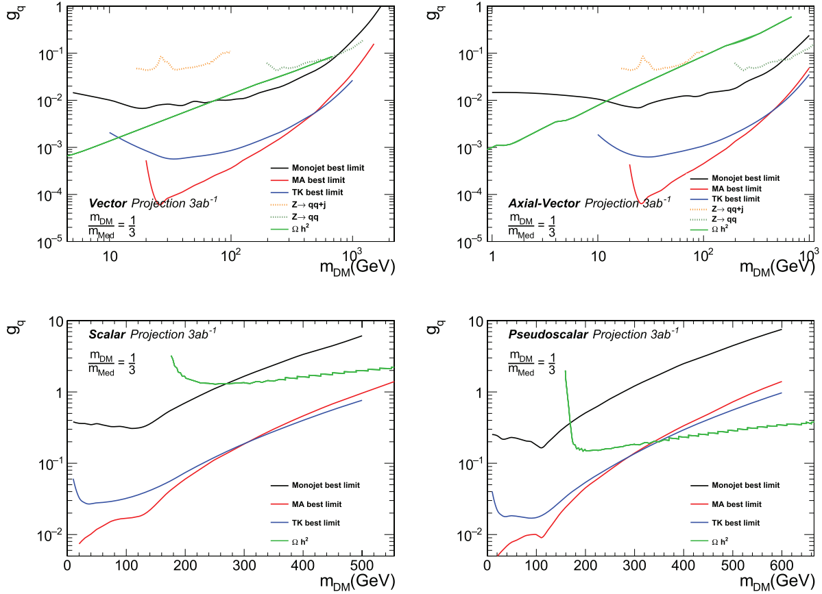
Figure 13. Expected minimum coupling g_q probed with 3000 \text{ fb}^{-1} of data for the optimal lifetime value (scanning all lifetimes) for spin-1 vector (top left) and axial vector (top right) mediators, and spin-0 scalar (bottom left) and pseudoscalar (bottom right) mediators, as a function of dark matter mass m_{\text{DM}} . In this plot g_{\text{DM}} = 1 , and the mediator mass m_{\text{med}} is fixed to be exactly three times the mass of the dark matter. The black line corresponds to the minimum coupling probed in a MET only search, the blue line corresponds to the case where a secondary vertex is identified in the missing energy search, and the red line corresponds to the minimum coupling with the MATHUSLA detector. The dashed lines correspond to visible search in either a boosted jet (dashed-orange) or a di-jet resonance (dashed-green), for both searches the dark matter branching ratio is accounted for. Lastly the solid green line \Omega h^2 corresponds to the minimum allowed coupling that will not overproduce dark matter (assuming a single dark matter candidate) for the shown spin-1 models where no lepton couplings are added, and the shown spin-0 models with a Yukawa coupling. While this coupling has no physical significance if the invisible particle is an LLP, it allows the shown coupling reaches to be compared to the sensitivity goal of the monojet searches.
