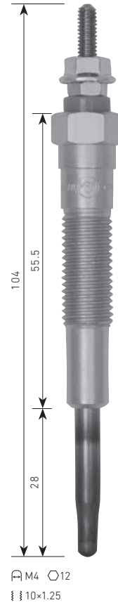
CP-20 TOYOTA 2L-TE ⚡11V
