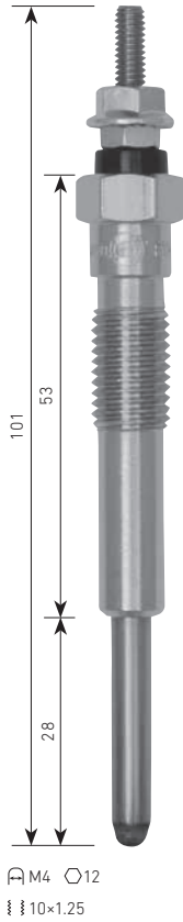
PT-109 TOYOTA 2B, 3B, 2J, B 420.5V
