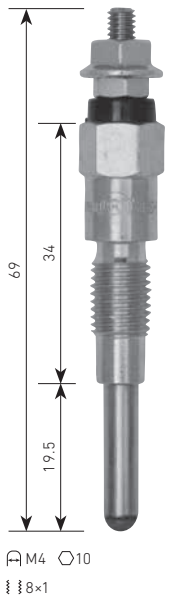
PS-206 KUBOTA D662, etc. ⚡11V
