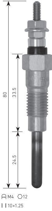
PS-207 KUBOTA D905, etc. ⚡11V
