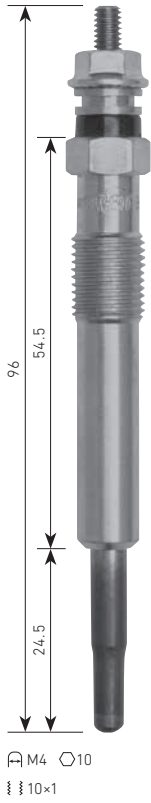
B-105 FORD BHDA, etc. 10V
