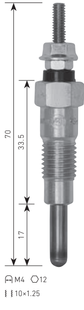
PS-201 KUBOTA D600-C, etc. ⚡10.5V
