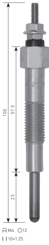
PM-66 mitsubishi 6D10, 6D11 ⚡21V
