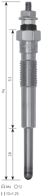
PT-146 TOYOTA 2J 46V
