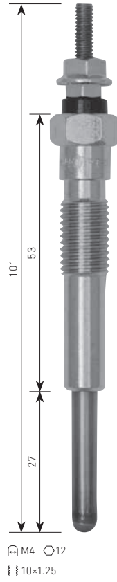
PT-93 TOYOTA B, 2J ⚡8V
