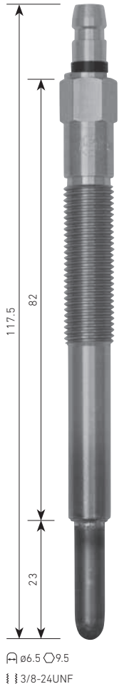
PK-98 KOMATSU 3300, 3304, 340 ↖24V
