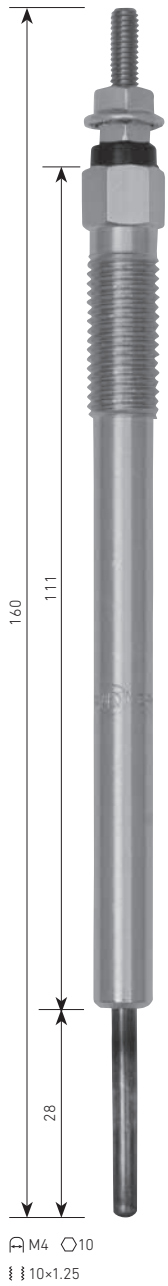
CP-23 TOYOTA 1VD-FTV, etc. ⚡11V
