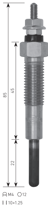
PS-203 ISHIKAWAJIMA ⚡10.5V
