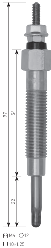
PM-166 HYUNDAI D4BA ↖11V
