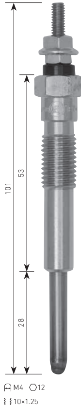
PT-141 TOYOTA 2B, 2H, 3B, H2H 414V
