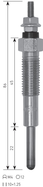
PZ-33 MAZDA R2, RF, XA ⚡10.5V
