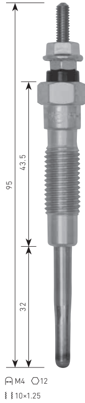
PT-142 TOYOTA 2J, 2L, L 416V
