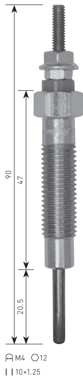
CP-05 MITSUBISHI 4M40 ⚡11V
