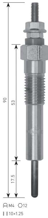
CP-50 MAZDA 4EE1 ⚡11V
