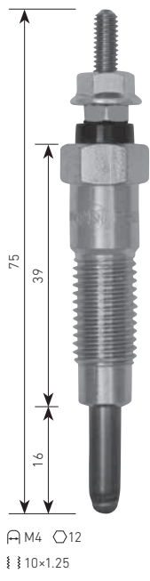
PS-202 KUBOTA D1102, etc. ⚡10.5V
