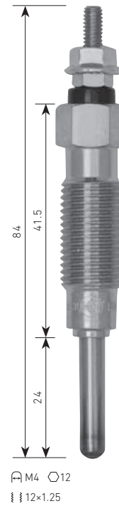
PM-77 MITSUBISHI 4DR5 ⚡11V
