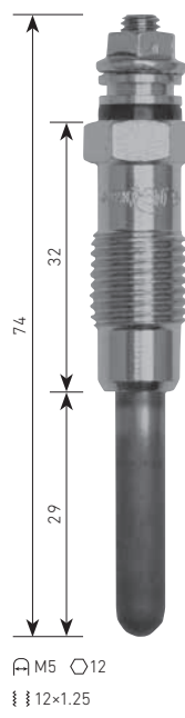
B-049 ALFA ROMEO VM80A, VM81A ⚡11V
