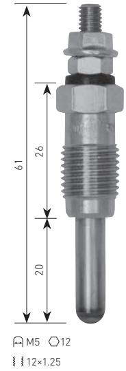
PN-121 NISSAN LD20, LD28 ⚡6.5V
