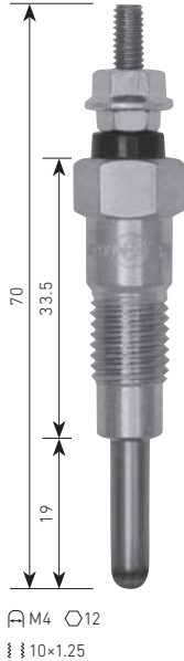
PN-123 NISSAN SD23, etc. ⚡8.5V
