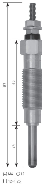
PM-162 MITSUBISHI 4DR7 ↖11V
