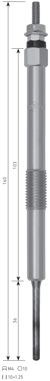
PT-159 TOYOTA 1ND-TV ⚡11V
