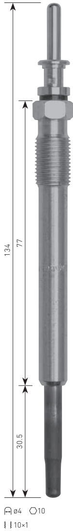
B-107 OPEL, VAUXHALL Y20 DTH, etc. 11V
