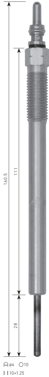
CP-08 MITSUBISHI 4N13, 4N14, 4N15 ⚡11V
