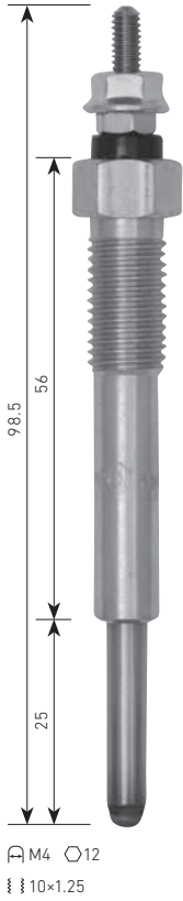
PK-96 KOMATSU 4D120, 4D130 ↖22.5V
