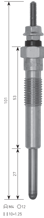
PT-94 TOYOTA B, 2J ⚡19V
