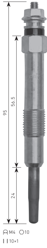
B-108 ALFA ROMEO AR 32302, etc. 11V
