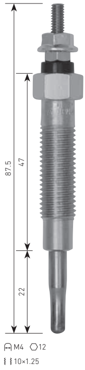
PM-400 MITSUBISHI 2.5L SOHC ⚡11V
