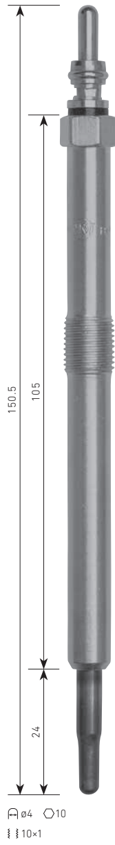
B-116 NISSAN, RENAULT G9T, G9U ⚡11V
