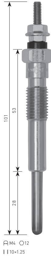
PT-145 TOYOTA 2B, 3B, 2J, B 410.5V
