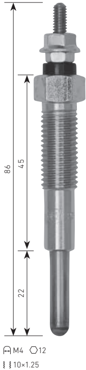
PZ-31 MAZDA HA, XA, ZB ⚡23V
