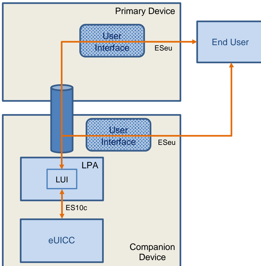
Figure 4: End User Interaction and Interfaces between a Primary and Companion Device, where the Companion Device MAY have a UI
