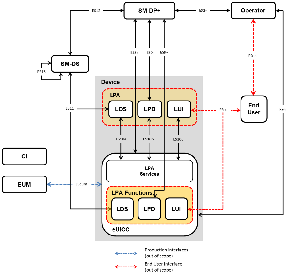
Figure 15: Interfaces on the eUICC Architecture with the LPA in the Device Configuration
