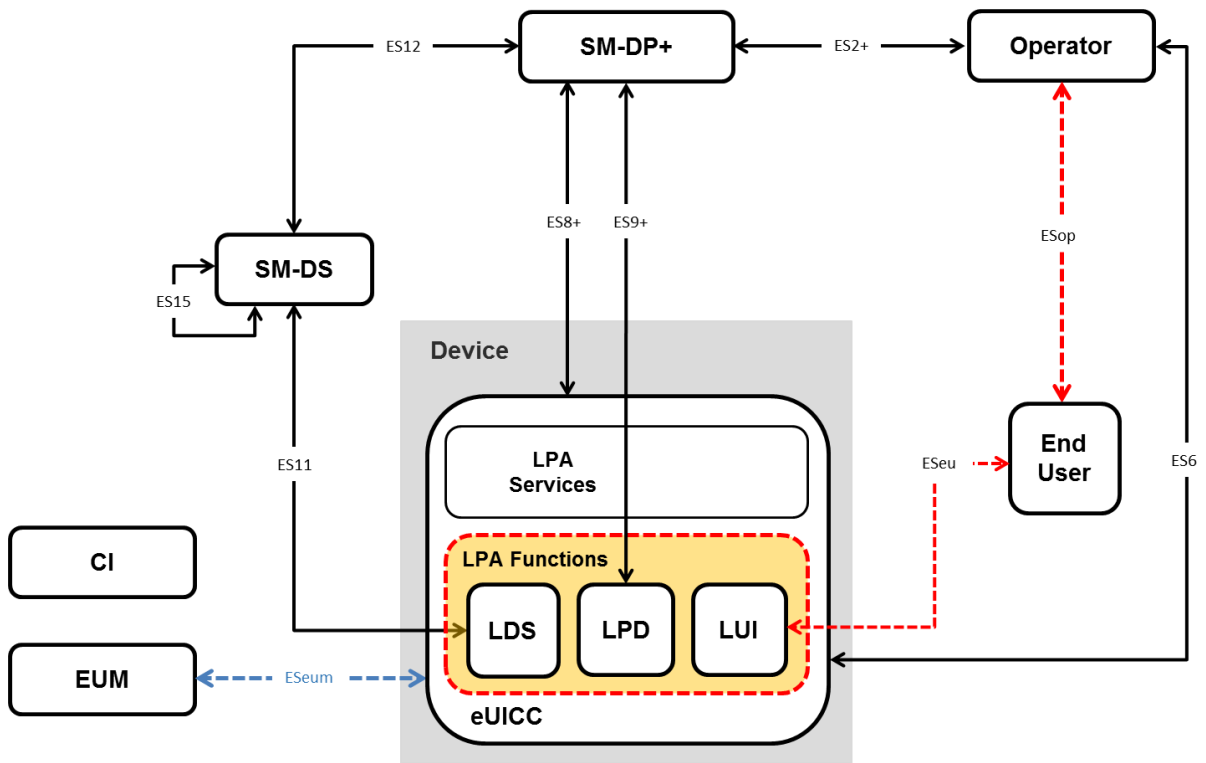
Figure 6: LPA in the eUICC
