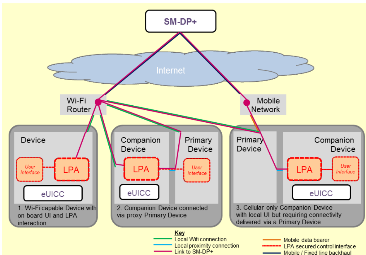
Figure 16: Example Connection Methods for Companion Devices to reach out to the SM-DP+
