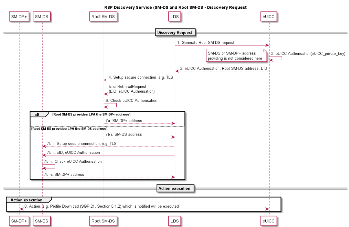
Figure 14: Discovery Request Procedure
