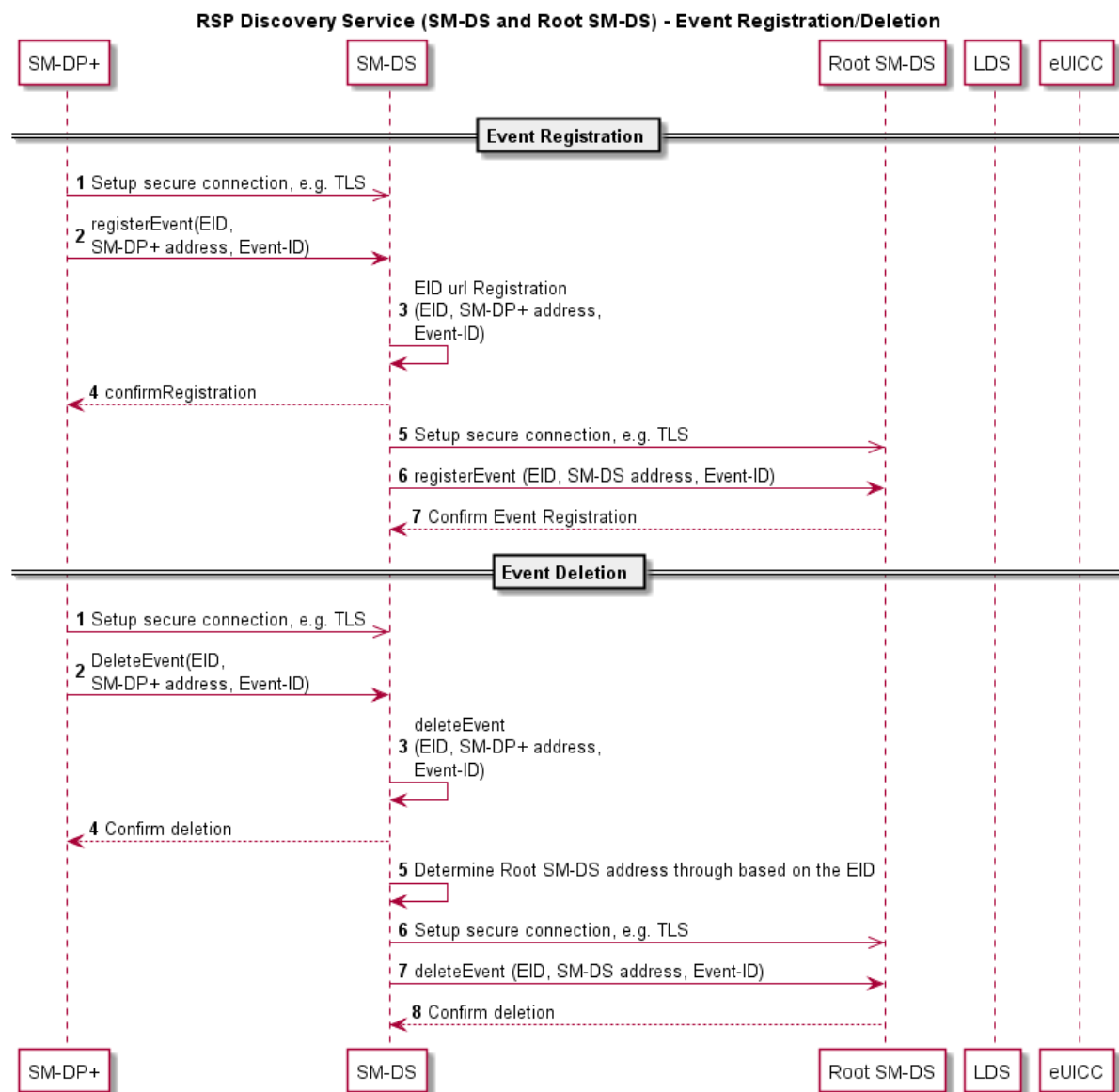
Figure 13: Event Registration/Deletion Procedure
