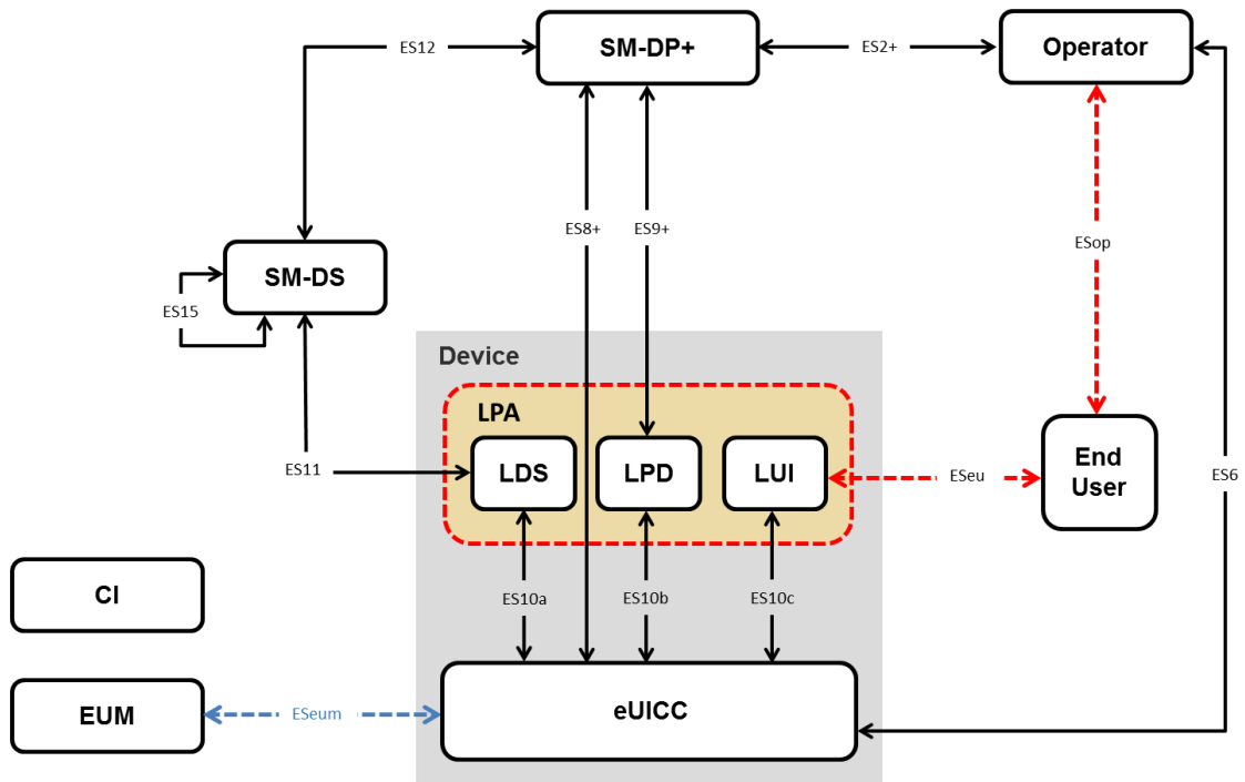
Figure 7: LPA in the Device
