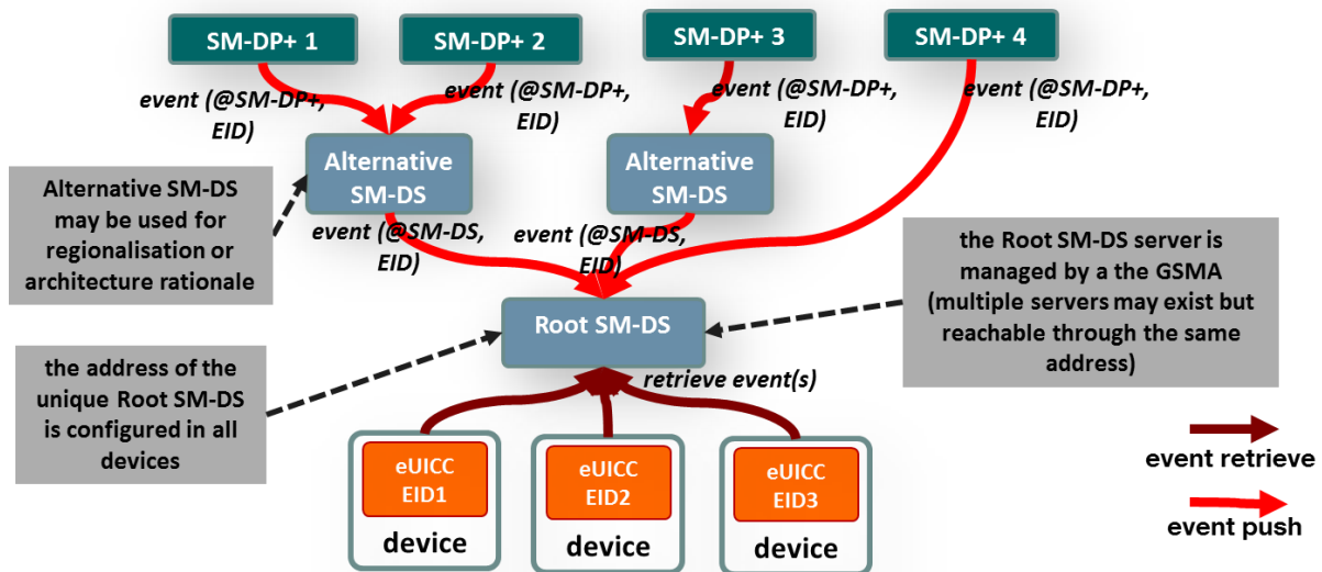
Figure 11: SM-DS Implementation
