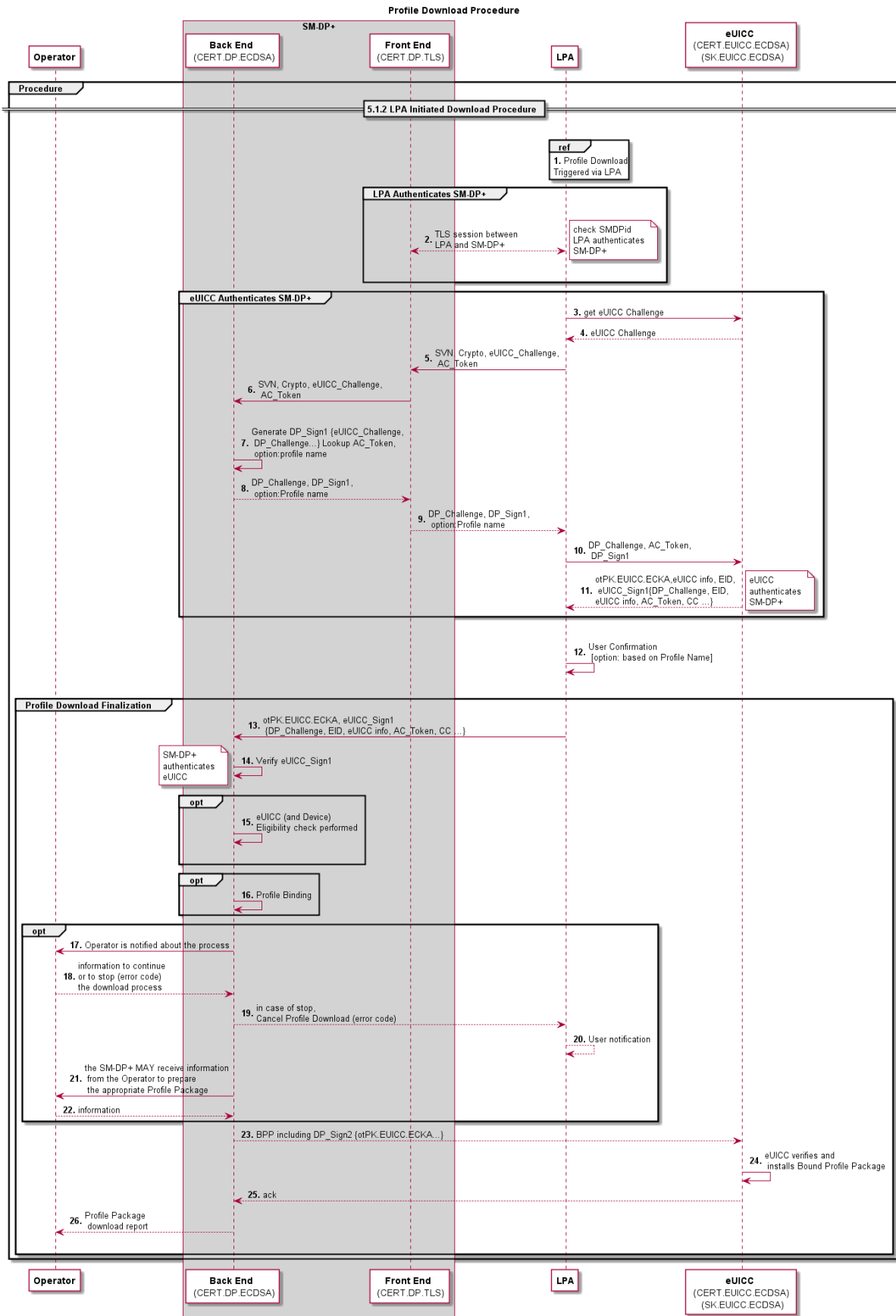
Figure 17: Profile Download Procedure
