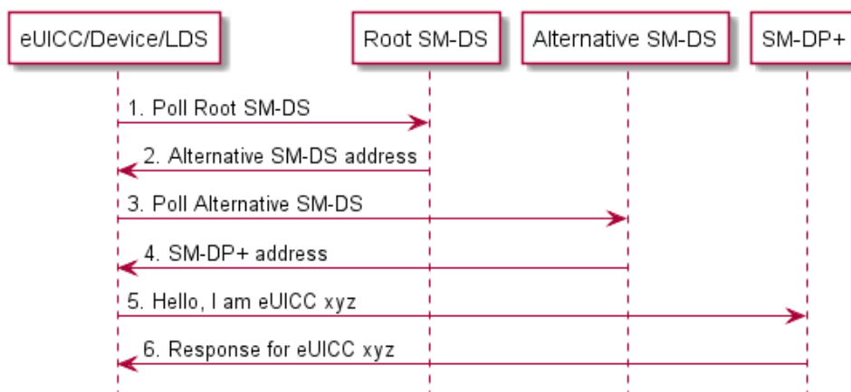
Figure 10: Alternative SM-DS Discovery
