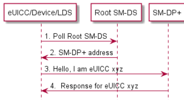
Figure 9: Root SM-DS Event Registration
