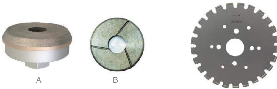
GENERATING WHEELS
