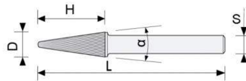
Conical With Radius End Shape
