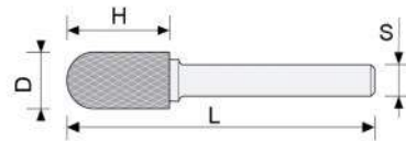
Cilindrica With Radius End Shape
