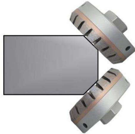
PRECUTTING WHEELS
