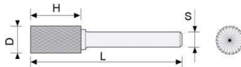
Cilindrical Shape with End Cut
