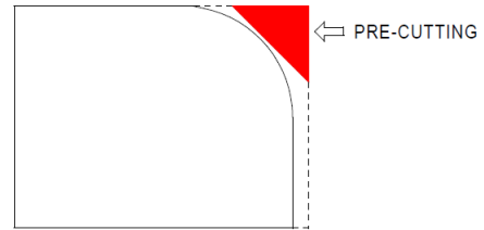
Pre Cutting Wheel Shape “Y” Slab Thickness 2-3-4 CM 45°
