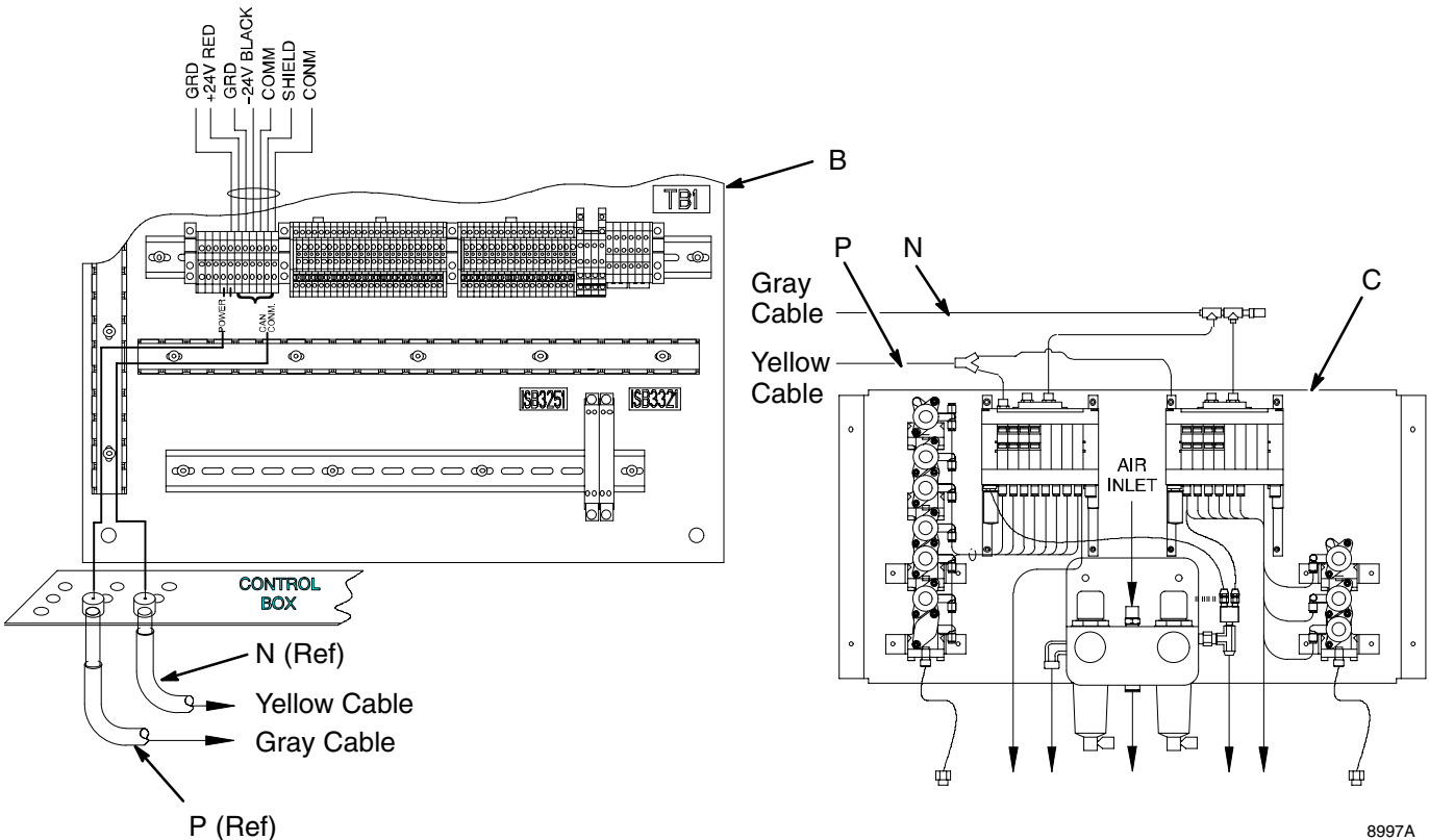
Fig. 3.13 Electrical Connections
