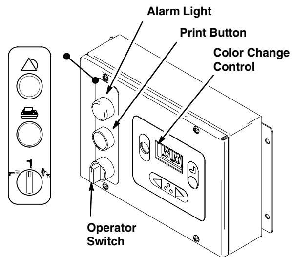
Operator Station
