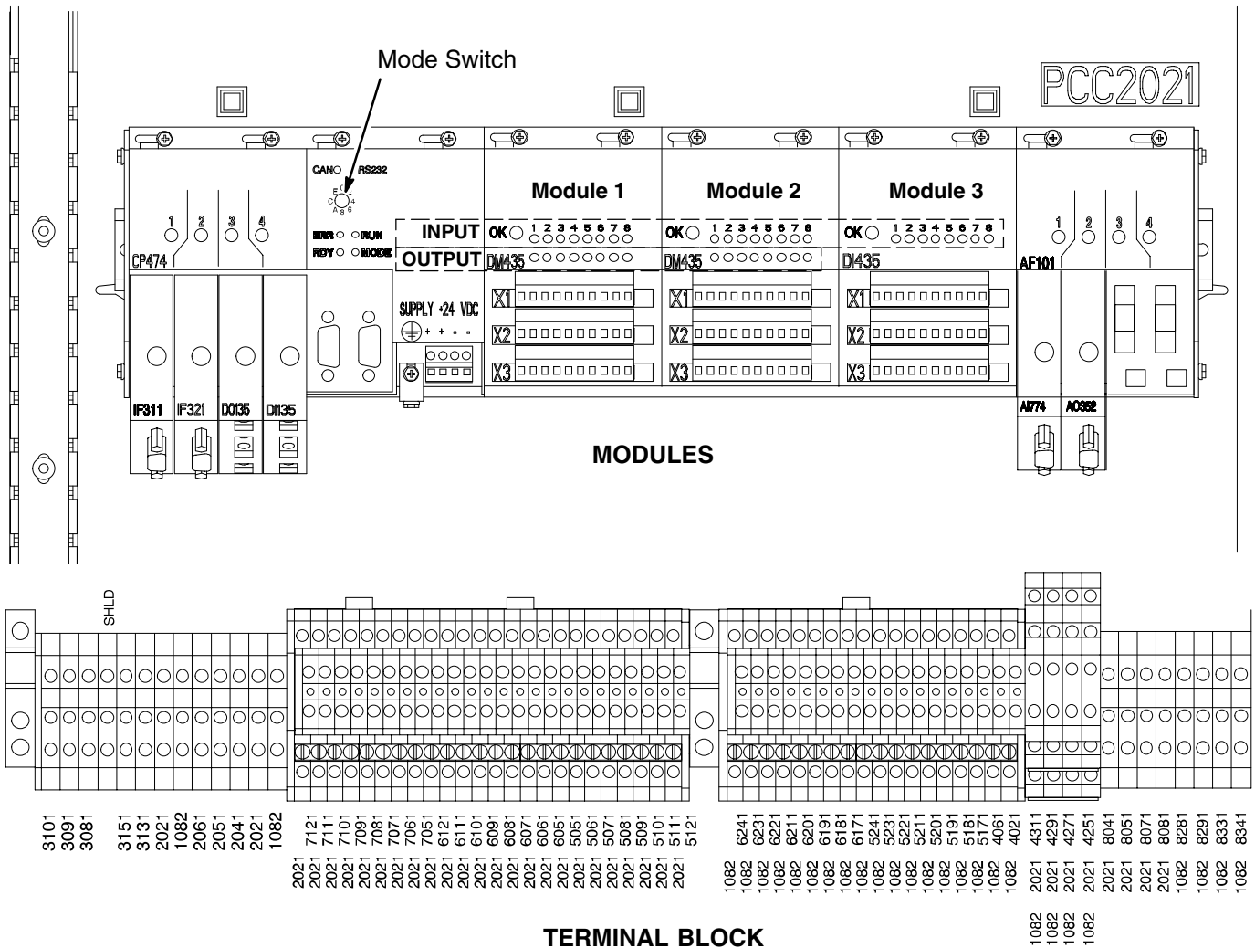
Fig. 10.2 CONTROLLER
