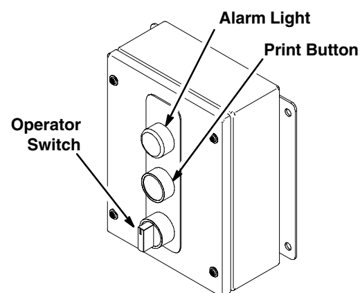
Operator Station
