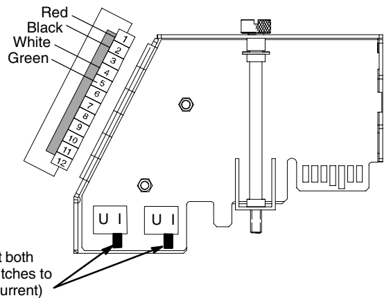
Fig. 11.13 Analog Output Submodule–AO352
