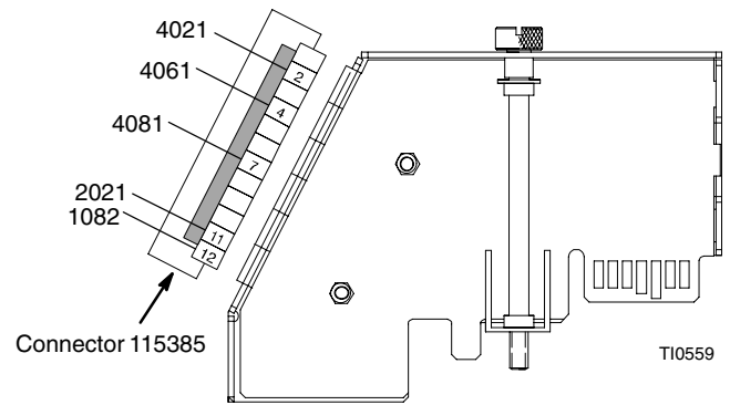
Fig. 11.11 Digital Output Submodule–114781
