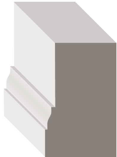
Stock Code Dimensions MFVG180 (1626279) 1 3/16" x 1 5/16" x RL
