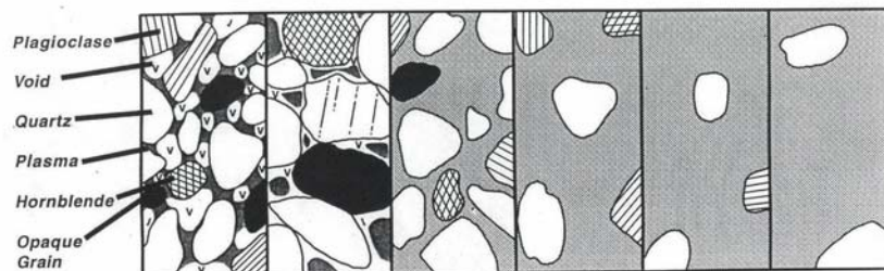
Figure 3. Calcium carbonate around skeletal (sand-sized) grains in a coarse-textured matrix. These carbonate coatings are referred to as calcitans (Brewer, 1976). Their formation illustrates attraction to and deposition of carbonates on mineral surfaces (e.g., quartz or feldspar grains) accessible to percolating water. Frame width = 0.9 mm. (Cax pedon, San Bernardino, Co., CA, Pedon 97P0420, Bkg2 horizon under crossed polarized light).
