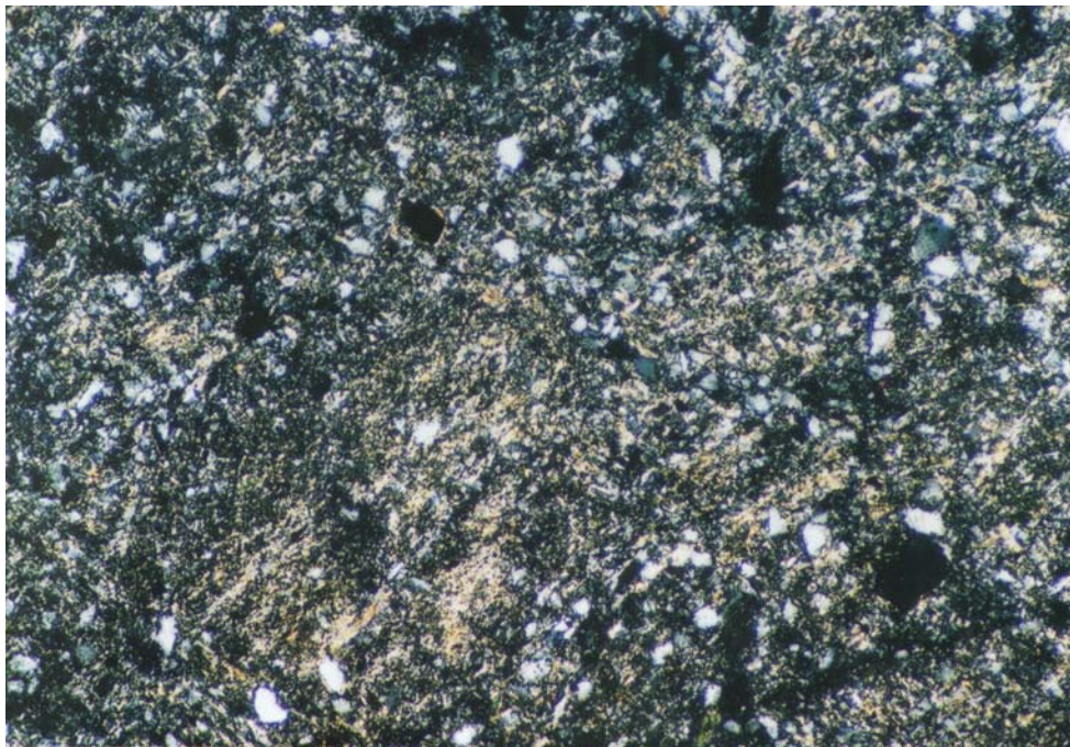
Figure 8. Mosaicic plasma fabric. Frame width = 1.3 mm. (Leonard pedon, Macon Co., MO, 87P0770, 2Btg3 horizon under crossed polarized light).
