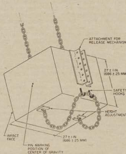
FIGURE W-21—Pendulum.
