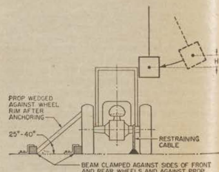
FIGURE W-23—Method of impact from side.
