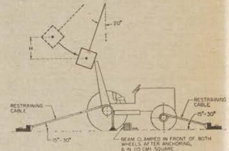
FIGURE W-22—Method of impact from rear.
