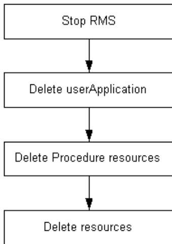
[Figure 7.5 Flow of Deleting the Cluster Environmental Configuration]
