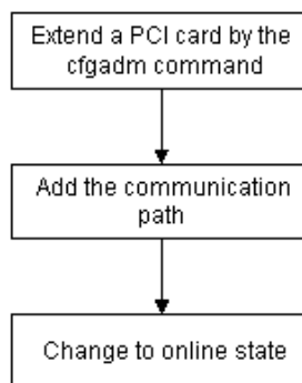
[Figure 8.4 Addition Procedure]
