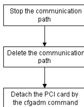
[Figure 8.5 Deletion Procedure]
