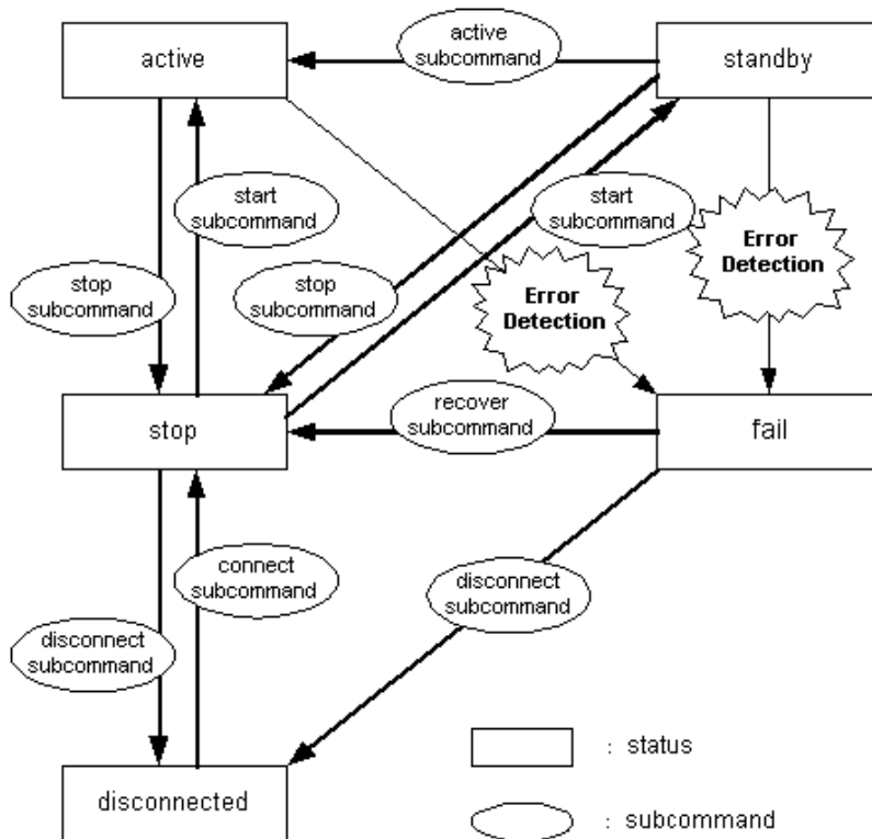
[Figure 2.5 State Transition of a Communication Path]
