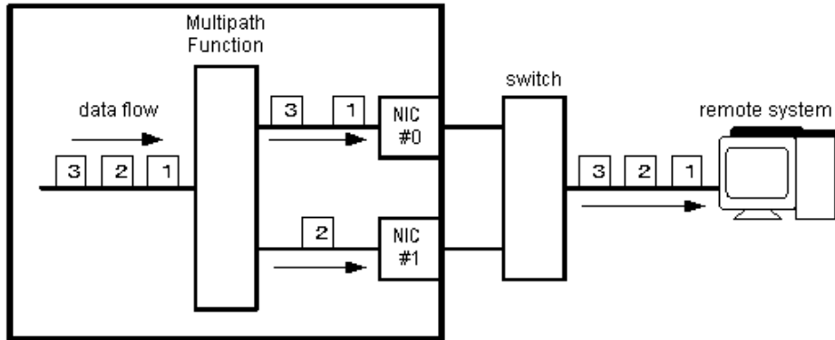
[Figure 1.6 Transmission data flow in round-robin distribution method]
