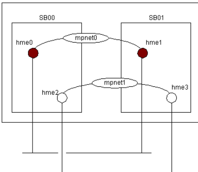
[Figure 8.1 recommendation LAN configuration]
