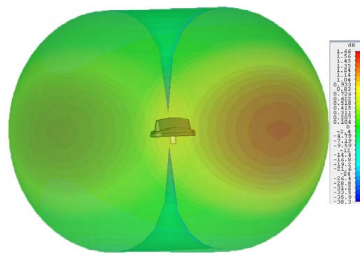
3D Gain Plot Top (1800MHz)
