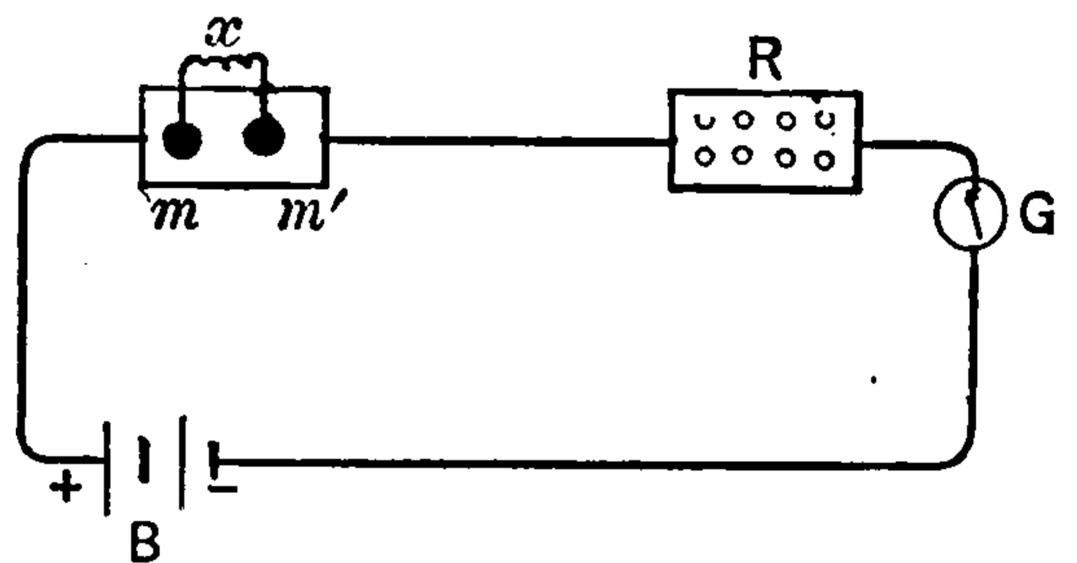
Fig. 491 Substitution Method.
