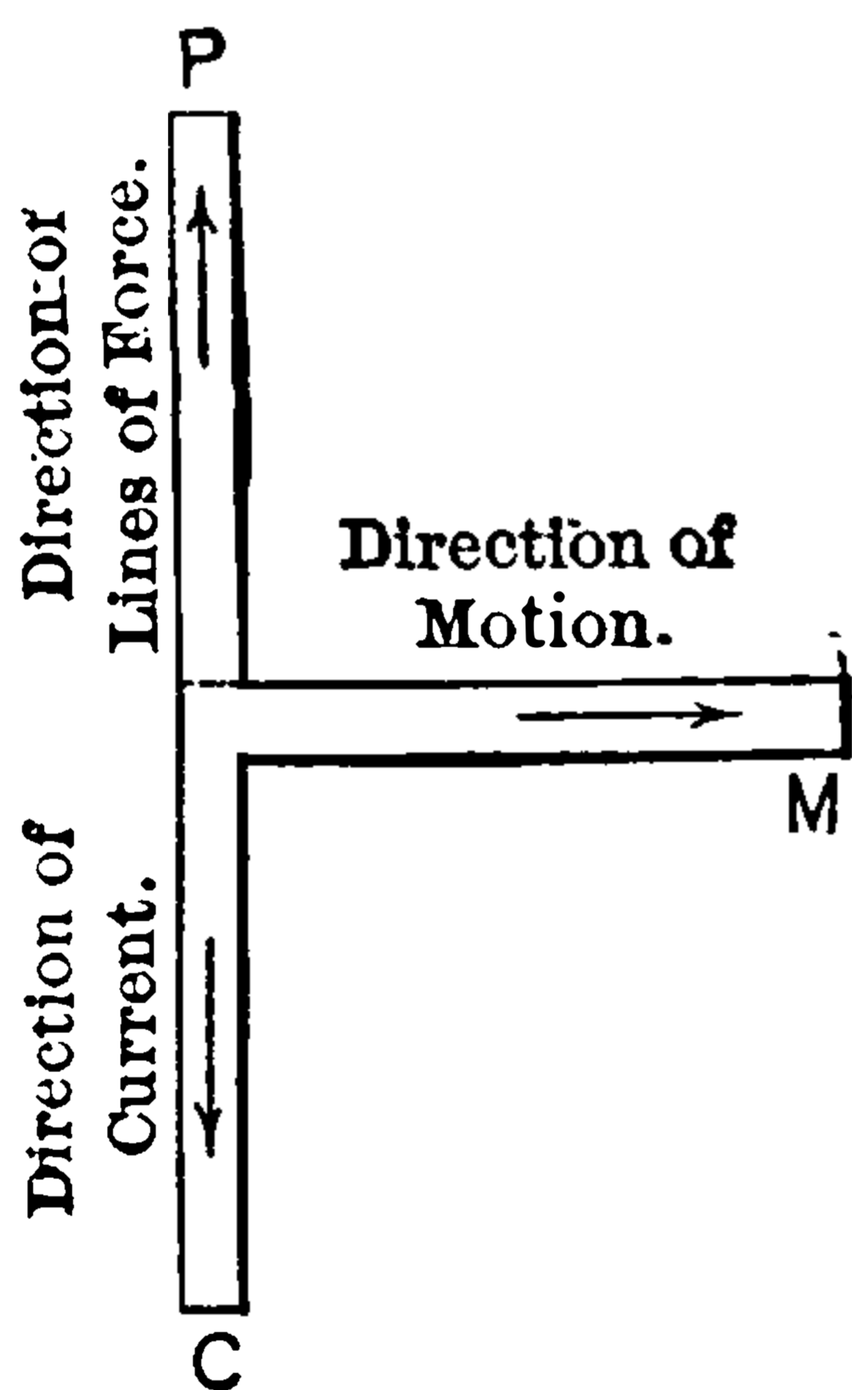
Fig. 304. Fleming's Rule.
