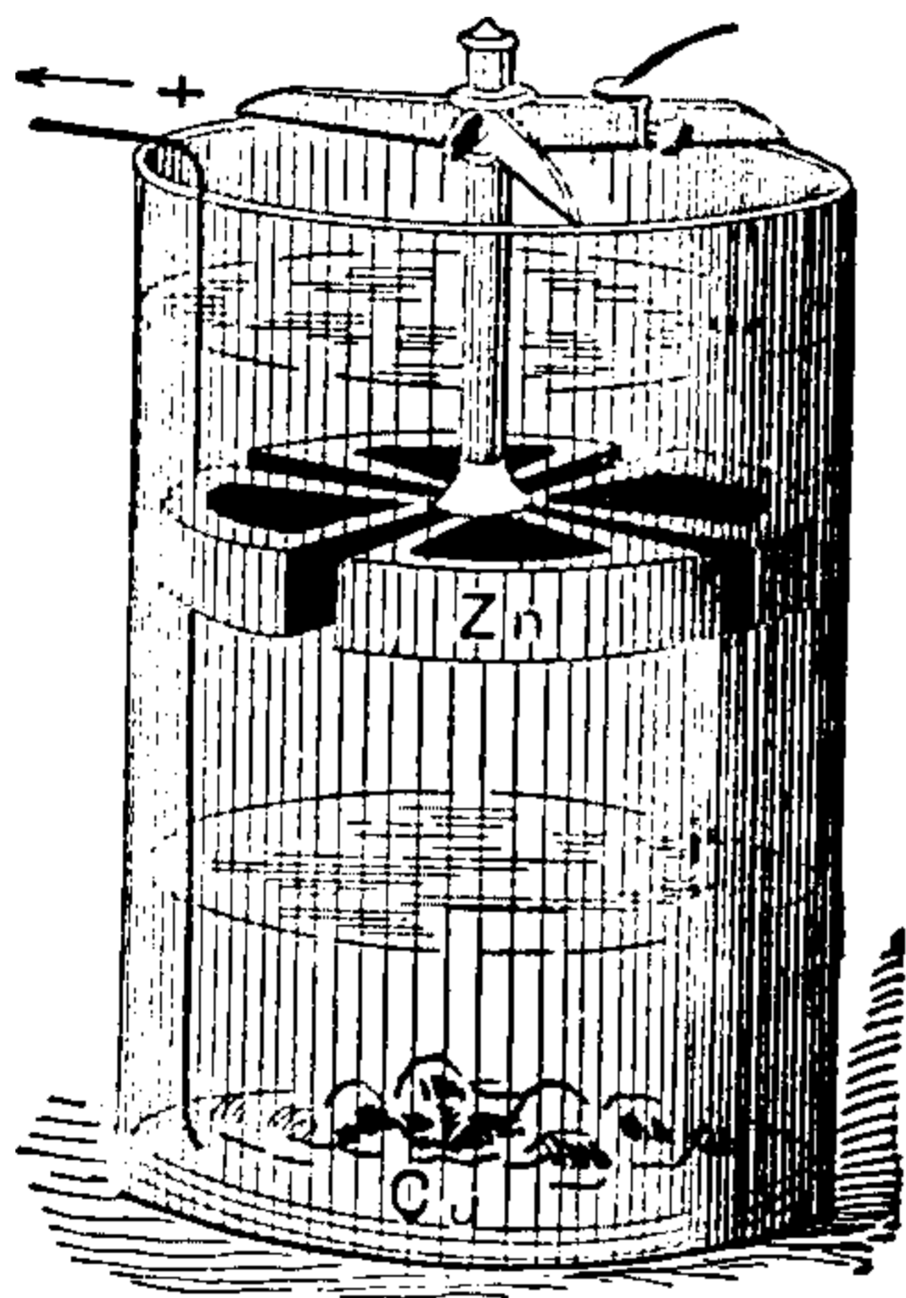
Fig. 109. The Gravity Cell.
