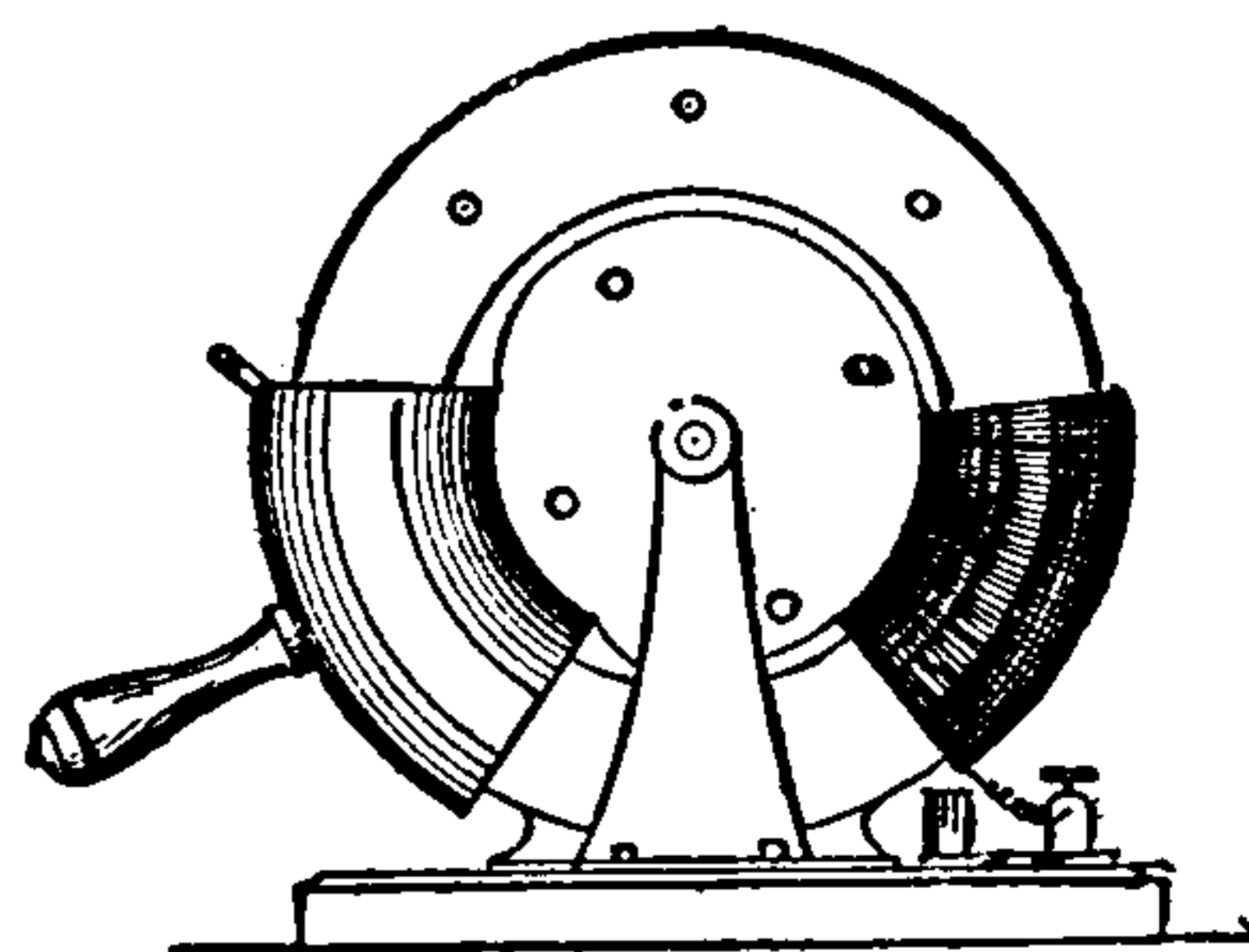
Fig. 201. Reaction Coil Dimmer.
