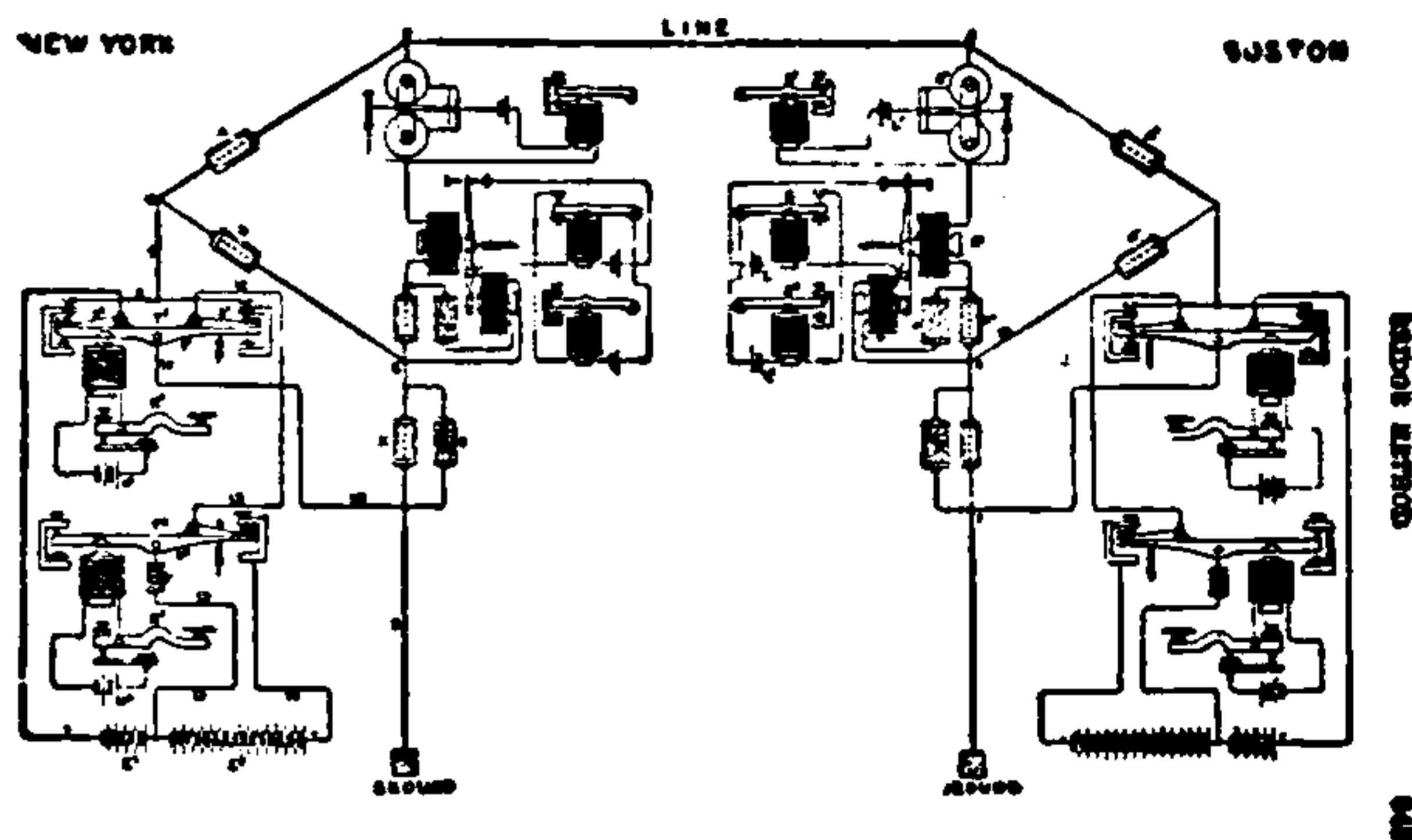
Fig. 533. Quadruplex Telegraphy, Bridge Method.
