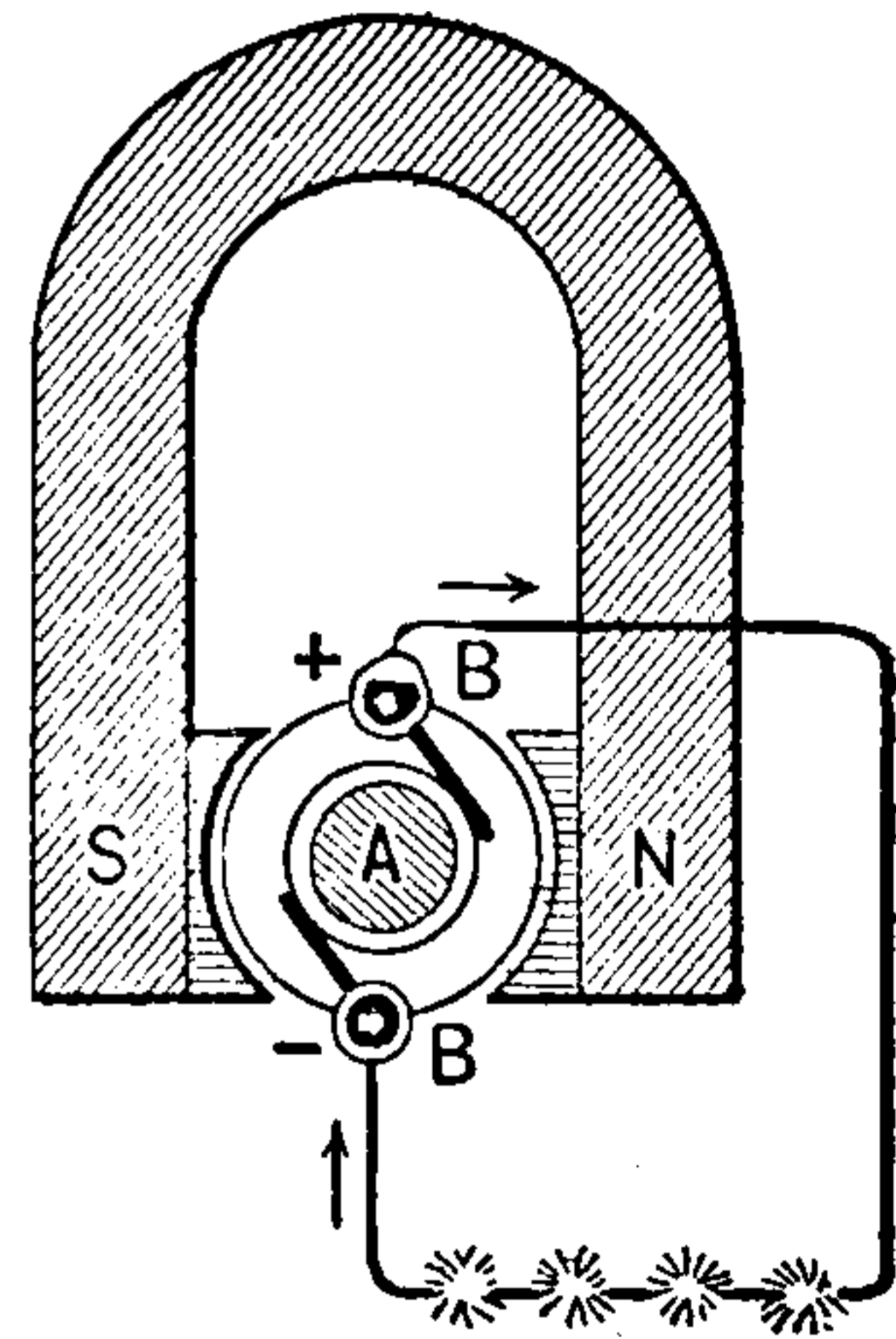
Fig. 361. Magneto-Electric Machine.
