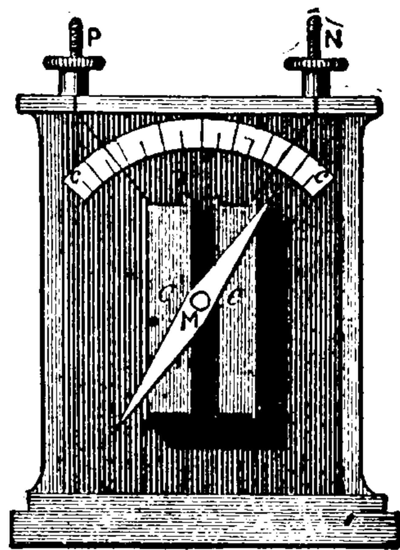
Fig. 279. Vertical Galvanometer.
