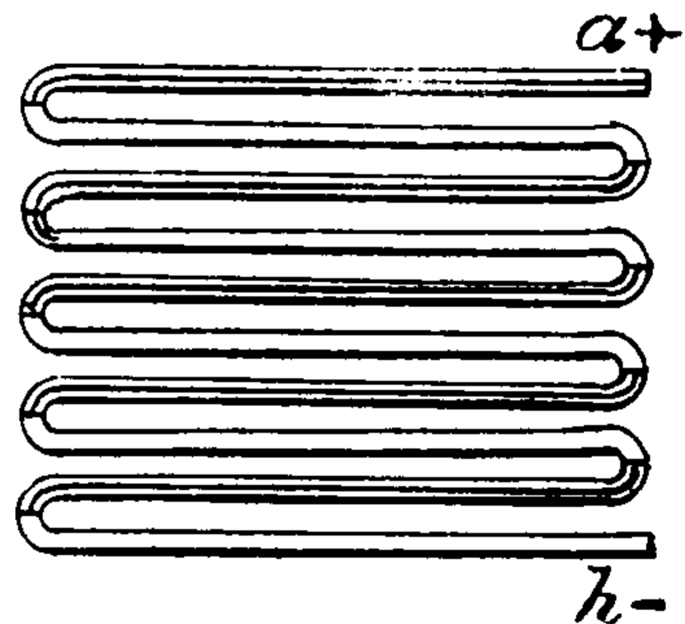
Fig. 434. Series-Connected Thermo-Electric Couples.
