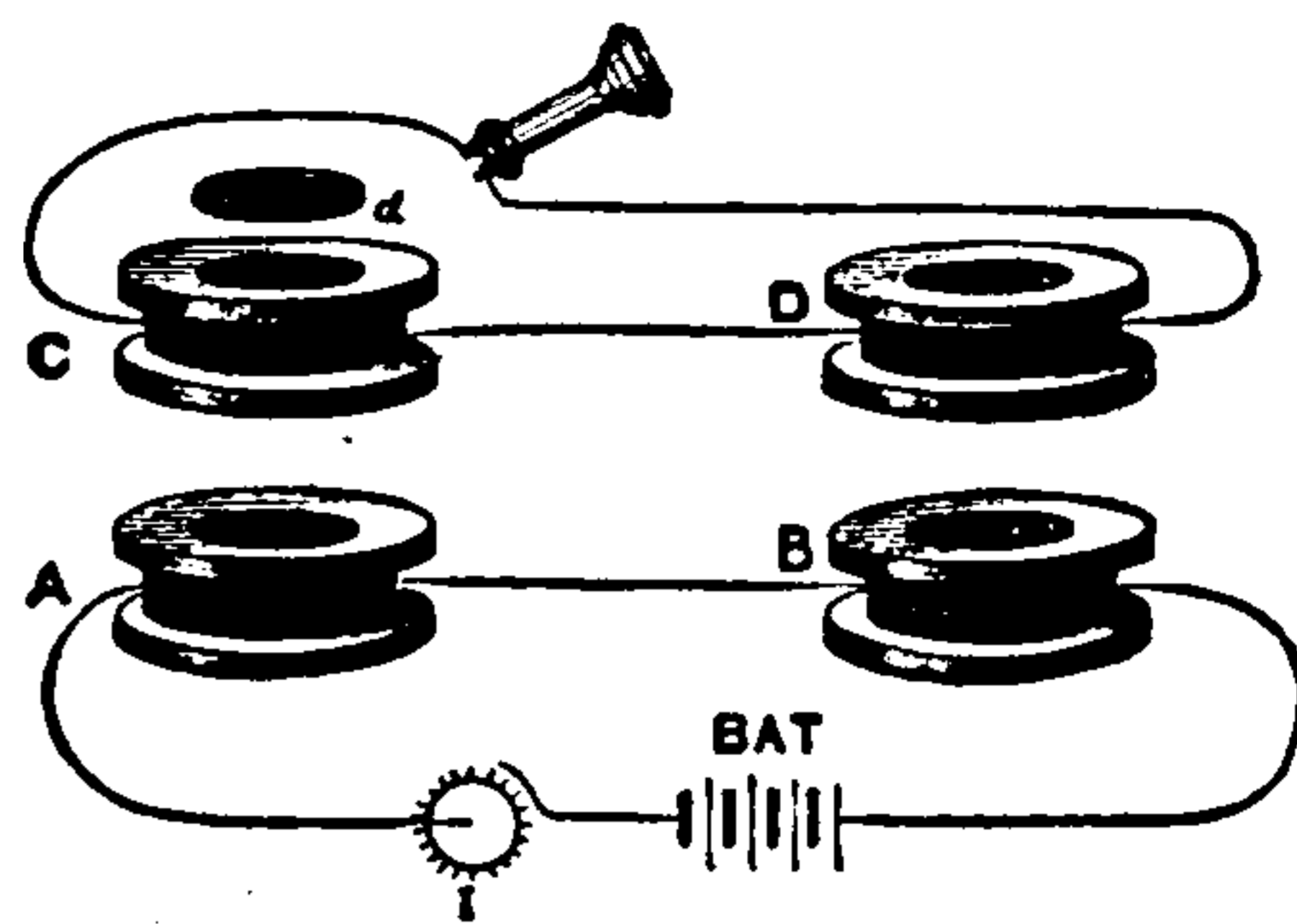
Fig. 35. Hughes' Induction Balance.
