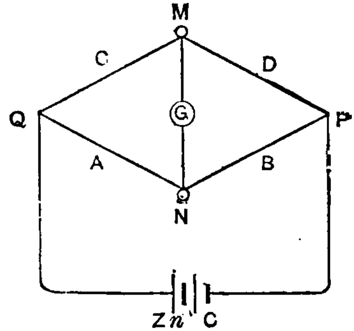
Fig. 73. Electric Balance.
