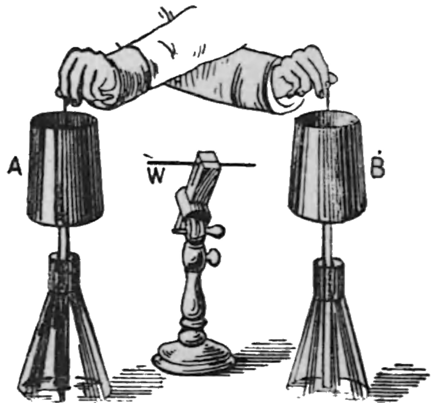
Fig. 488. Action of Replenisher.
