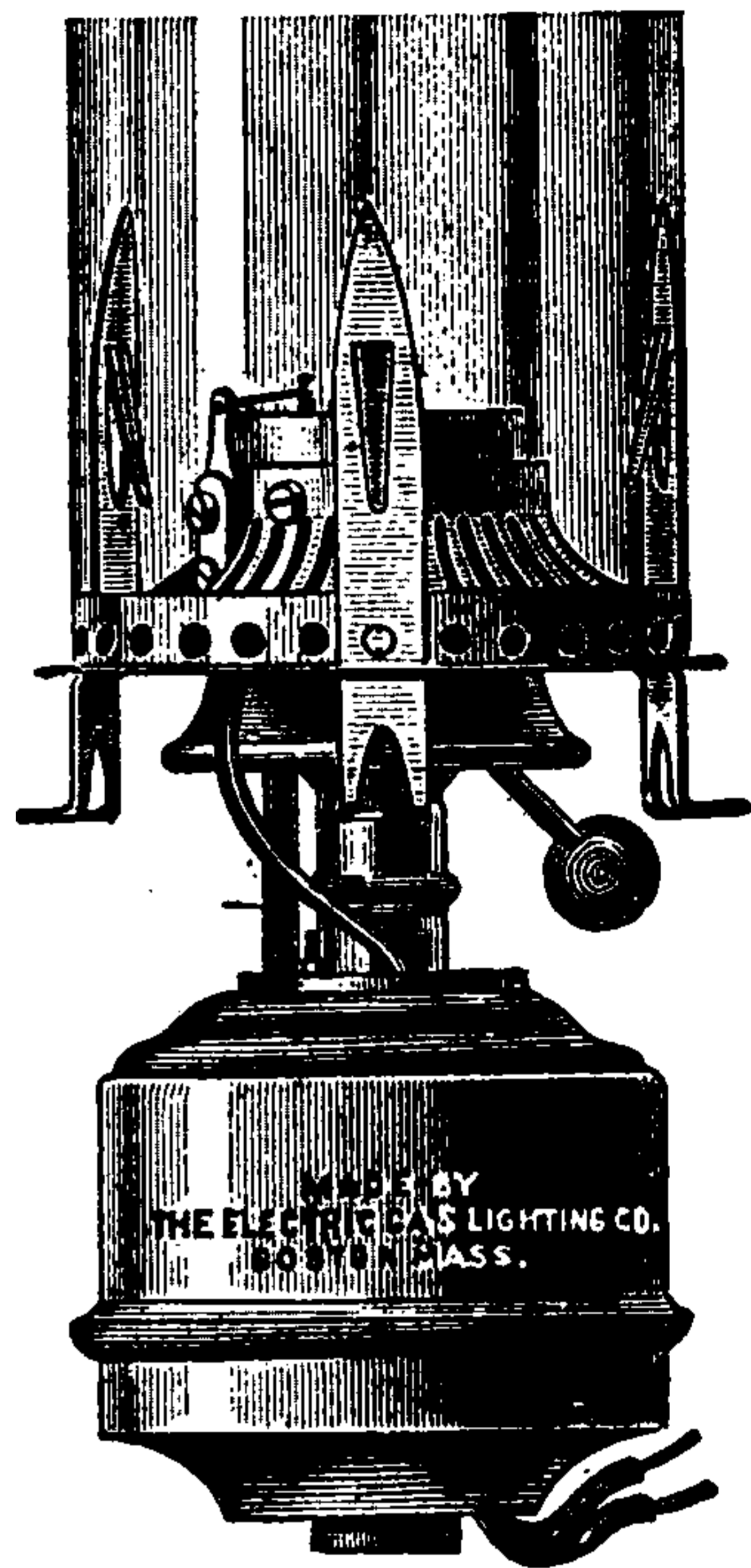
Fig. 85. Argand Electric Burner.
