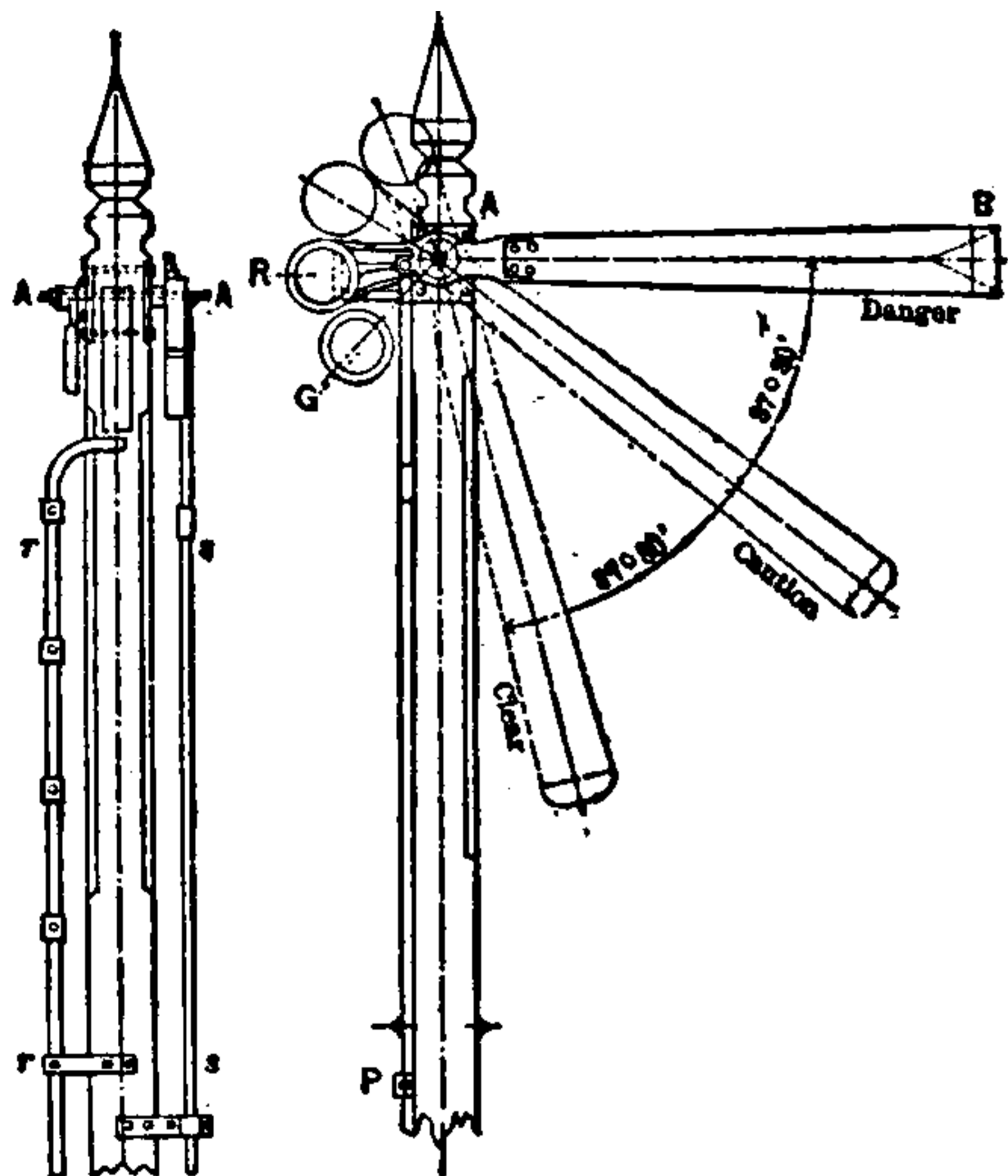
Fig. 464. Semaphore Signal—Permissive System.
