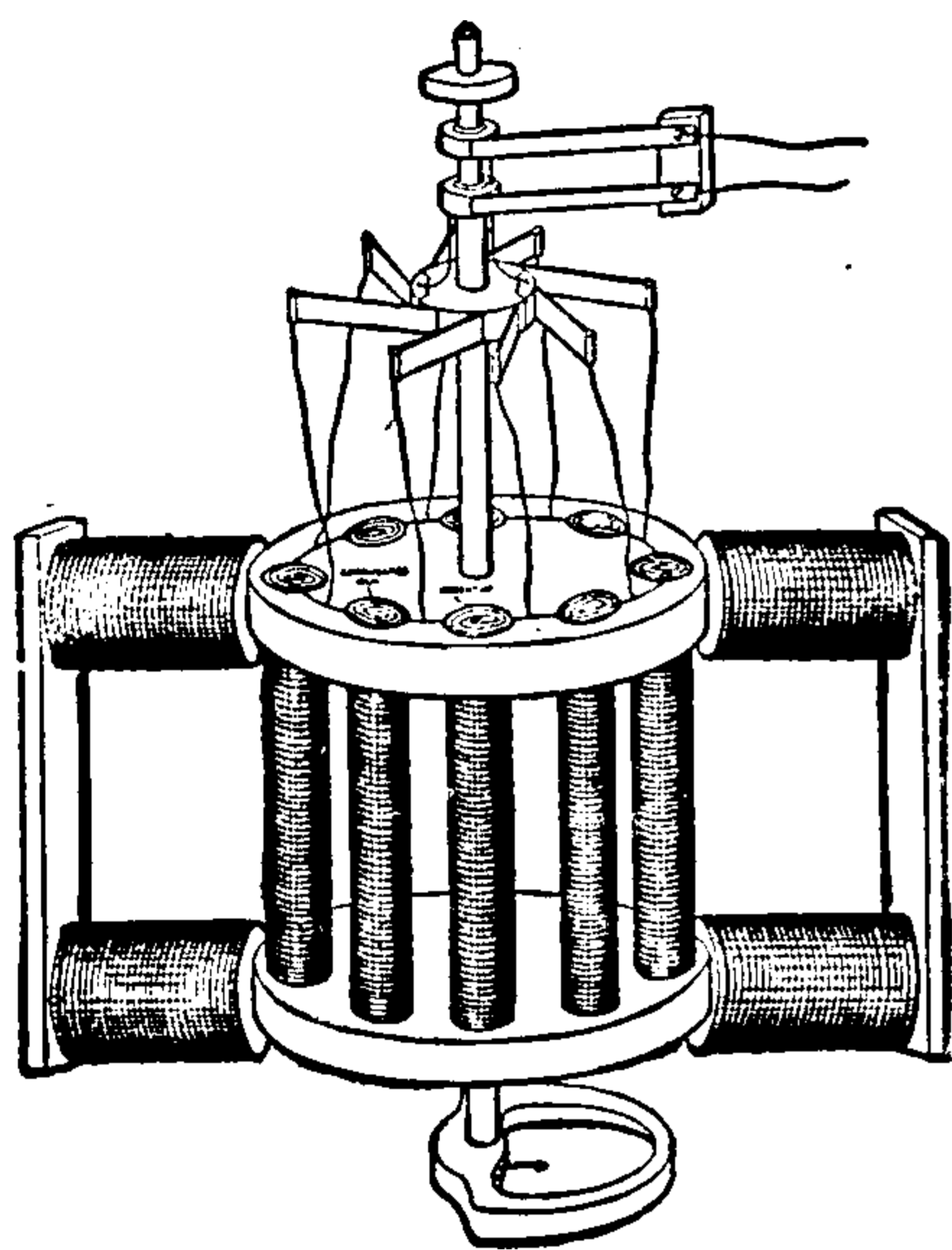
Fig 287. Edison's Pyro-Magnetic Generator.
