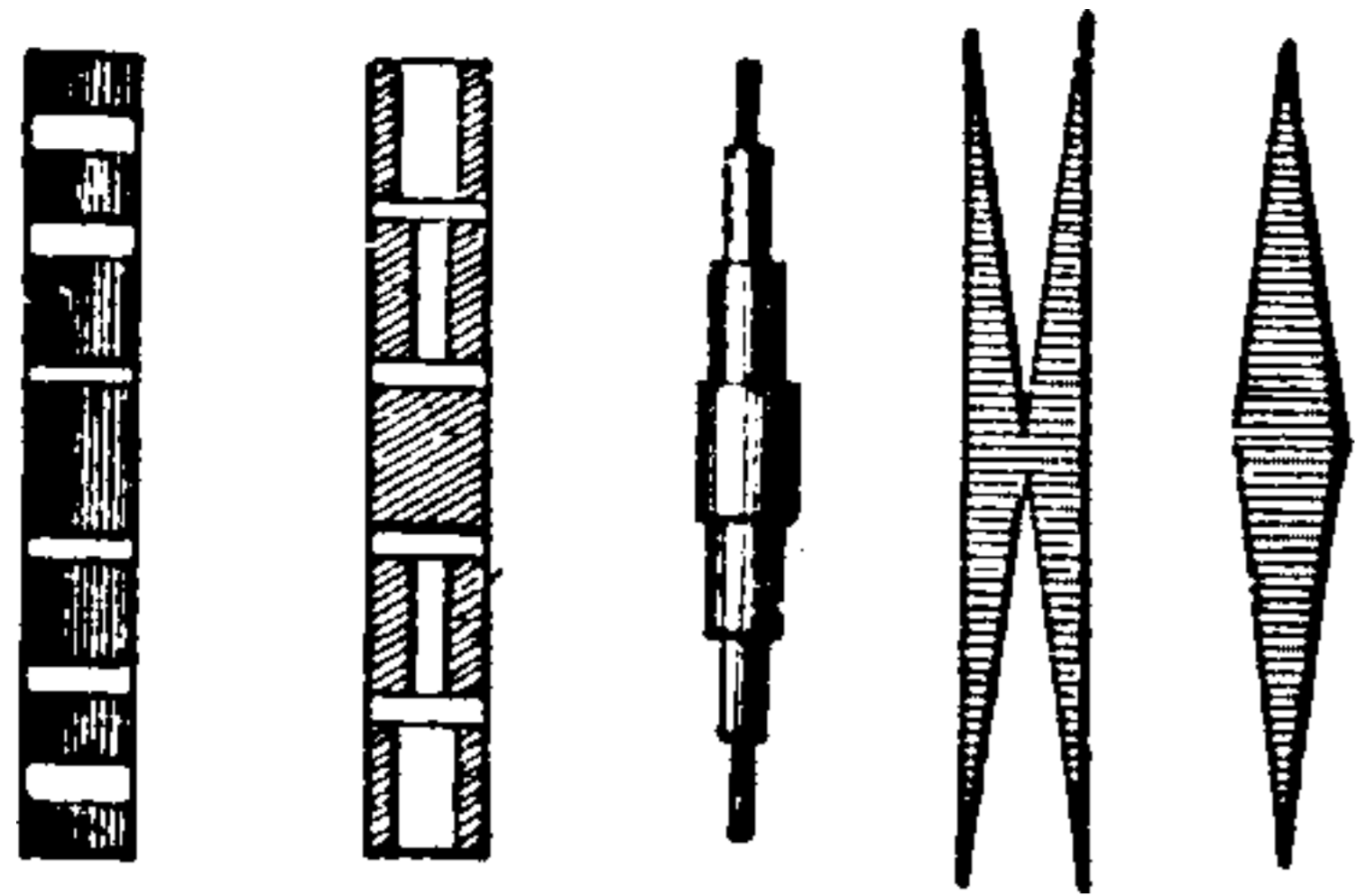
Fig. 37. Krizik's Bars.
