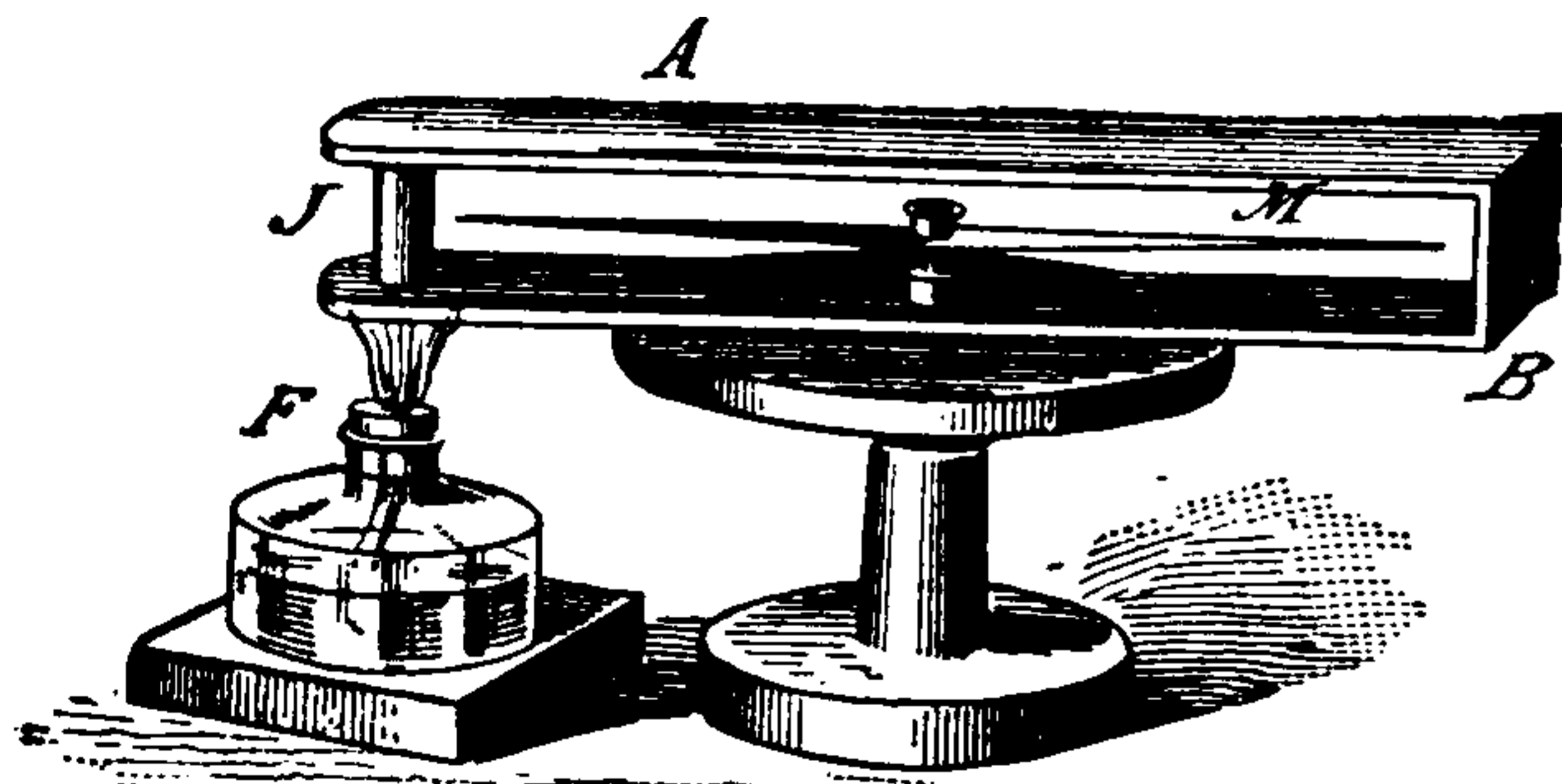
Fig. 229. Thermo-Electric Circuit.
