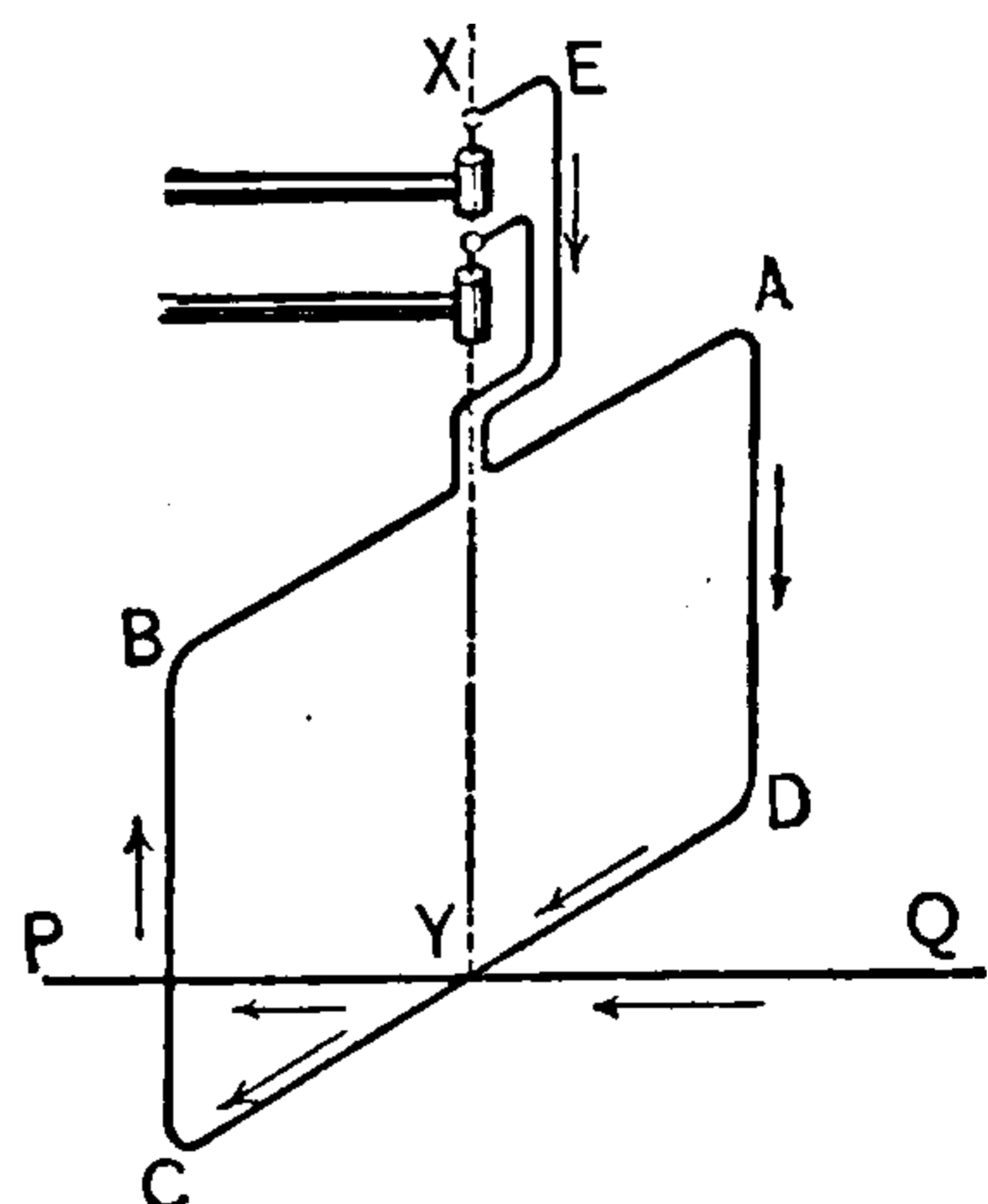
Fig. 220. Electro-Dynamic Attraction.
