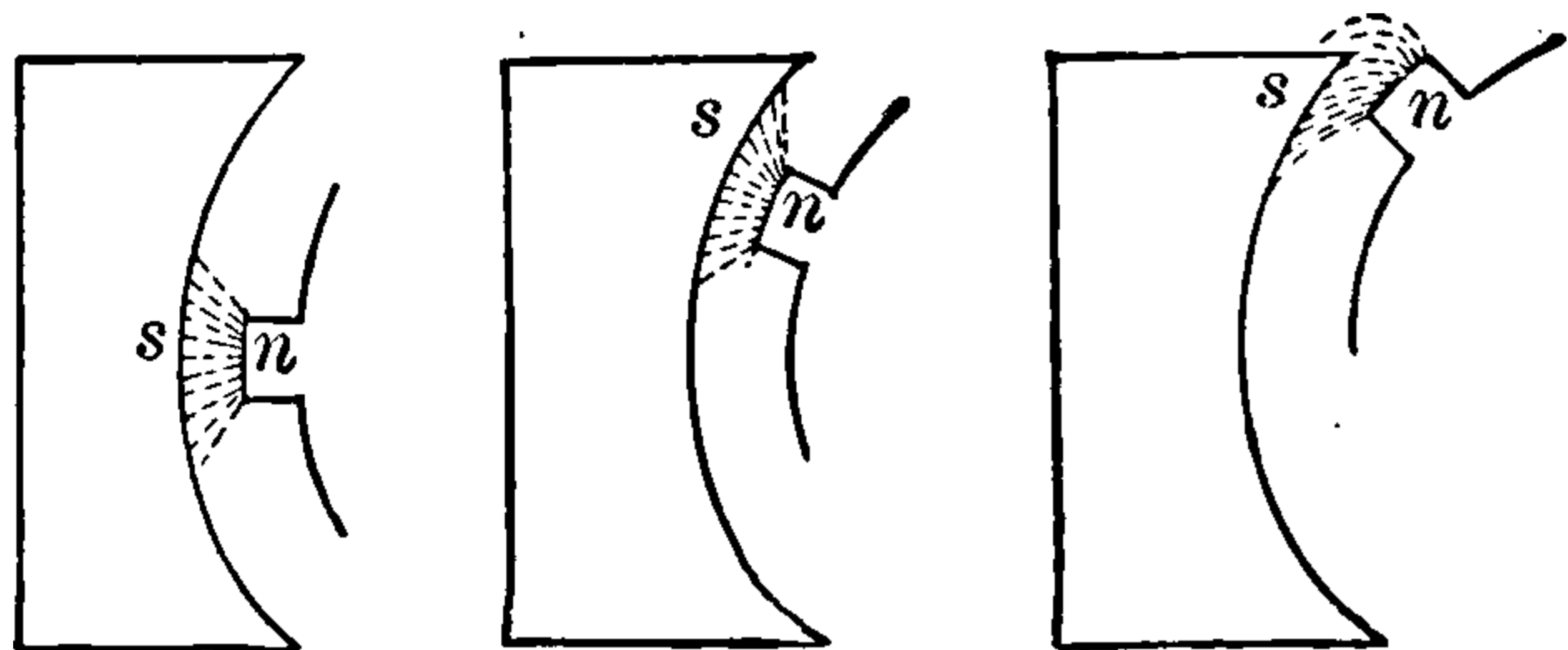
Fig. 184. Foucault Currents in Pole Pieces.
