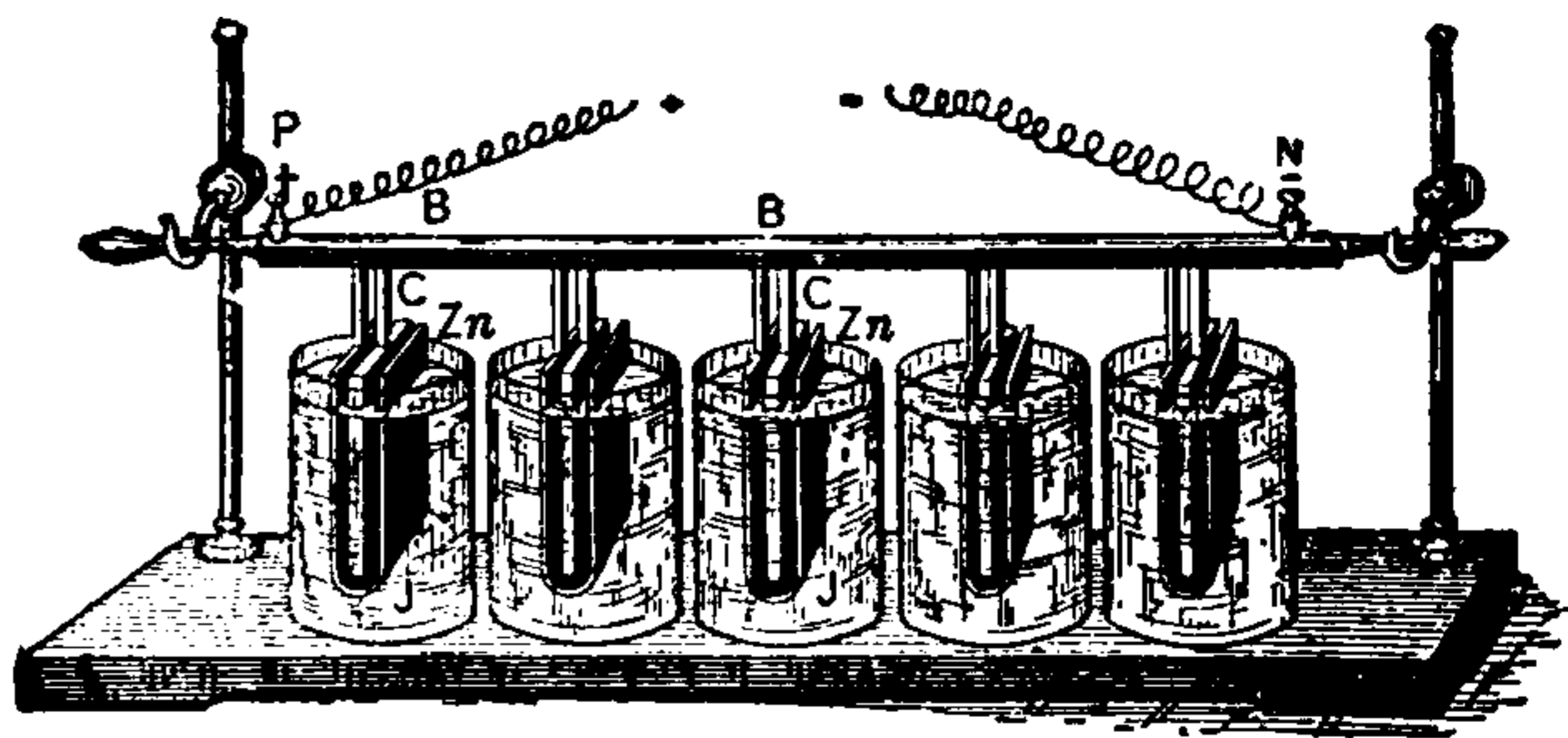
Fig. 42. Plunge Battery.
