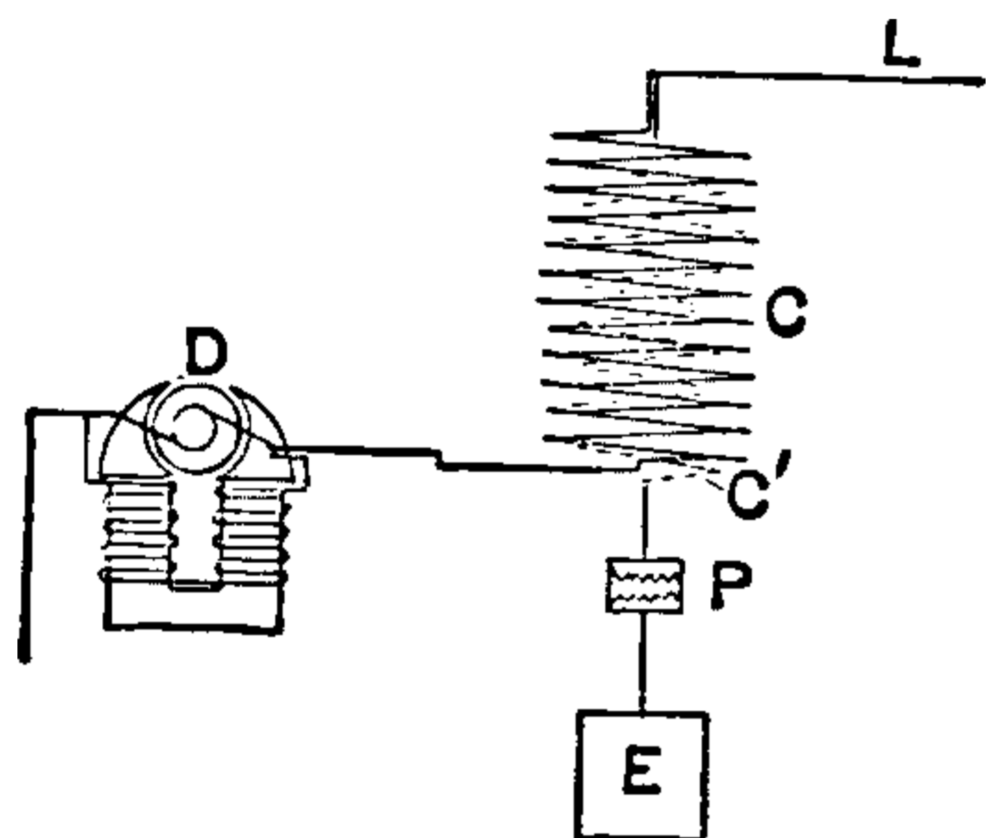
Fig. 26. Counter-Electromotive Force Lightning Arrester.
