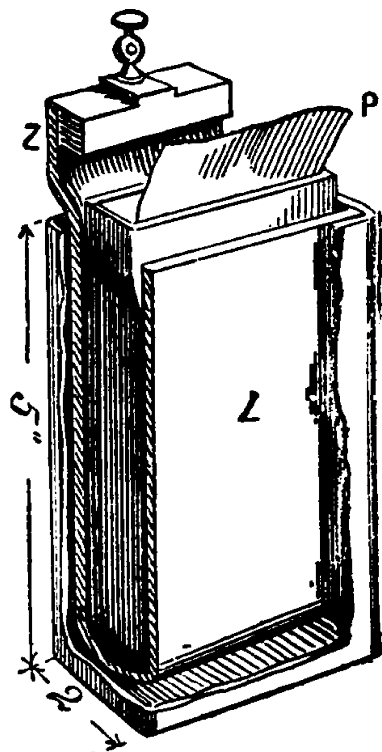
Fig. 110. Grove's Cell.
