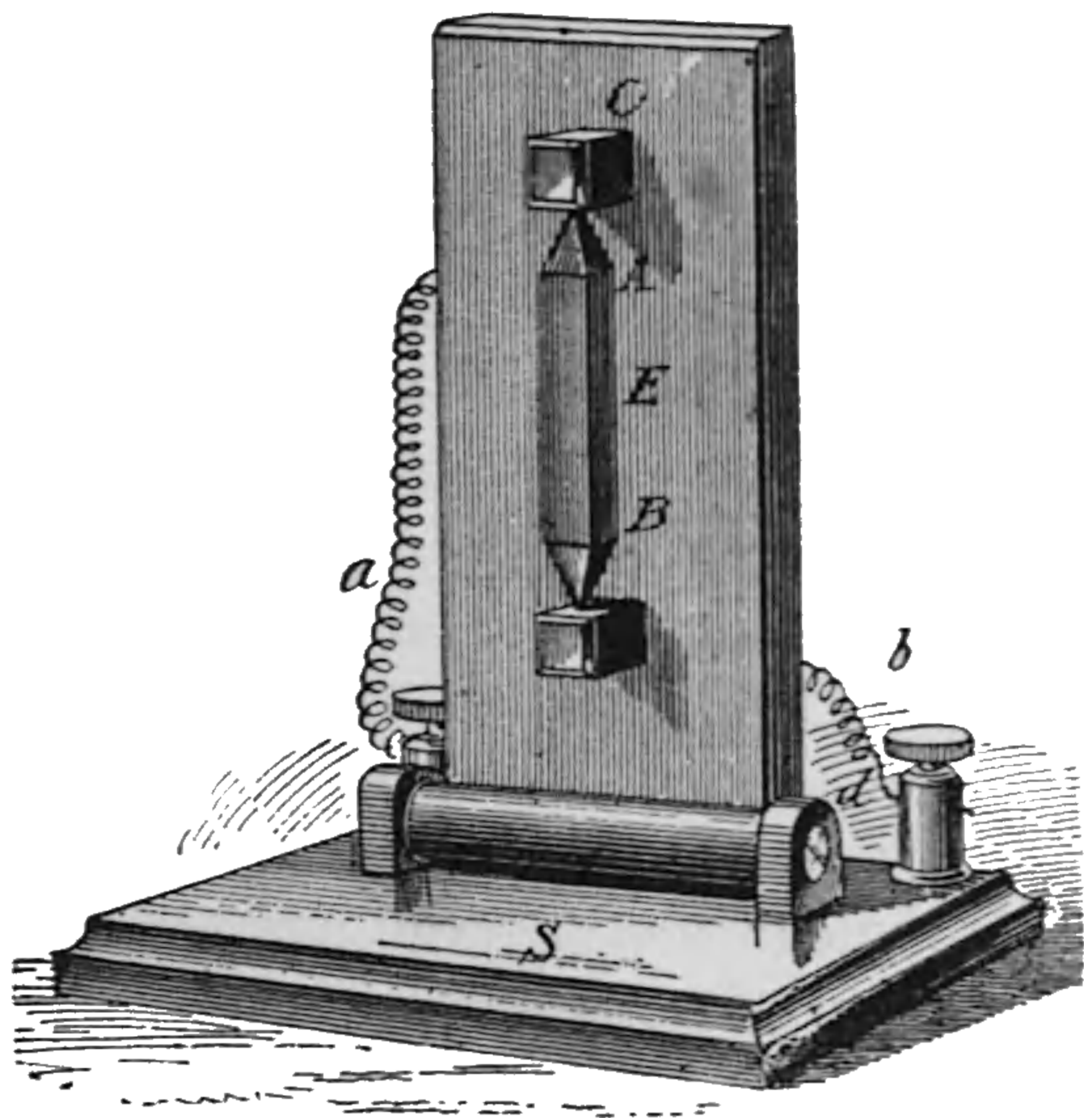
Fig. 397. Microphone.
