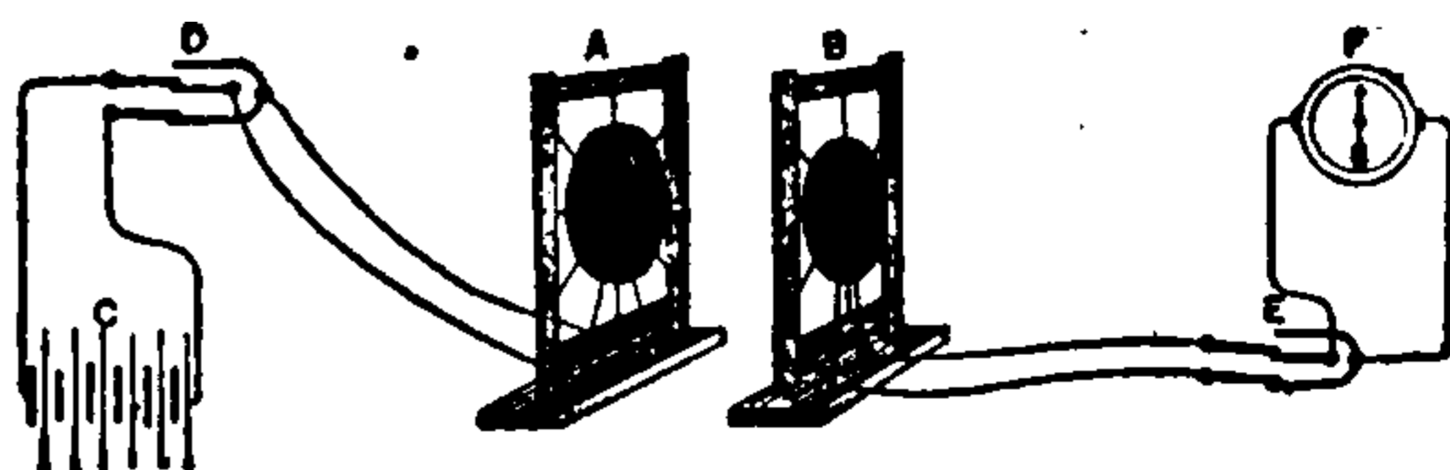
Fig. 500. Willoughby Smith's Apparatus.
