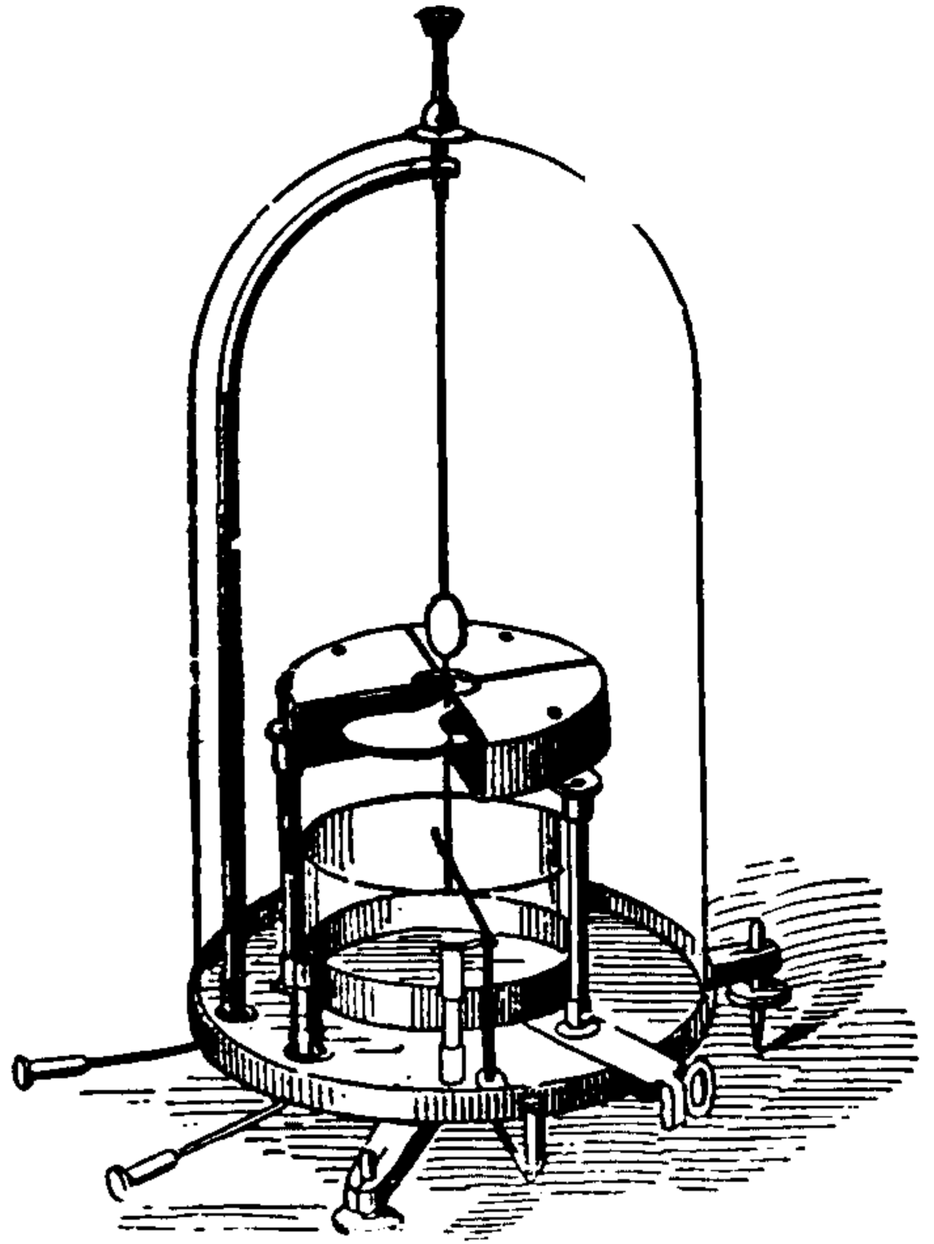
Fig. 233. Quadrant Electrometer, Showing Suspended Needle.
