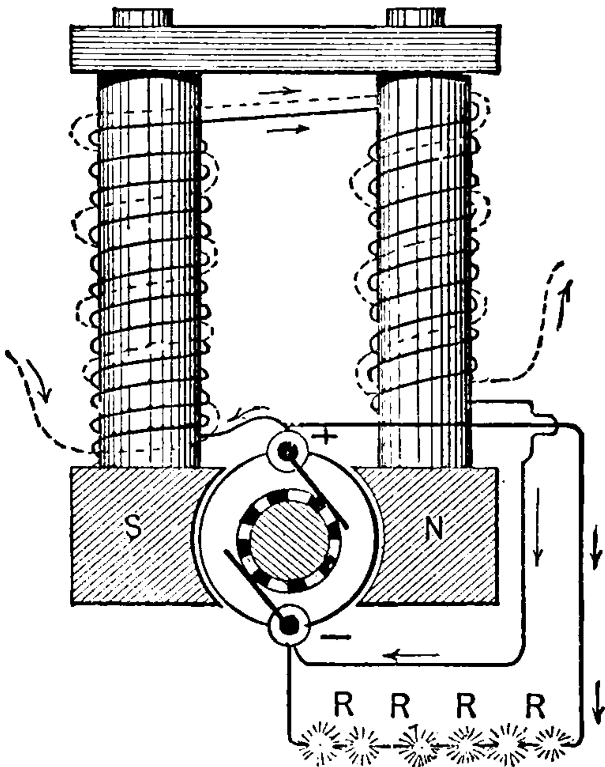
Fig. 356. Shunt and Separately Excited Dynamo.
