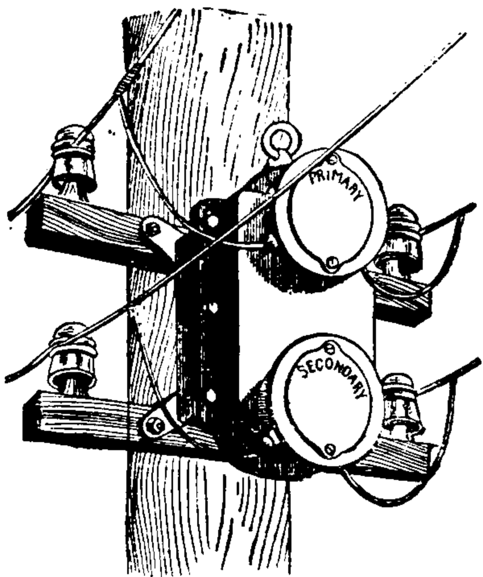
Fig. 558. Transformer Attached to Poles.
