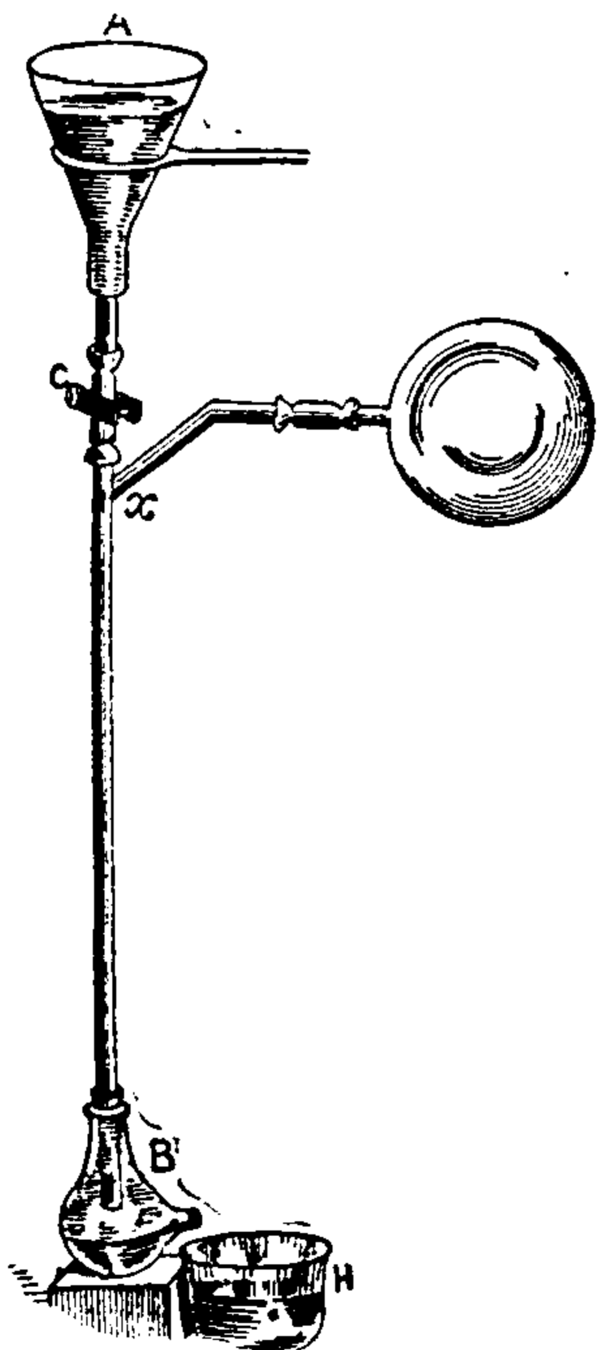
Fig. 456. Sprengel's Mercurial Air Pump.
