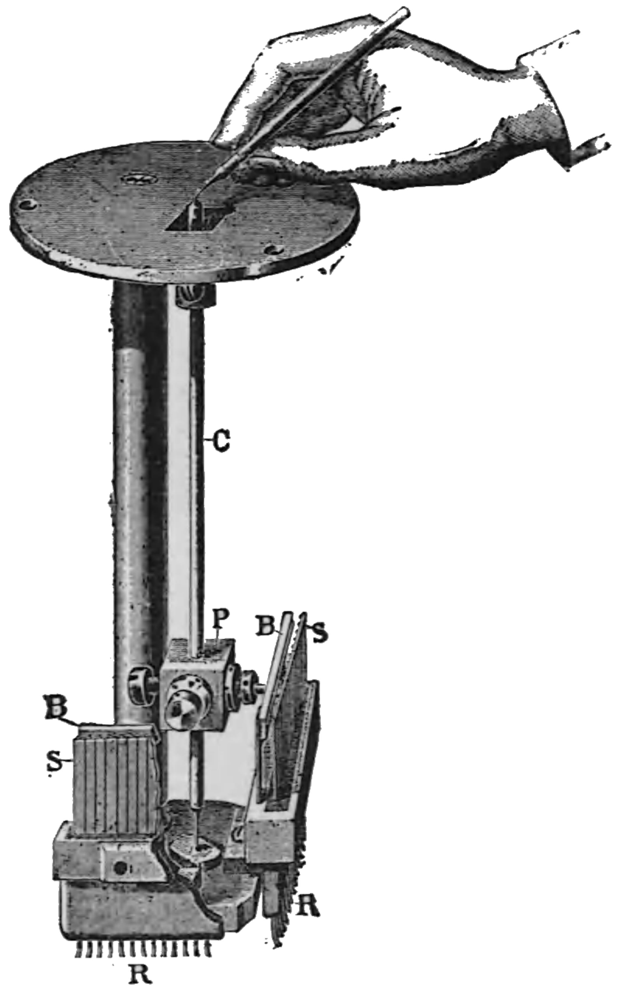
Fig. 547. Transmitter of Writing Telegraphy.
