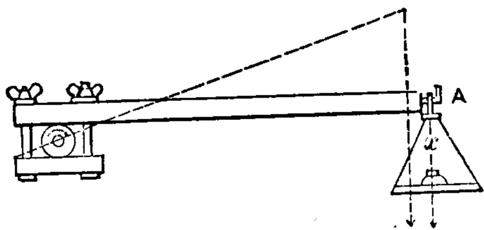
Fig. 69. Prony Brake.
