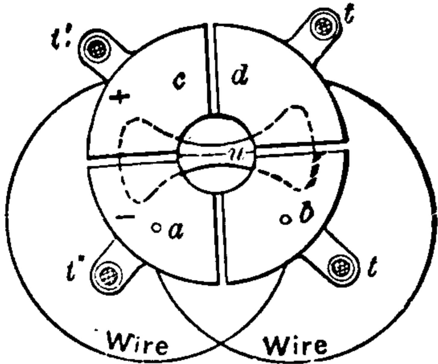
Fig. 232. Quadrant Electrometer.
