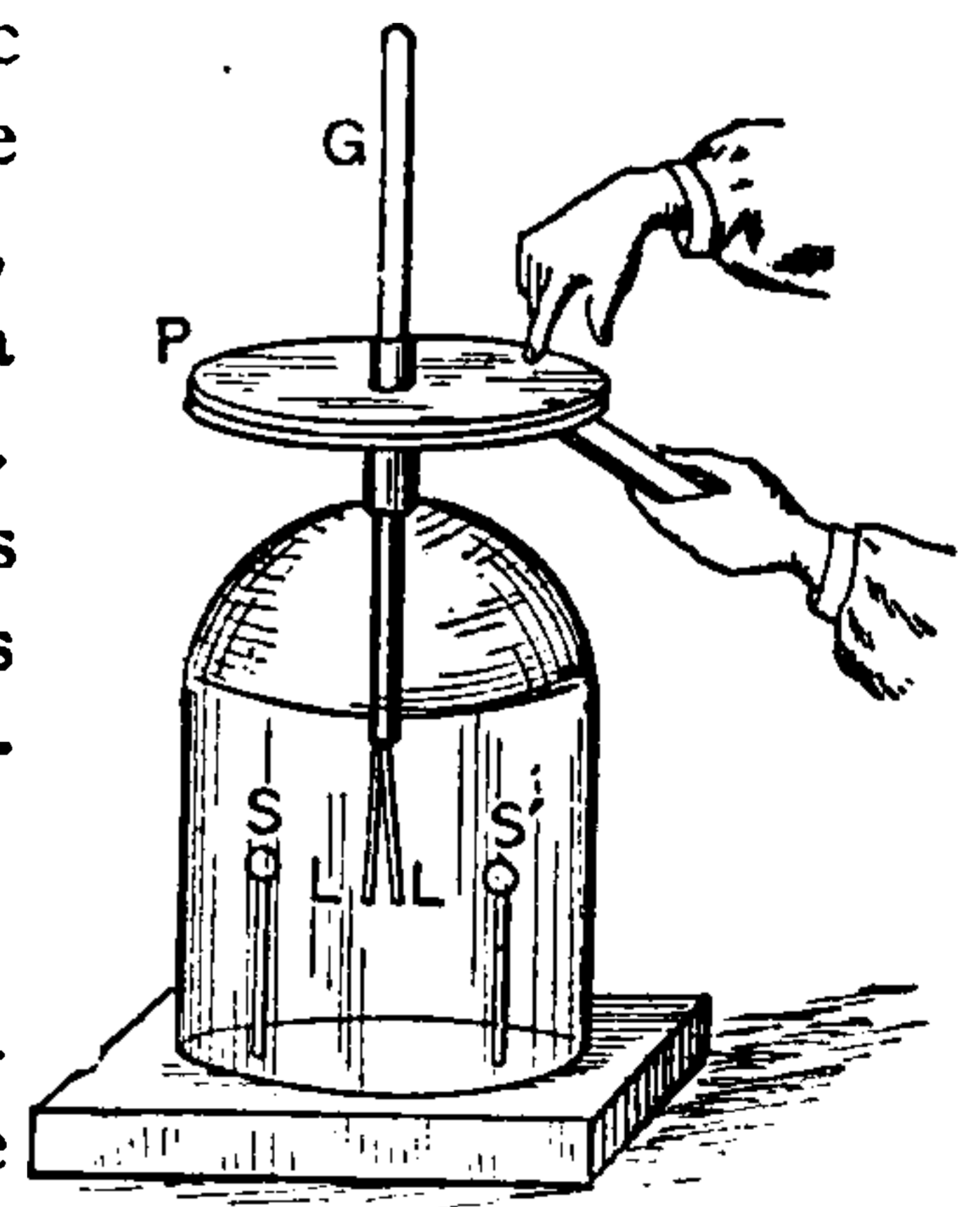
Fig. 238. Condensing Electroscope.
