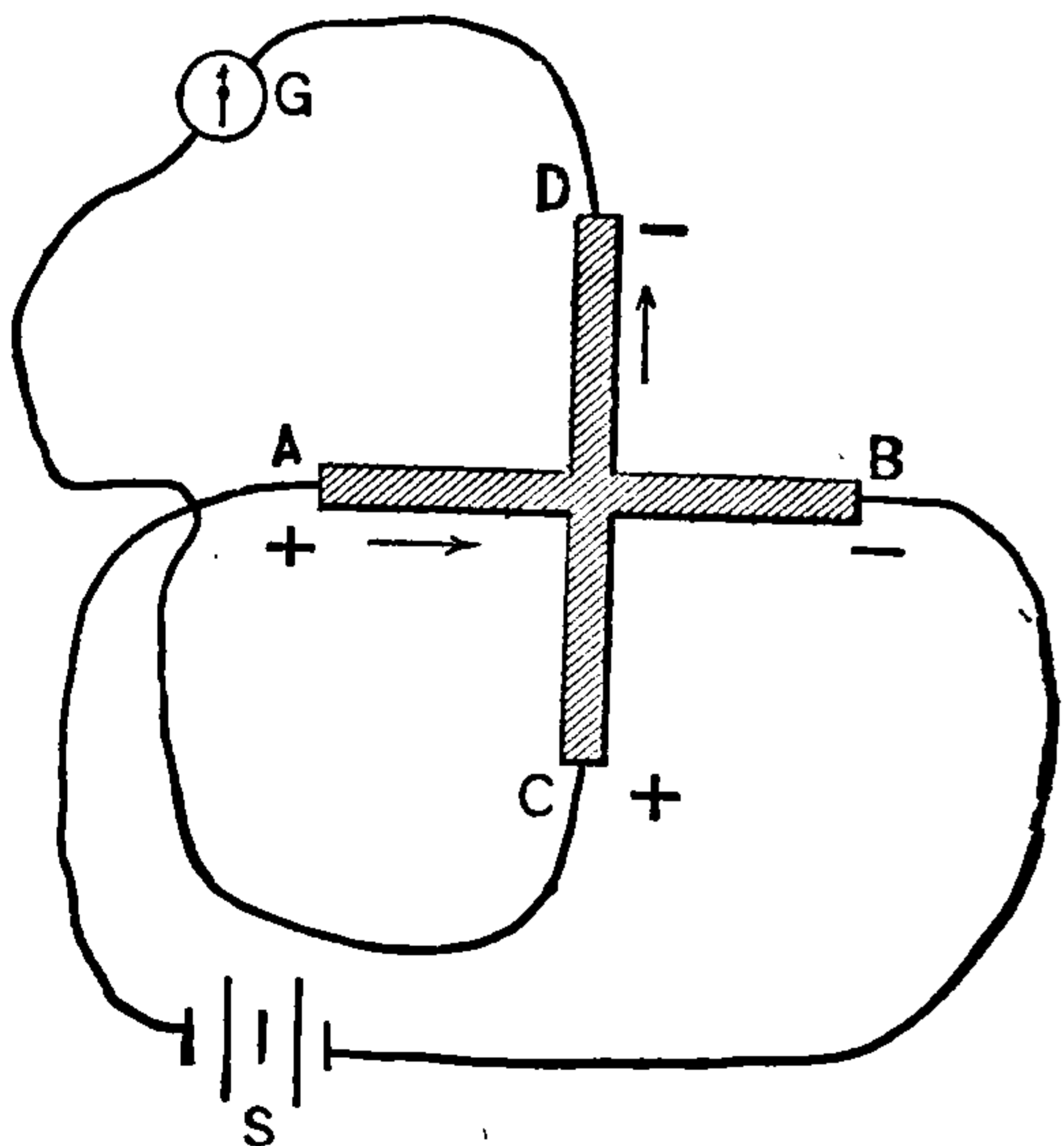
Fig. 226. Hall Effect.
