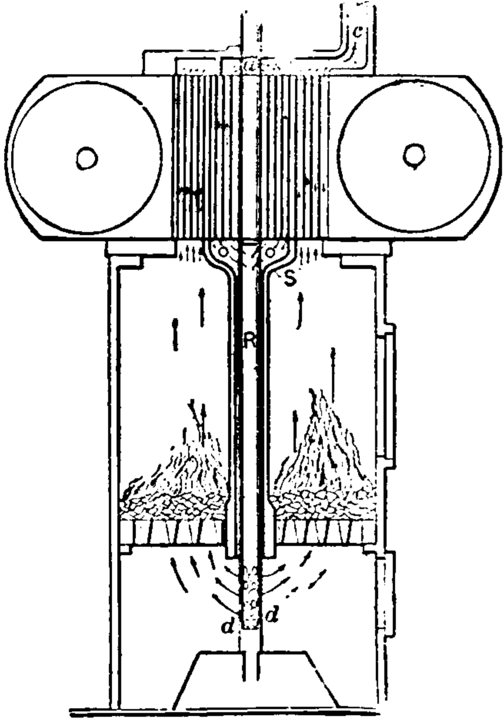
Fig. 400. Pyromagnetic Motor.
