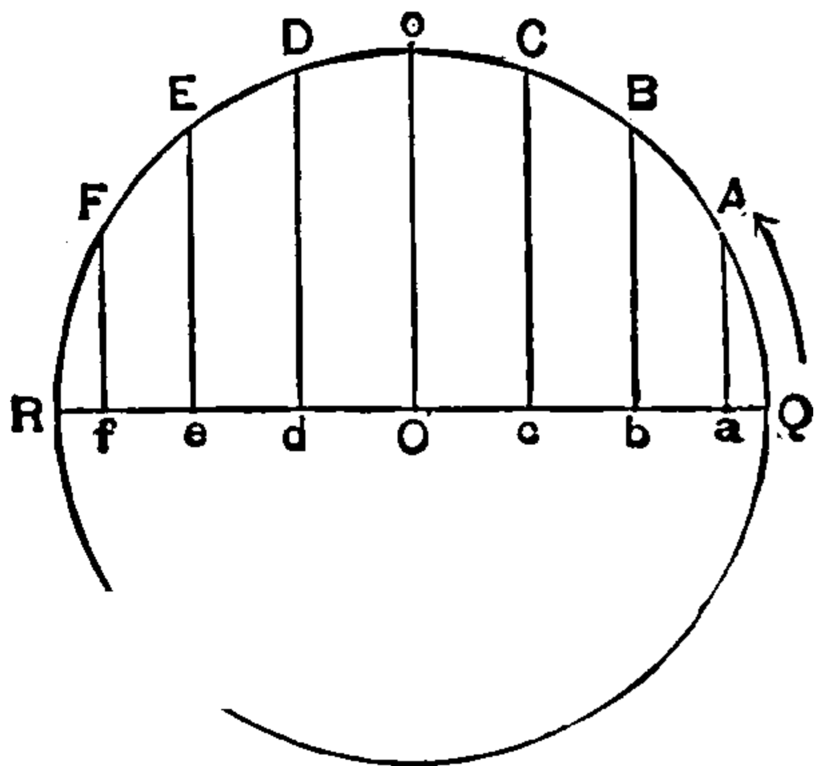
Fig. 398. Simple-Harmonic Motion.
