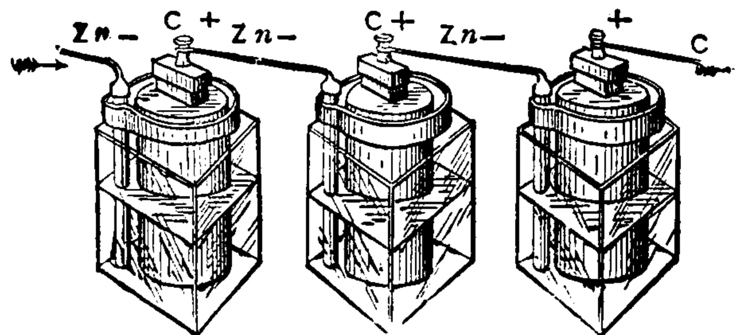
Fig. 133. Voltaic Cells Connected in Series.
