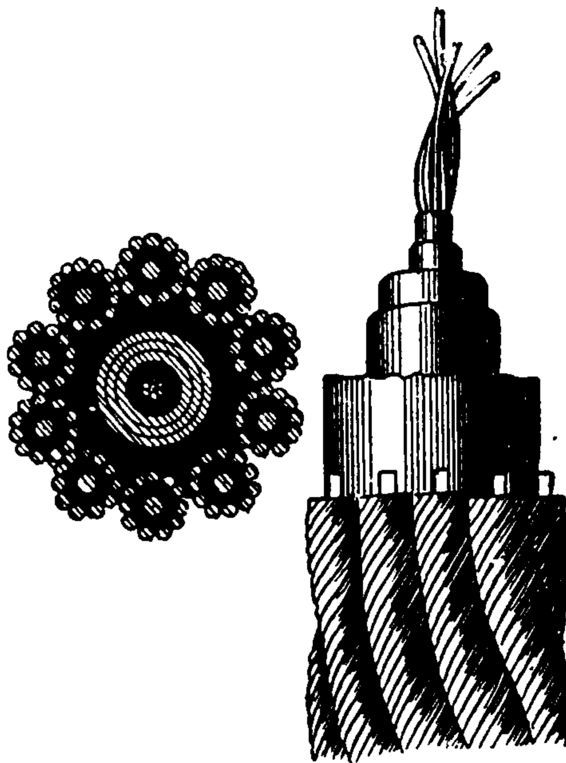
Fig. 94. Electric Cable .
