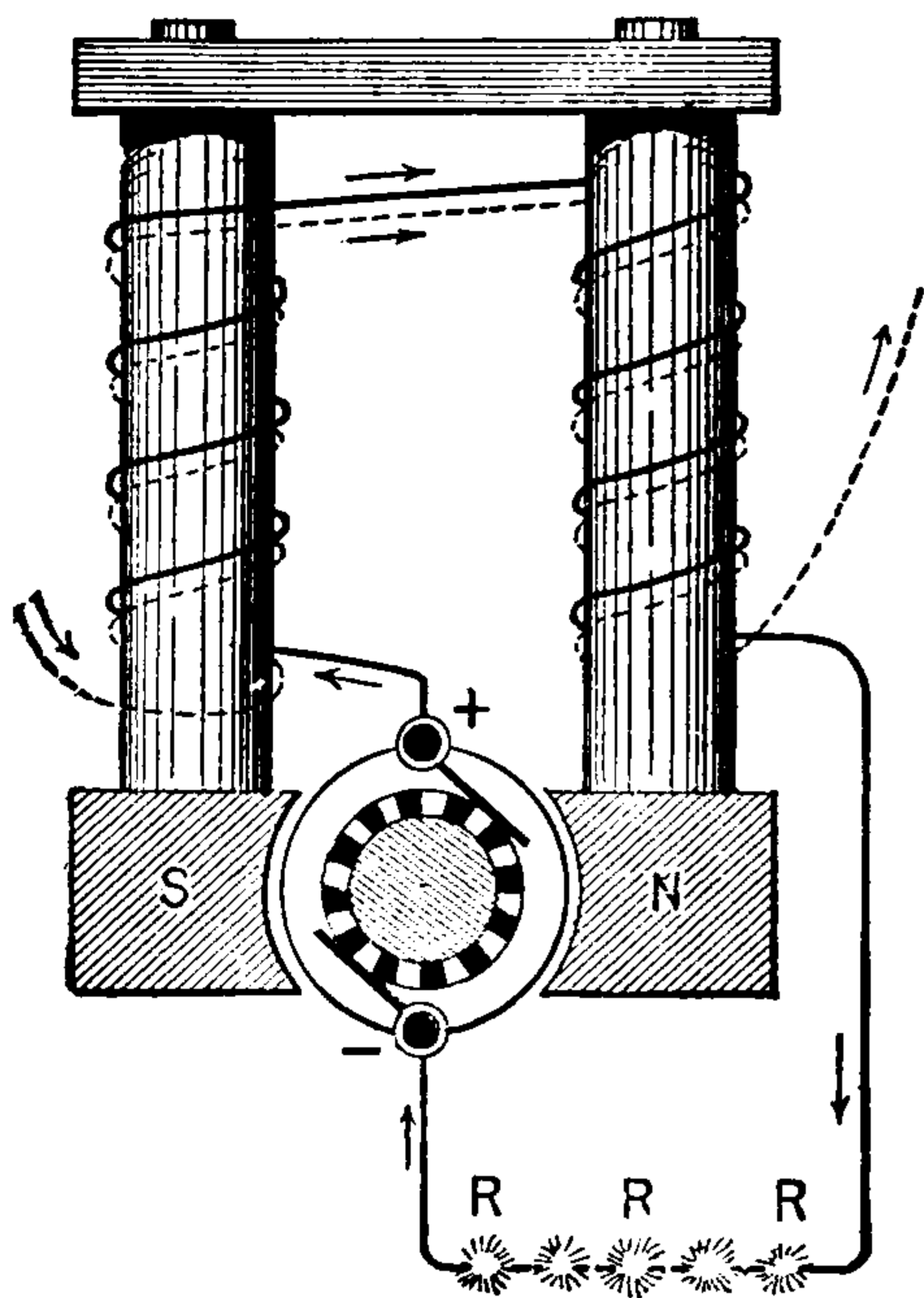
Fig. 352. Series and Separately Excited Dynamo.
