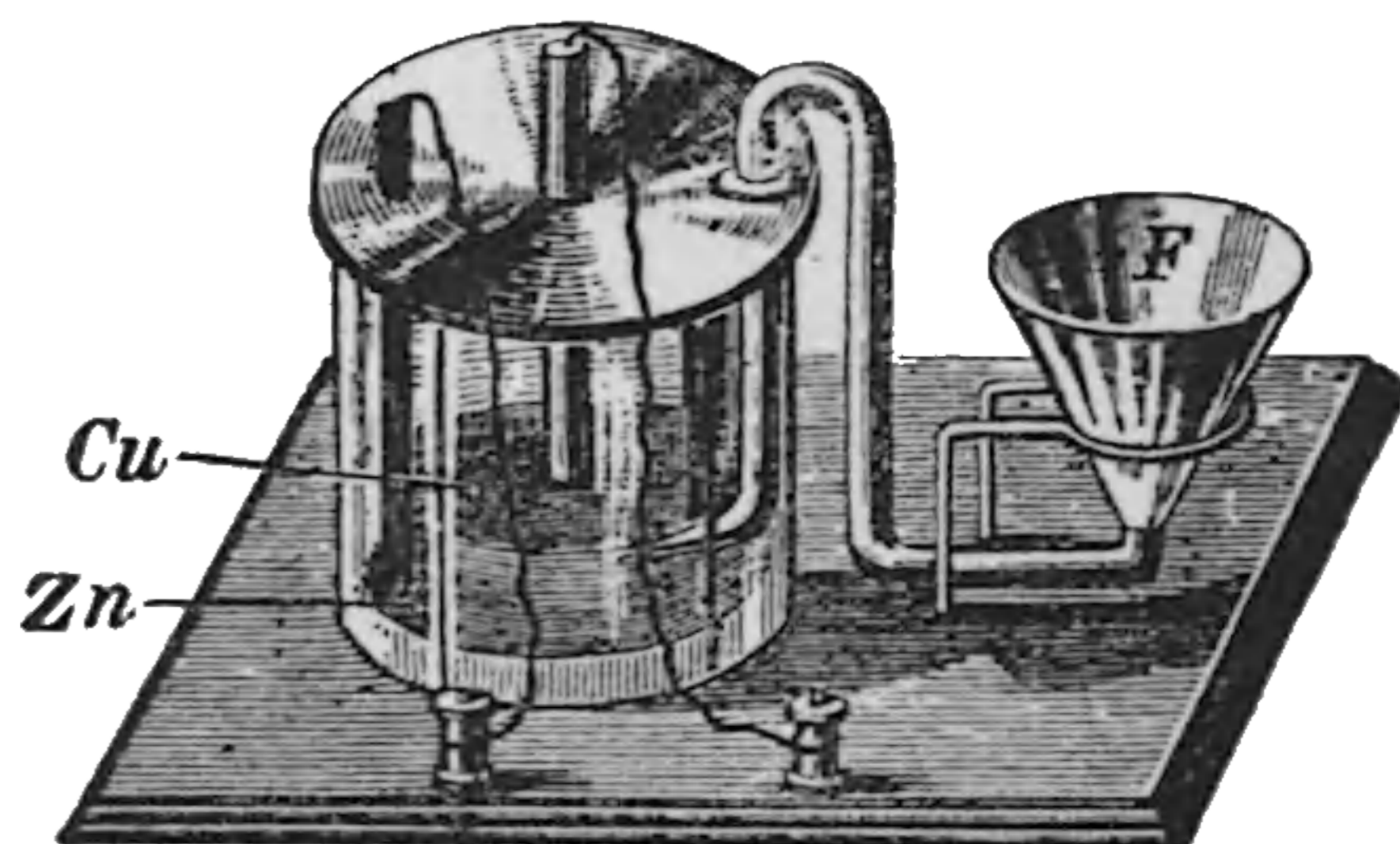
Fig. 119. Thomson's Form of Daniell's Cell.
