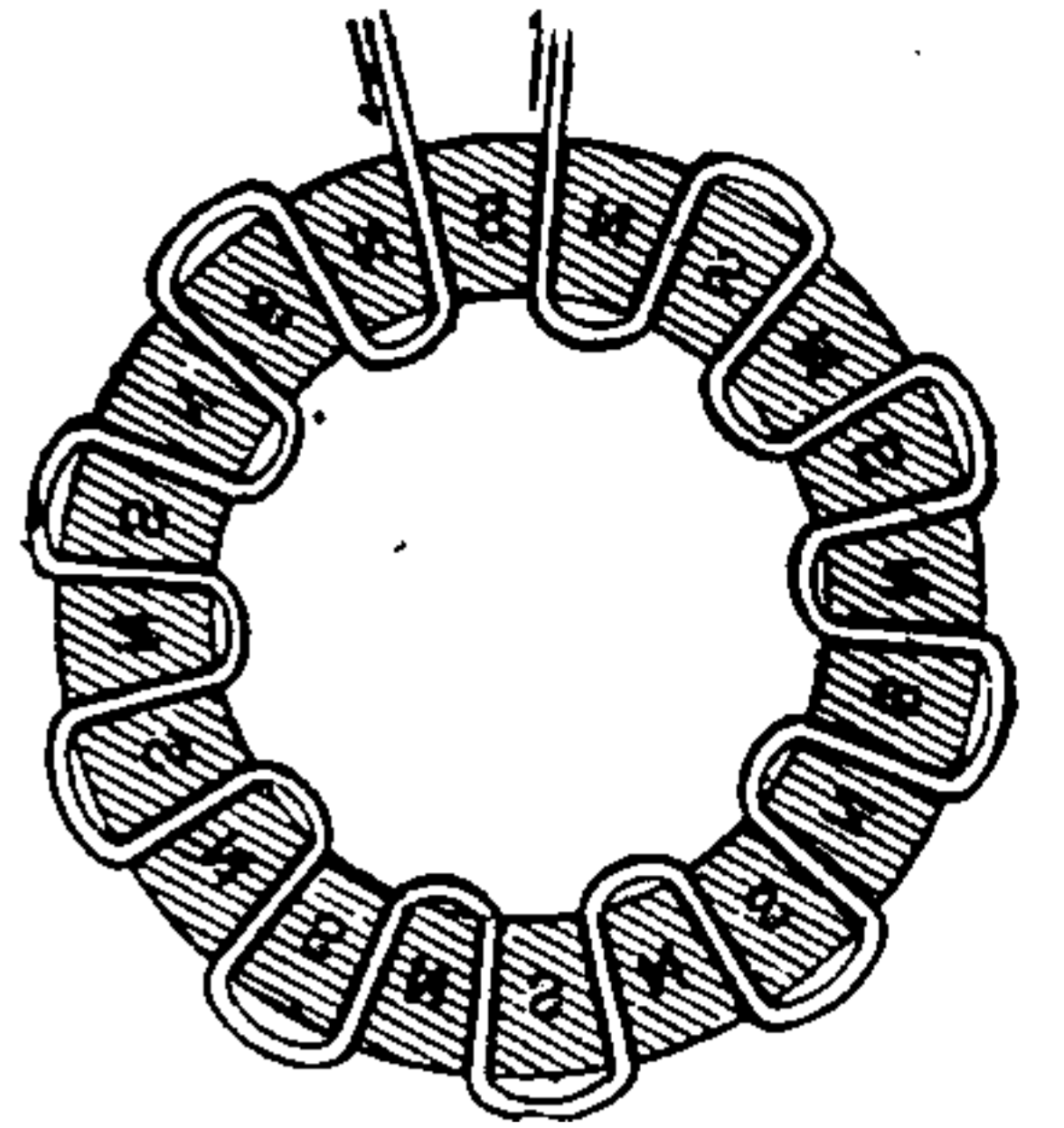
Fig 378 Zigzag Electro-Magnet.
