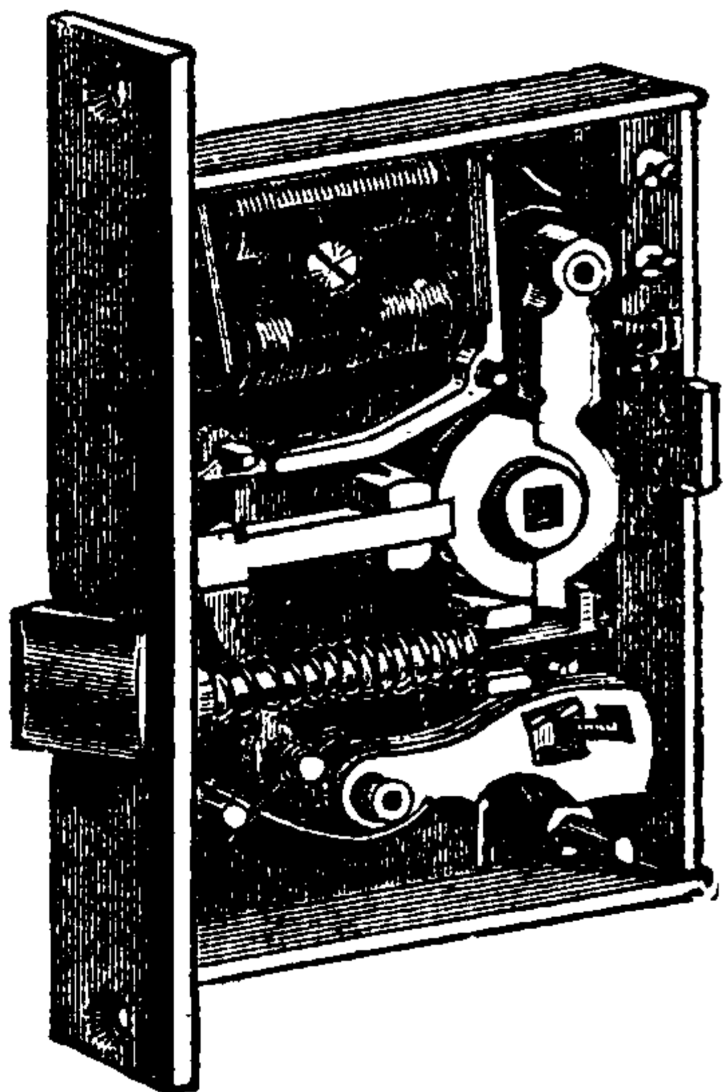
Fig. 347. Electric Lock.
