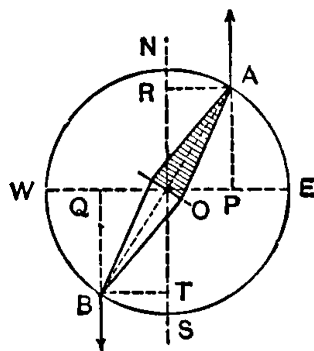
Fig. 174. Magnetic Couple.
