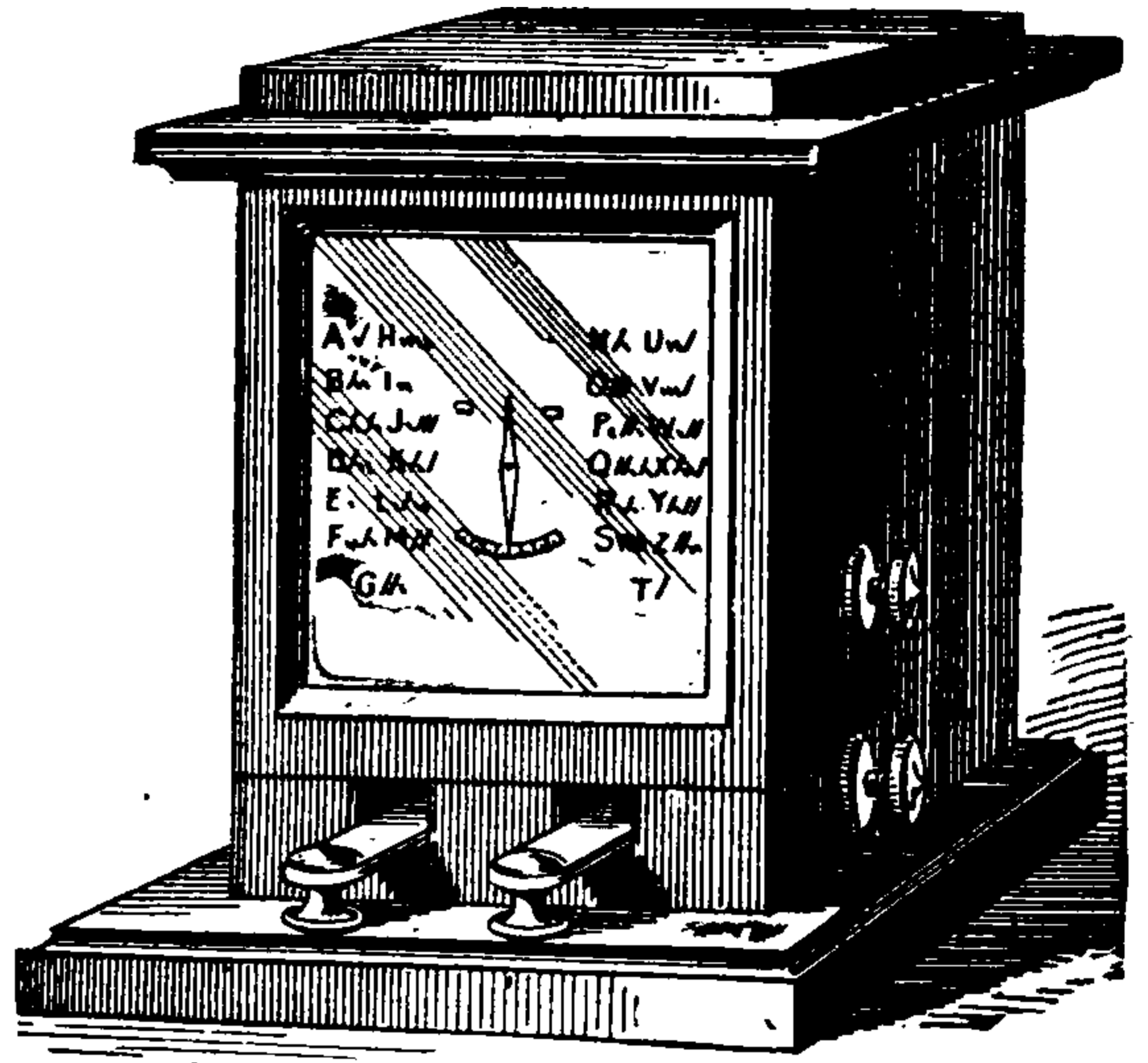
Fig. 537. Wheatstone and Cooke's Single-Needle Apparatus, External View.
