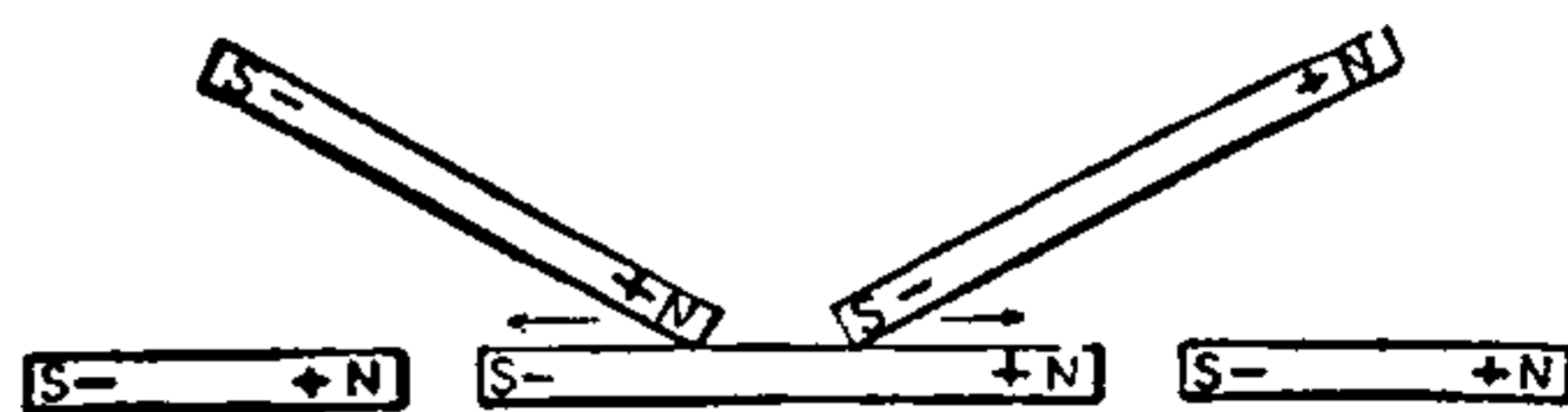
Fig. 385. Magnetization by Separate Touch.
