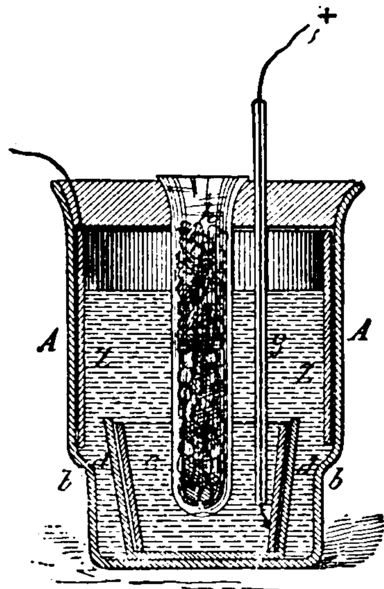
Fig. 112. The Meidinger Cell.
