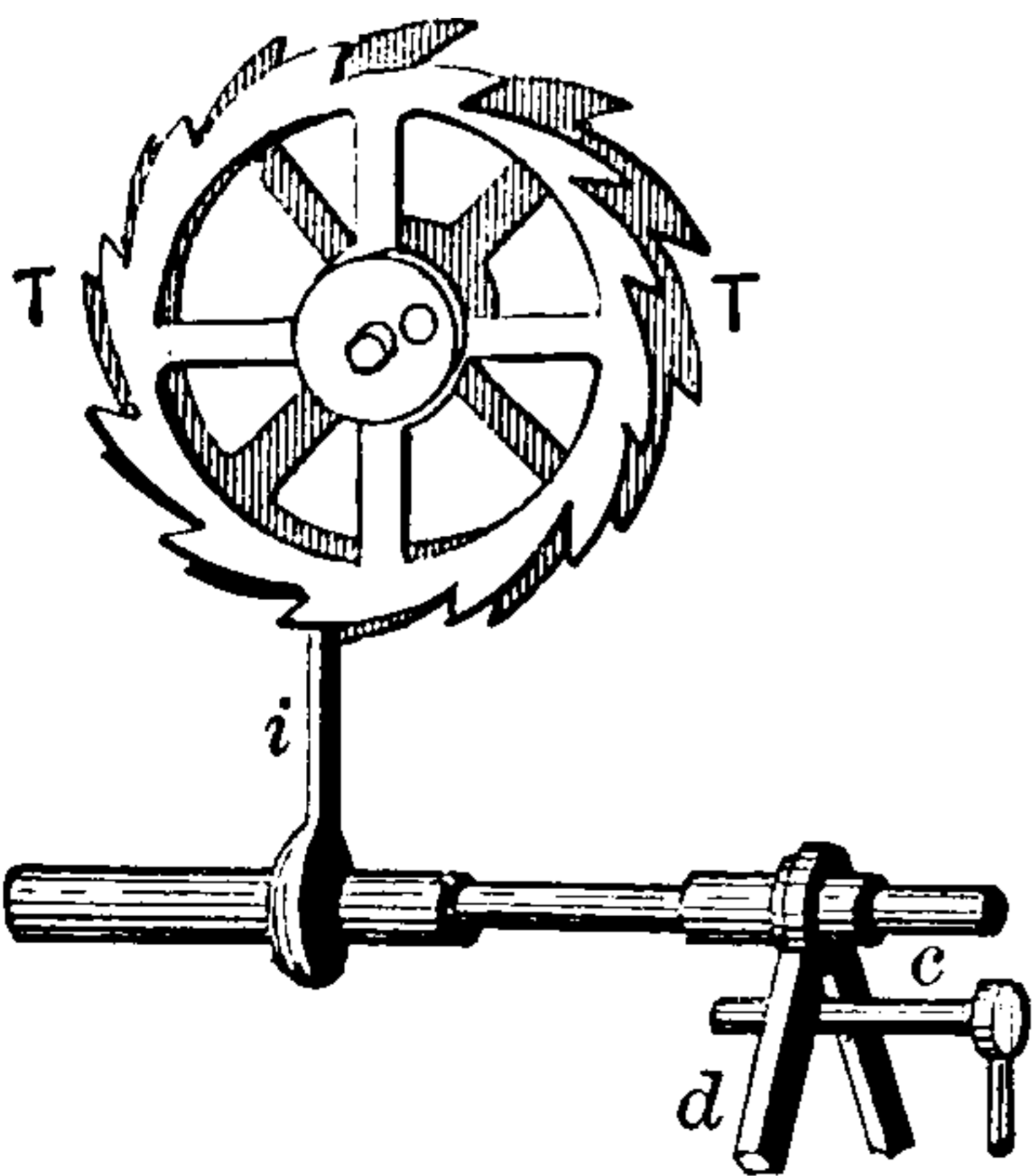
Fig. 540. Step-by-Step Wheel.
