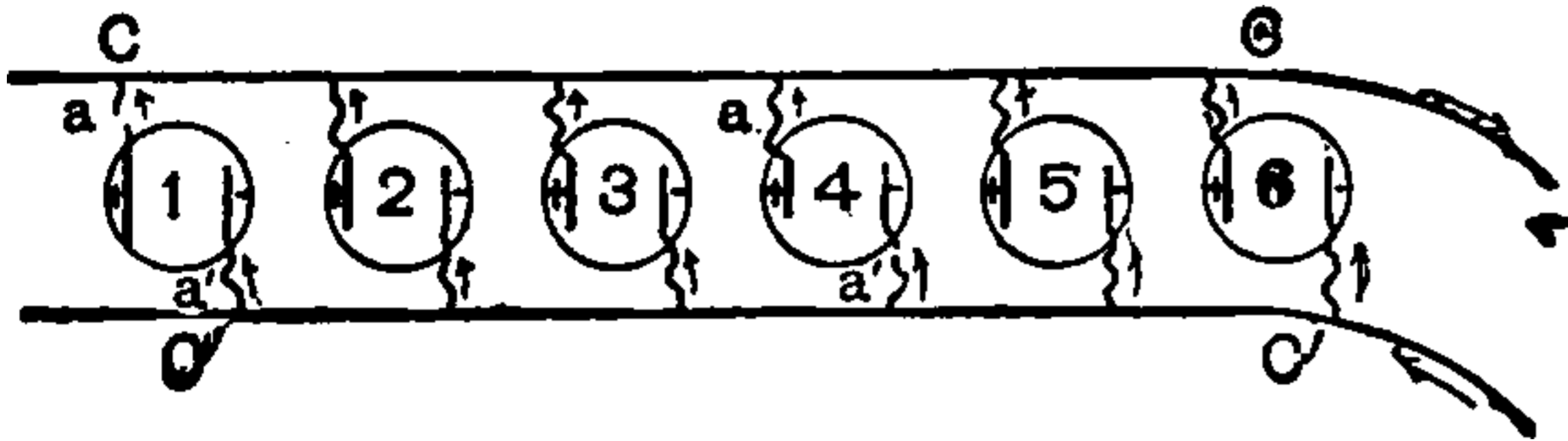
Fig. 129. Six Cells Connected in Multiple.
