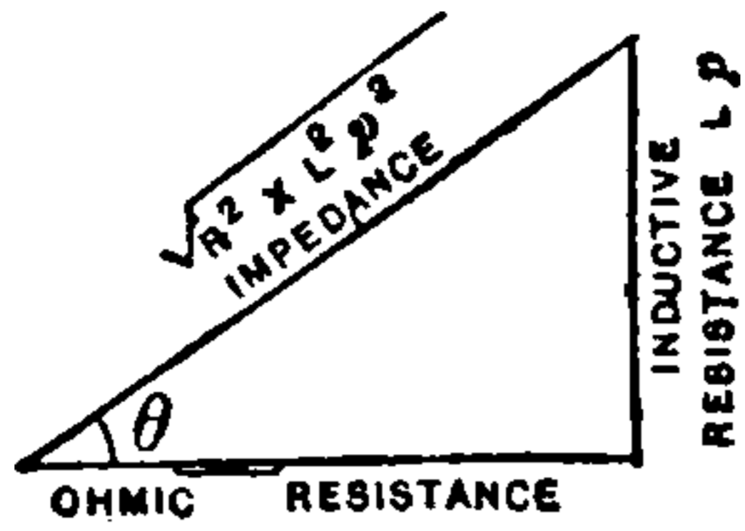
Fig. 296. Geometrical Representation of Impedance.
