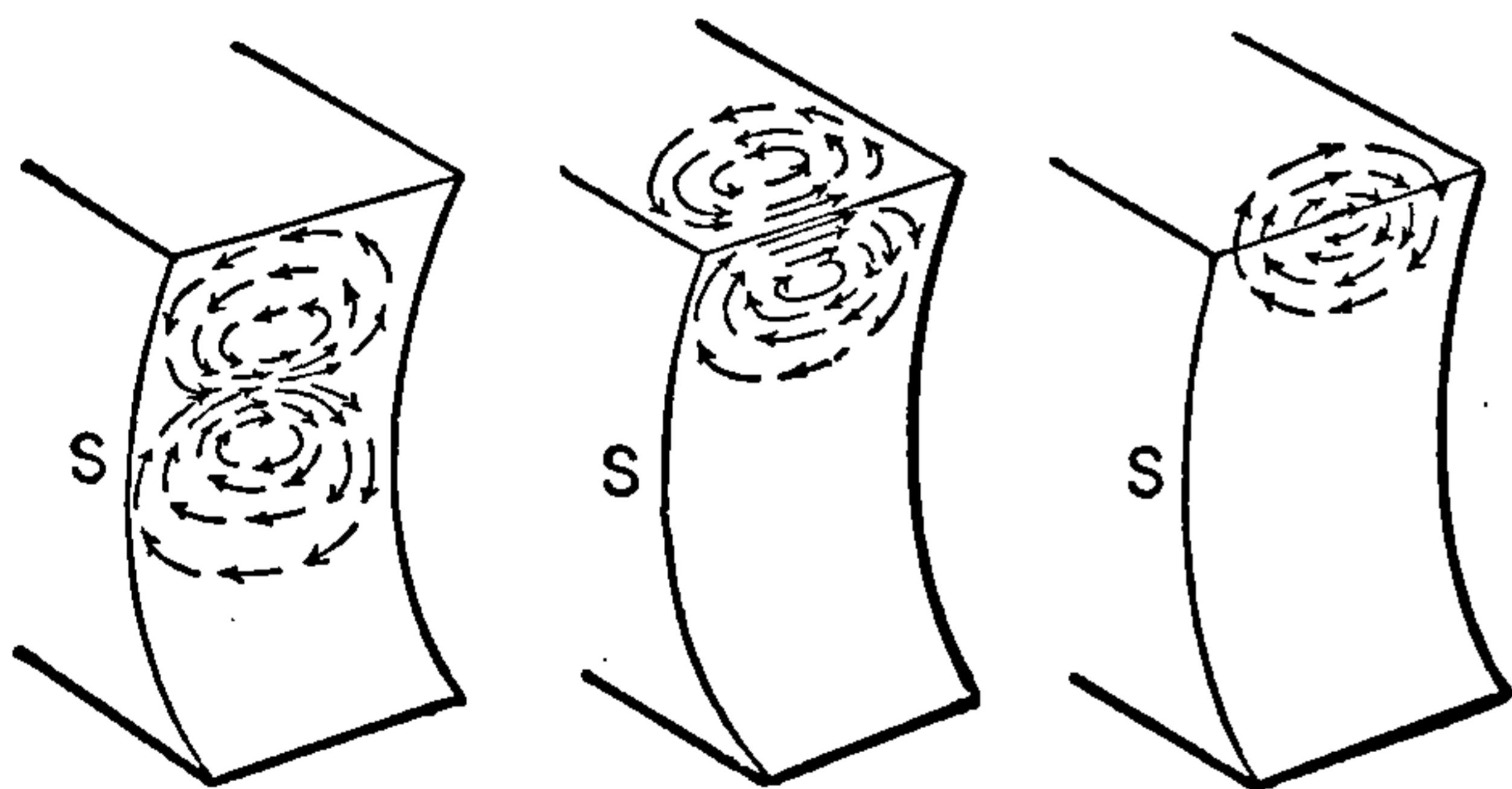
Fig. 185. Foucault Currents in Pole Pieces.
