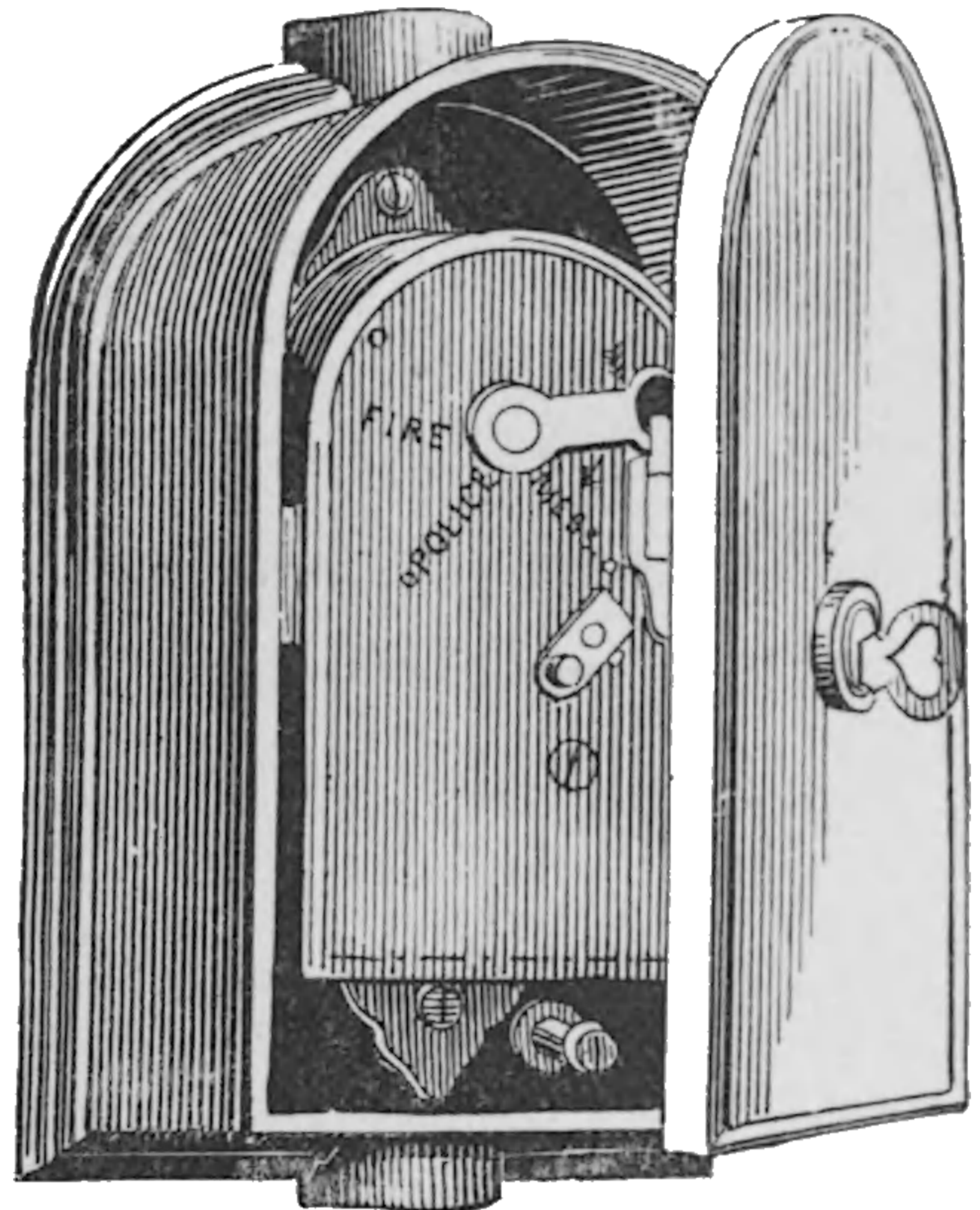
Fig. 62. Patrol Box.
