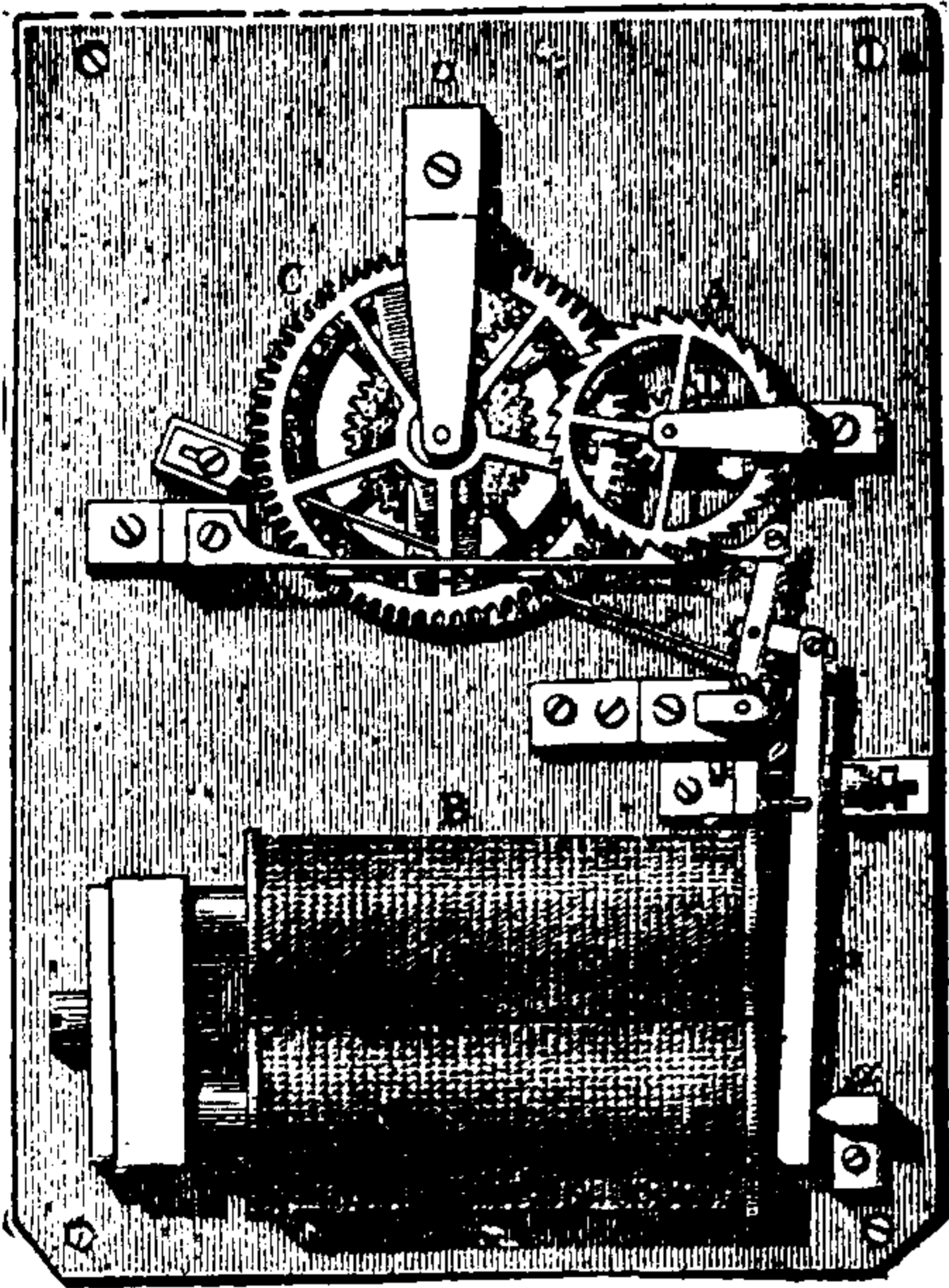
Fig. 139. Mechanism of Secondary Clock.
