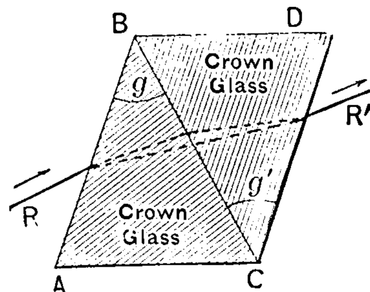
Fig. 342. Equal and Opposite Refracting Angles.
