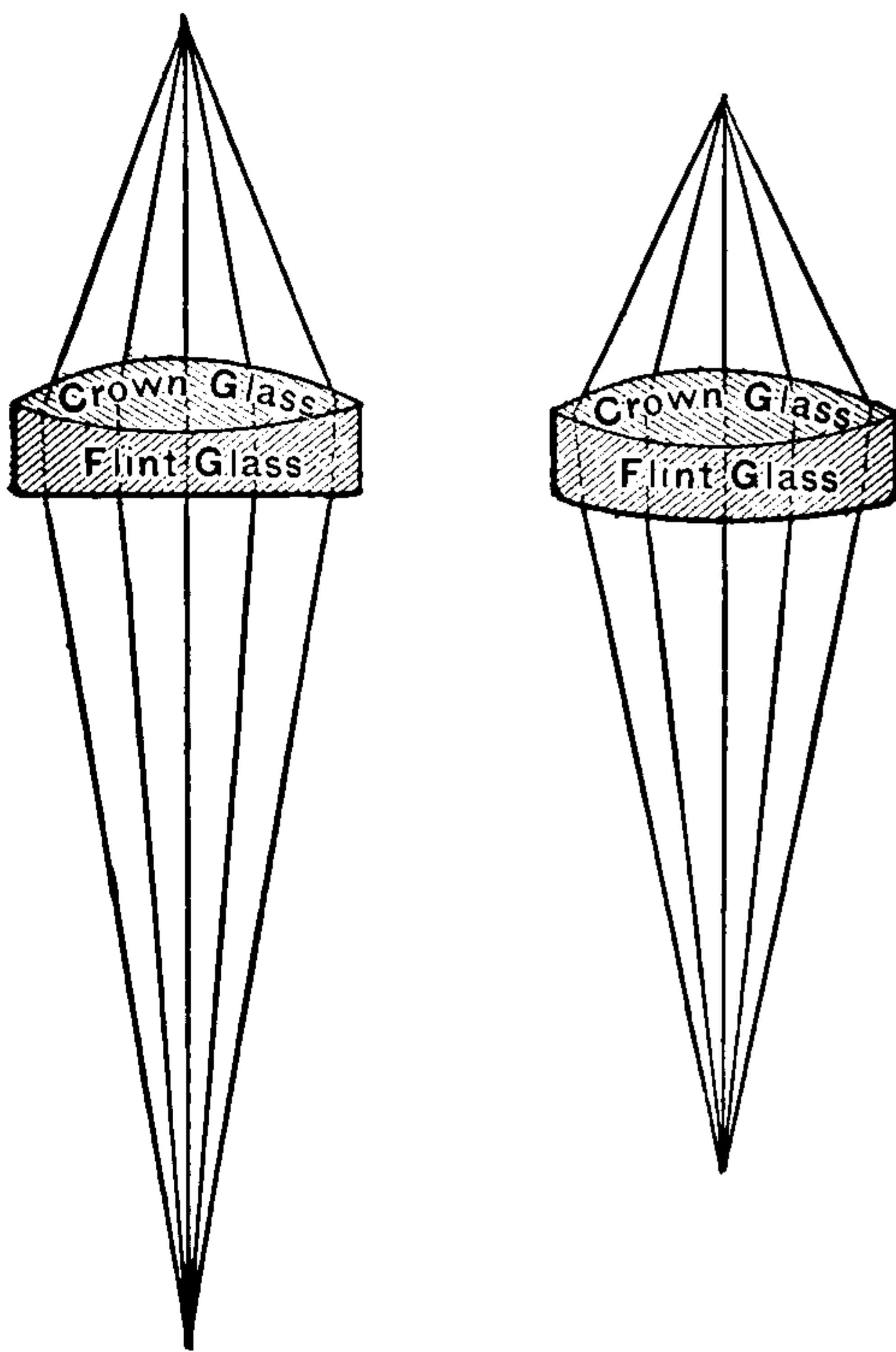
Fig. 344. Plano-Convex Achromatic Lens. Fig. 345. Achromatic Lens.
