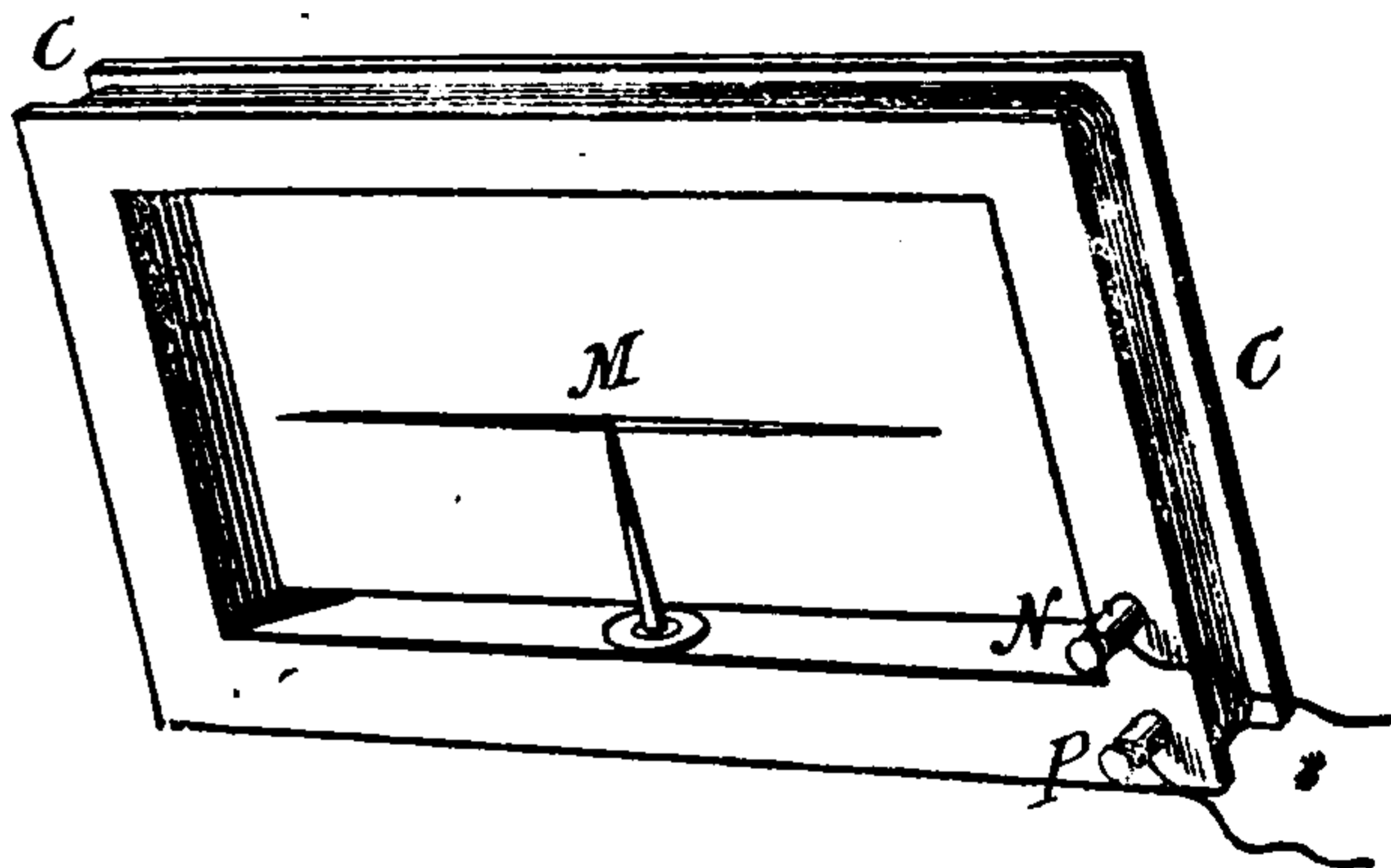
Fig. 266. Schweigger's Multiplier.
