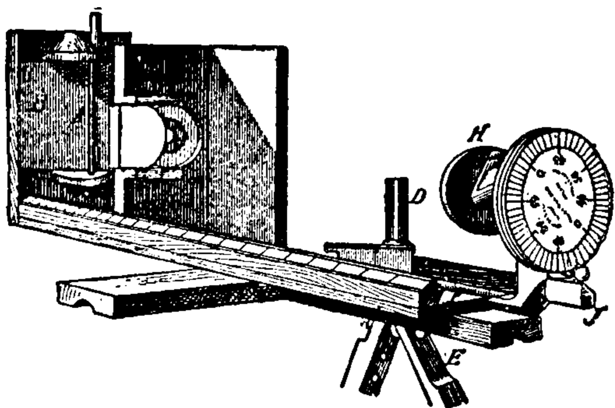
Fig. 428. Ayrton & Perry's Dispersion Photometer.
