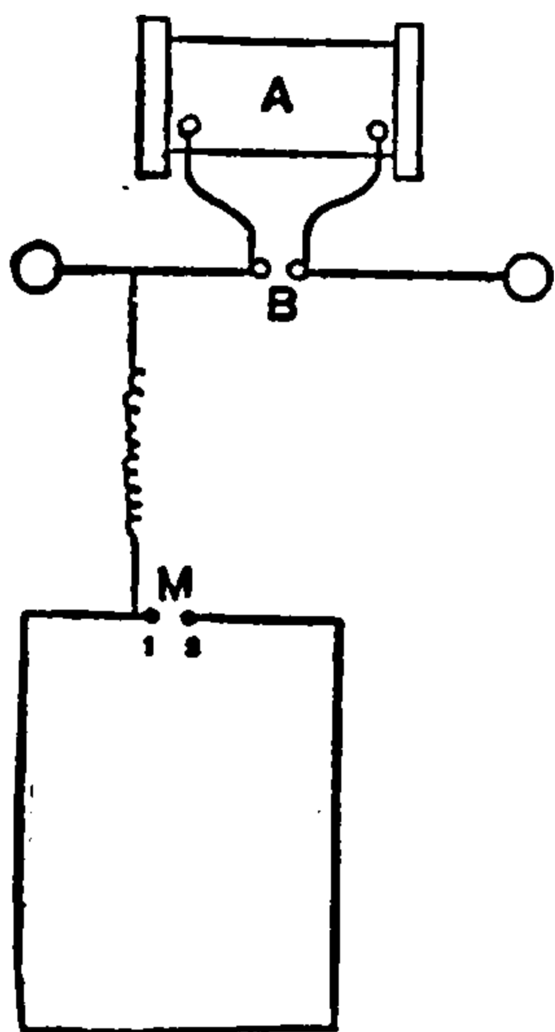
Fig. 492. Electrical Resonance.
