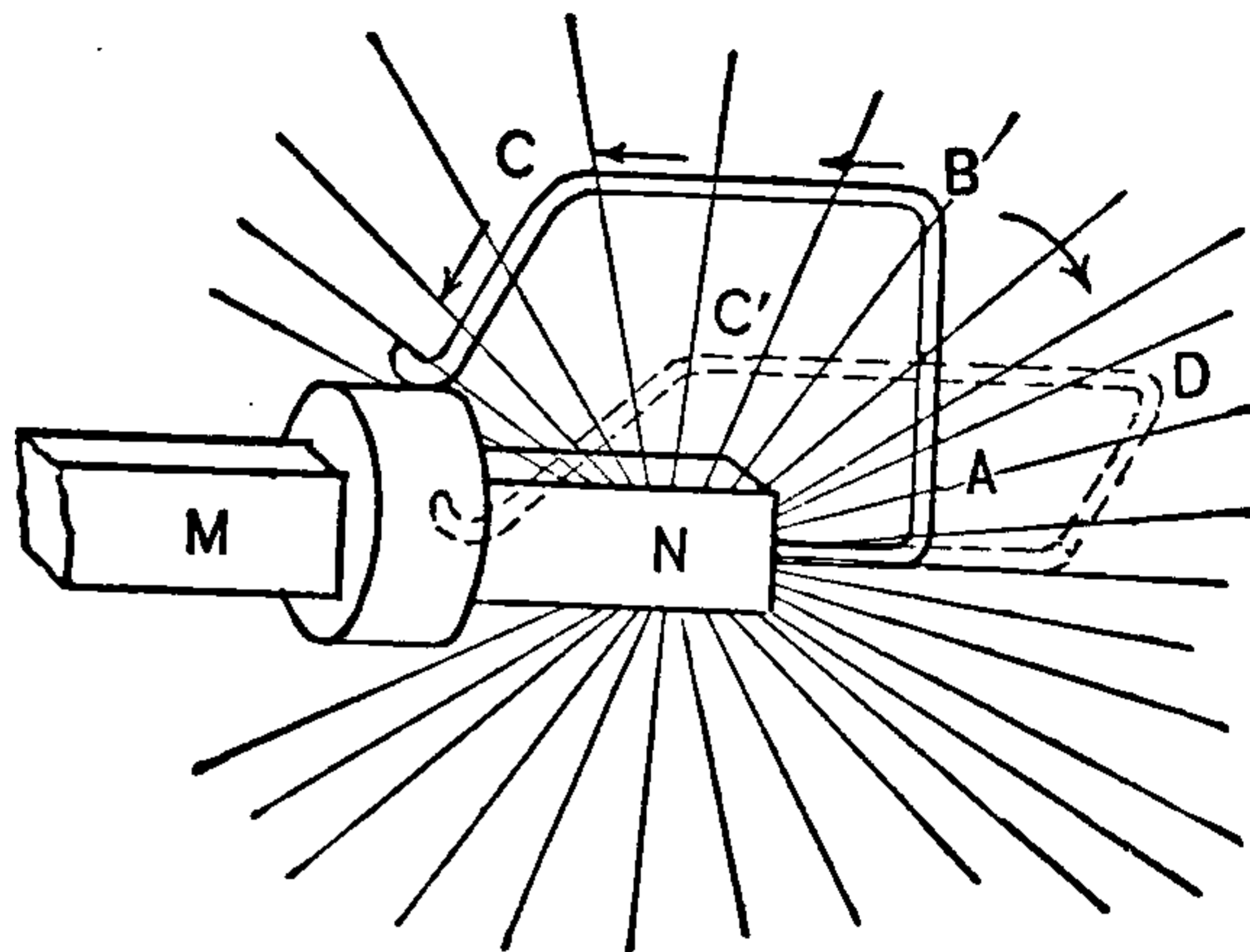
Fig. 309. Unipolar Induction.
