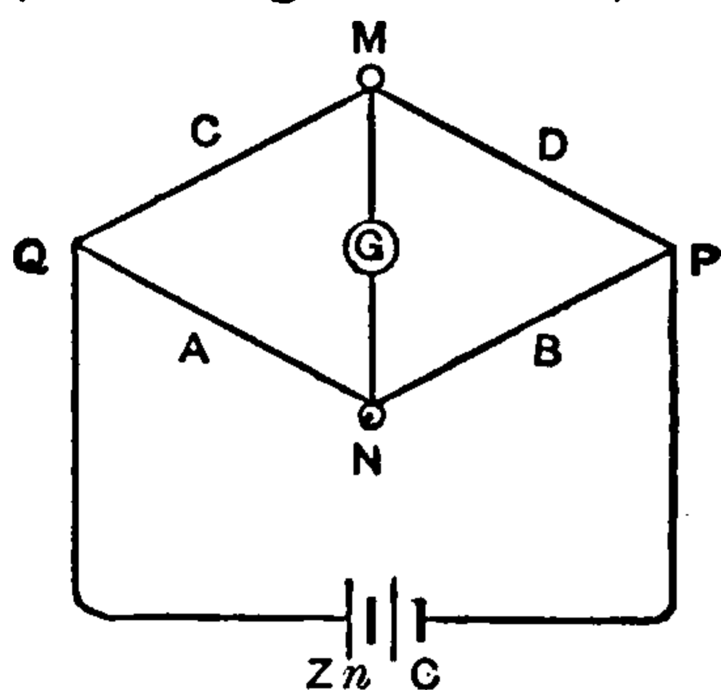
Fig. 24. Arms of Balance.
