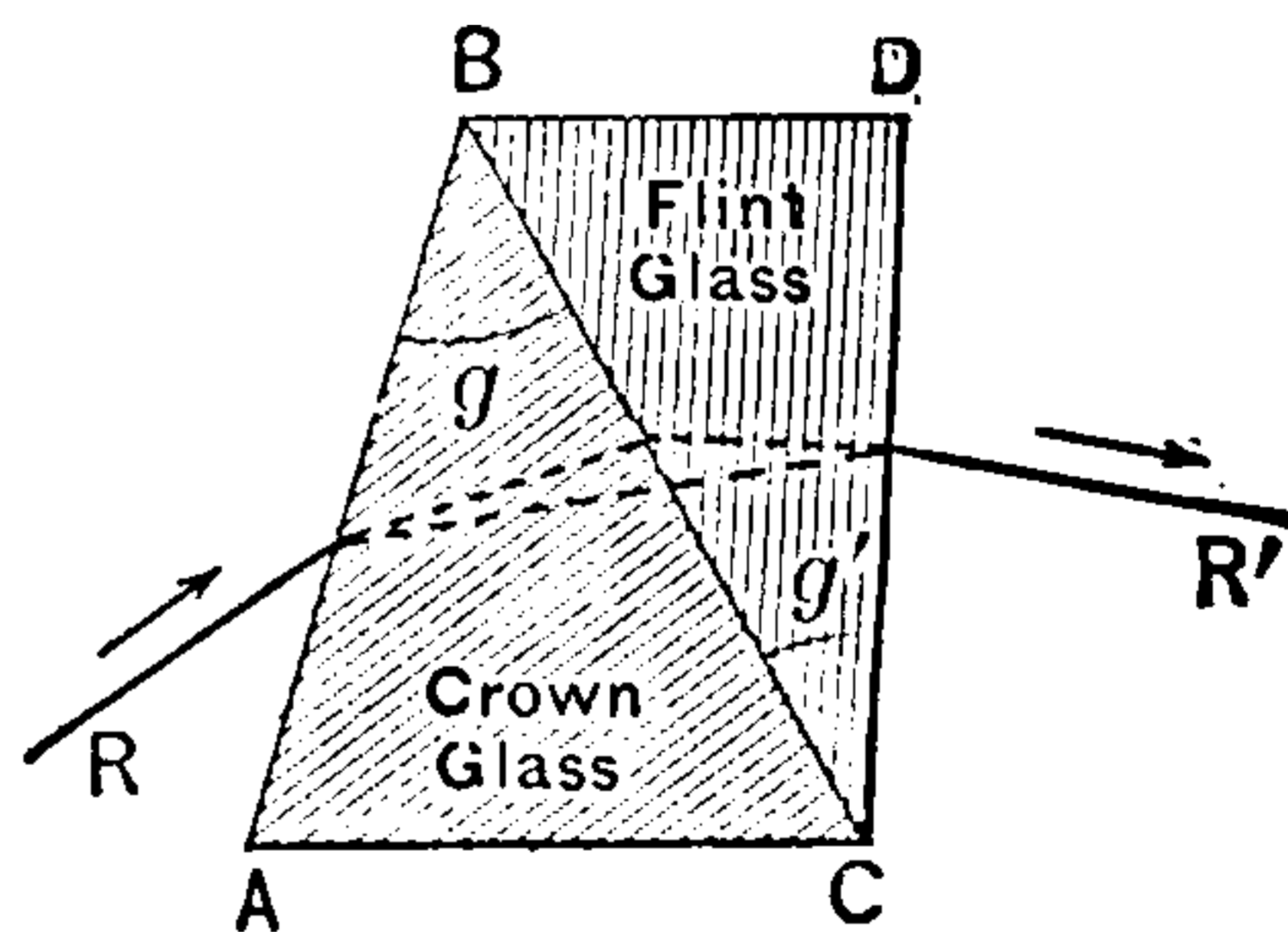
Fig. 343. Principle of Achromatism.
