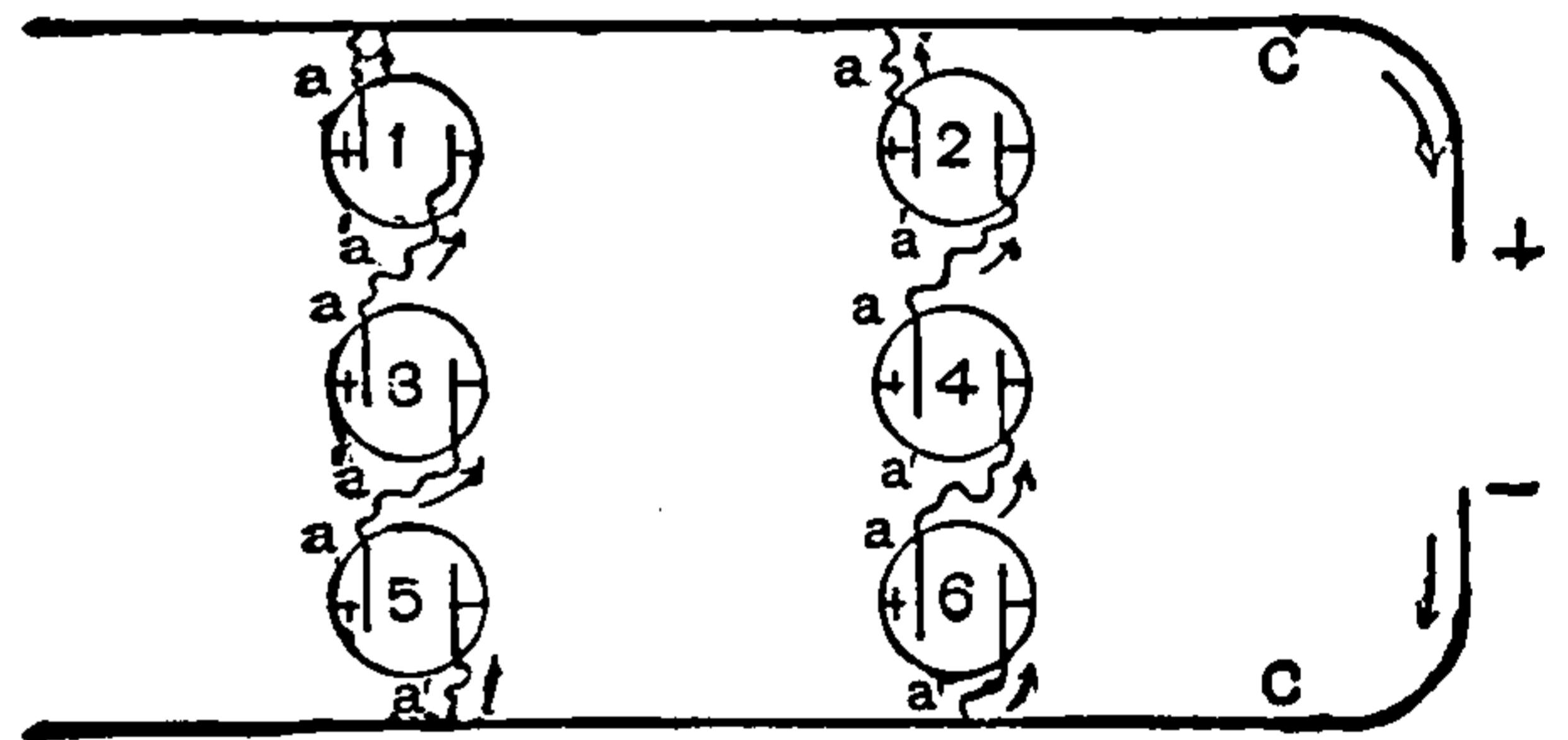
Fig. 131. Cells Connected in Multiple-Series.
