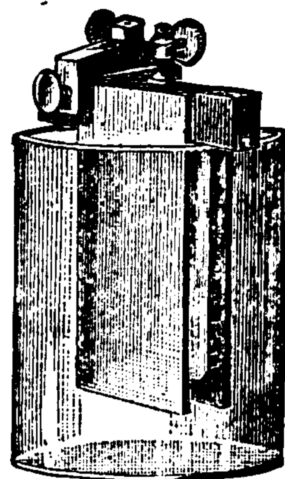
Fig. 114. Smee Cell.
