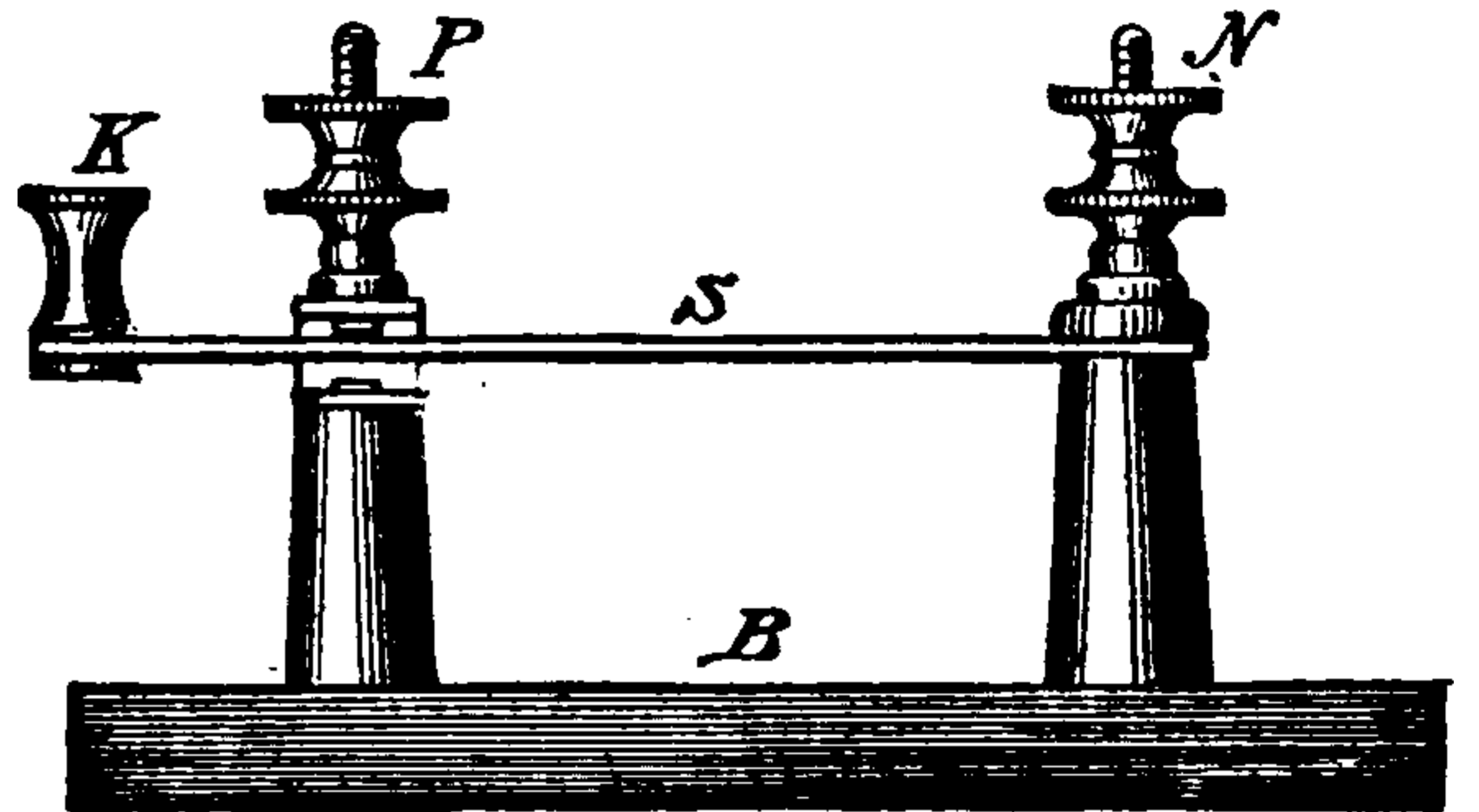
Fig. 329. Short-Circuit Key.
