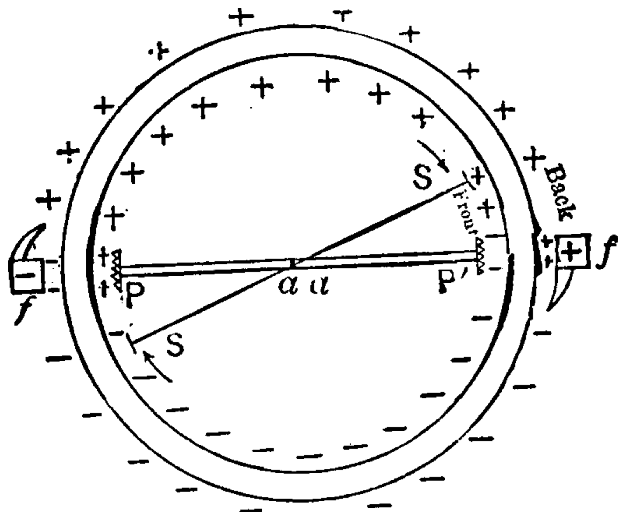
Fig. 359. Plate of Holtz Machine.
