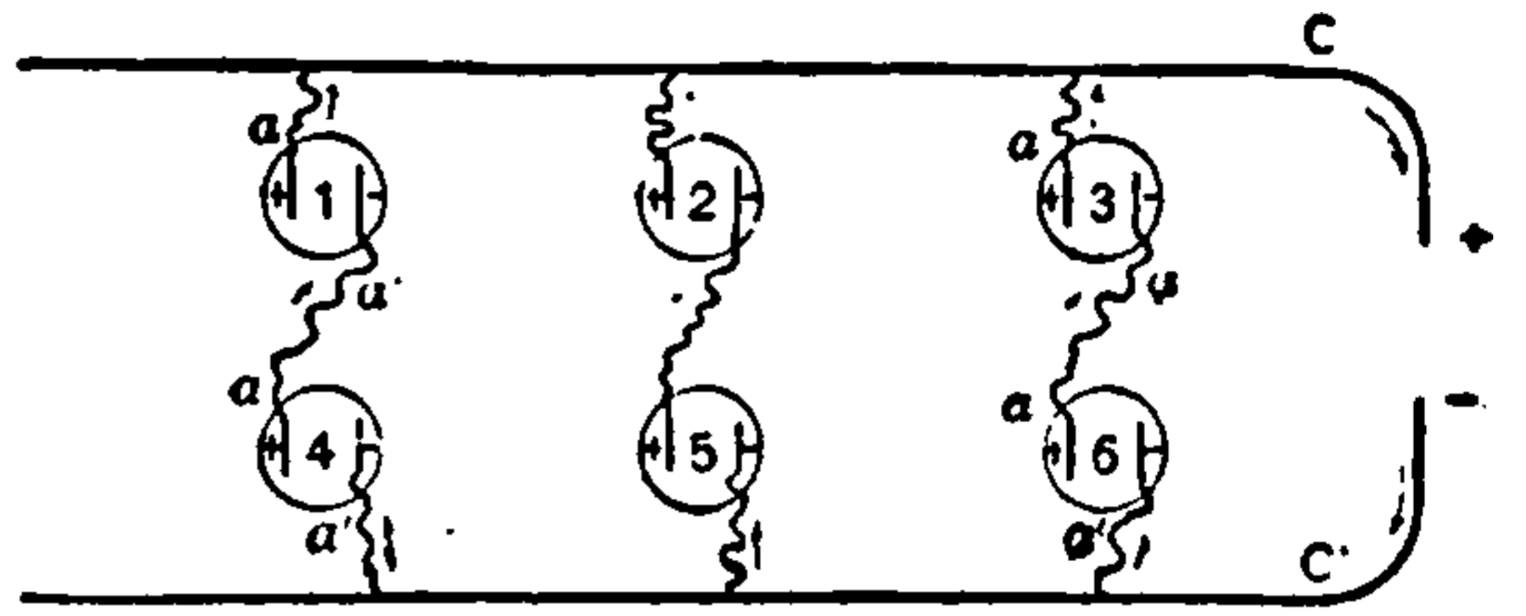
Fig. 130. Multiple-Series-Connected Cells.
