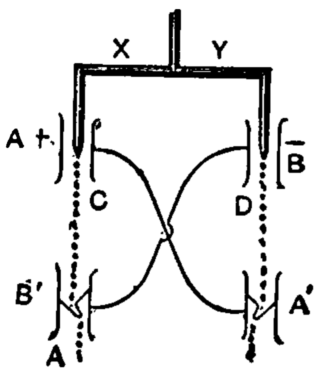
Fig. 3. Water-Dropping Accumulator.
