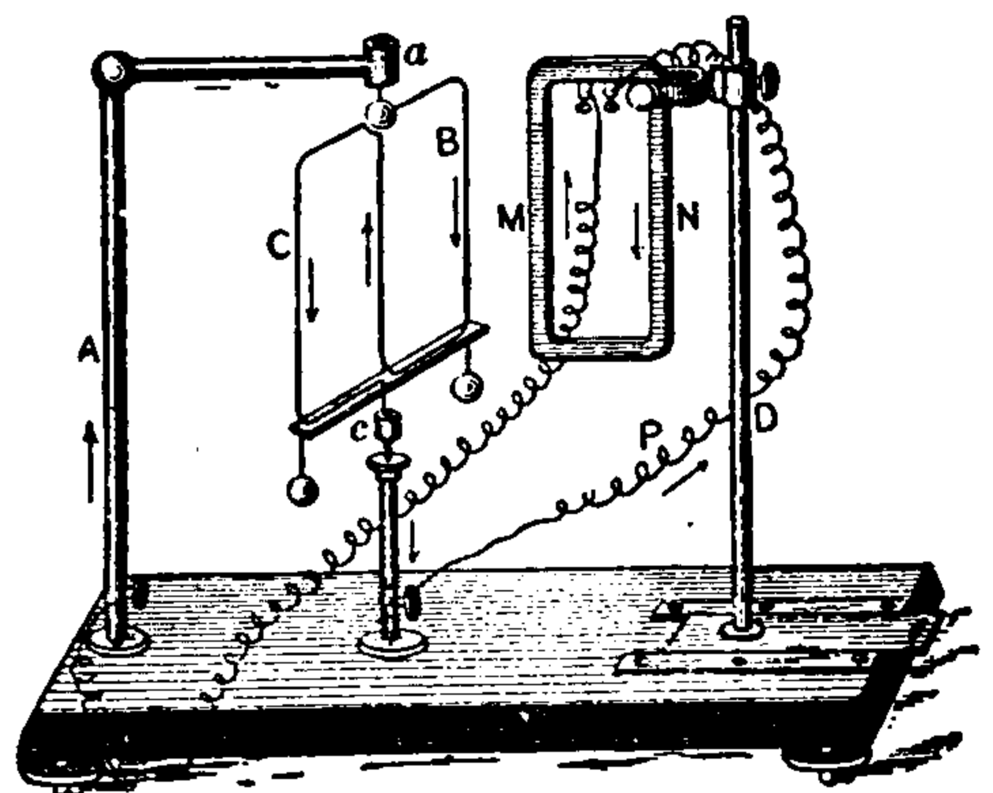
Fig. 219. Ampère's Stand.
