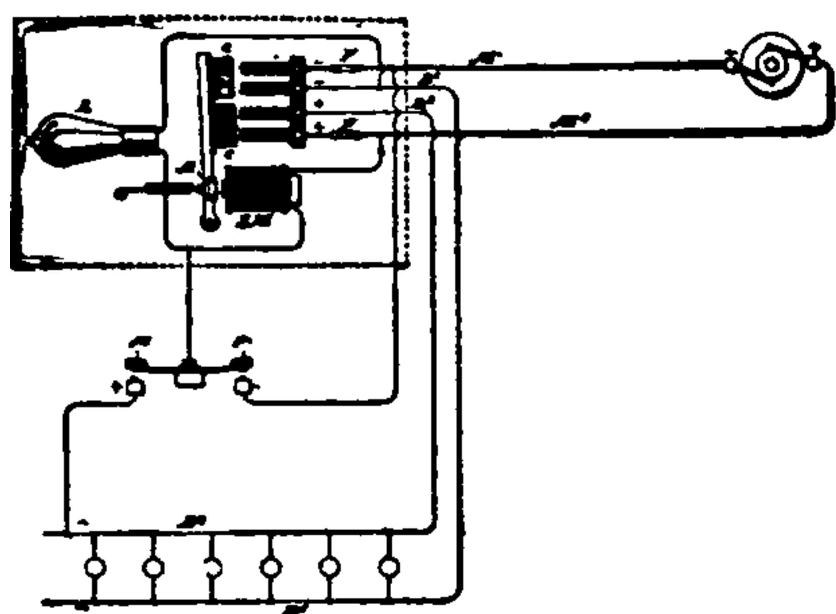
Fig. 520. Automatic Switch.
