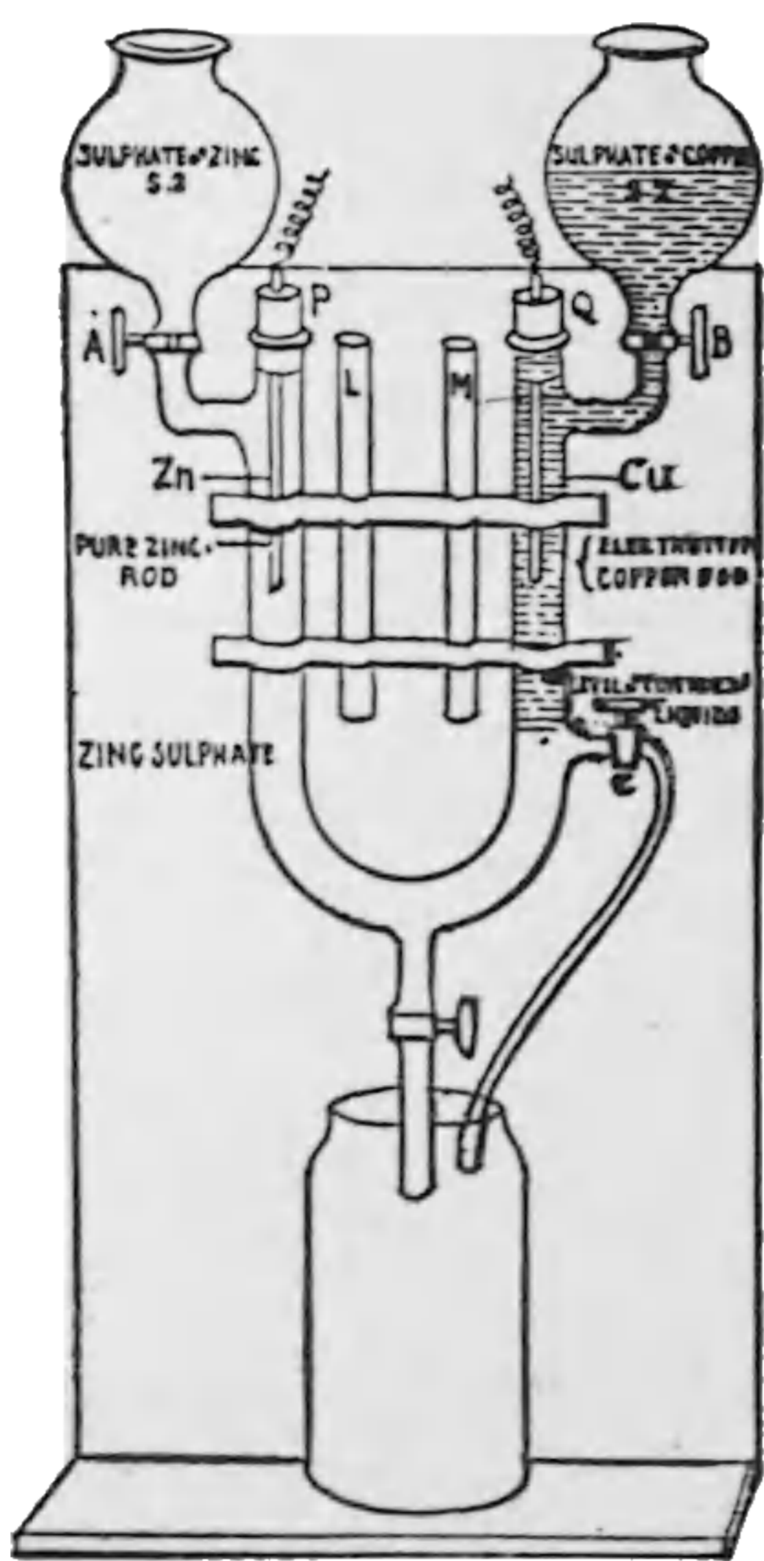
Fig. 117. Fleming's Standard Cell.
