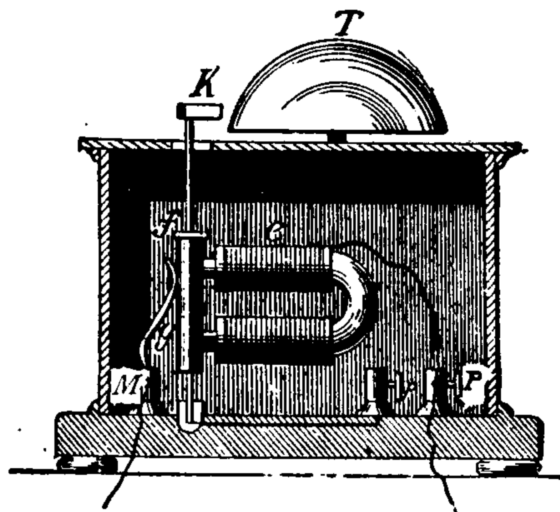
Fig. 8. Automatic Make-and-Break.
