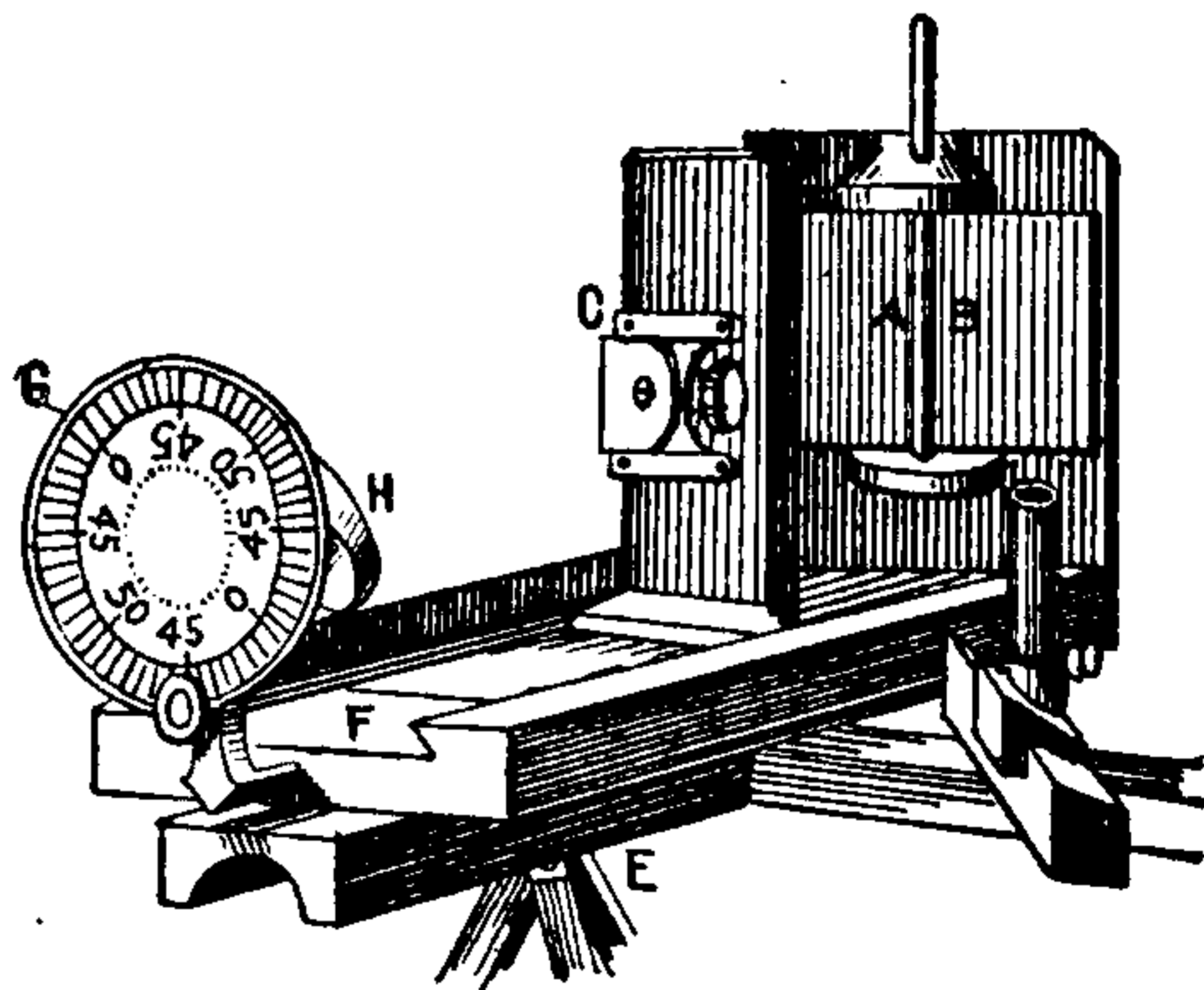
Fig. 429. Ayrton and Perry's Dispersion Photometer.
