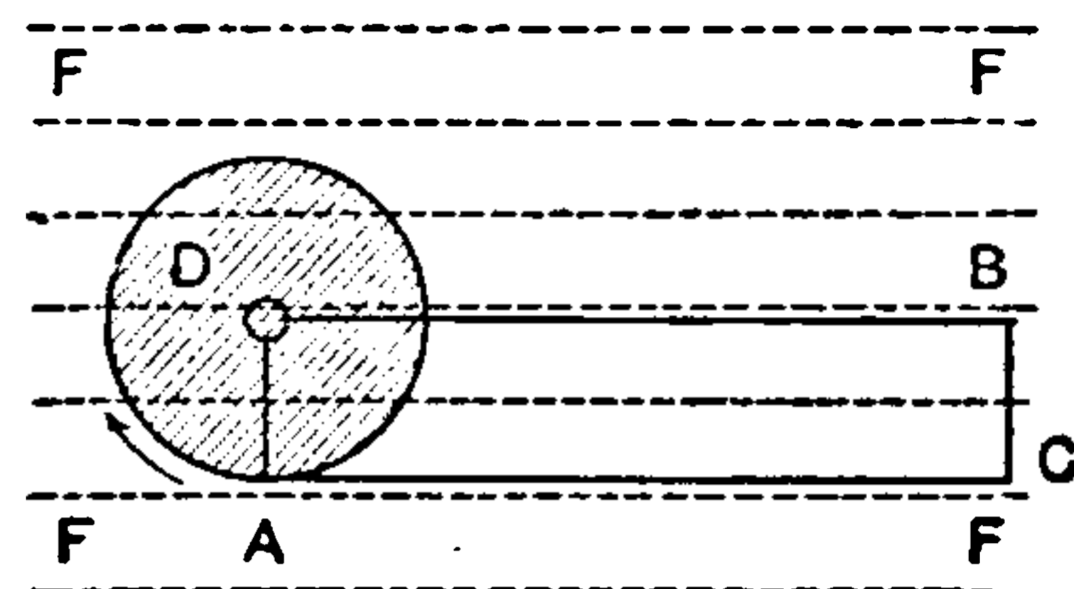
Fig. 2. Barlow's Wheel.
