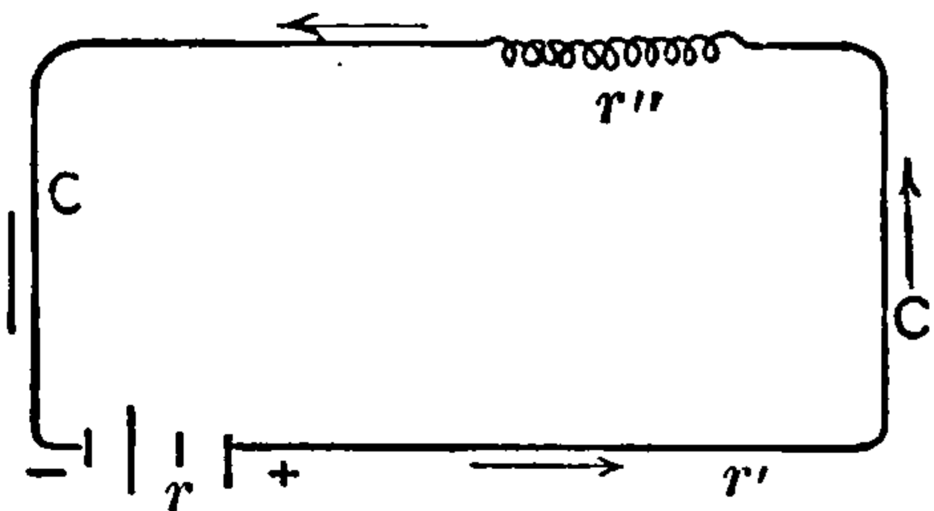
Fig. 341. Current Strength in Circuit.
