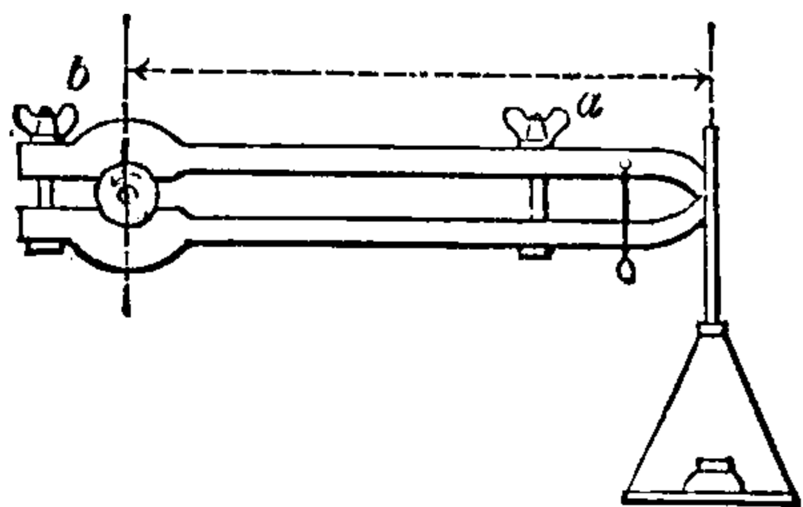
Fig. 71. Prony Brake.
