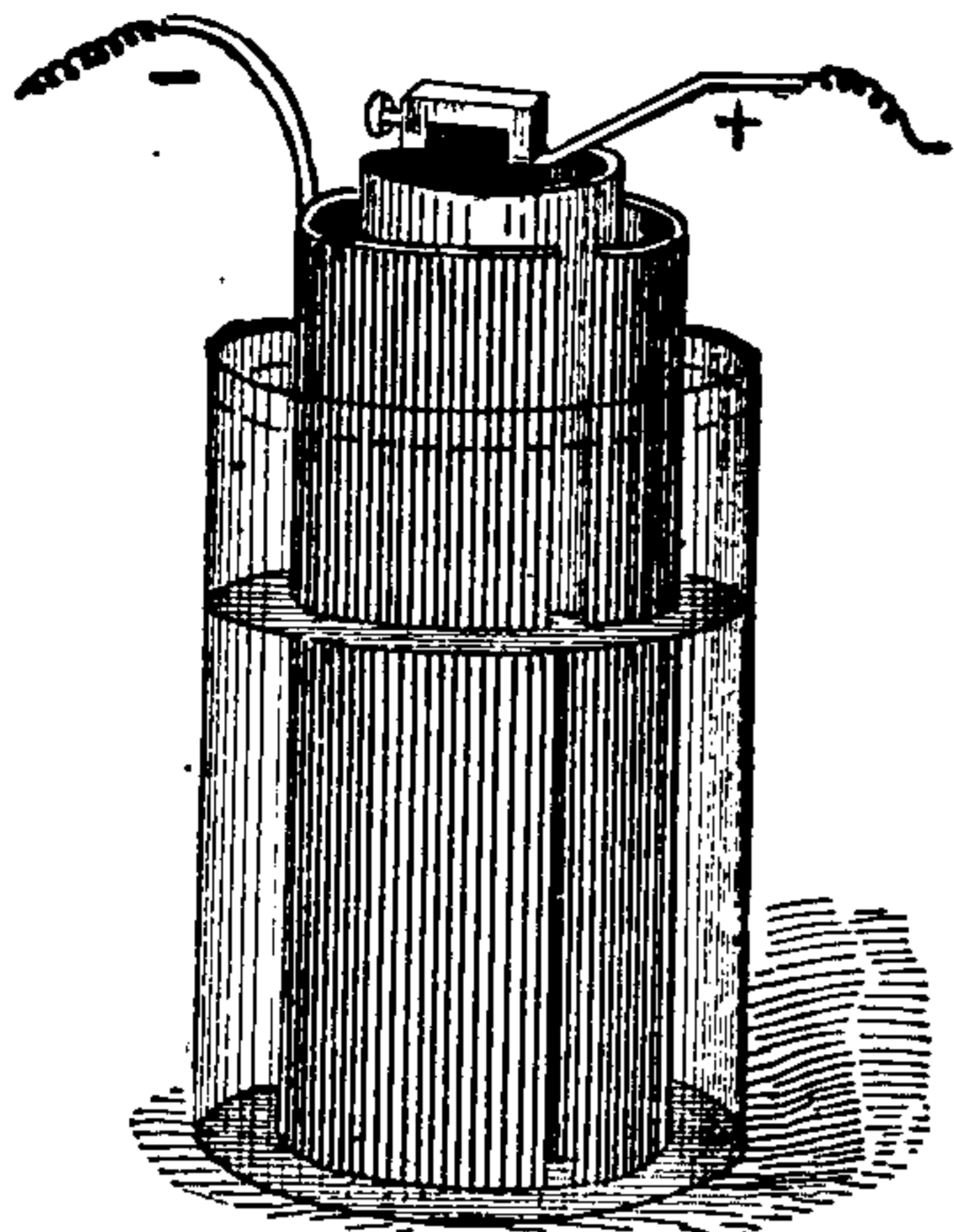
Fig. 105. Bunsen Cell.
