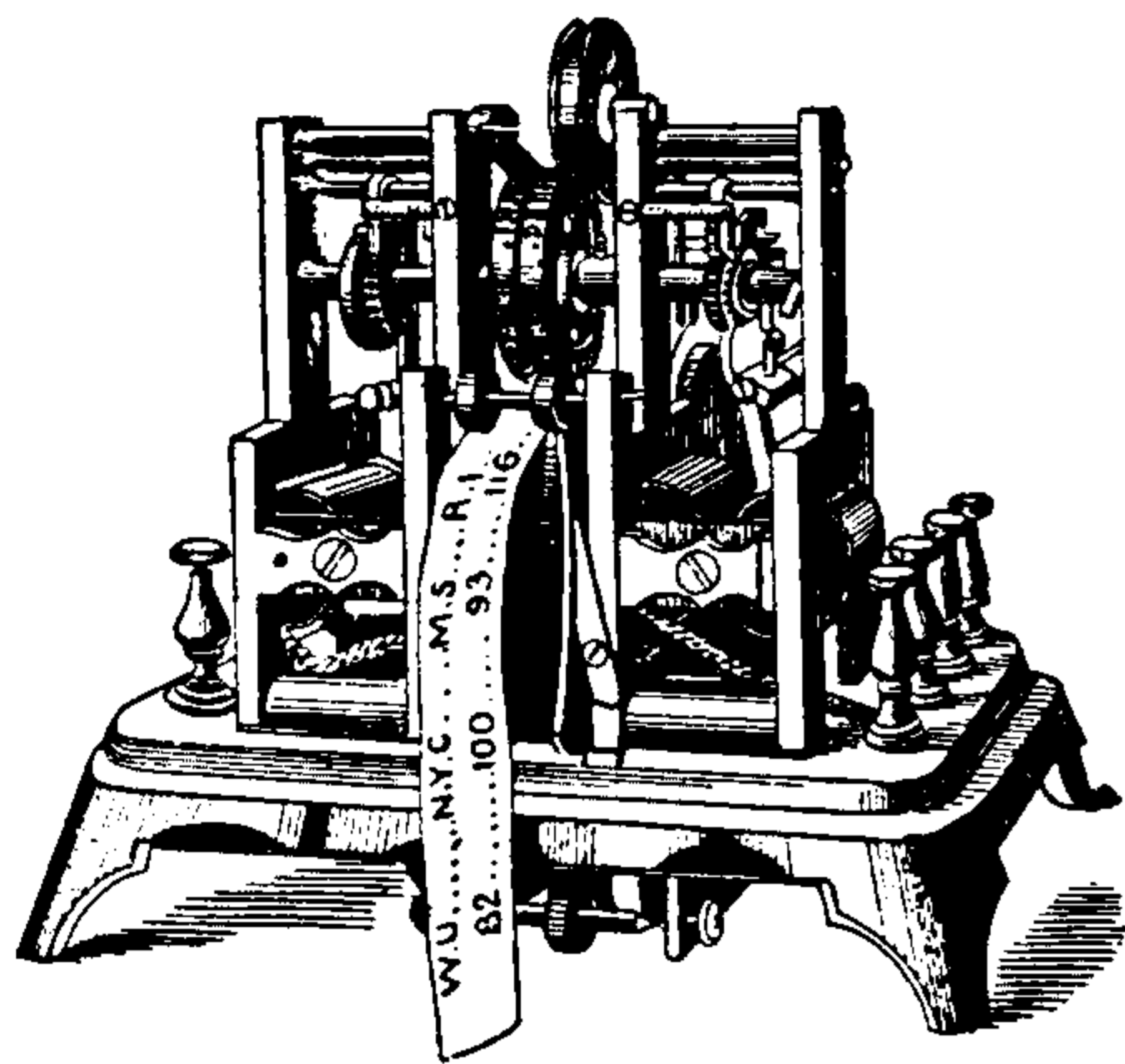
Fig. 532. Callahan's Printing Telegraph.
