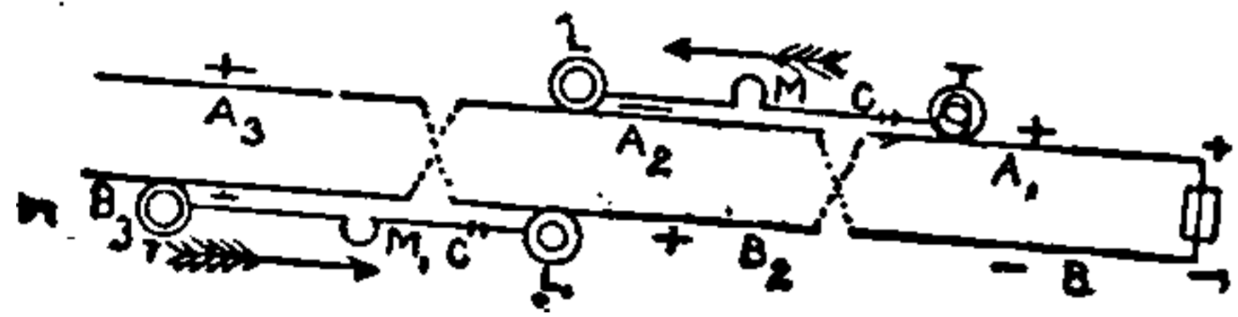
Fig. 554. Circuit for Telpherage System.
