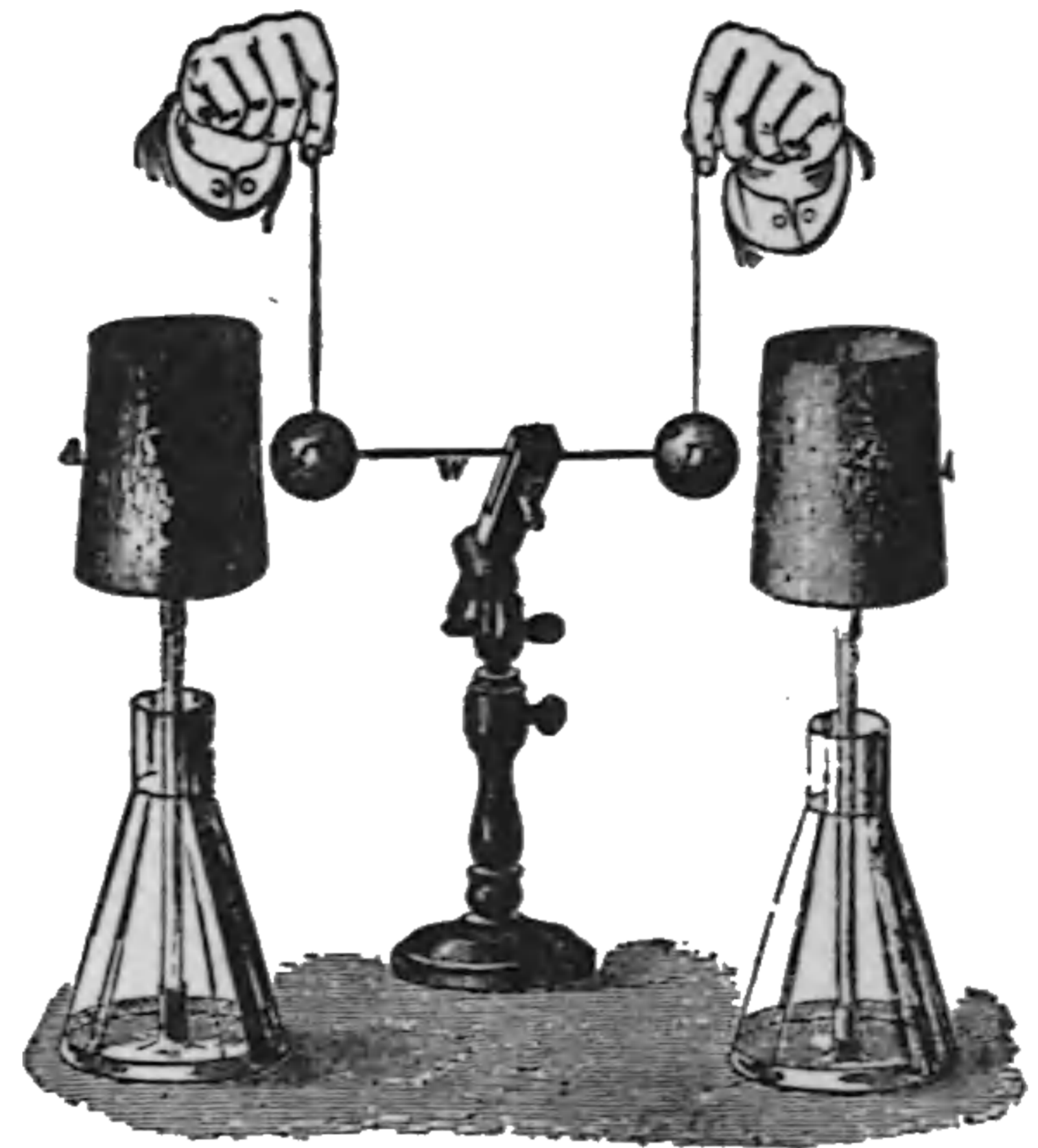
Fig. 487. Action of Replenisher.
