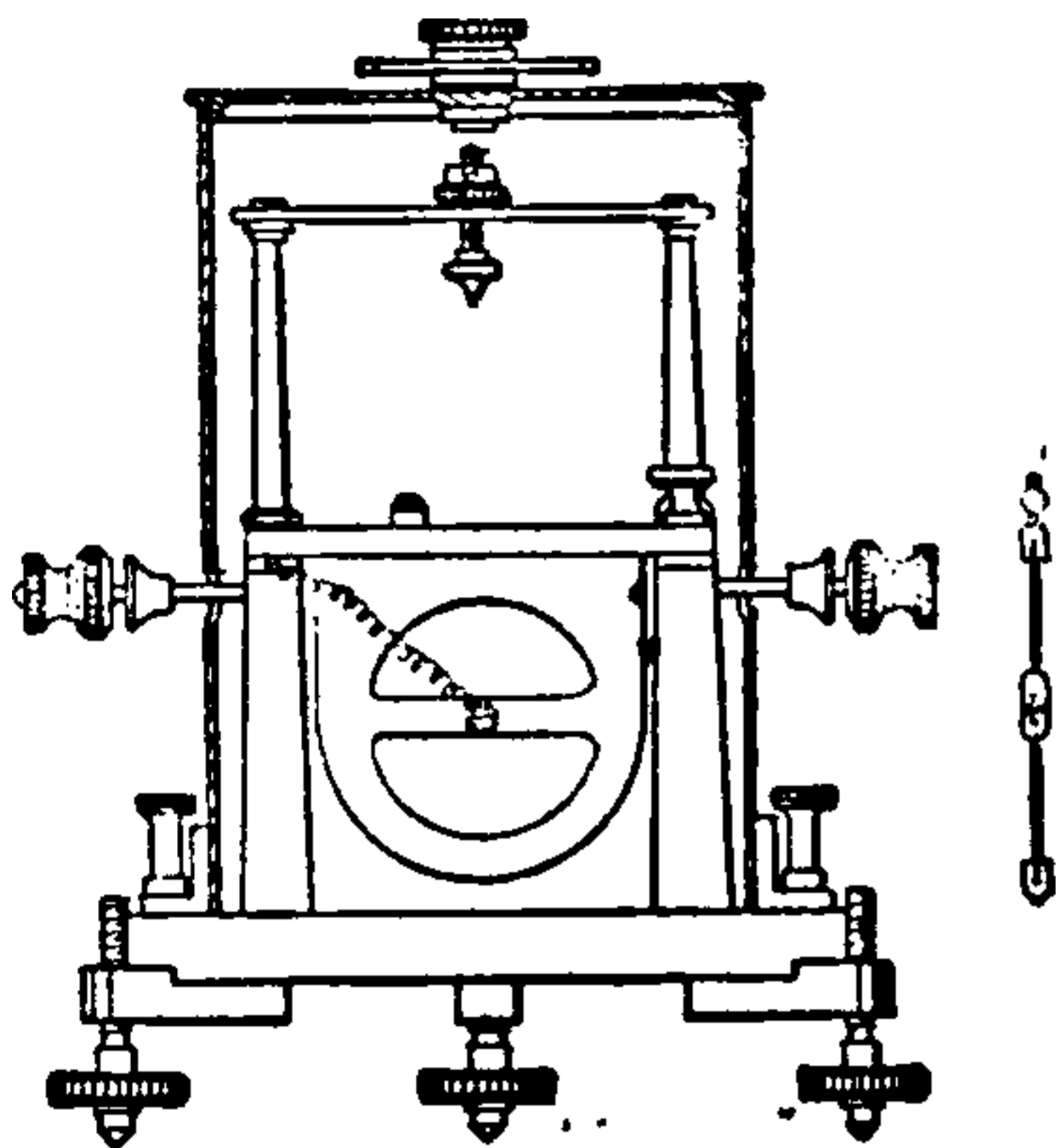
Fig. 270. Nalder's Galvanometer.
