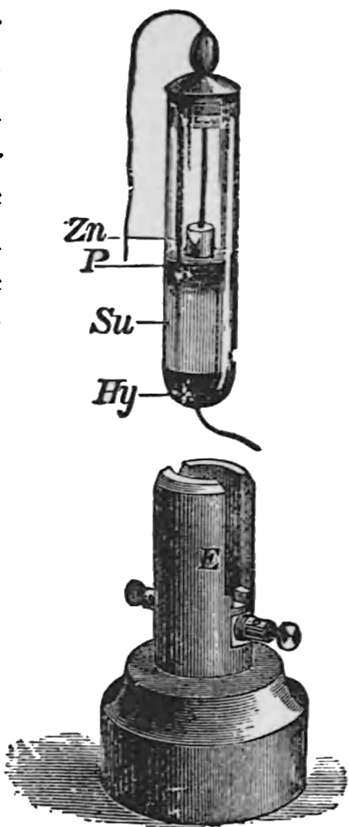
Fig. 116. Rayleigh's Form of Clark's Standard Cell.
