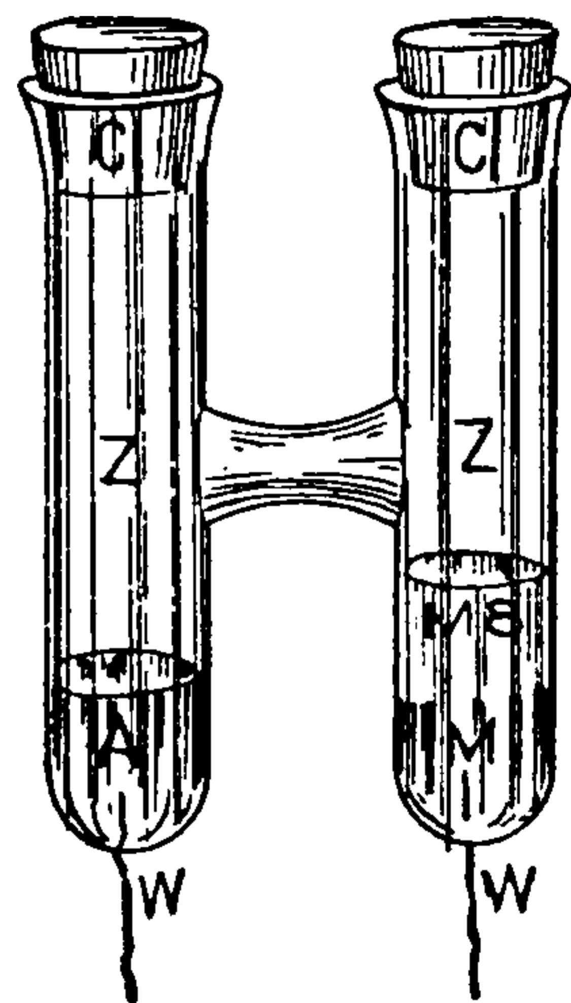
Fig. 115. Clark's Standard Cell.
