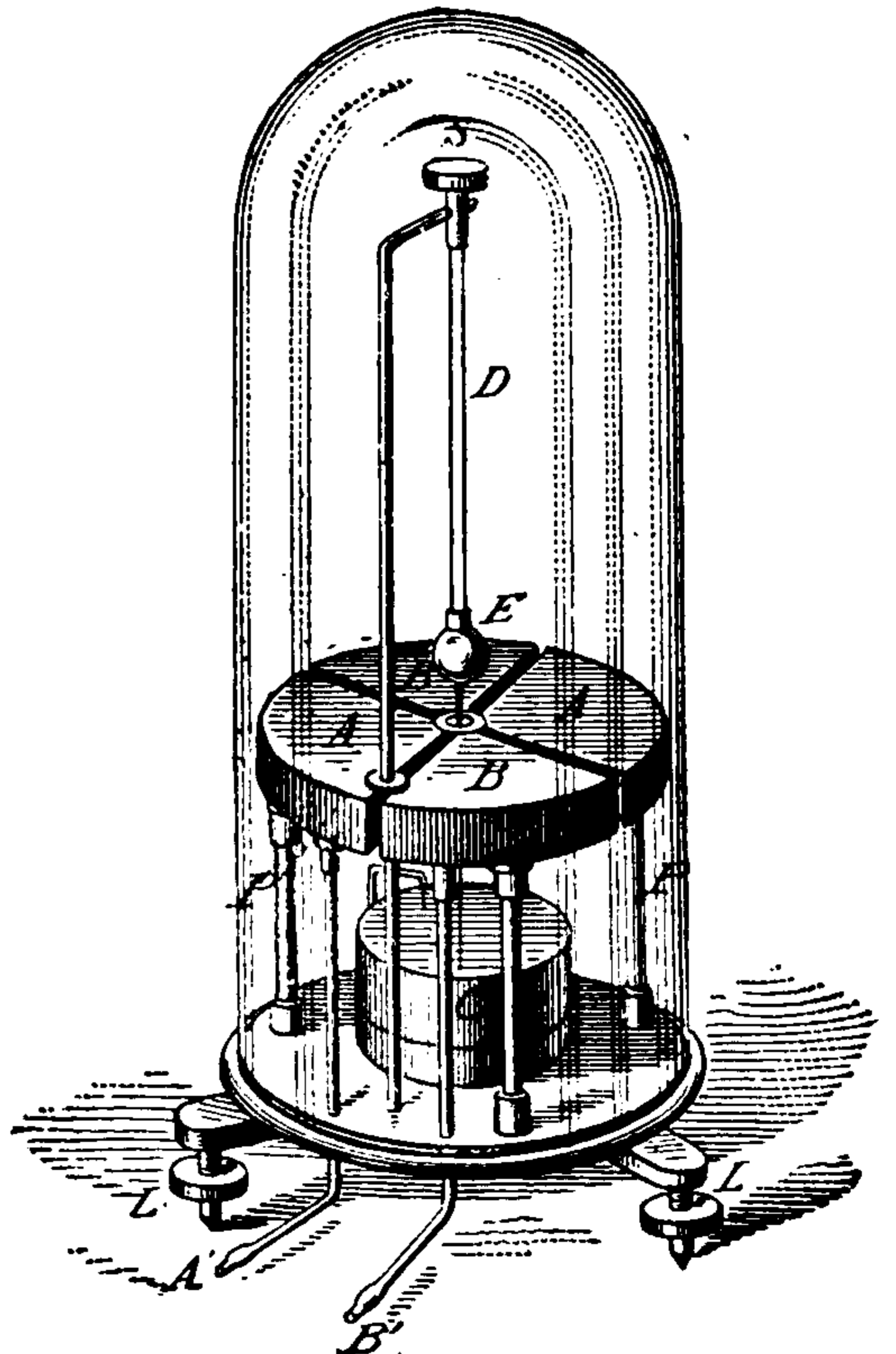
Fig. 234. Quadrant Electrometer.
