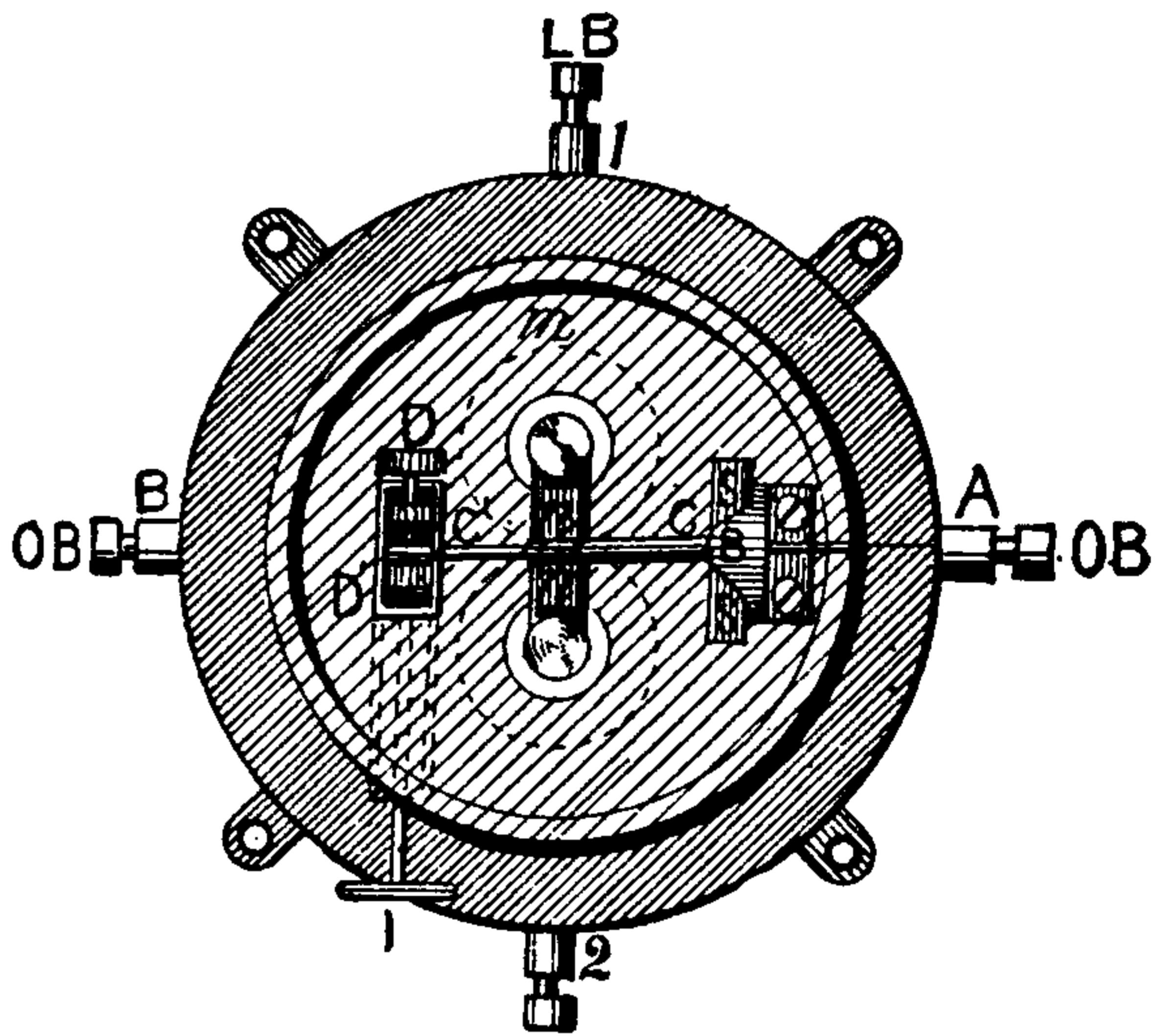
Fig. 483. A Detail of the Polarized Relay.
