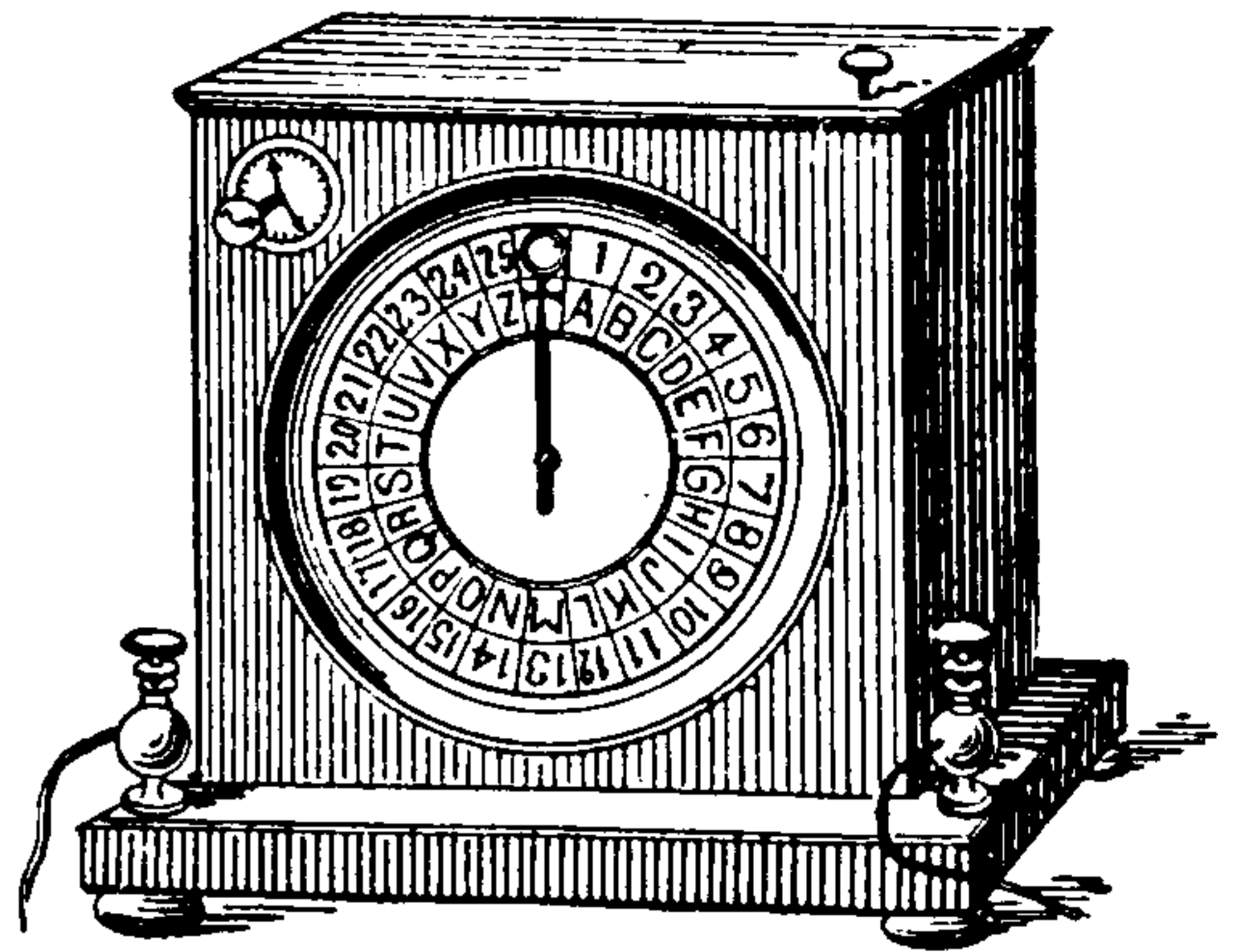
Fig. 541. Breguet's Indicator.
