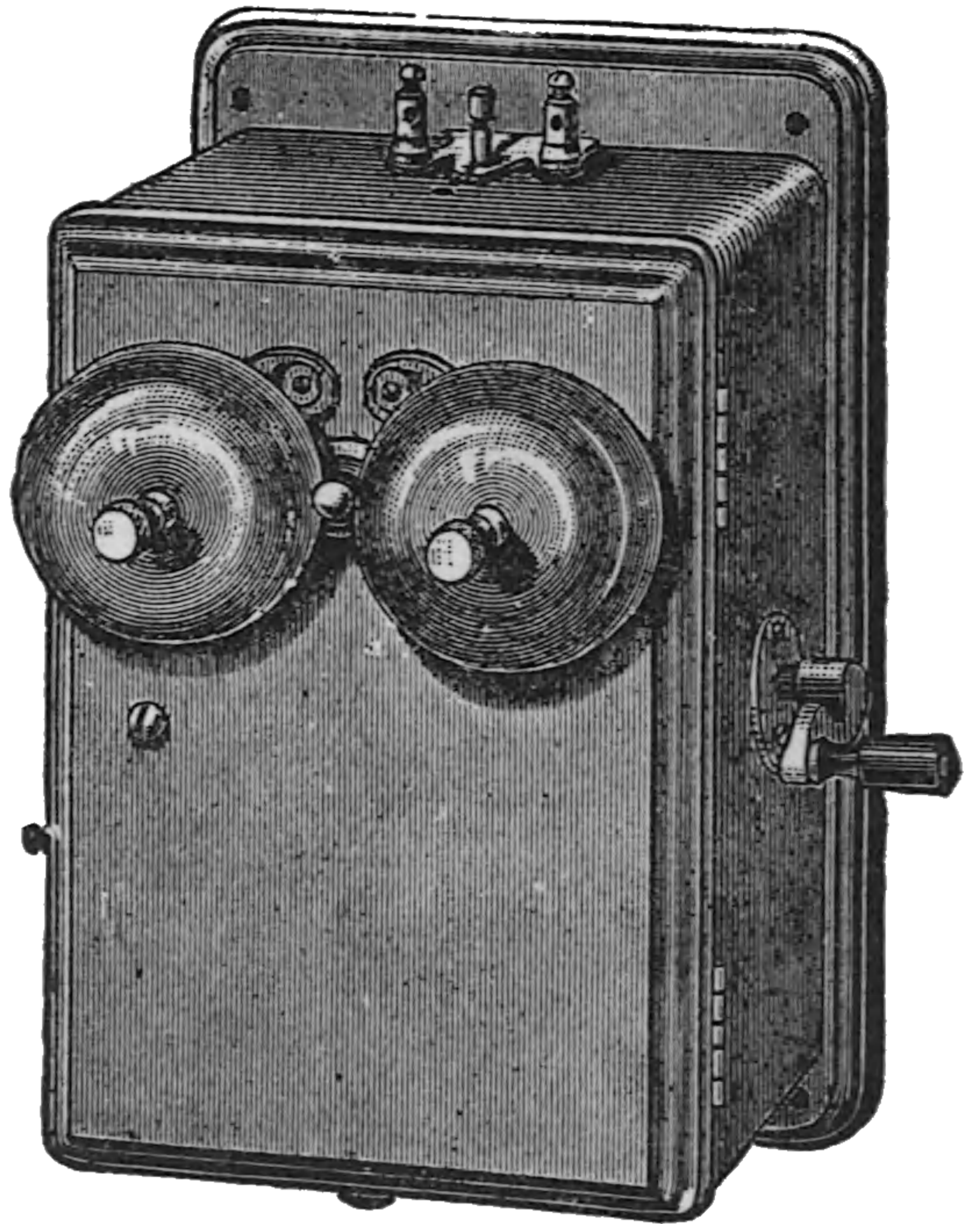
Fig. 96. Magneto Call Bell.
