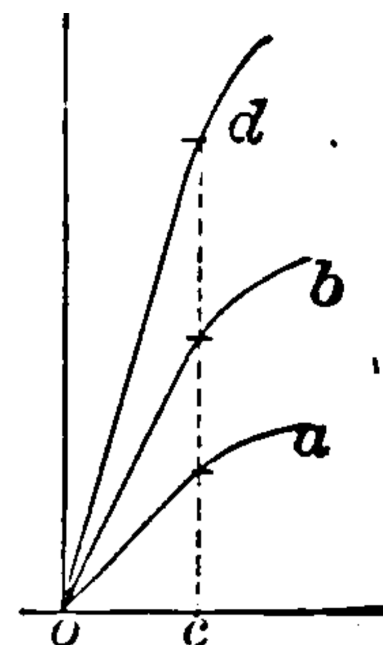
Fig 178. Critical Curve of Dynamo Current
