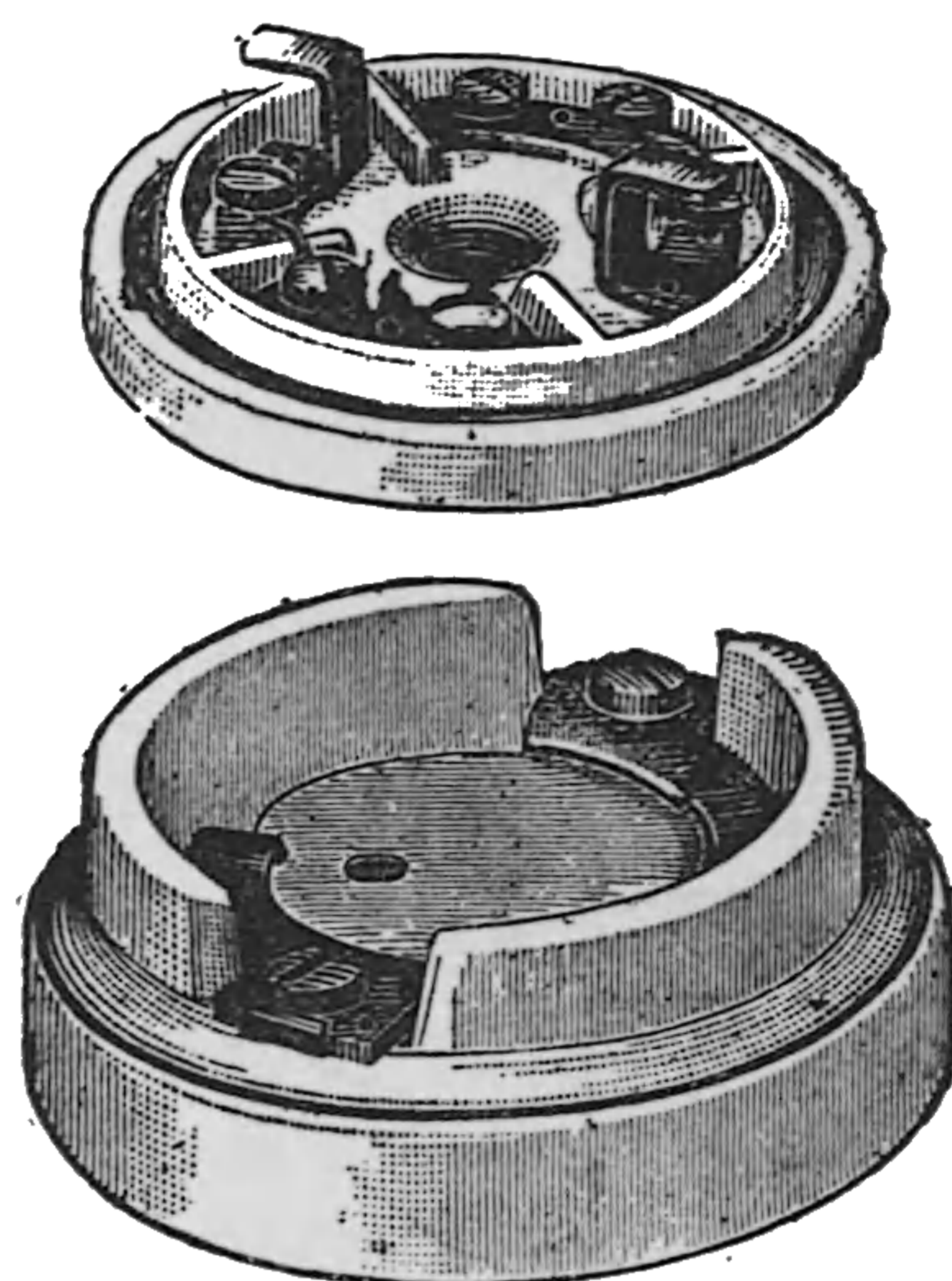
Fig. 192. Ceiling Cut-Out.
