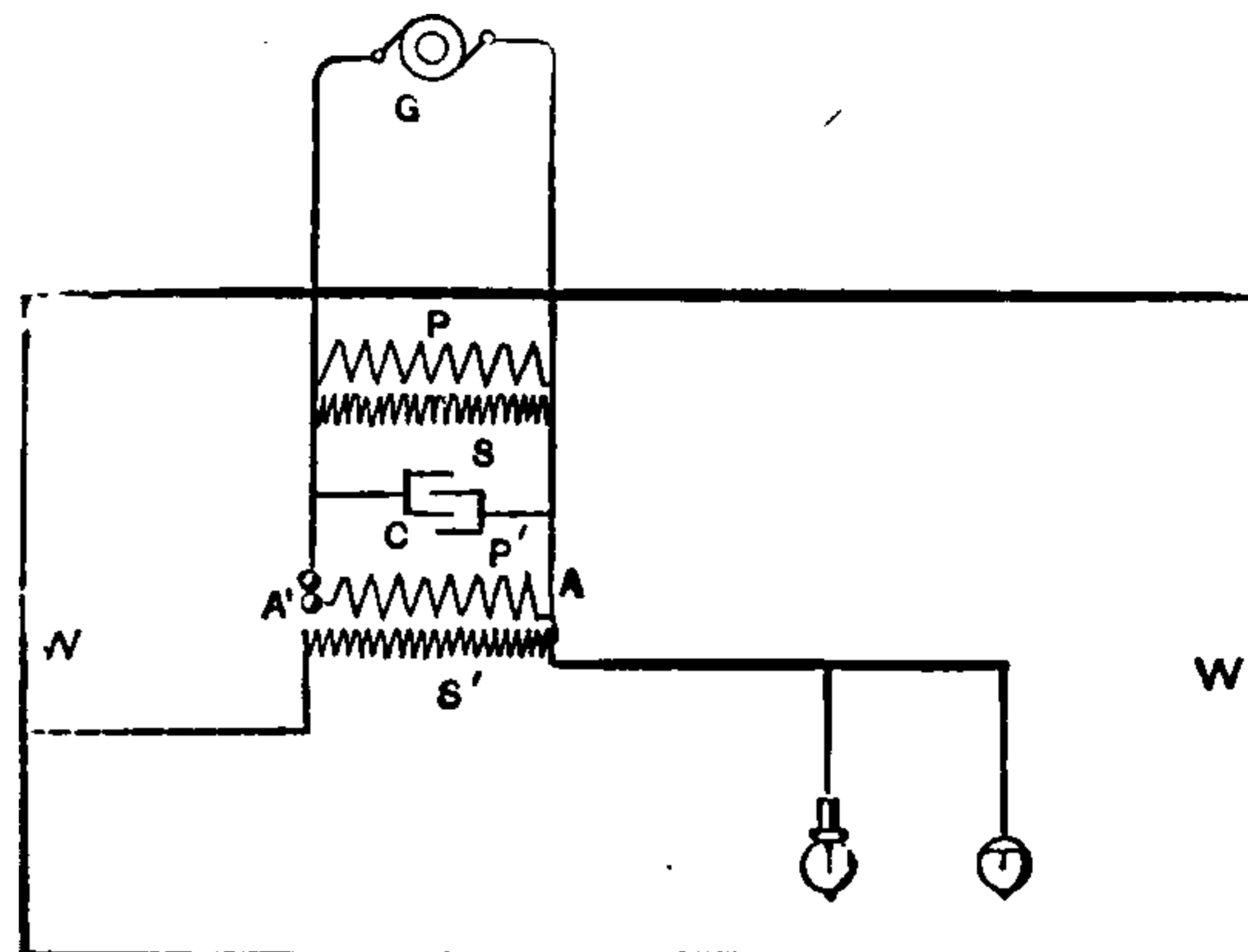
Fig. 346. Tesla's High Frequency Currents System of Lighting.
