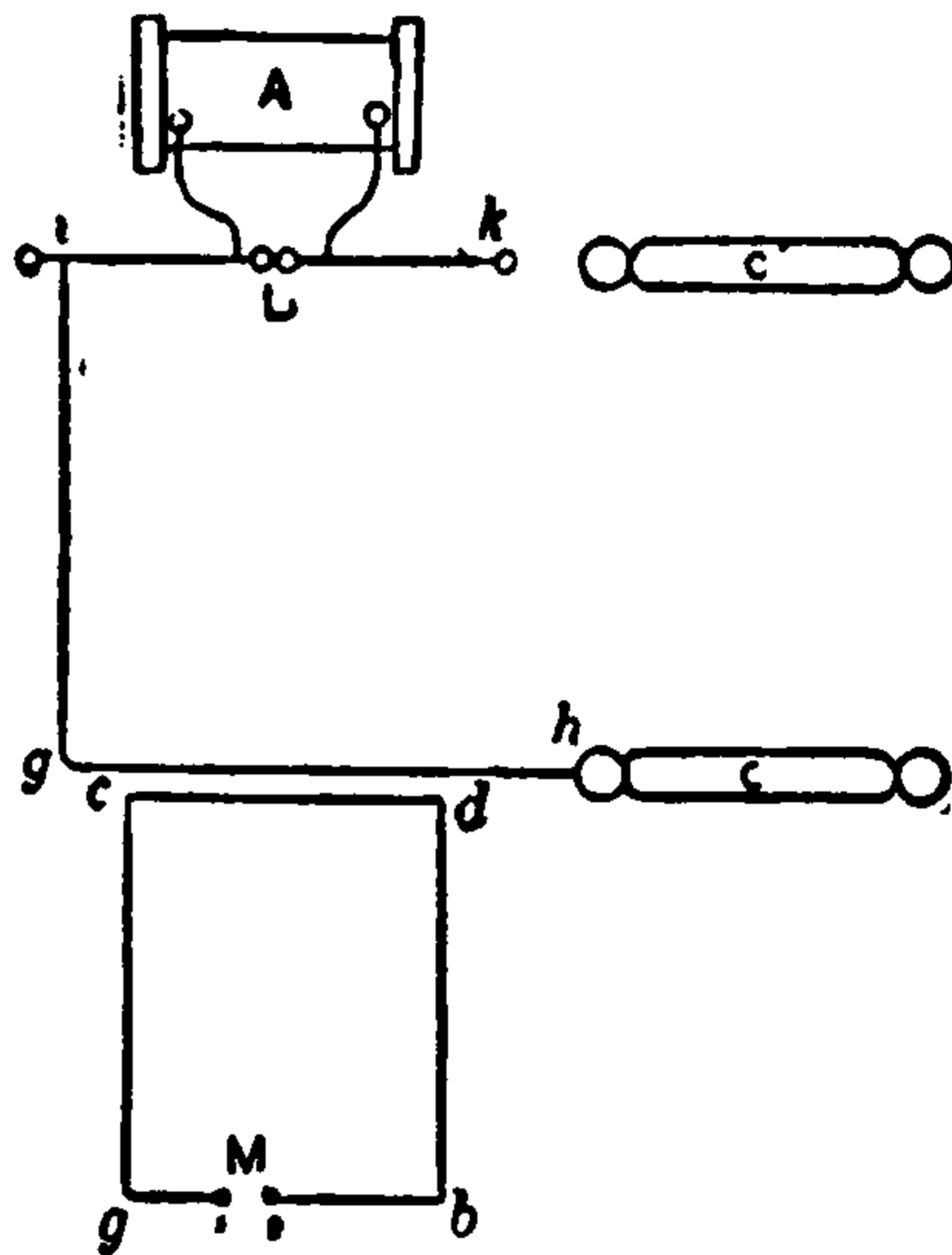
Fig. 493. Electric Resonance.
