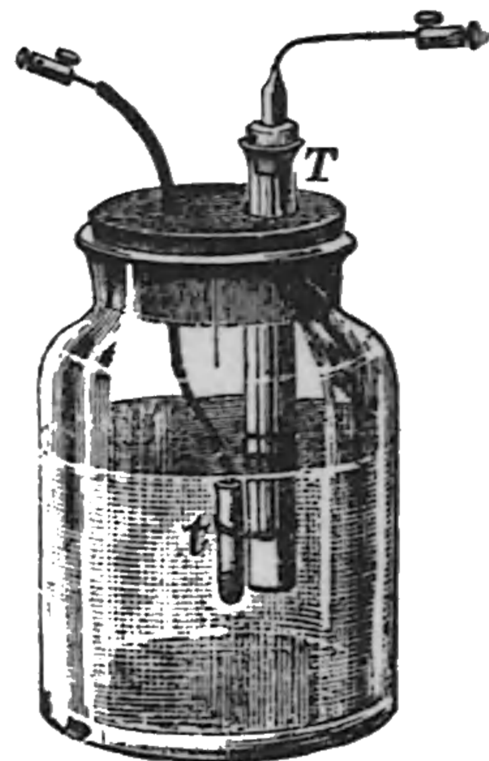
Fig. 118. Lodge's Form of Daniell's Cell.
