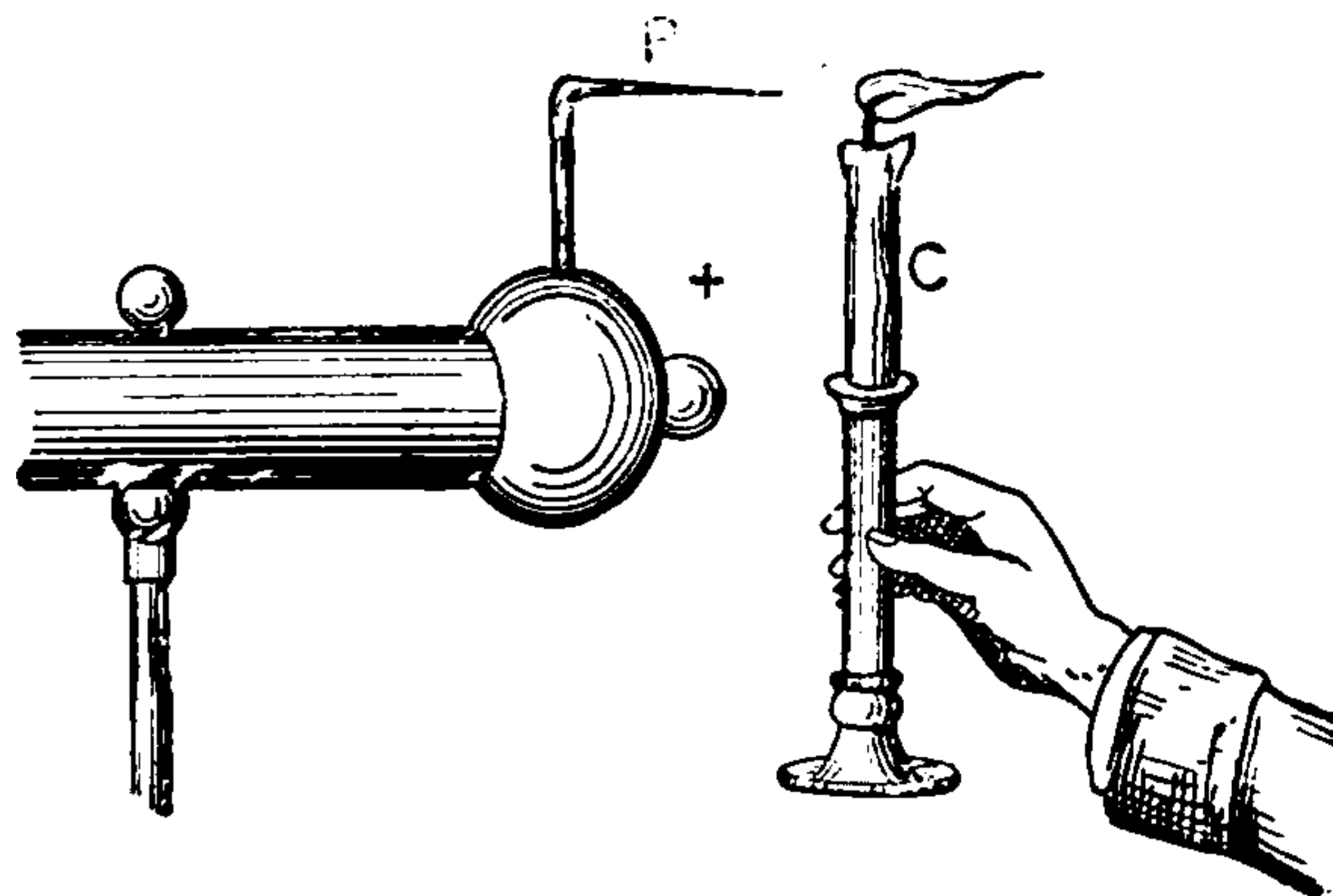
Fig. 50. Convection Blow-Pipe.
