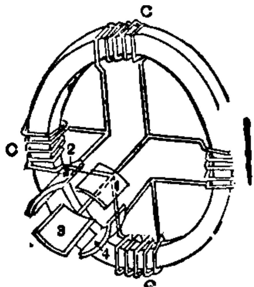
Fig. 159. Four-part Commutator.
