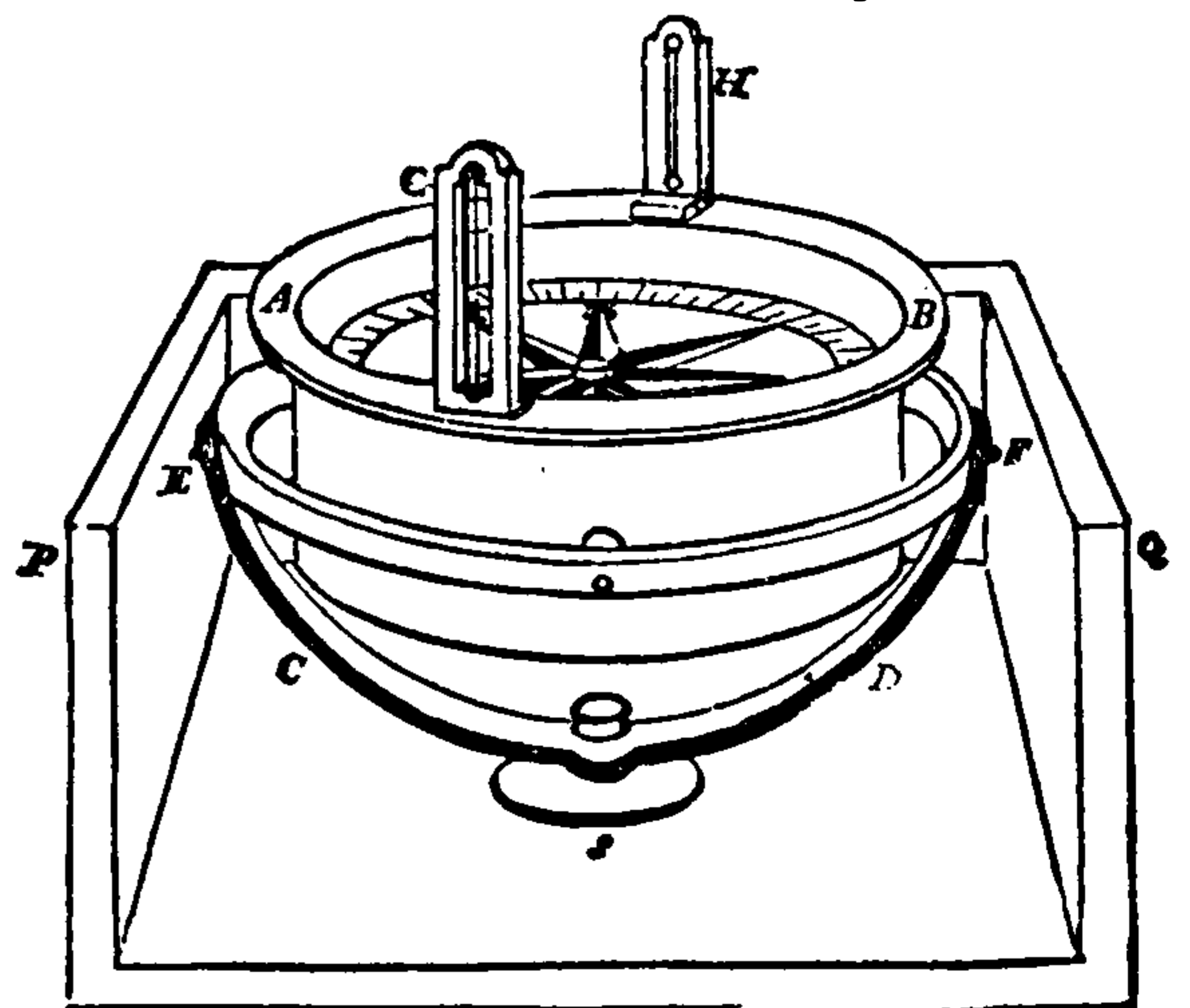
Fig. 161. Azimuth Compass.
