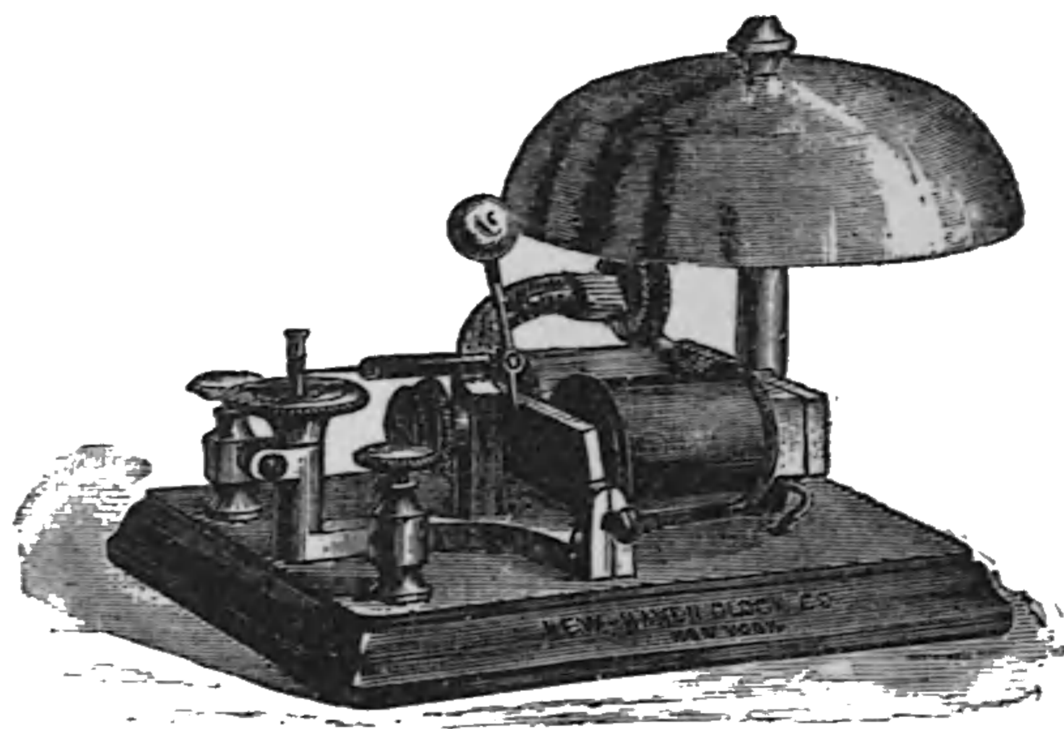
Fig. 47. Single-Stroke Bell.
