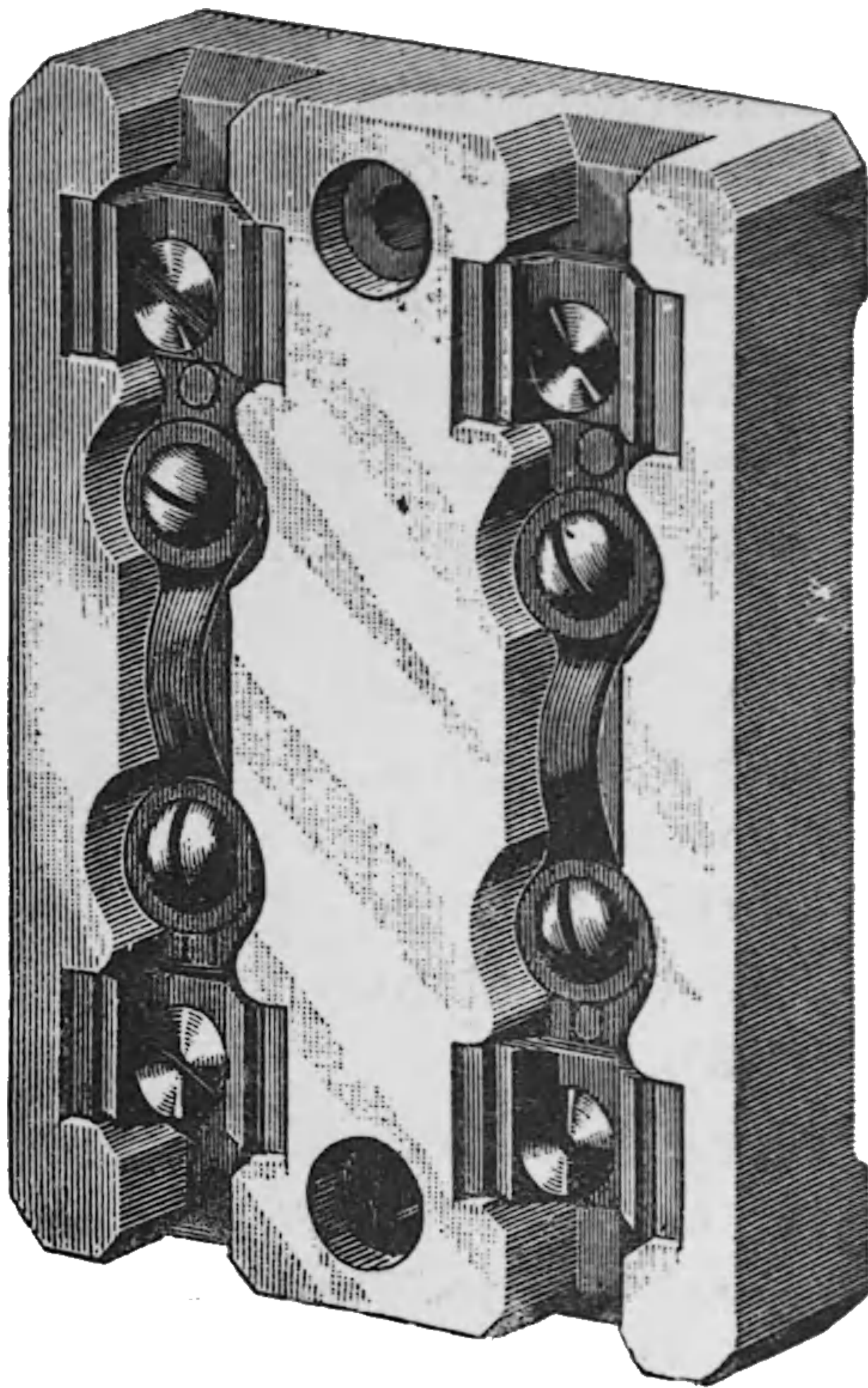
Fig. 194. Main-Line Cut-Out.
