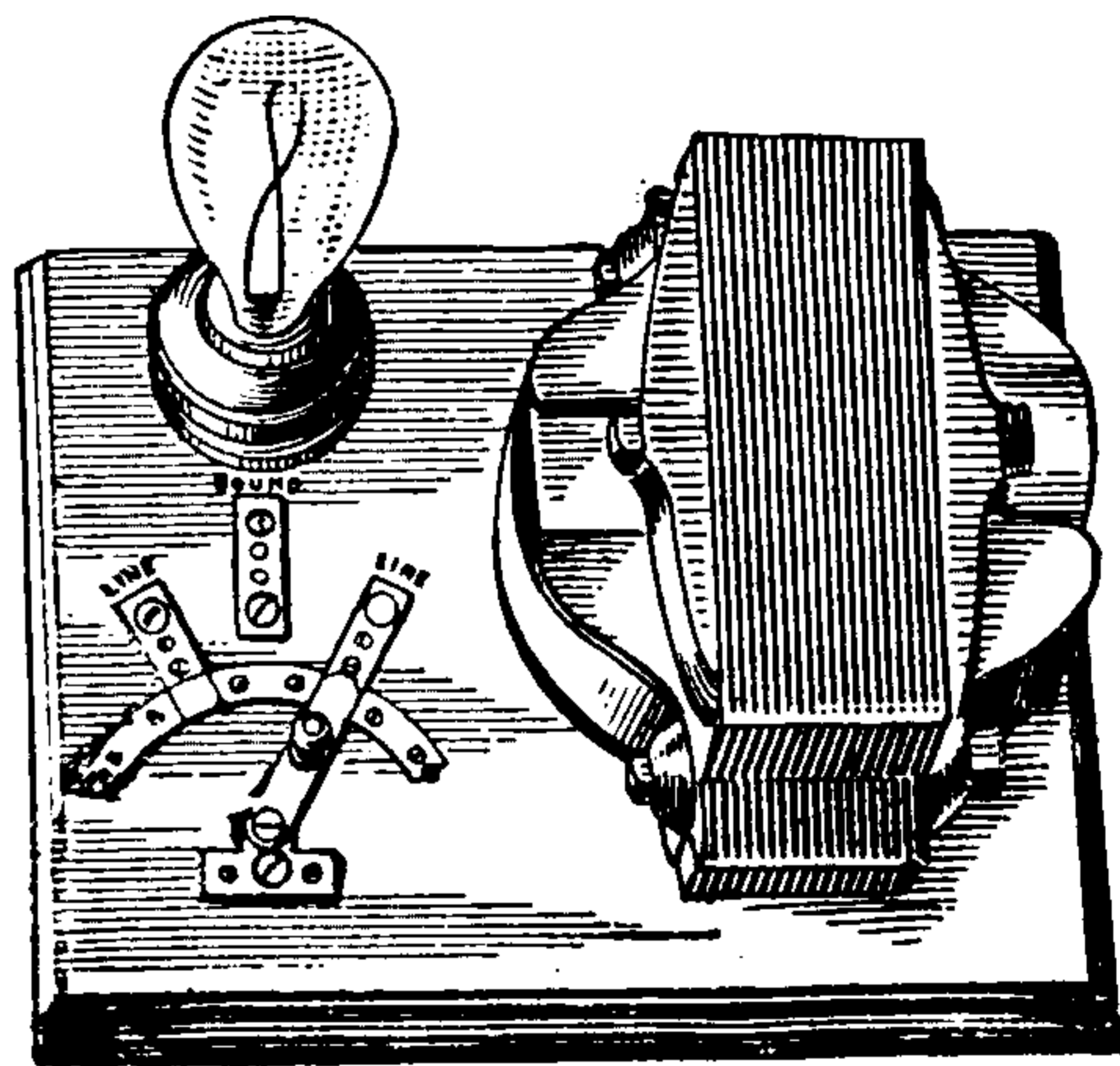
Fig. 196. Ground-Detector .
