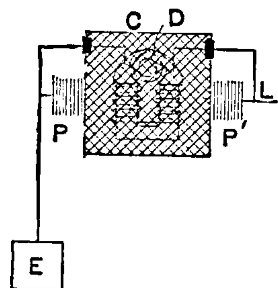
Fig. 27. Counter-Electromotive Force Lightning Arrester.
