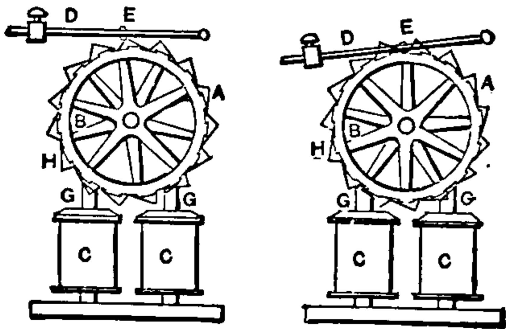
Fig. 140. Spellier's Electric Clock.
