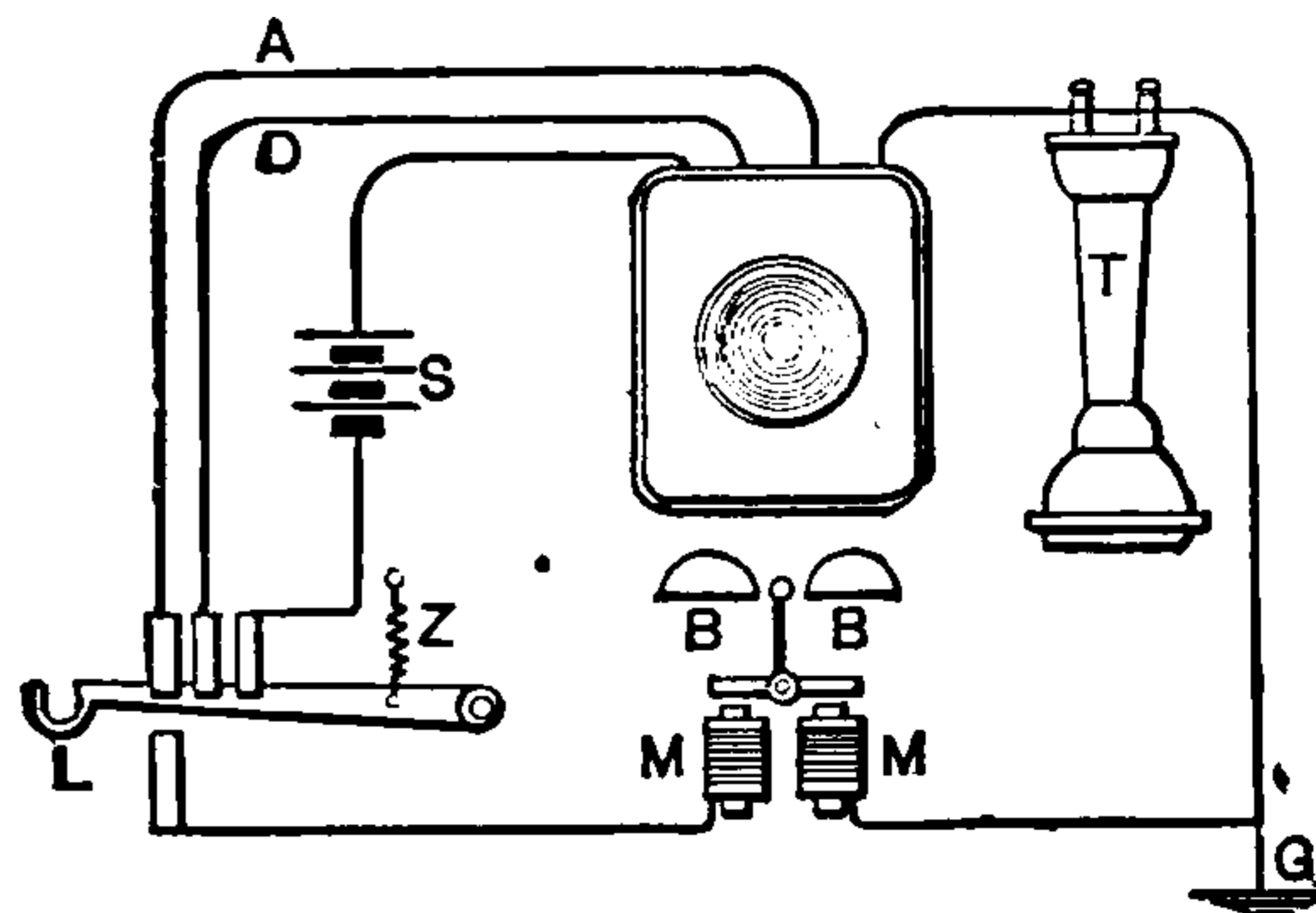
Fig. 525. Automatic Telephone Switch.
