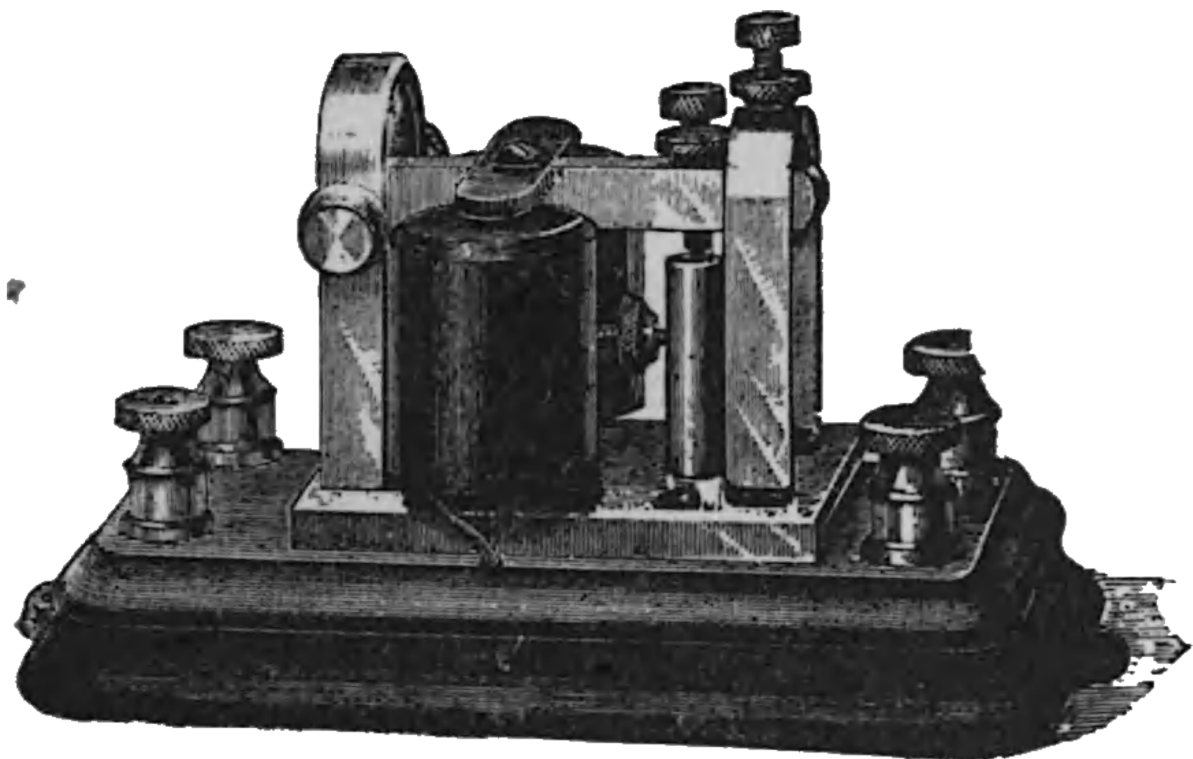
Fig. 511. Telegraphic Sounder.
