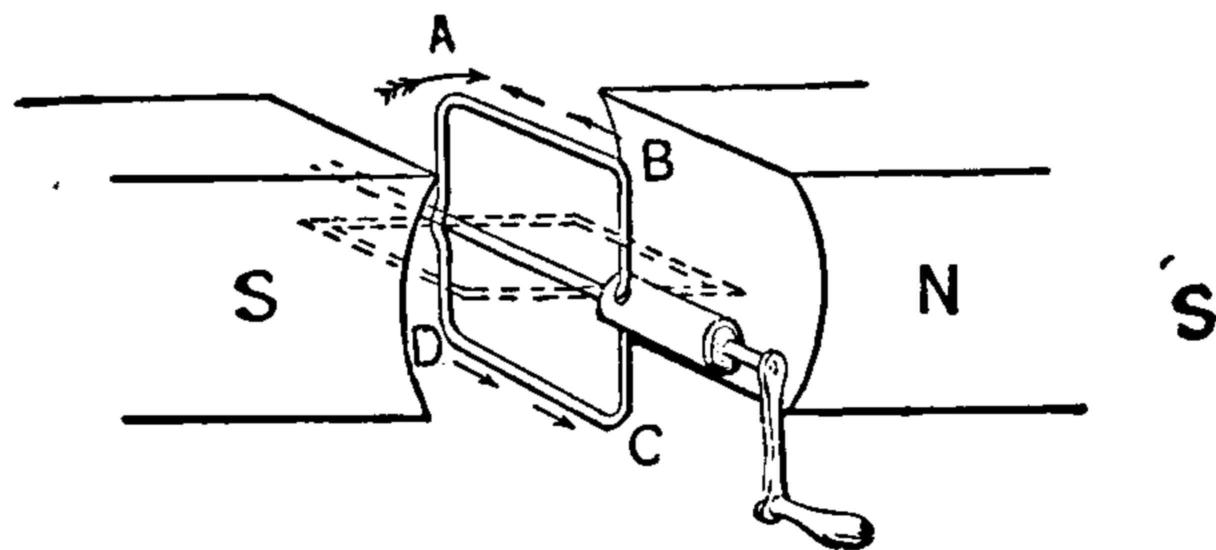
Fig. 179. Induction in Armature Loop.
