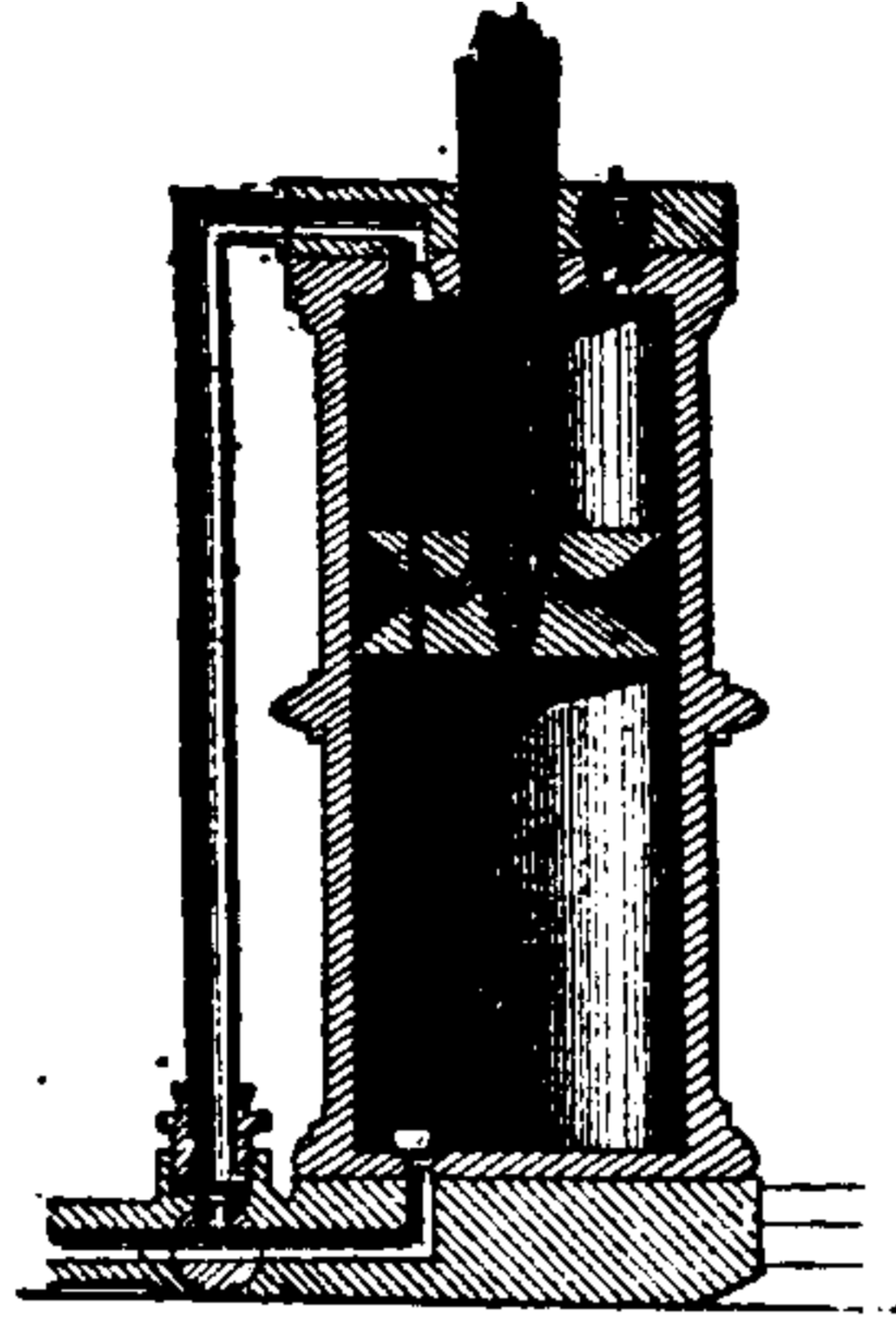
Fig. 455. Barrel of Bianchi's Air Pump.
