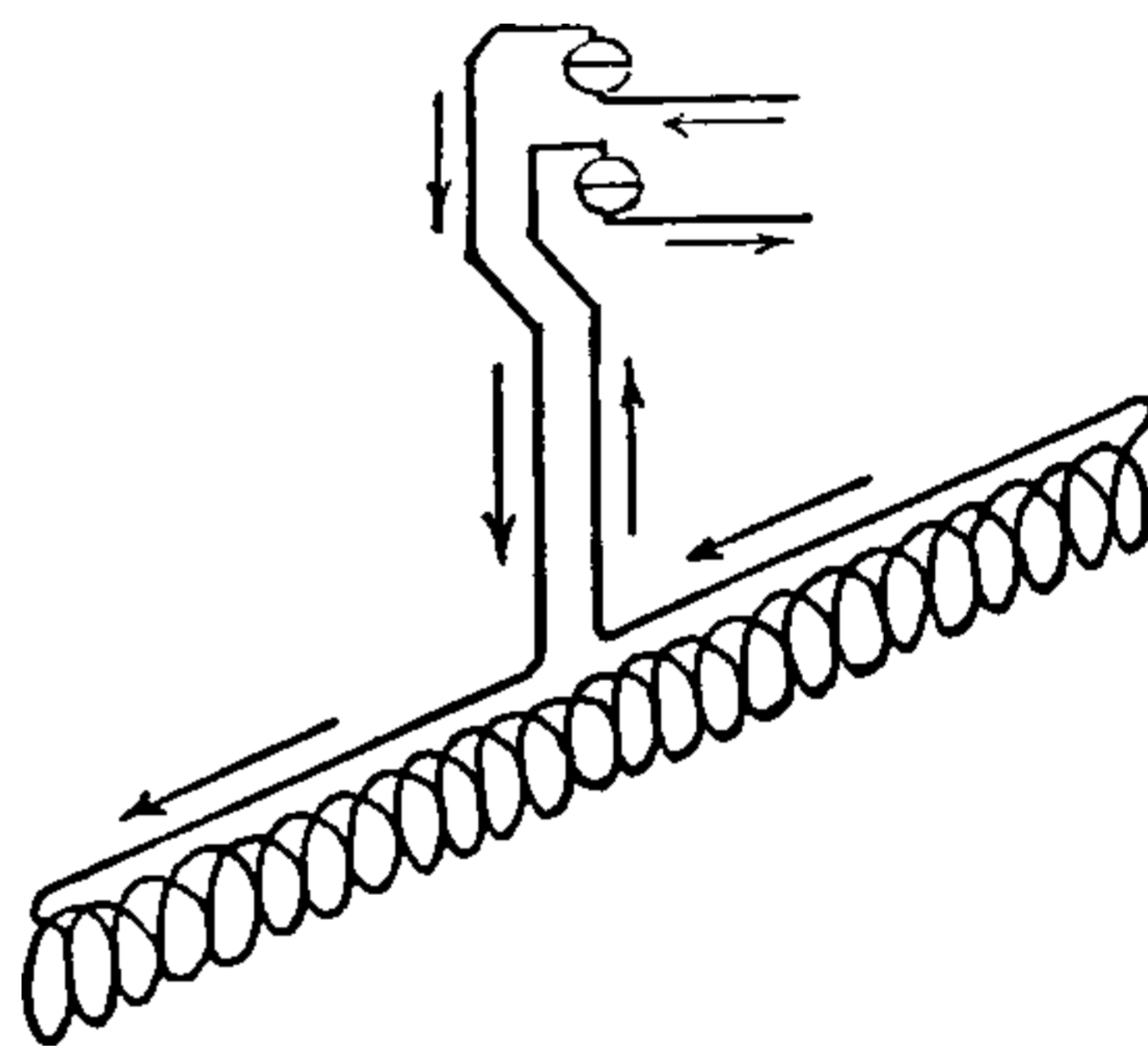
Fig. 506. Practical Solenoid.
