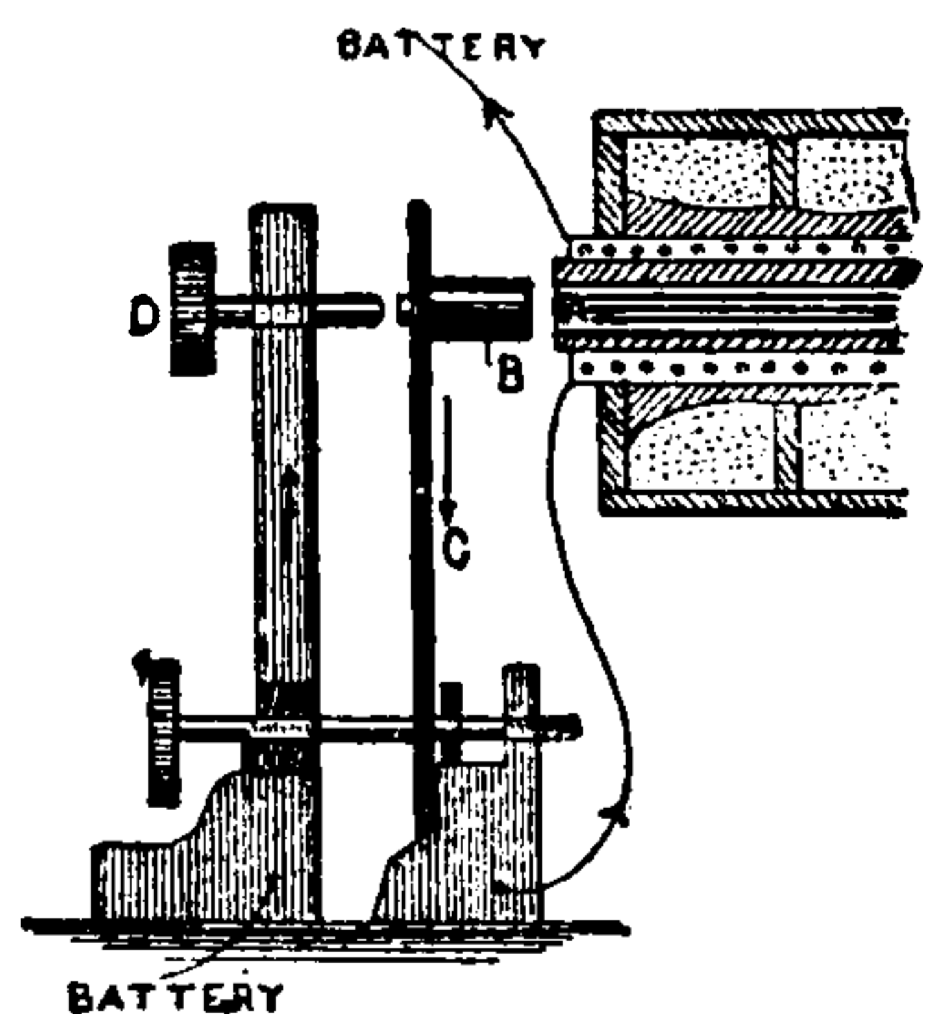
Fig. 171. Automatic Contact Breaker.
