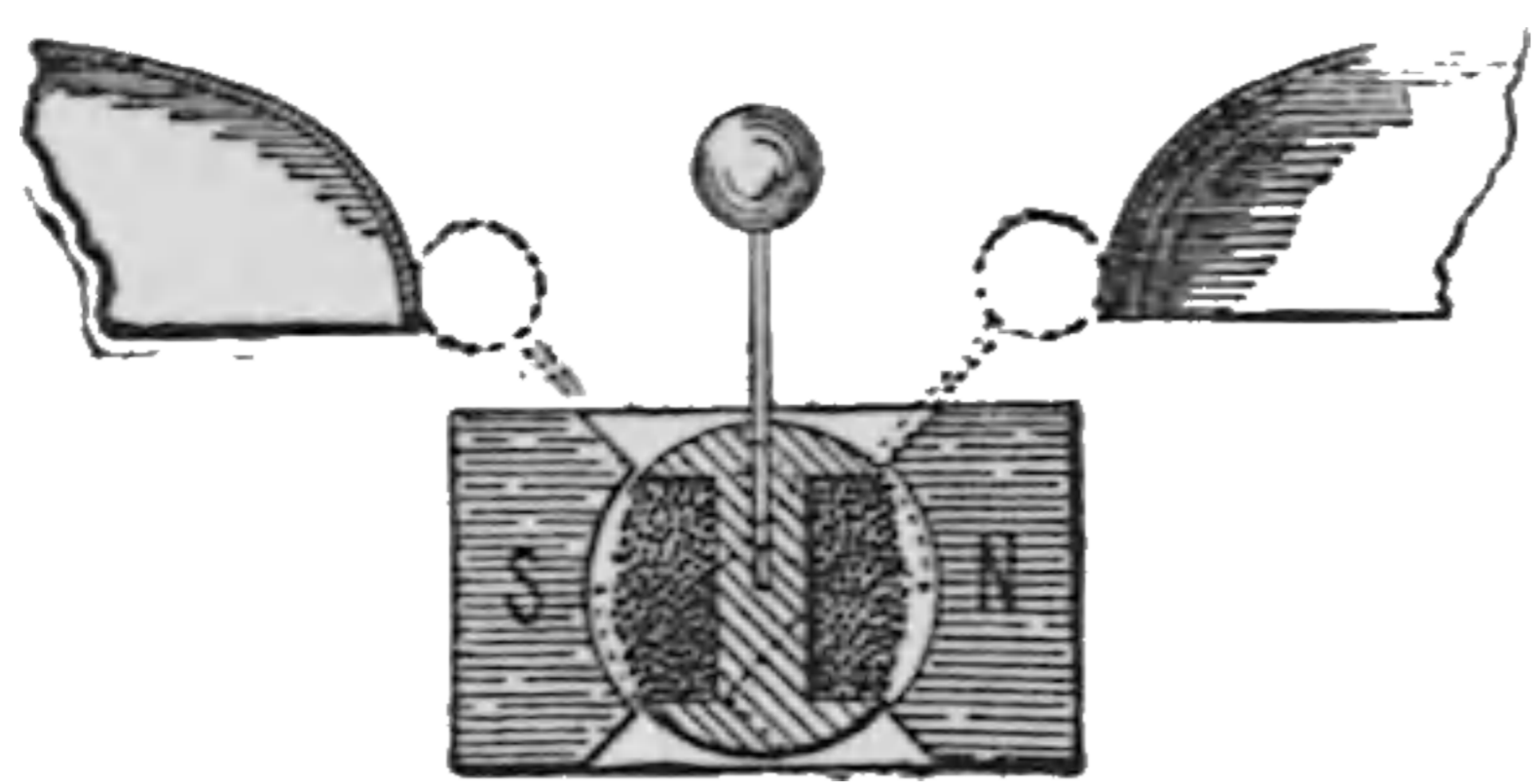
Fig. 45. Siemens-Armature Form of Electro-Magnetic Bell.
