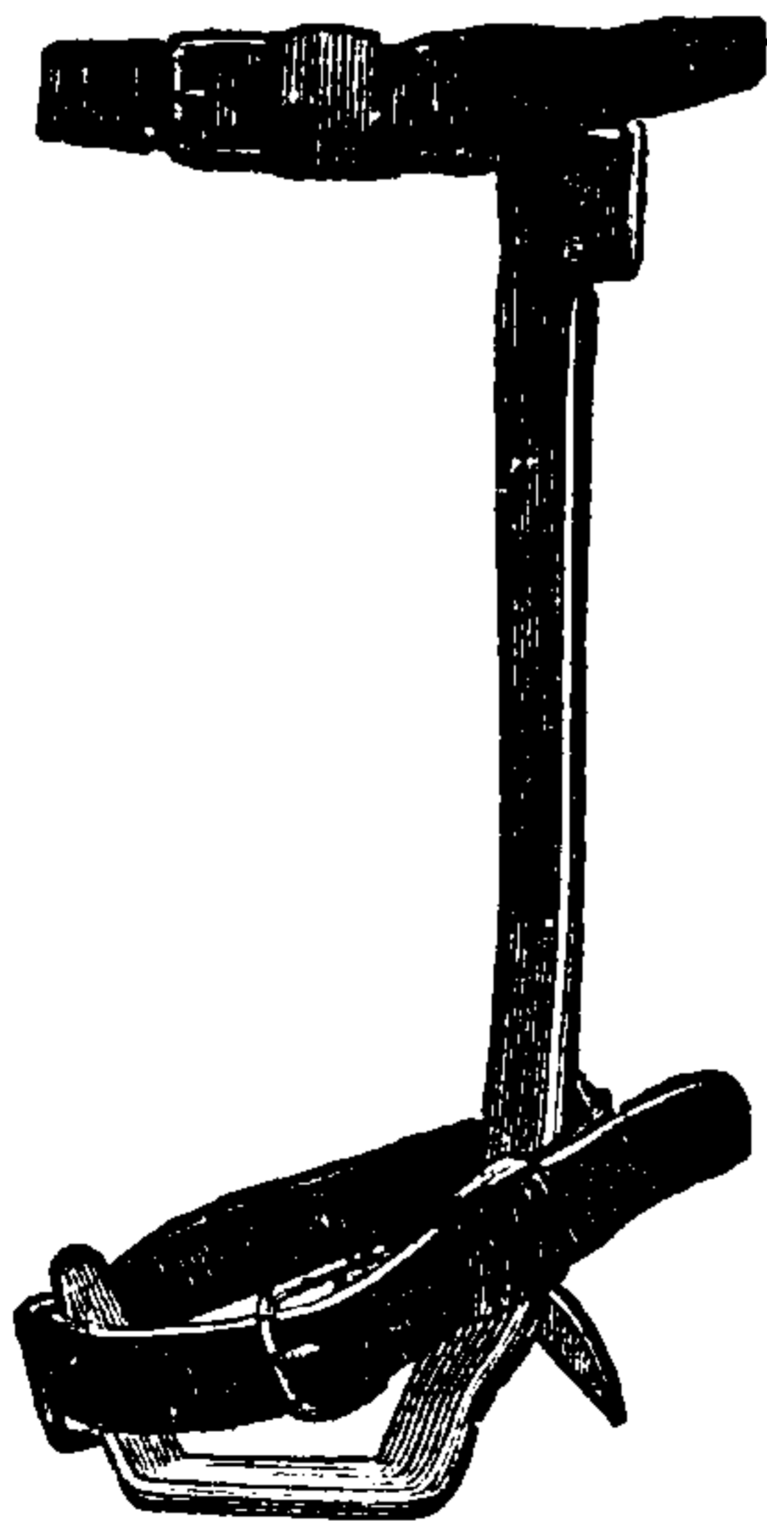
Fig. 136. Climber and Straps.
