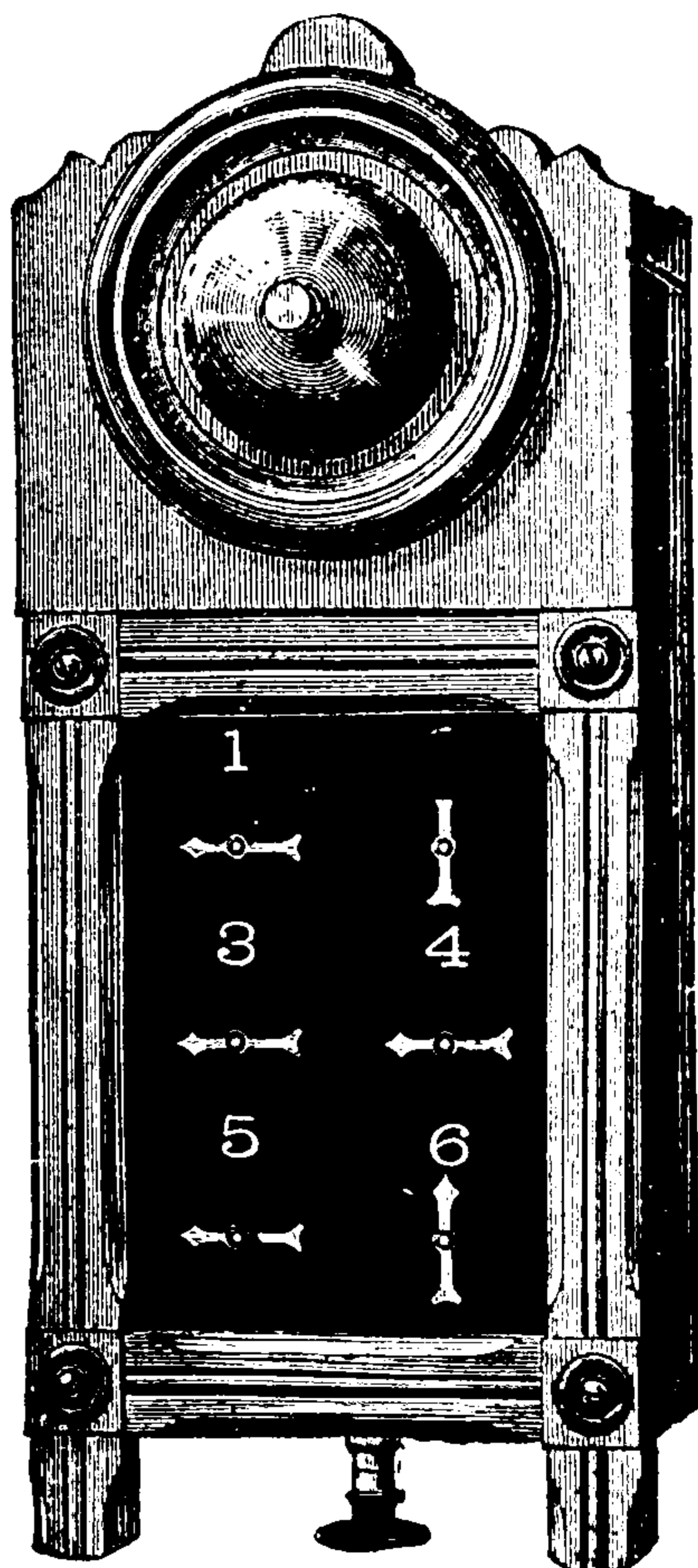
Fig. 17. Needle-Annunciator.
