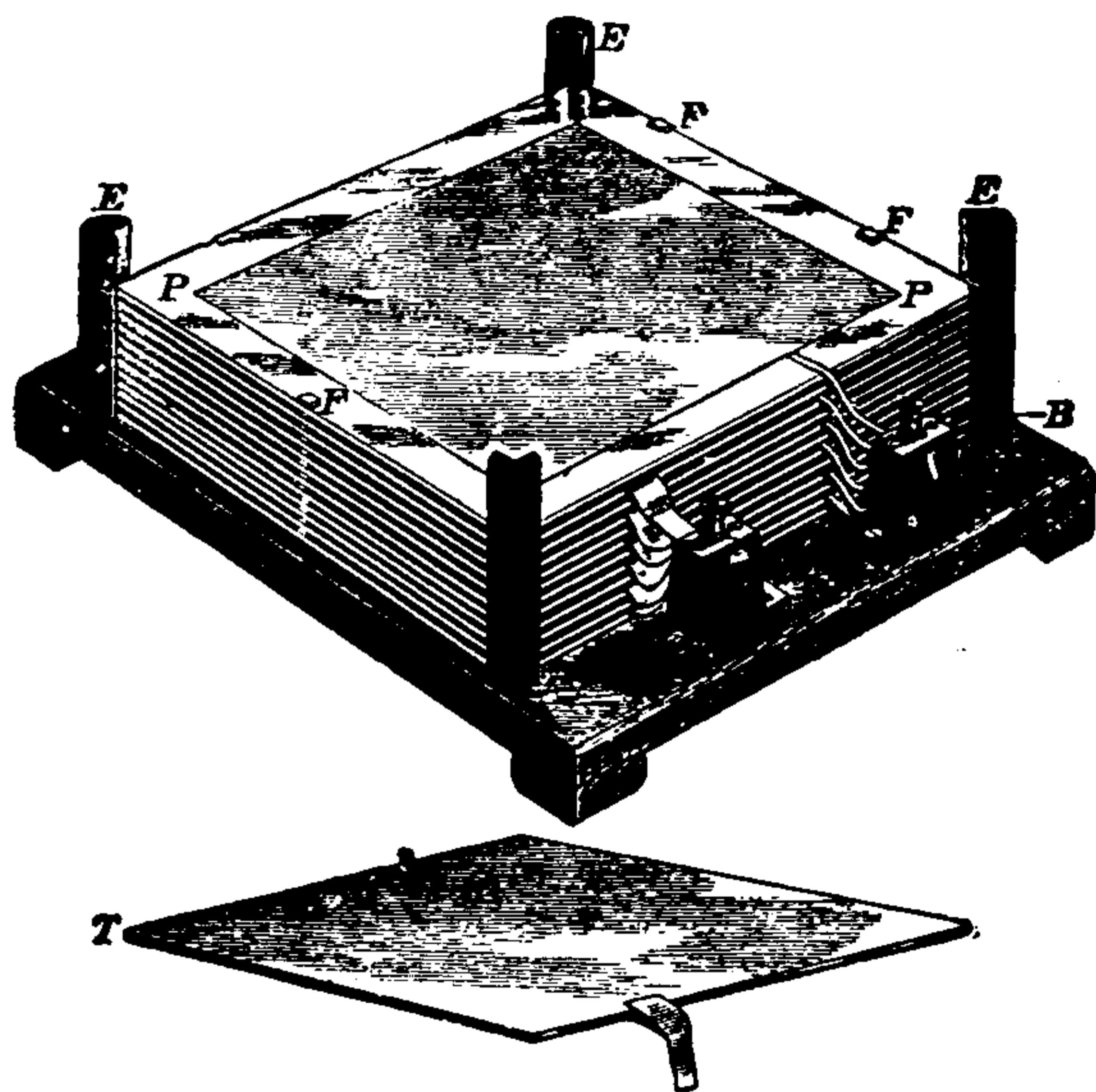
Fig. 169. Air Condenser.
