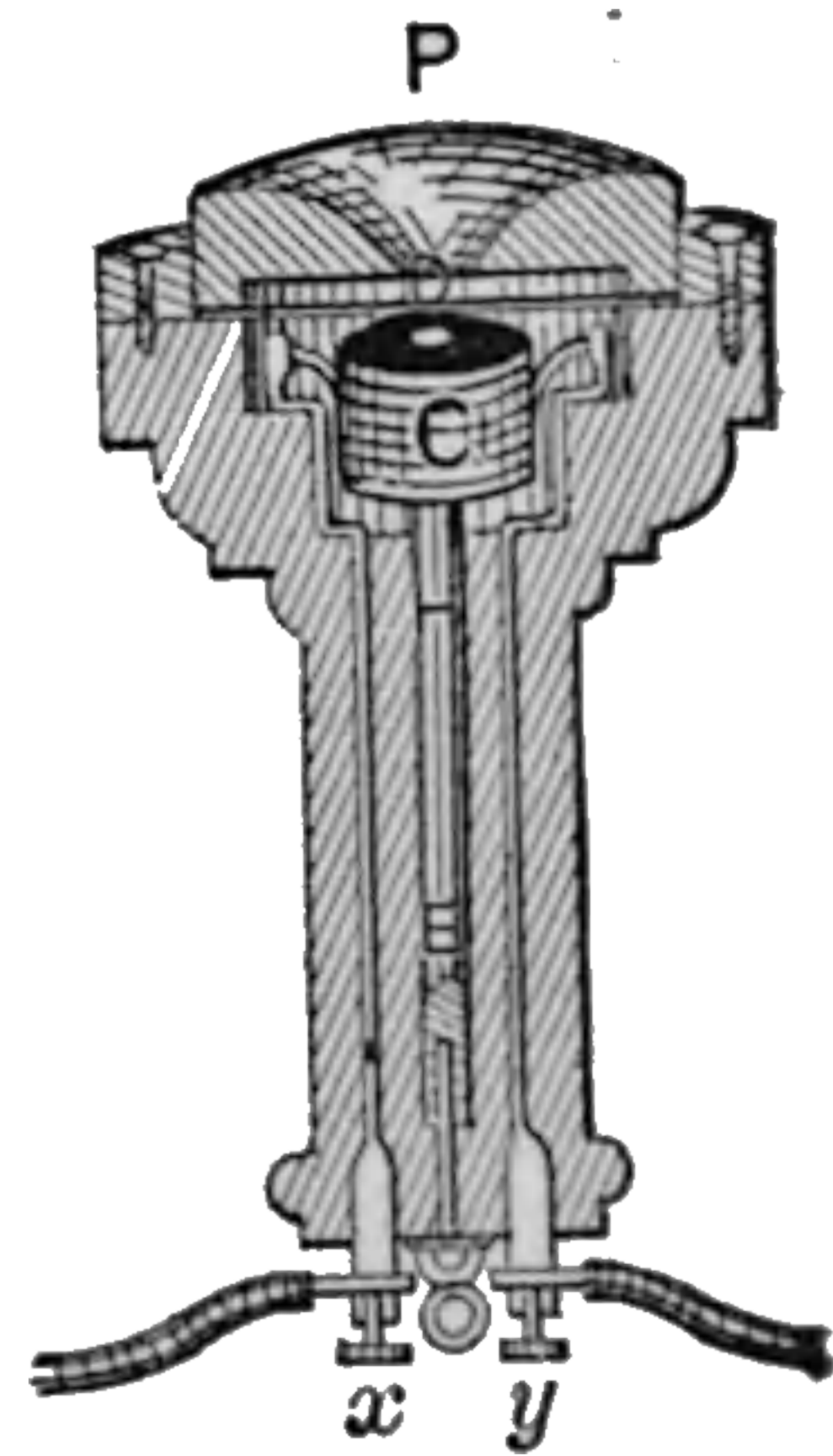
Fig. 549. Telephone.
