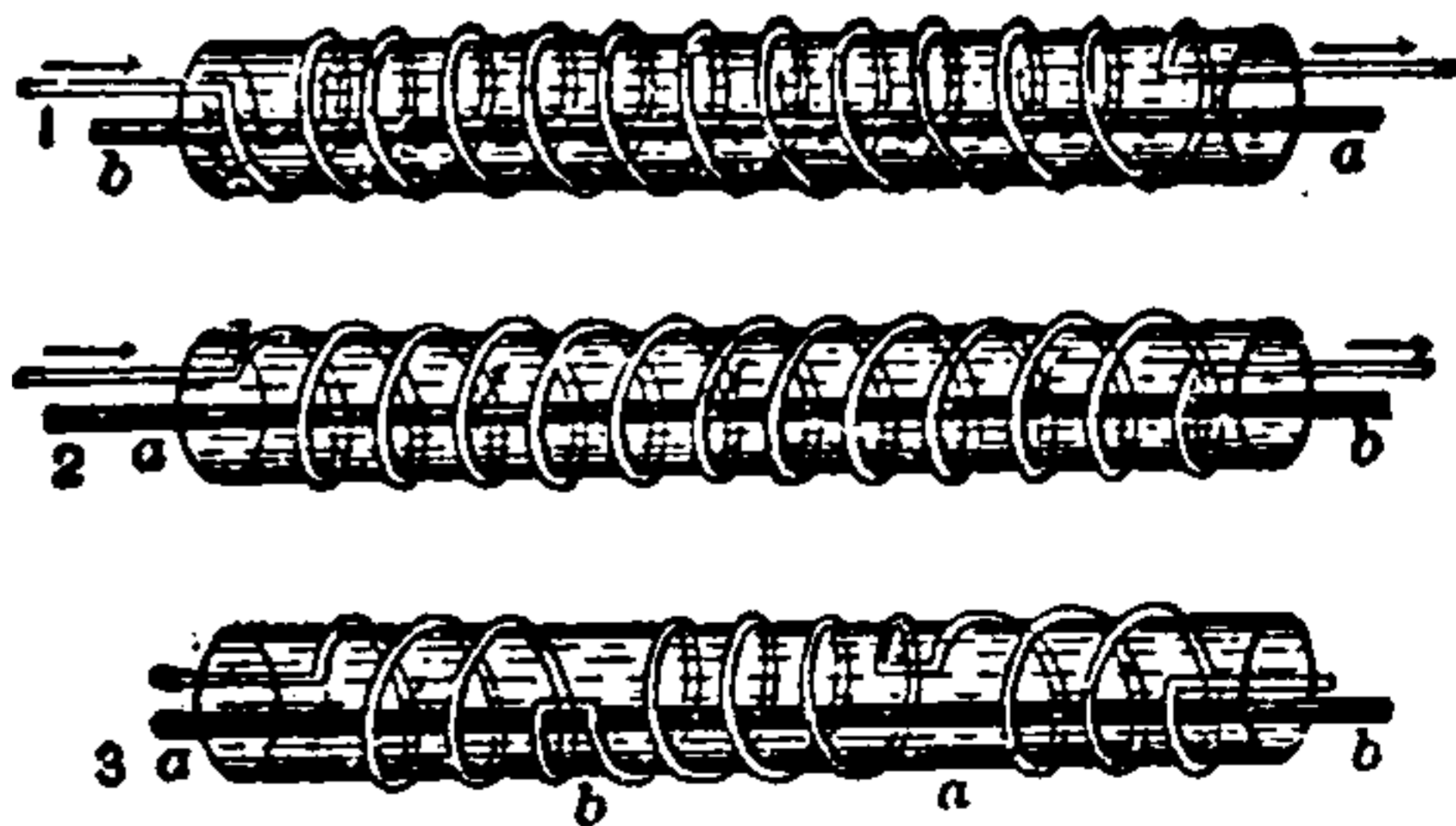
Fig. 507. Right-Handed Helix. Fig. 508. Left-Handed Helix. Fig. 509. Helix, with Consequent Poles.
