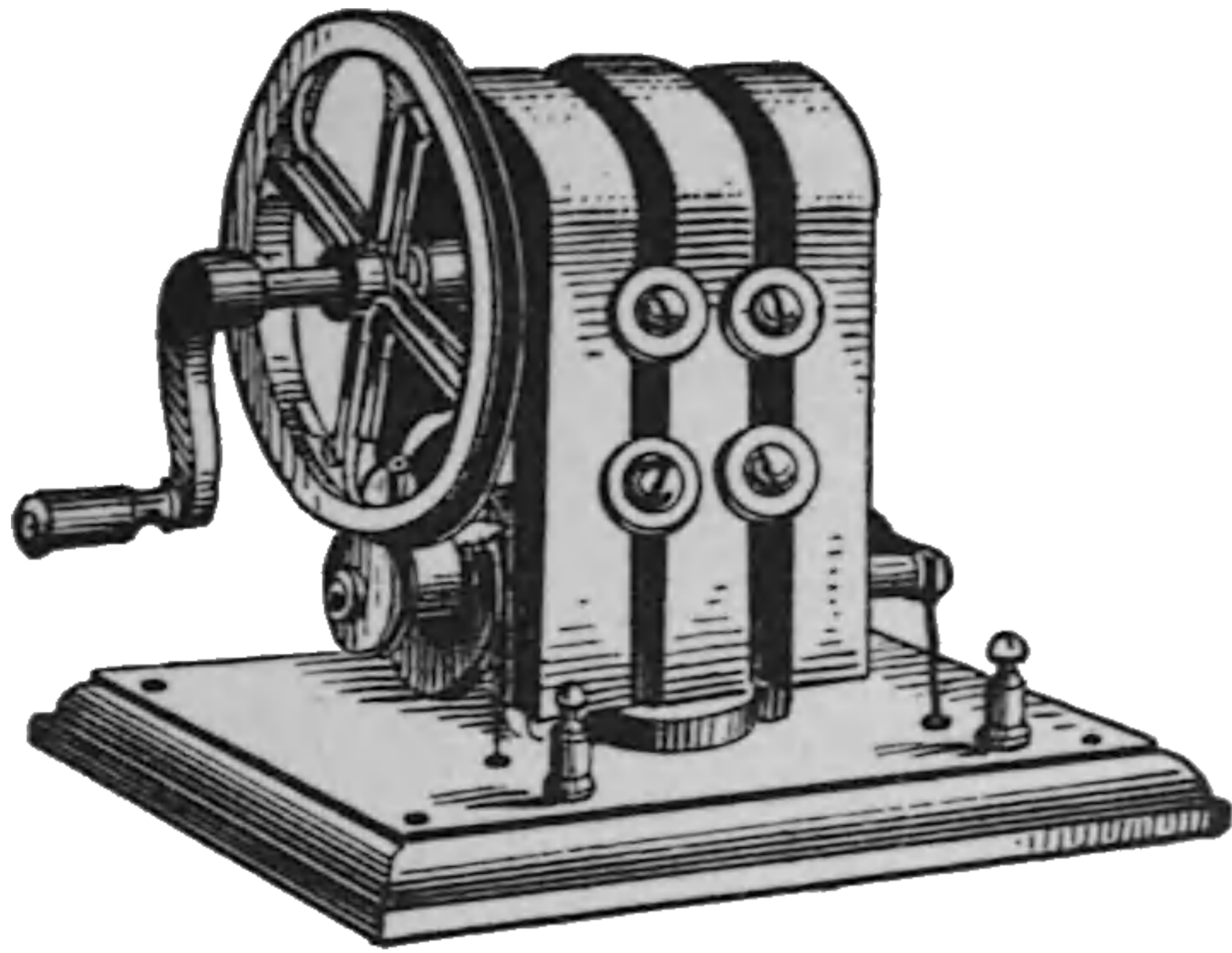
Fig. 362. Magneto-Electric Machine.
