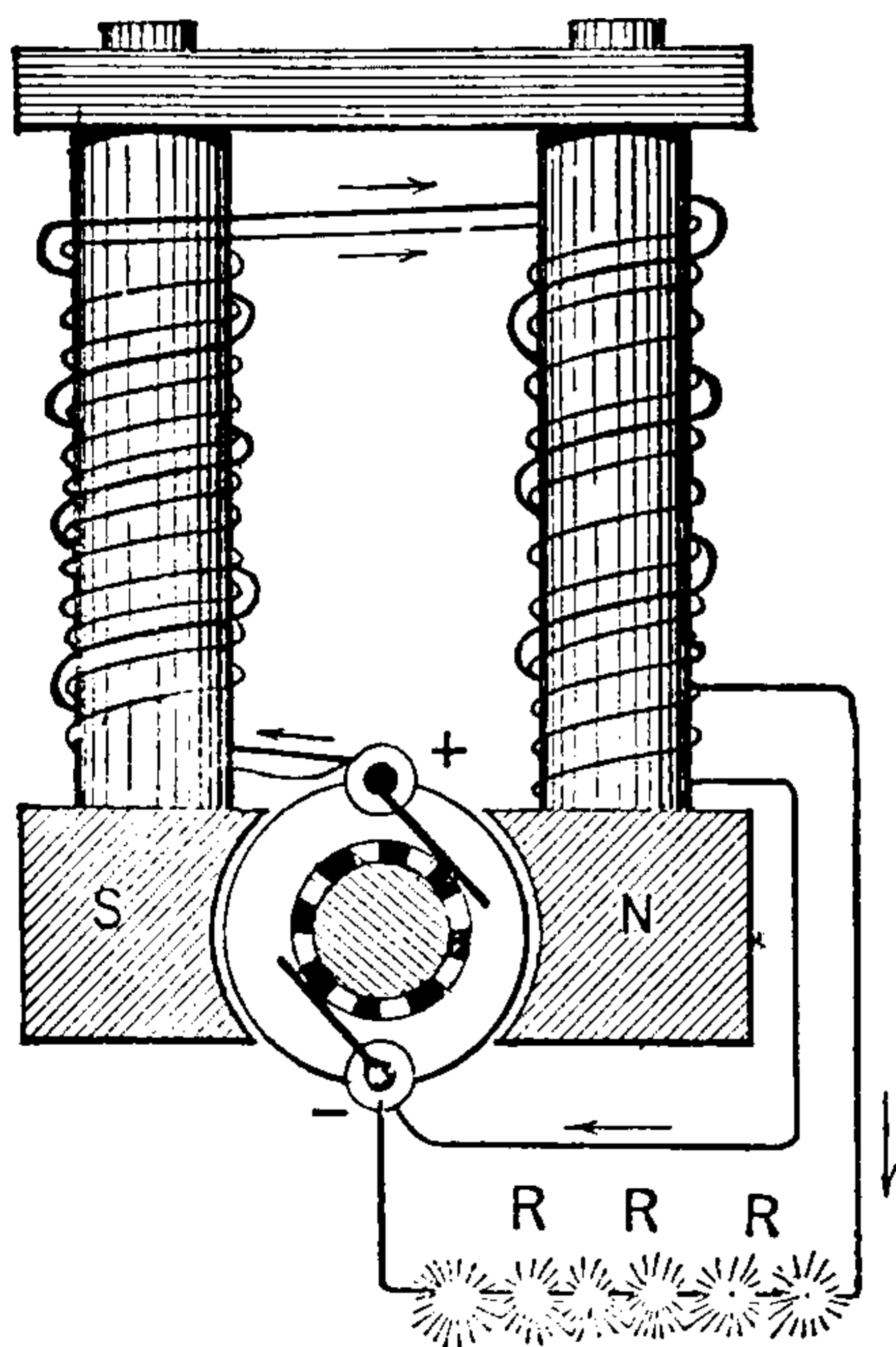
Fig. 353. Series and Shunt-Wound Dynamo.
