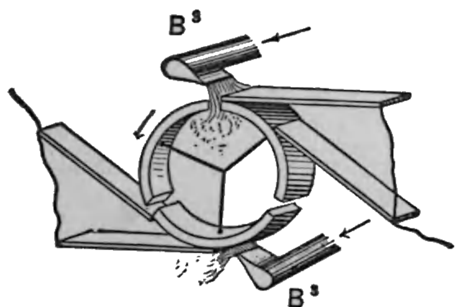
Fig. 4. Air-Blast on Commutator
