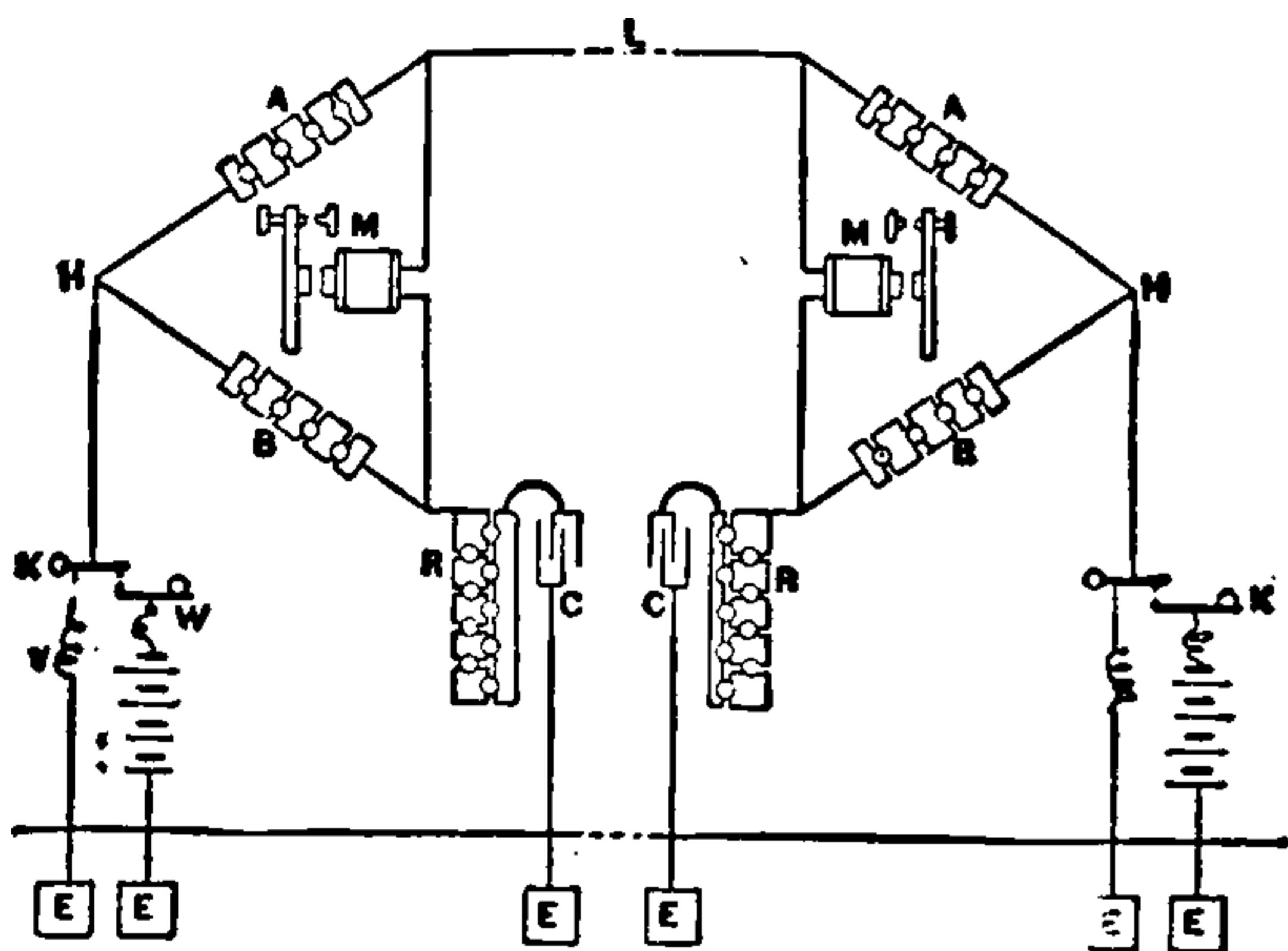
Fig. 528. Duplex Telegraphy, Bridge Method.
