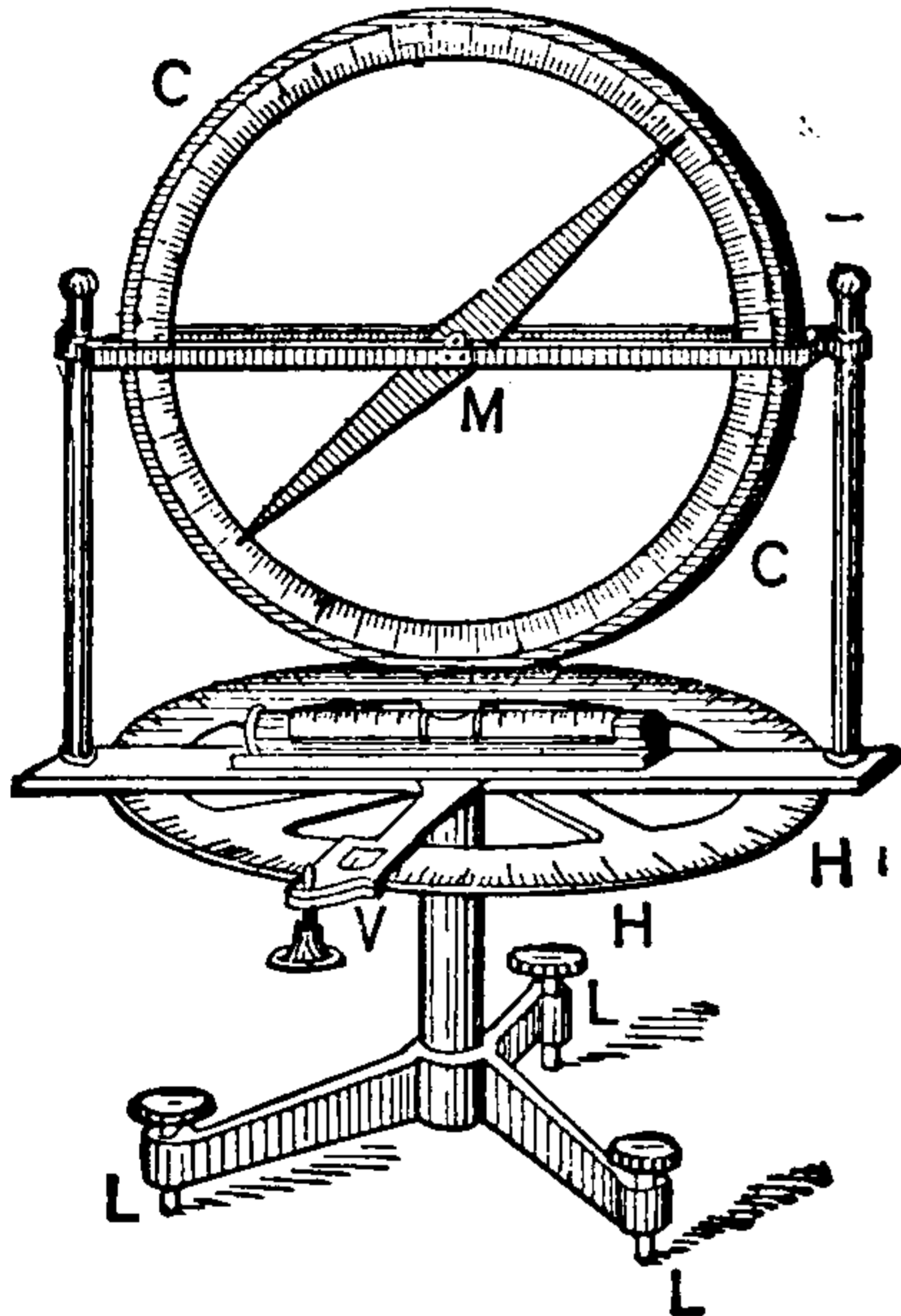
Fig. 162 Inclination Compass.
