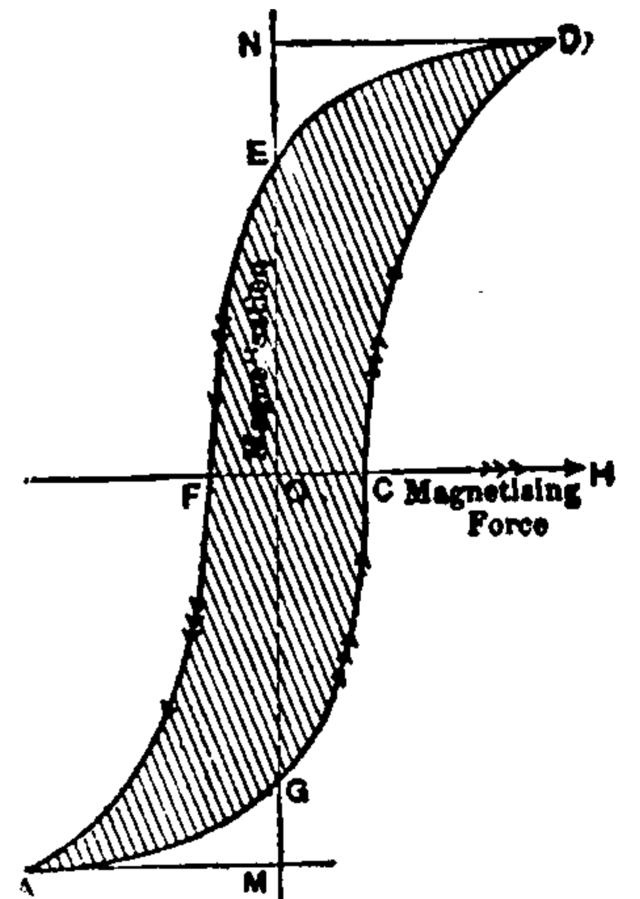
Fig. 295. Curves of Hysteresis (Ewing).
