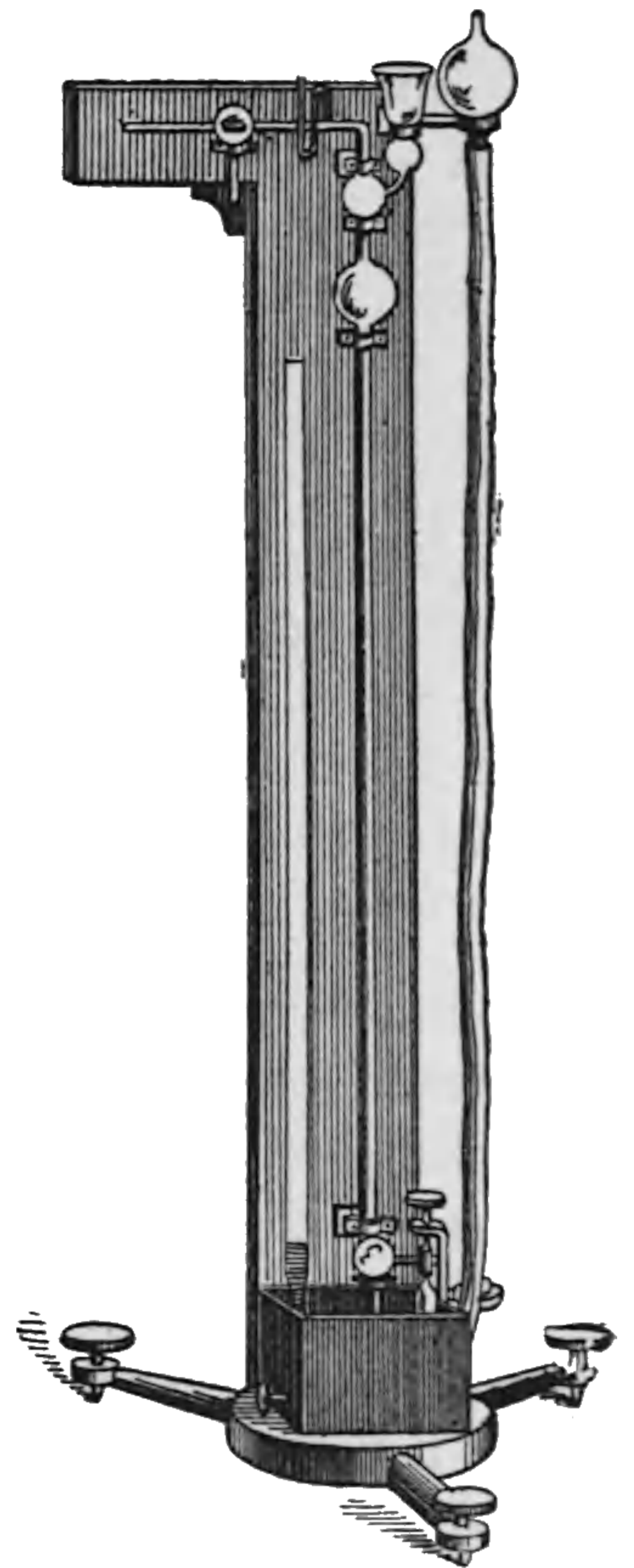
Fig. 454. Geissler's Mercurial Air Pump.
