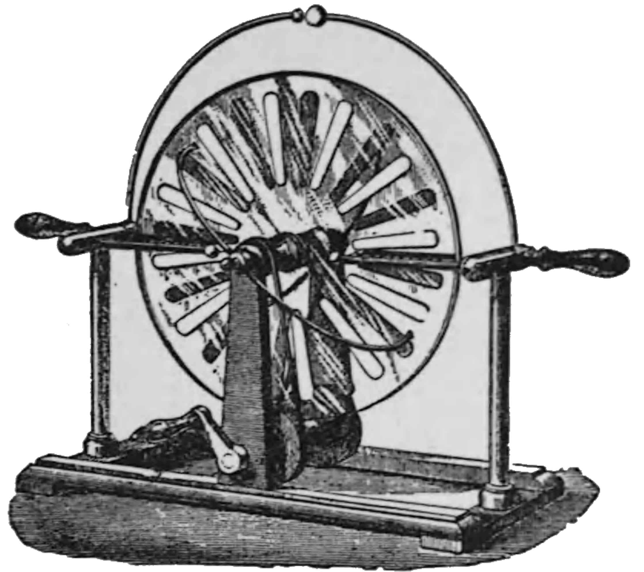
Fig. 363. The Wimshurst Electrical Machine.
