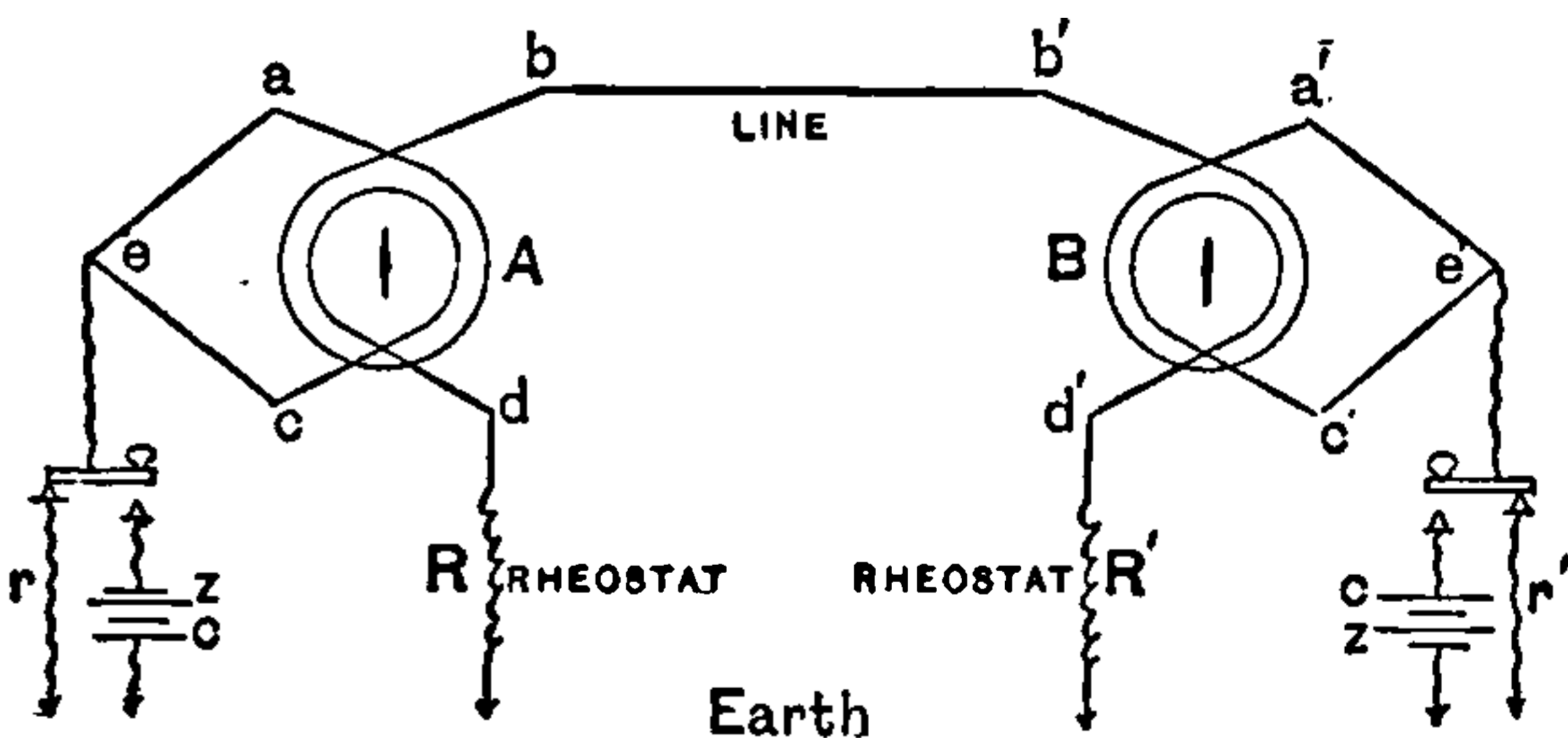
Fig. 529. Duplex Telegraphy, Differential Method.
