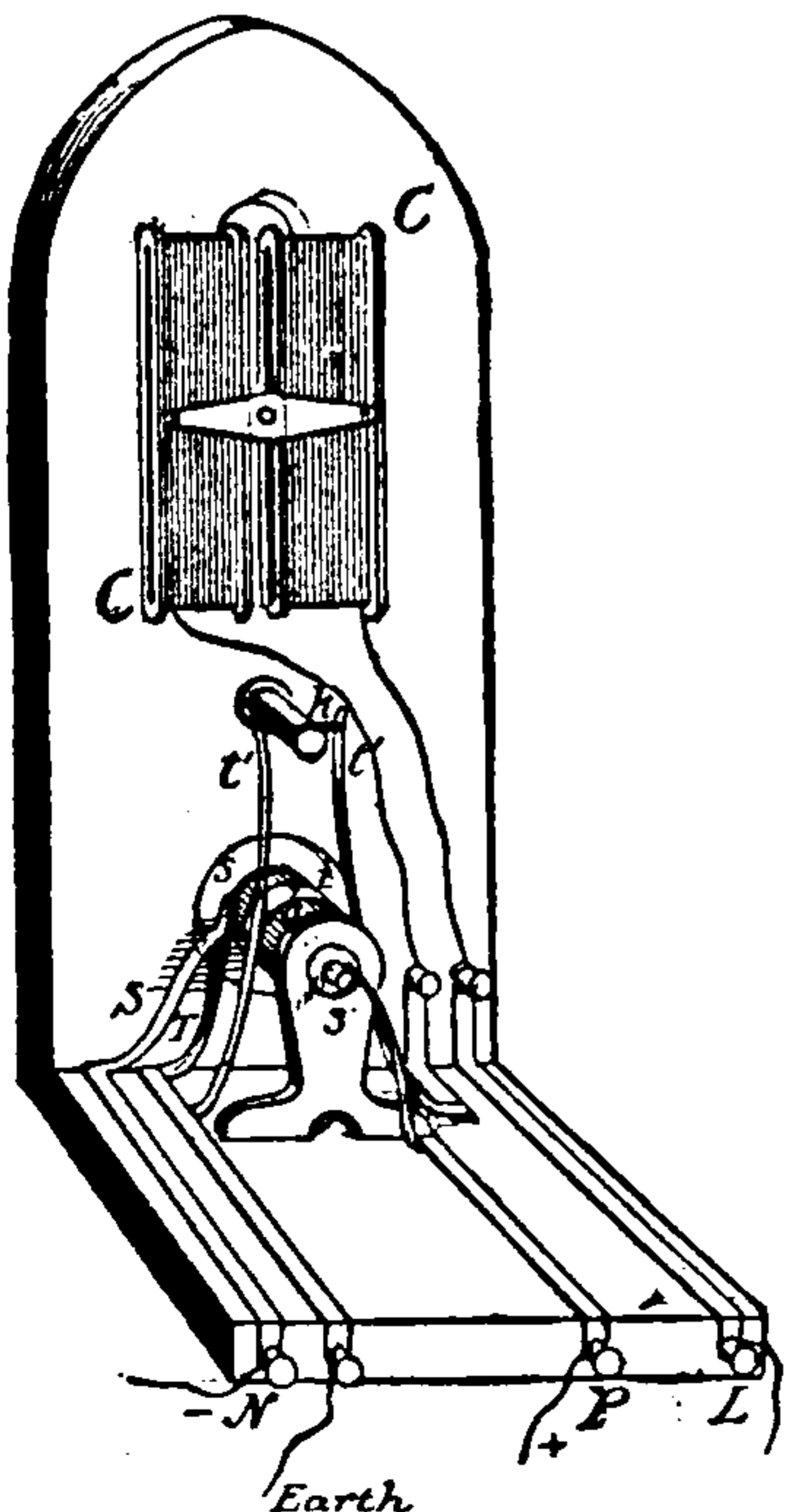
Fig. 536. Wheatstone and Cooke's Single-Needle Apparatus, Internal Arrangement.
