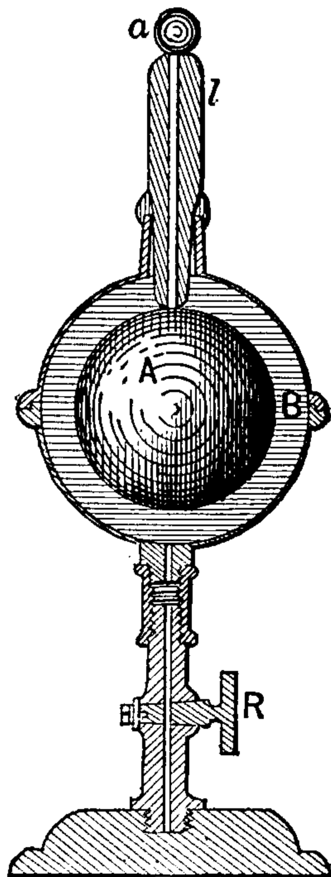
Fig 99. Condenser.
