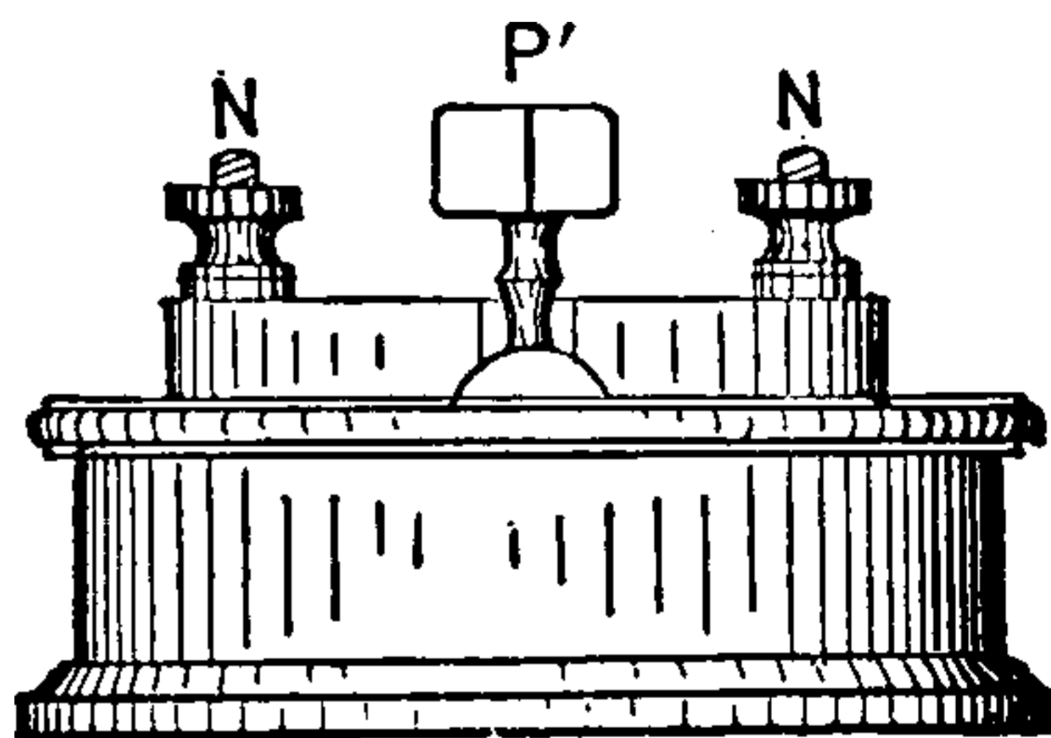
Fig 245. Elevation of Standardized Condenser.
