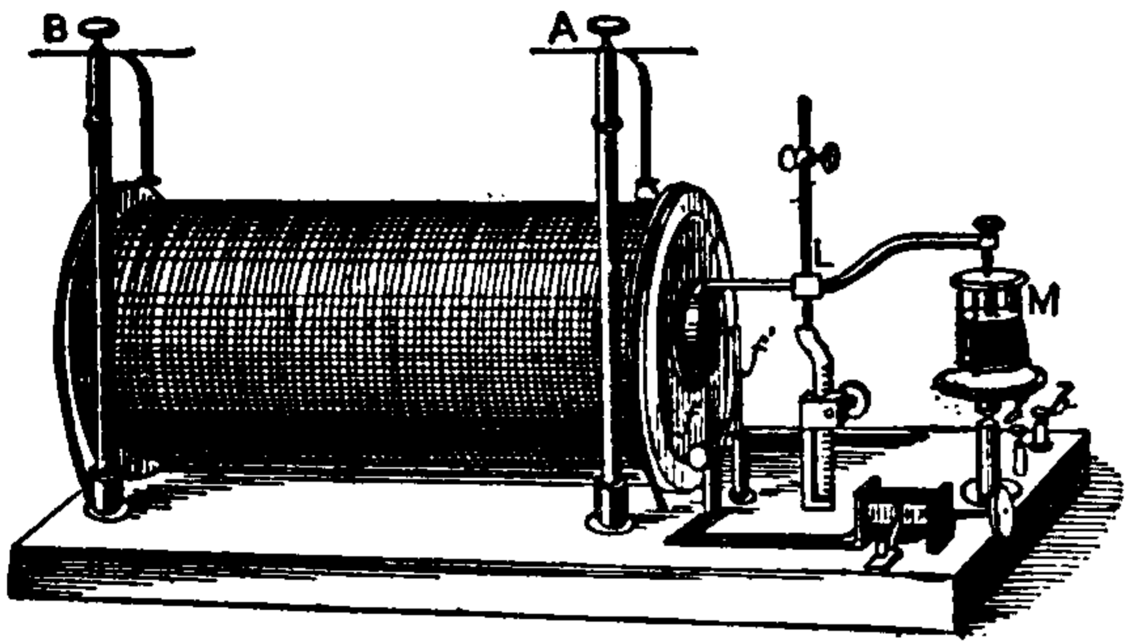
Fig. 142. Ruhmkorff Coil.
