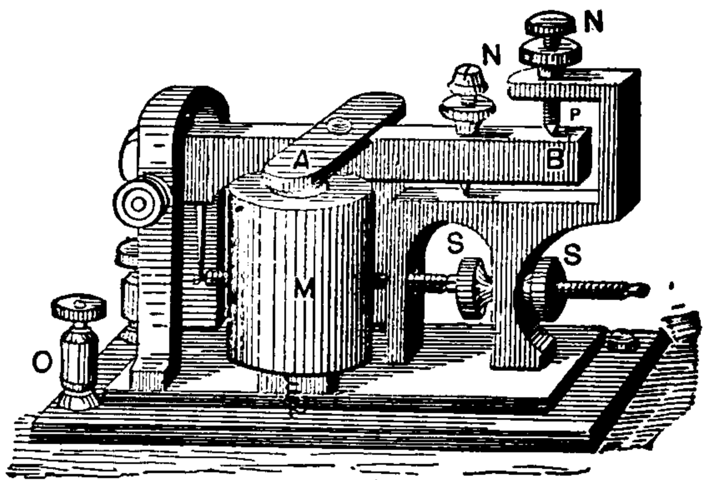
Fig 510. Morse Sounder.
