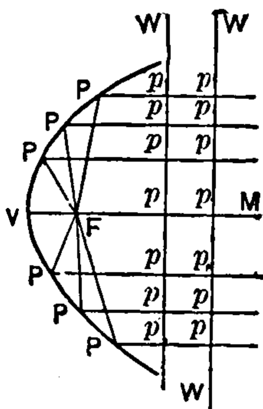
Fig. 472. Parabolic Reflector.
