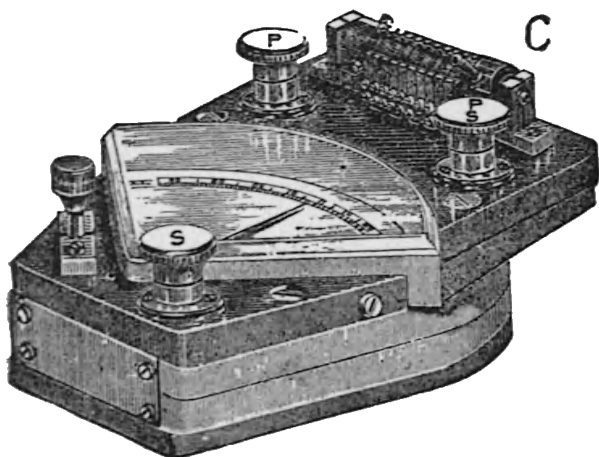
Fig. 12. Ayrton and Perry Ammeter.
