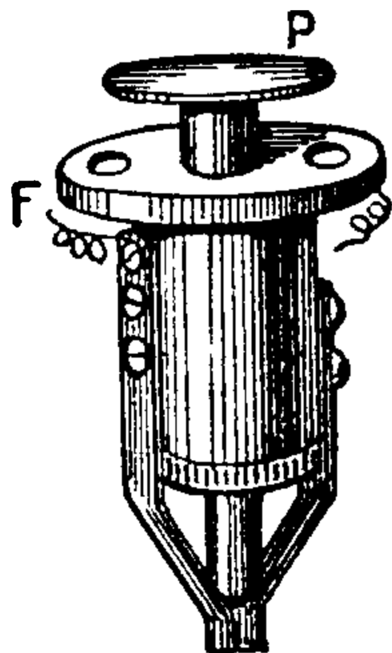
Fig. 90. Floor Push.
