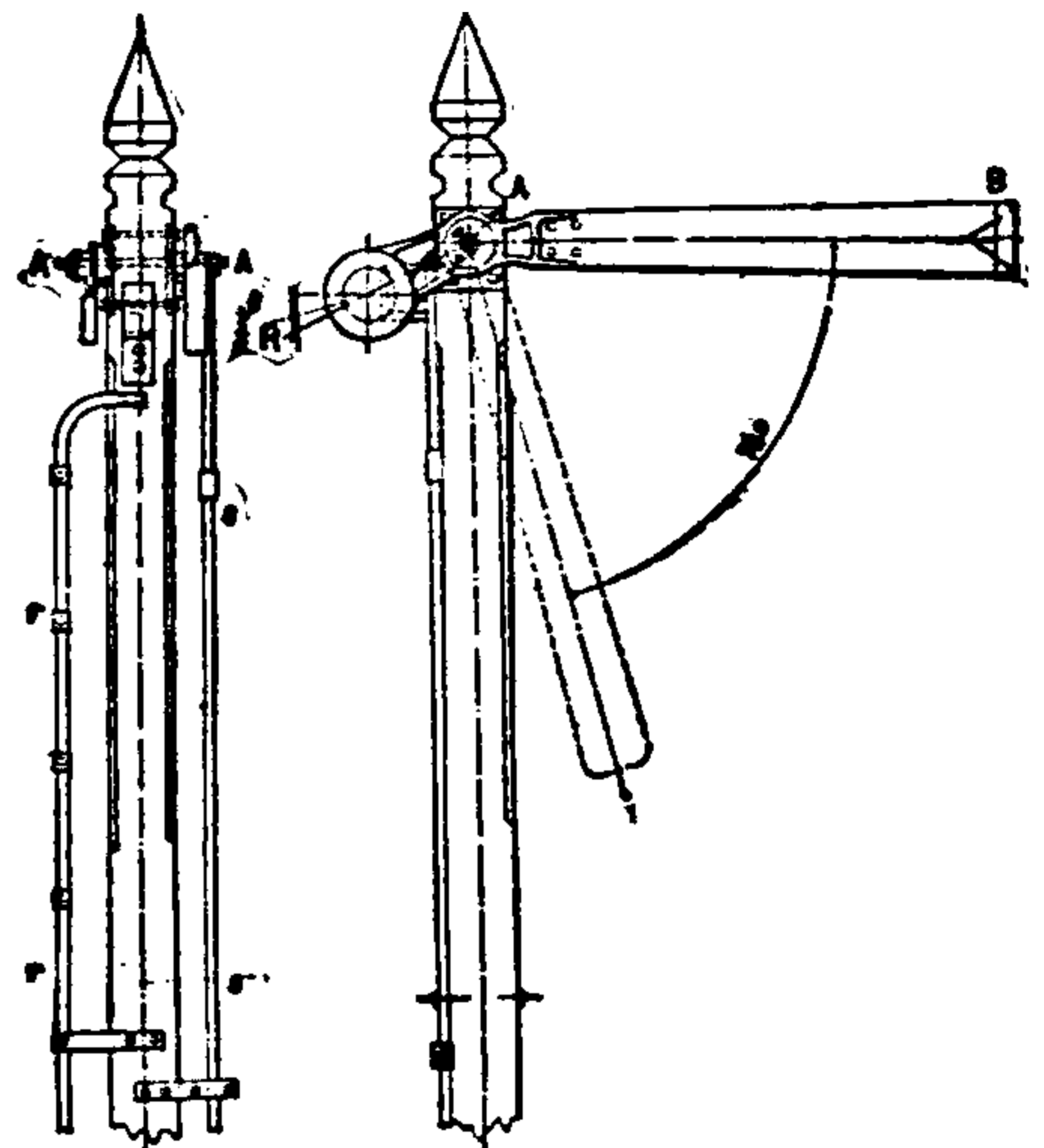
Fig. 463. Semaphore Signal—Absolute System.
