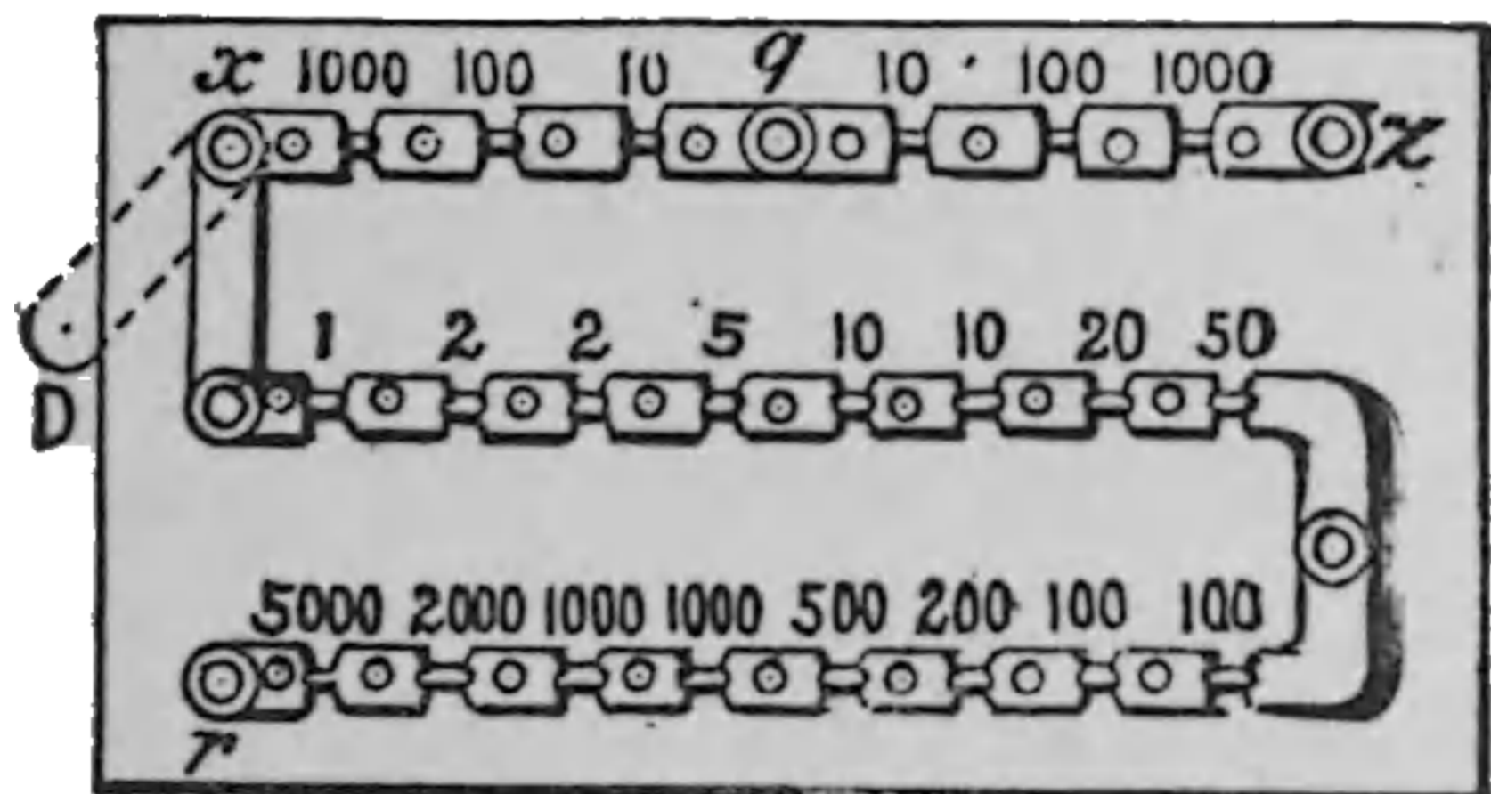
Fig. 75. Box Balance.
