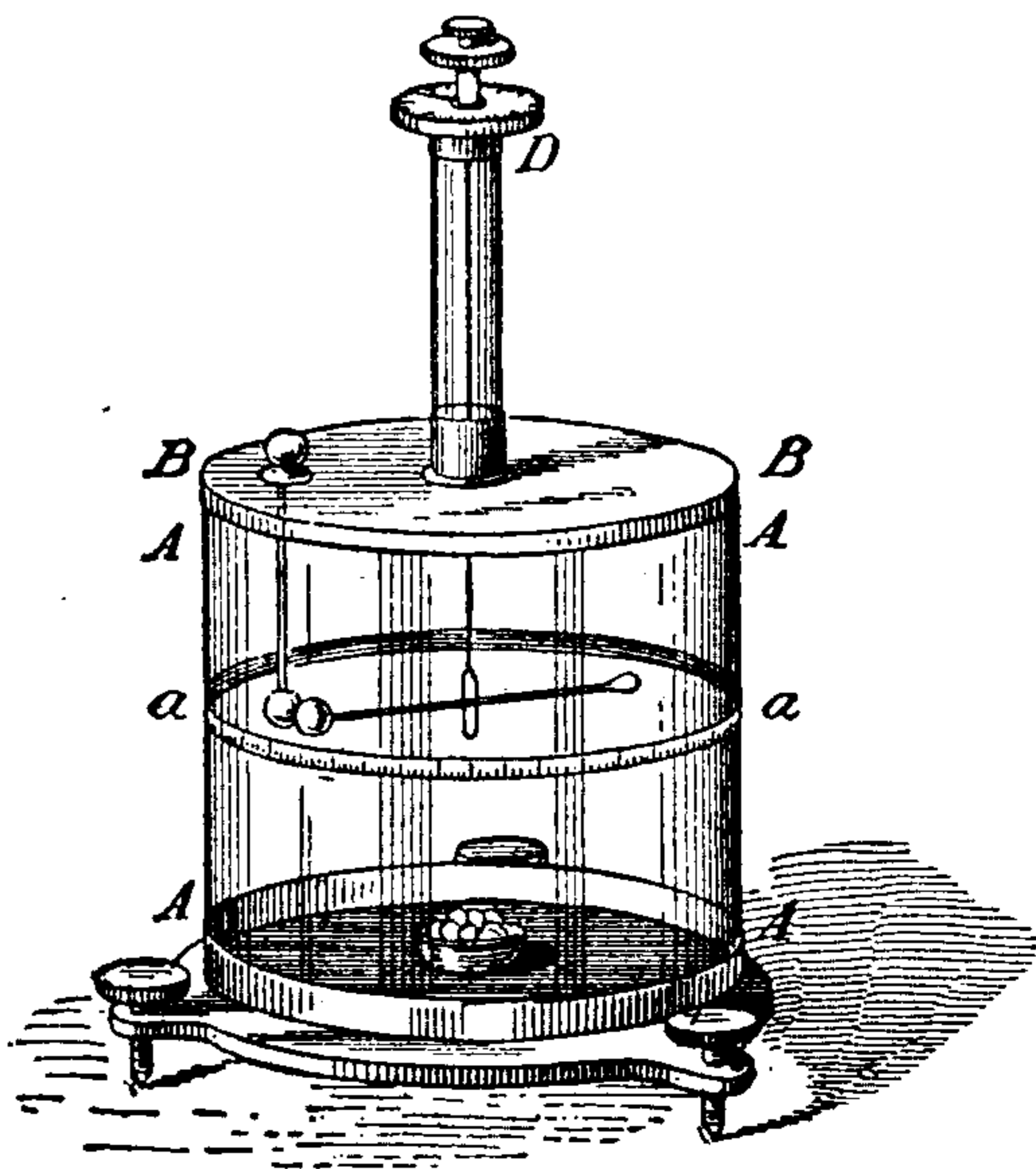
Fig. 34. Coulomb's Torsion Balance.
