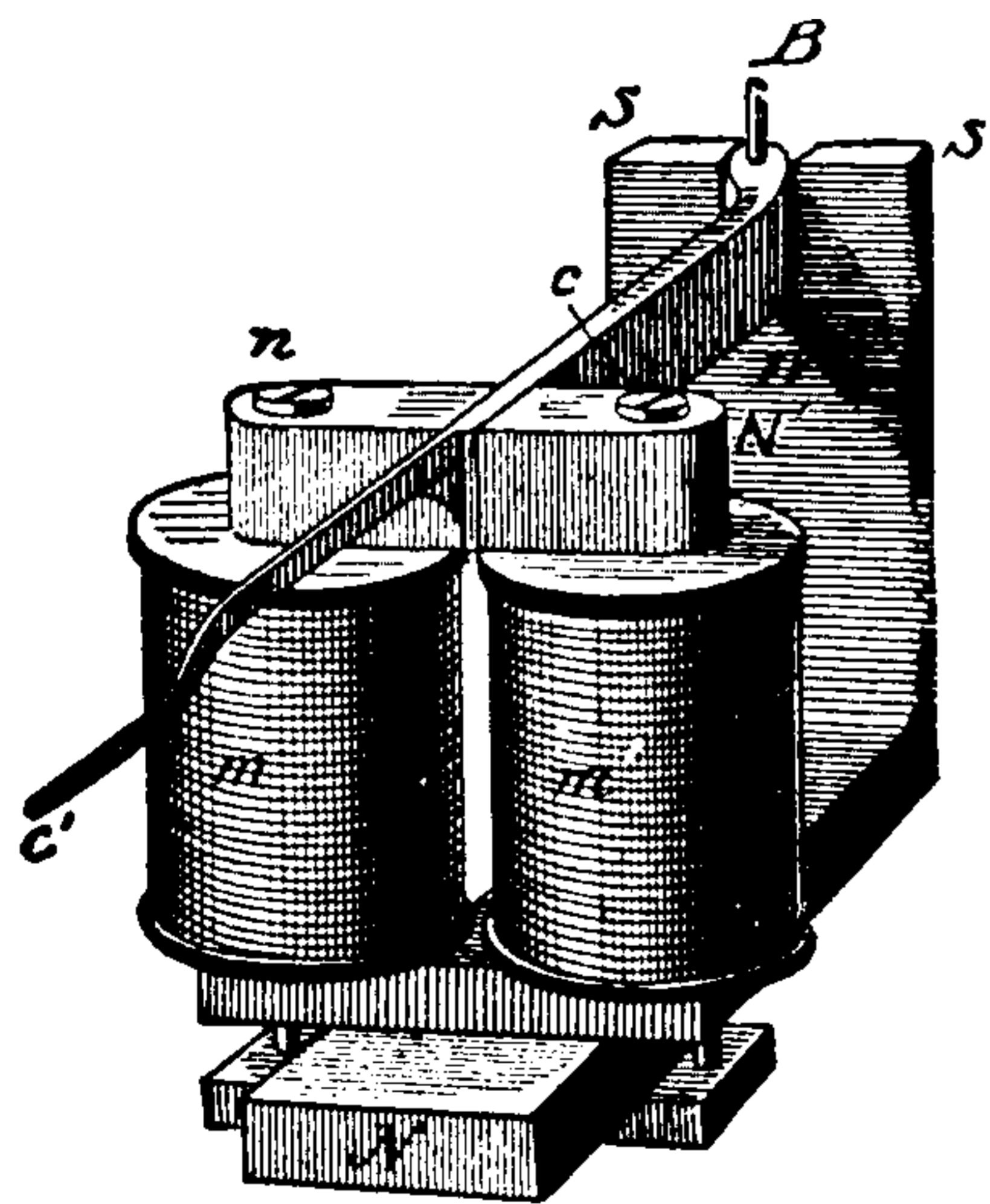
Fig. 482. Polarized Relay.
