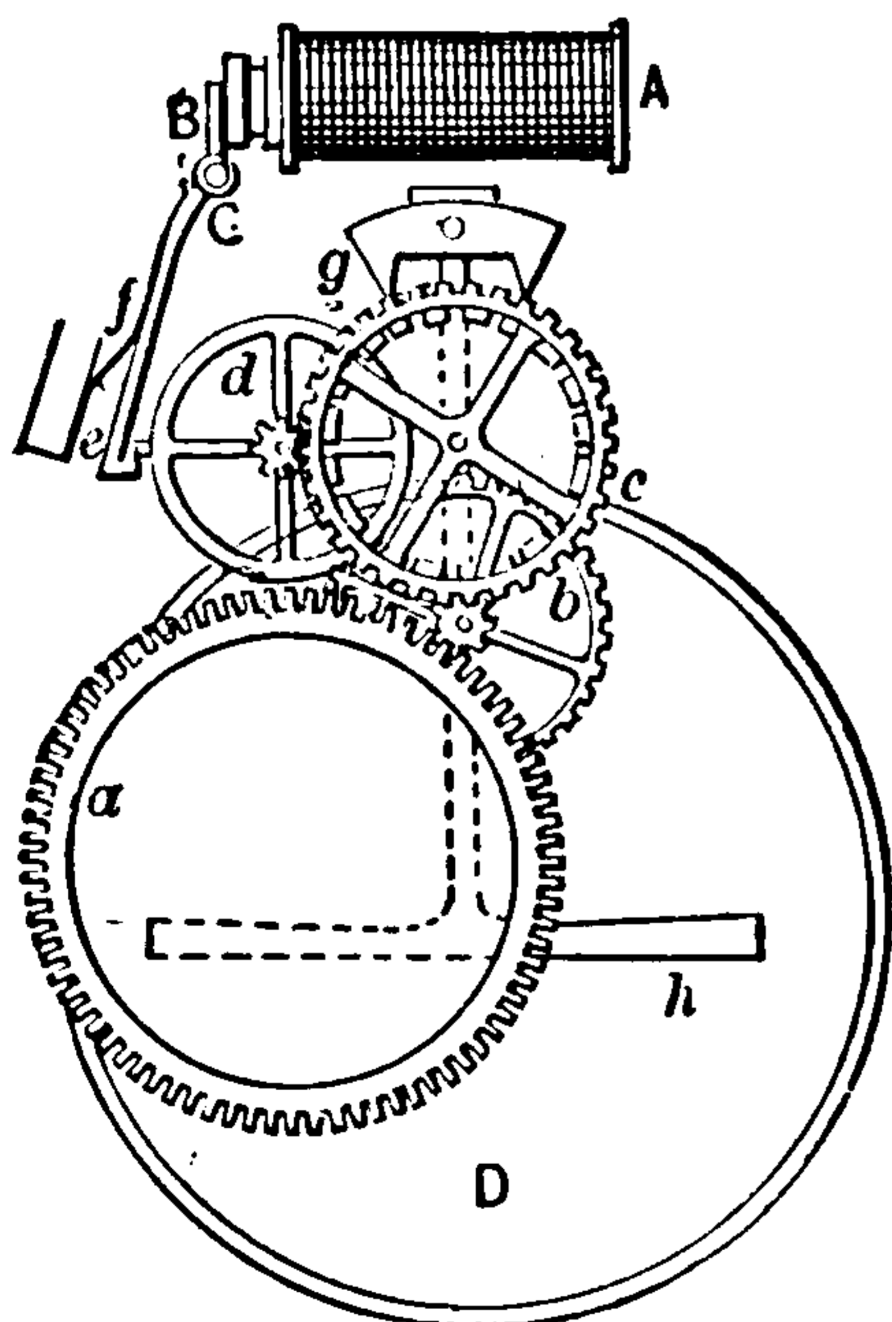
Fig. 7. Electrically Started Mechanical Alarm.
