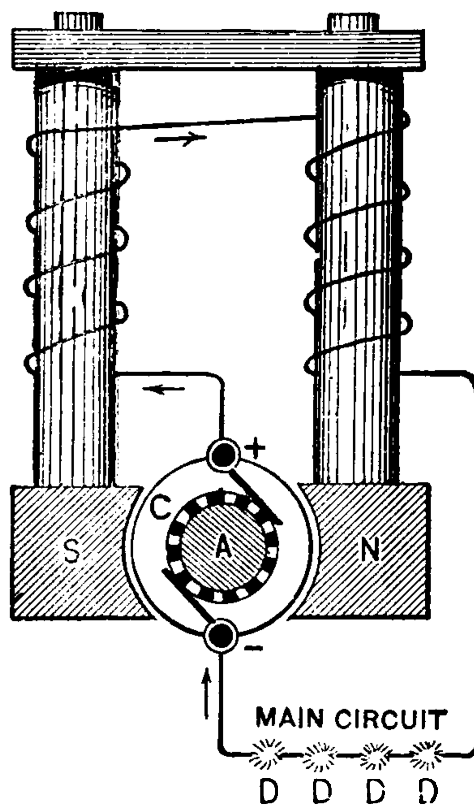
Fig. 354. Series Dynamo.
