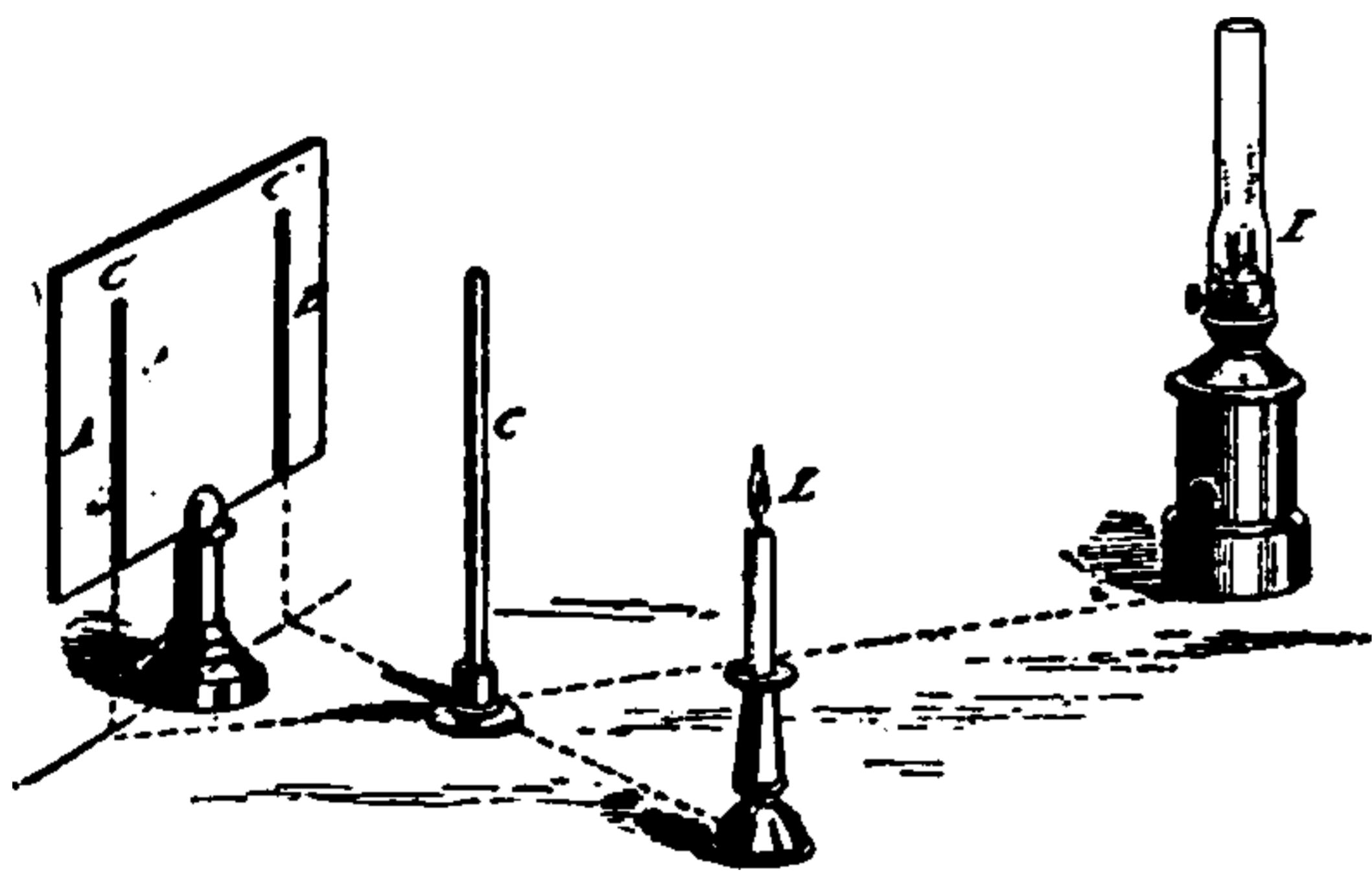
Fig. 427. The Shadow Photometer.
