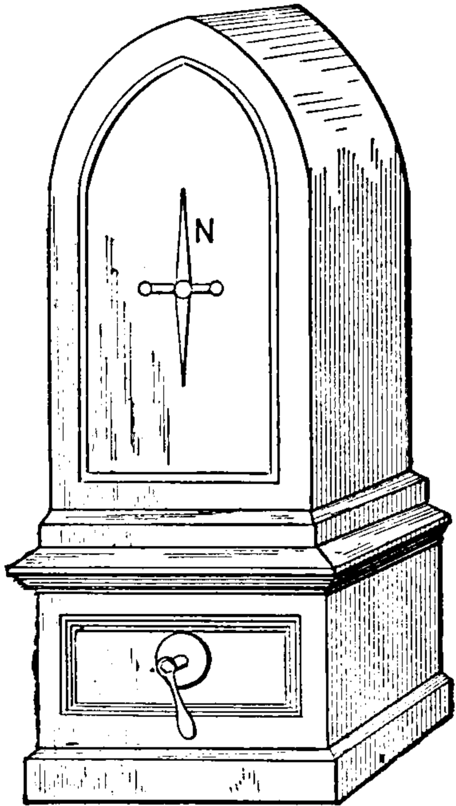
Fig. 535. Single-Needle Telegraphic Apparatus.
