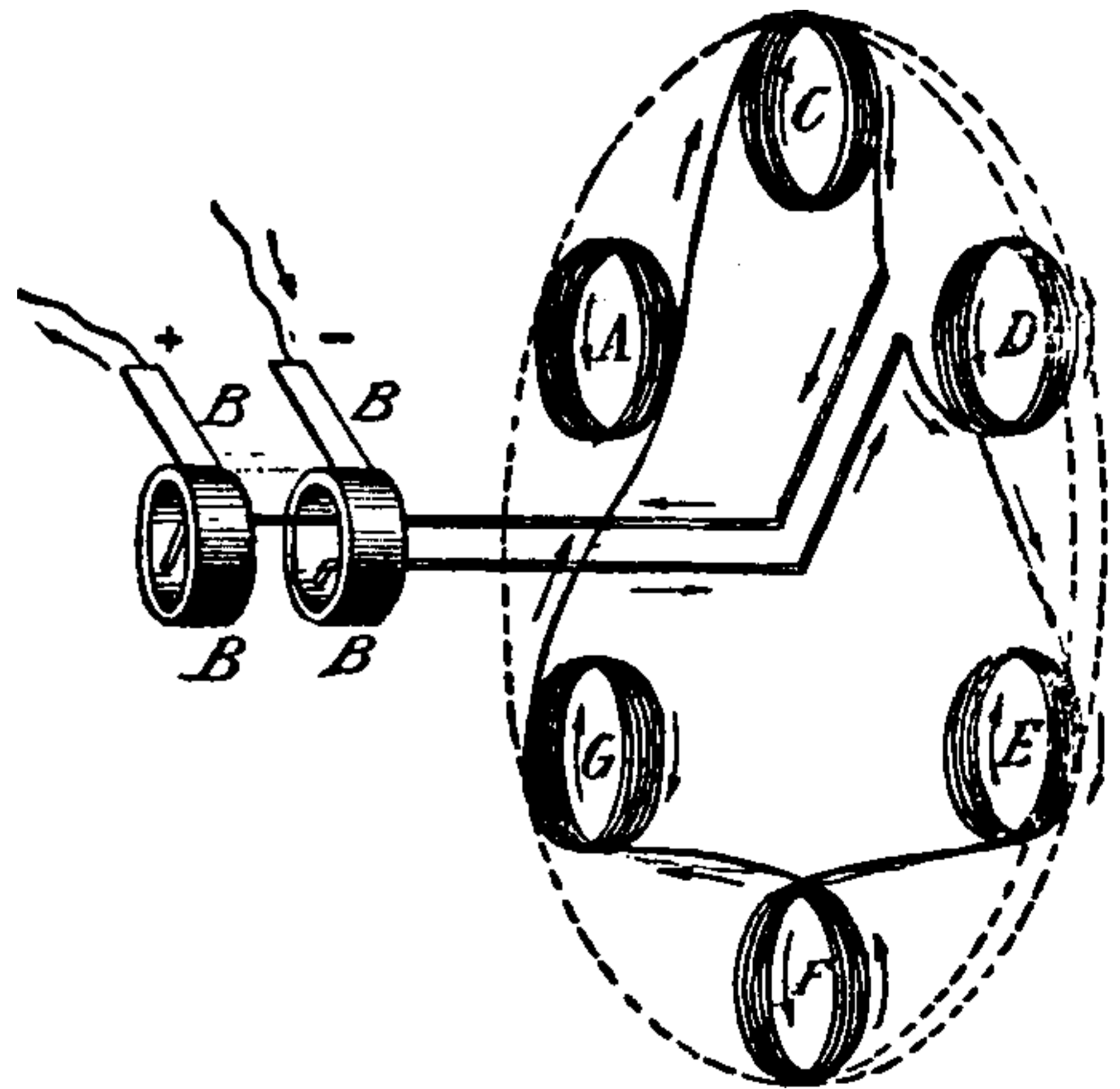
Fig. 150. Series Connection of Armature Coils.
