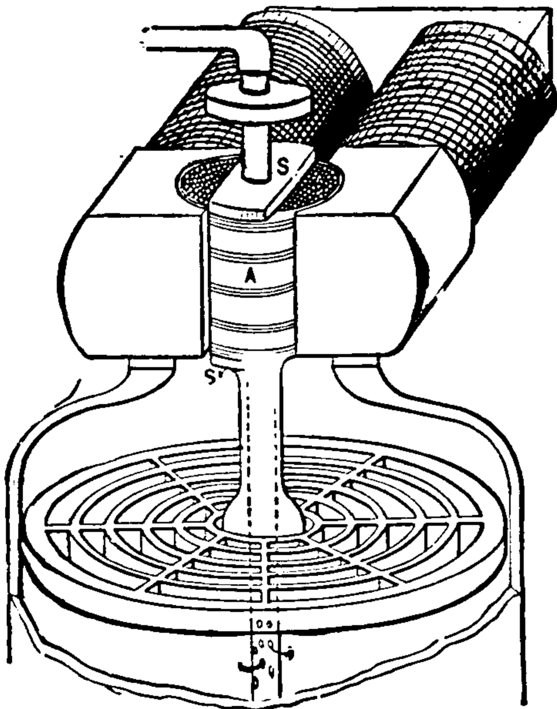
Fig. 401. Pyromagnetic Motor.
