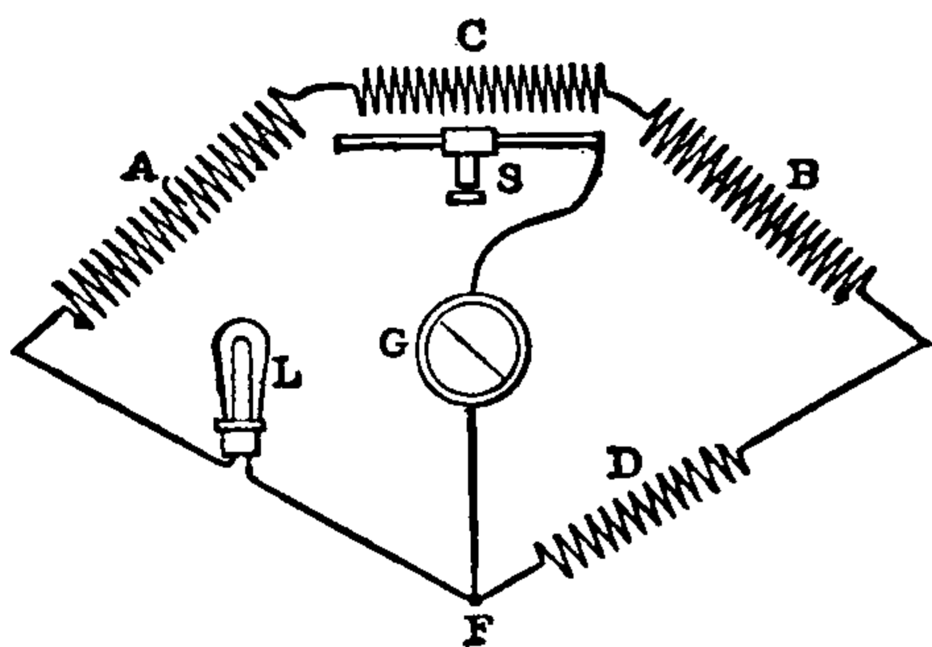
Fig. 297. Edison-Howell Lamp Indicator.
