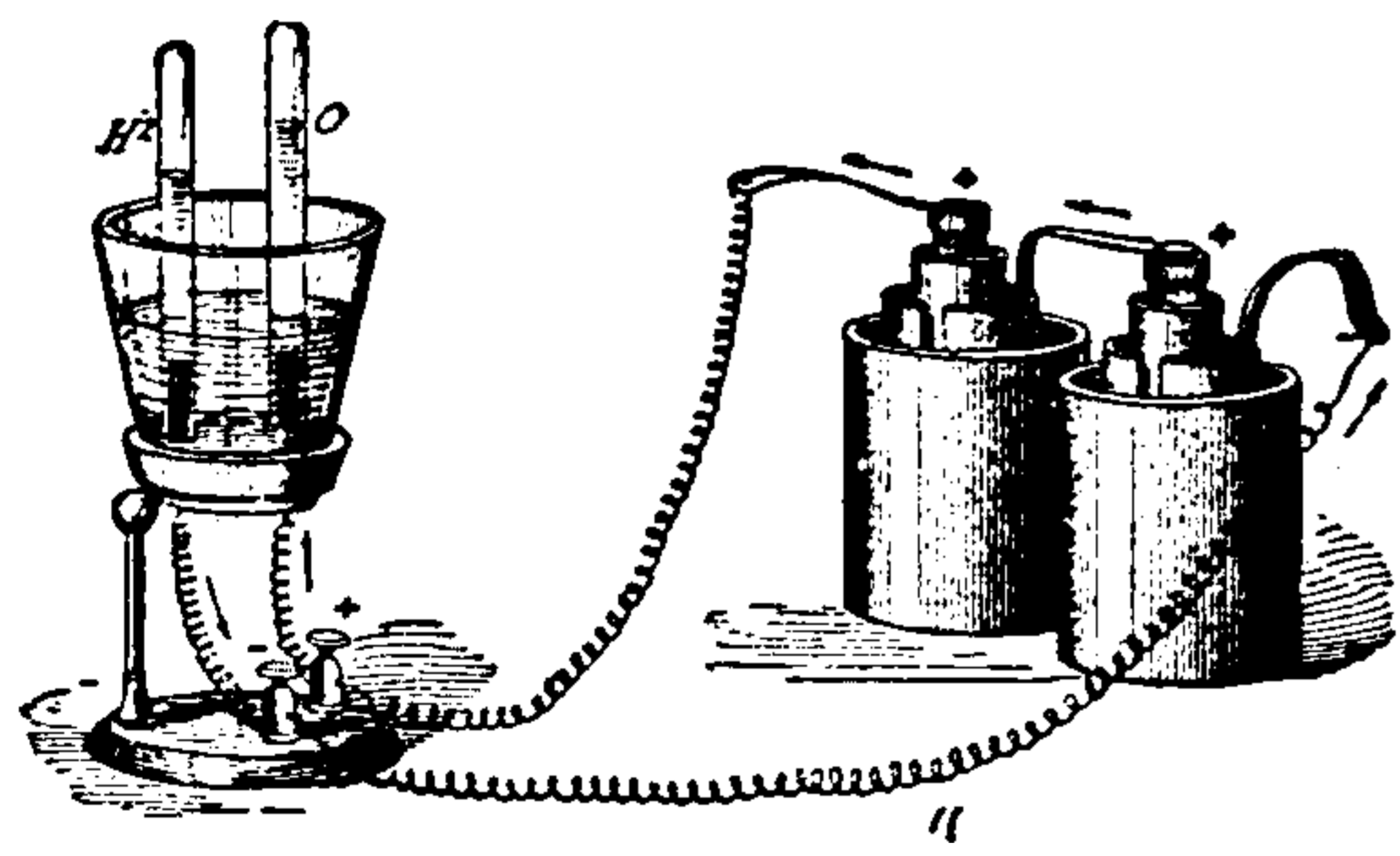
Fig. 562. A Sulphuric Acid Voltmeter.
