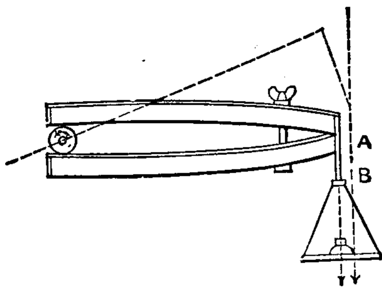
Fig. 70. Prony Brake.
