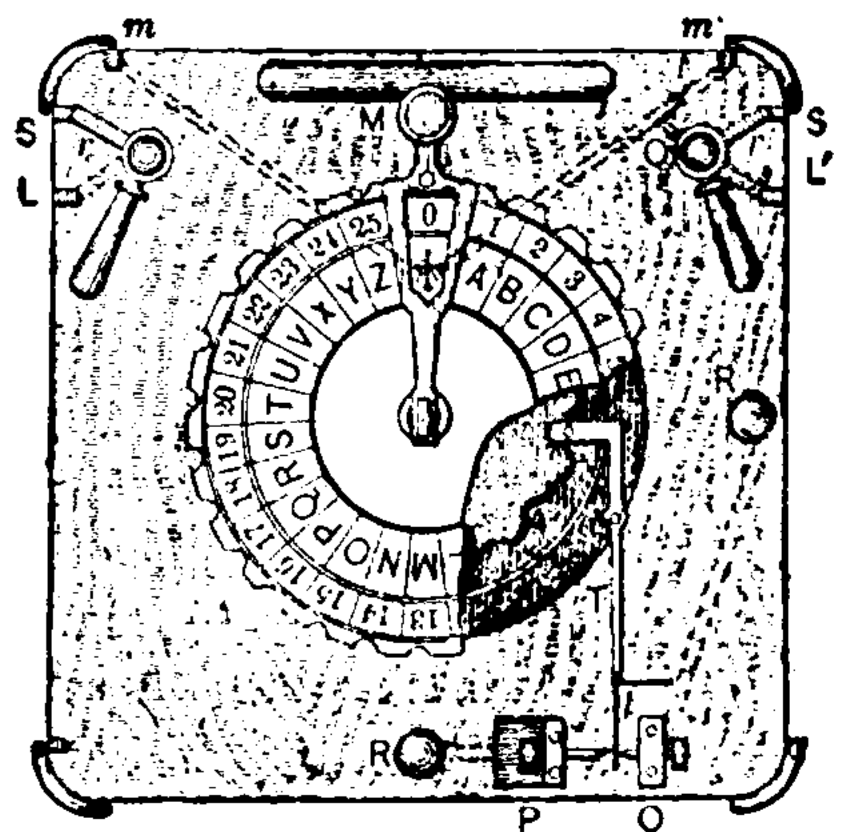
Fig. 542. Breguet's Manipulator.
