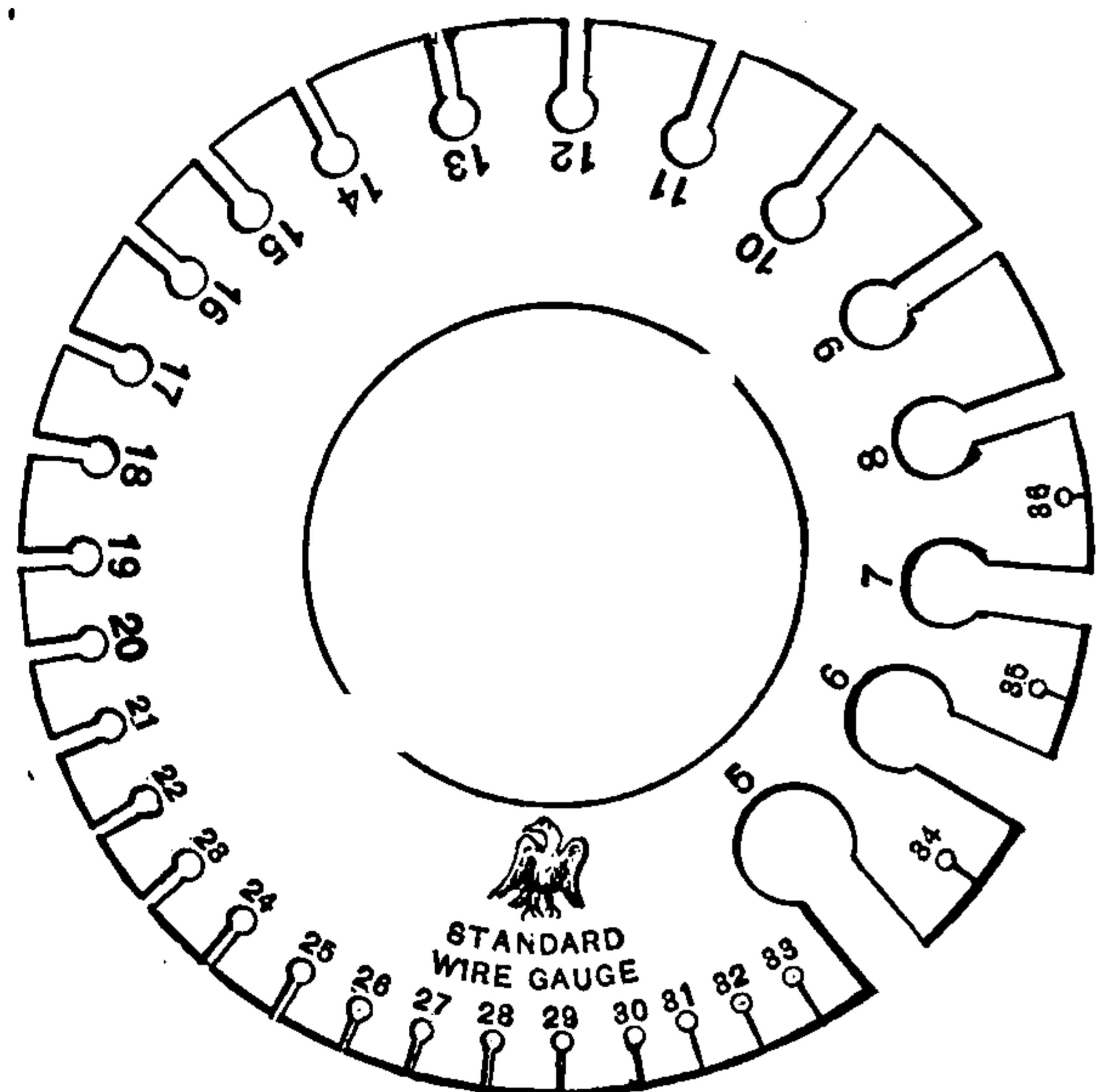
Fig. 284. Round Wire Gauge.
