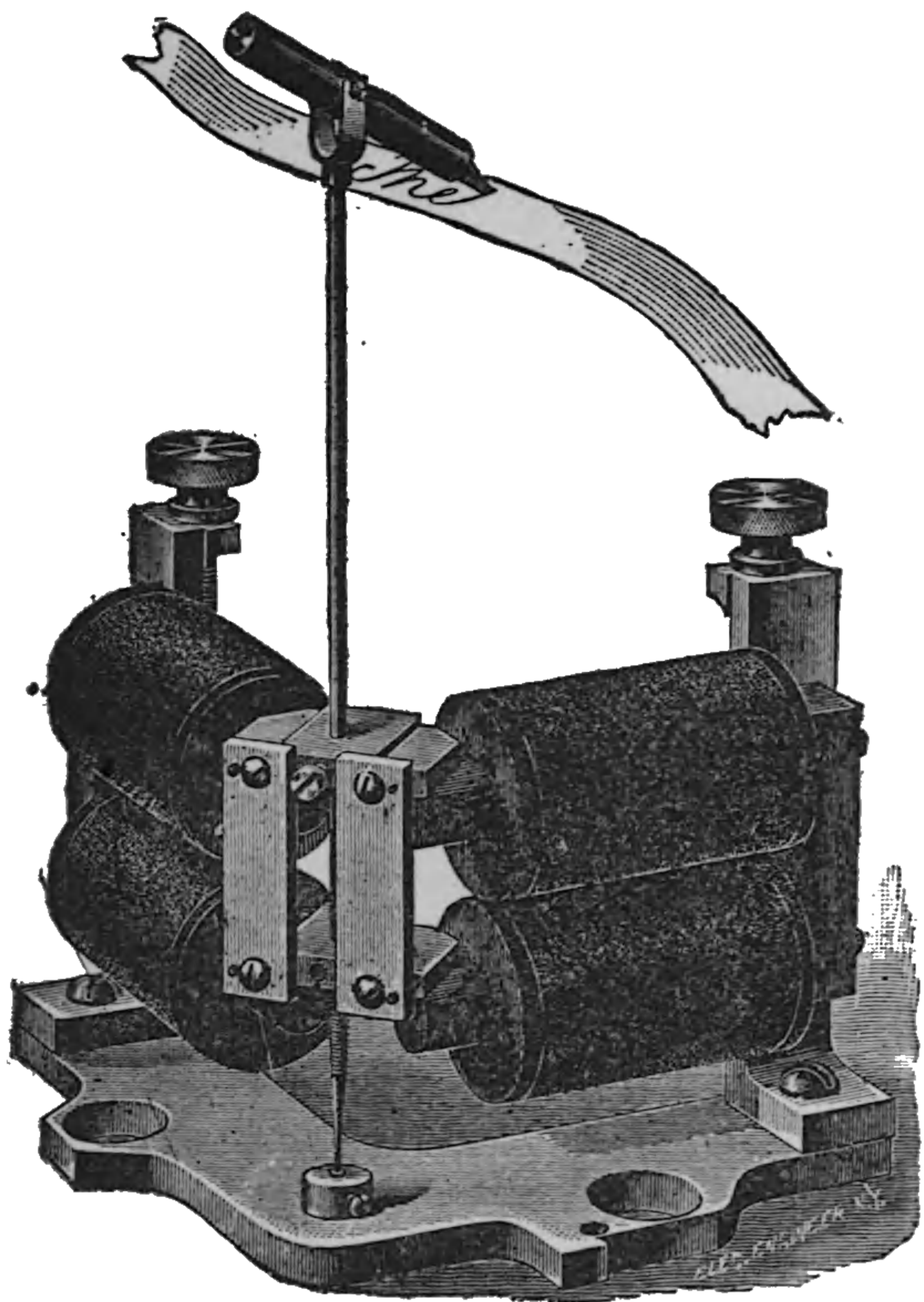
Fig. 548. Receiver of Writing Telegraph.
