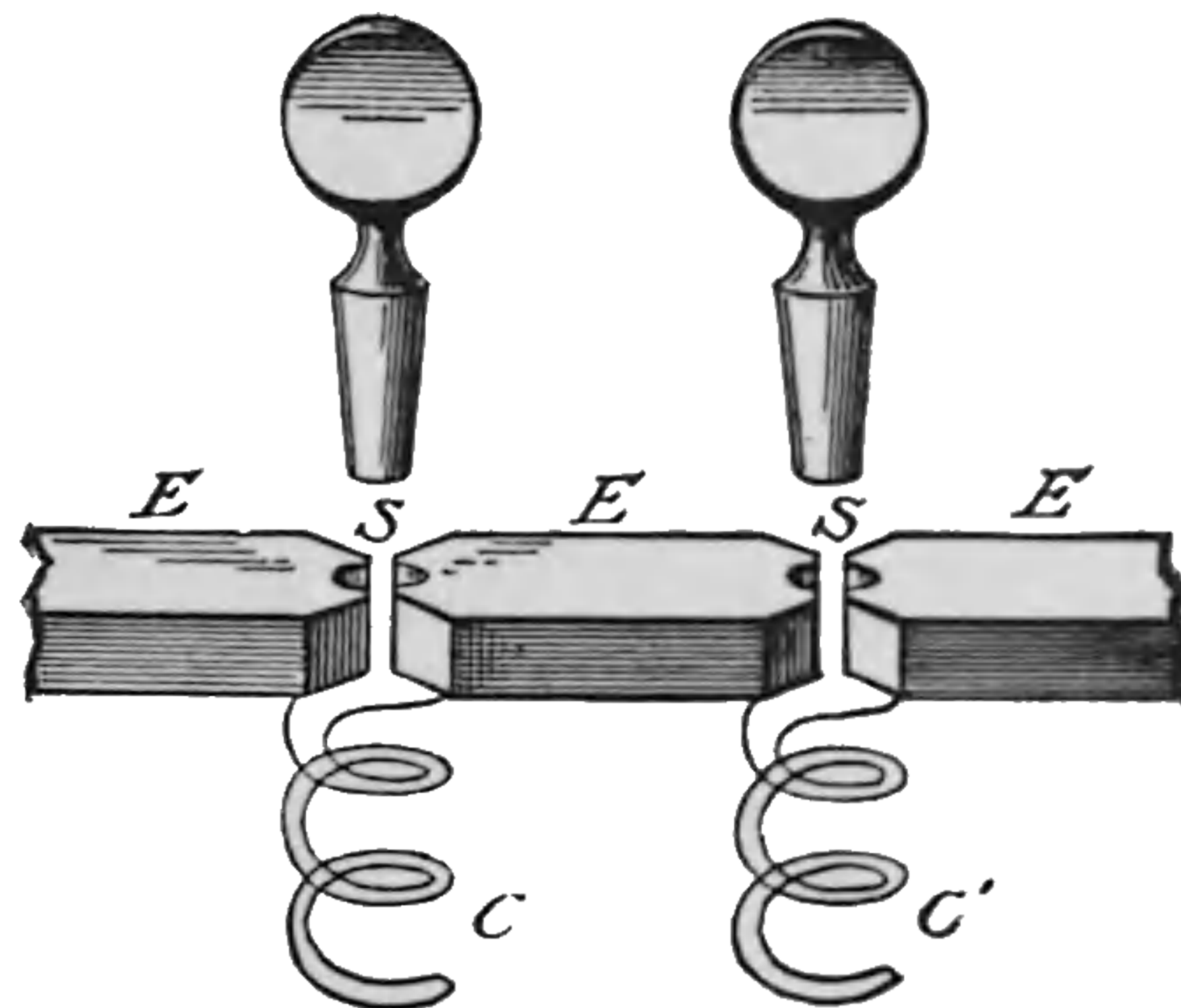
Fig. 76. Resistance Coils.
