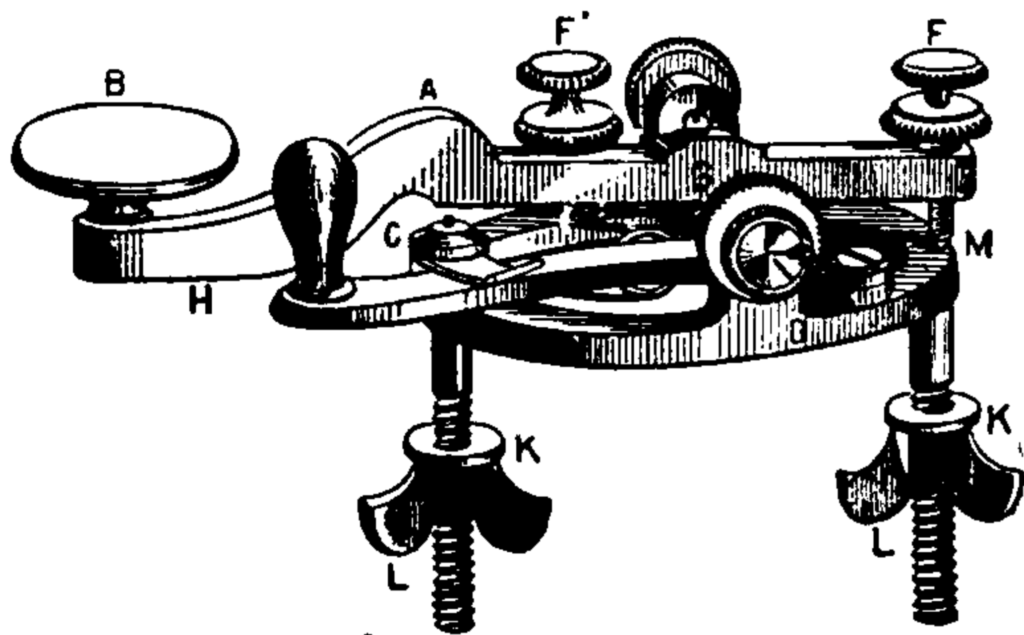
Fig. 531. Telegraphic Key.
