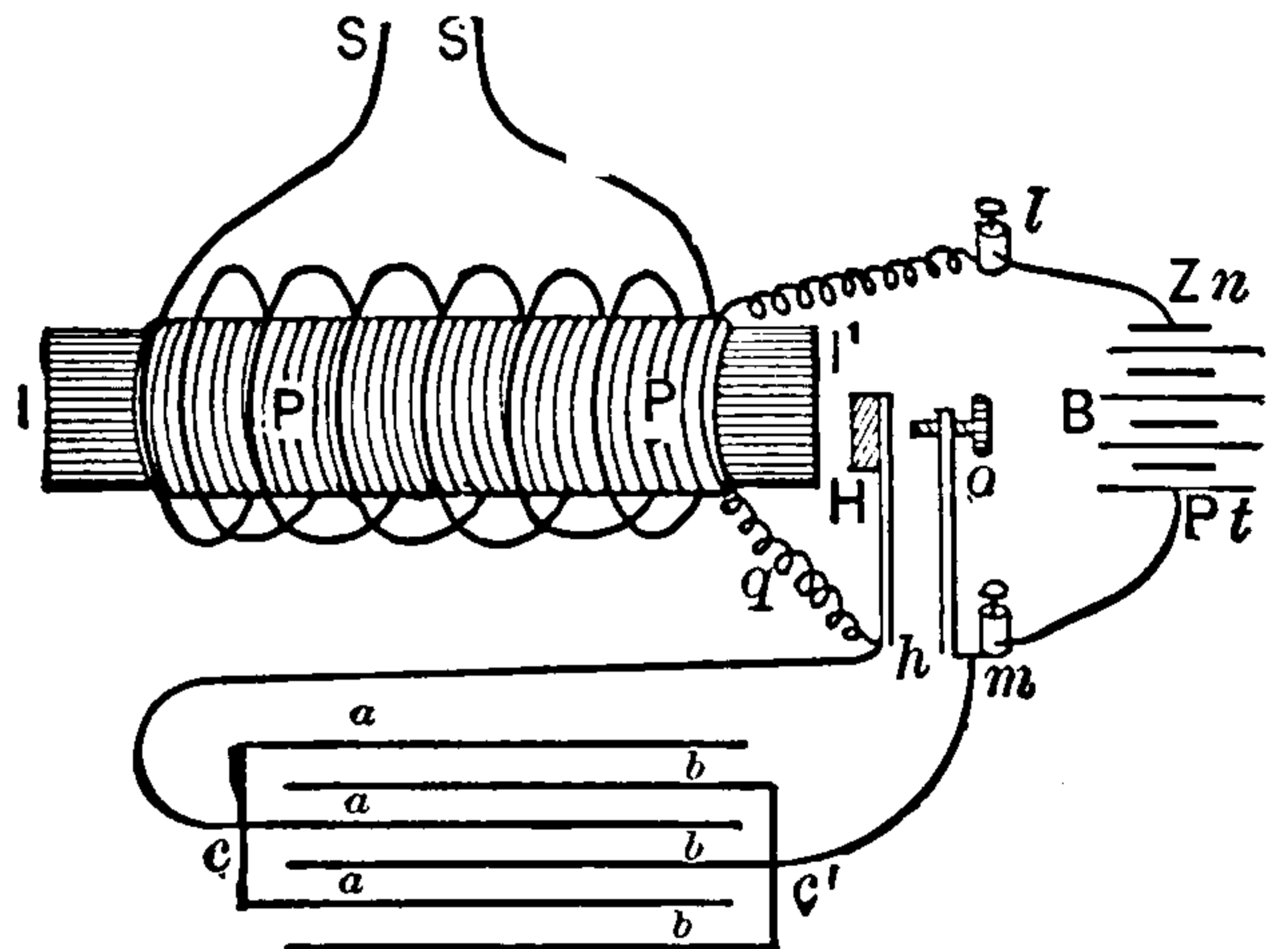
Fig. 143. Circuit Connections of Induction Coil.
