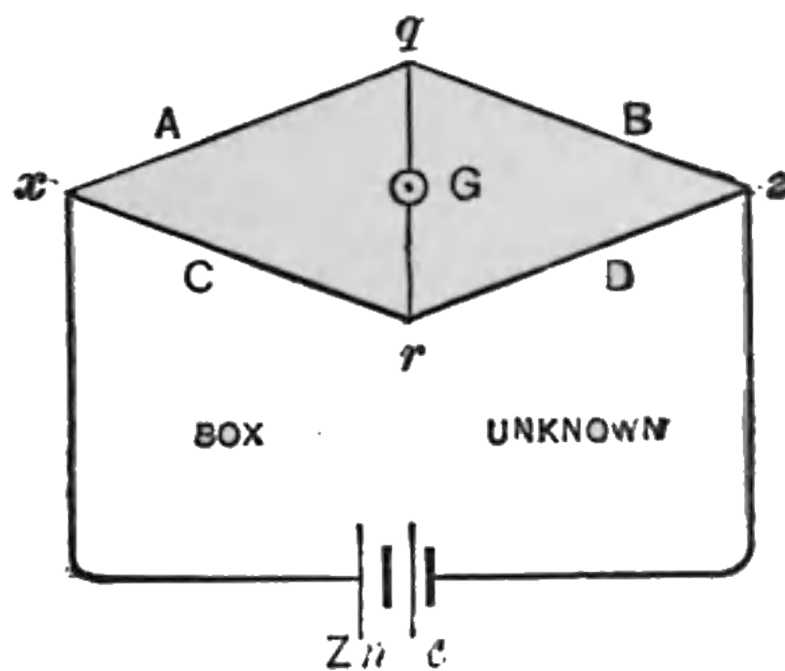
Fig. 77. Electric Balance.
