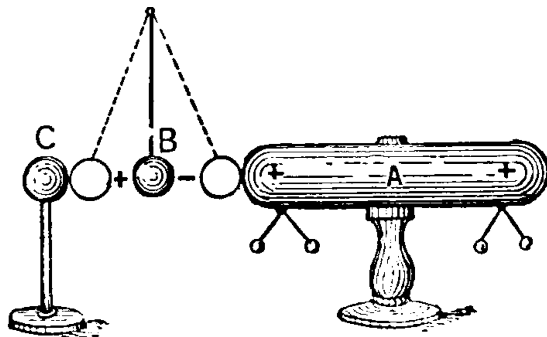
Fig. 306. Induction Precedes Attraction.
