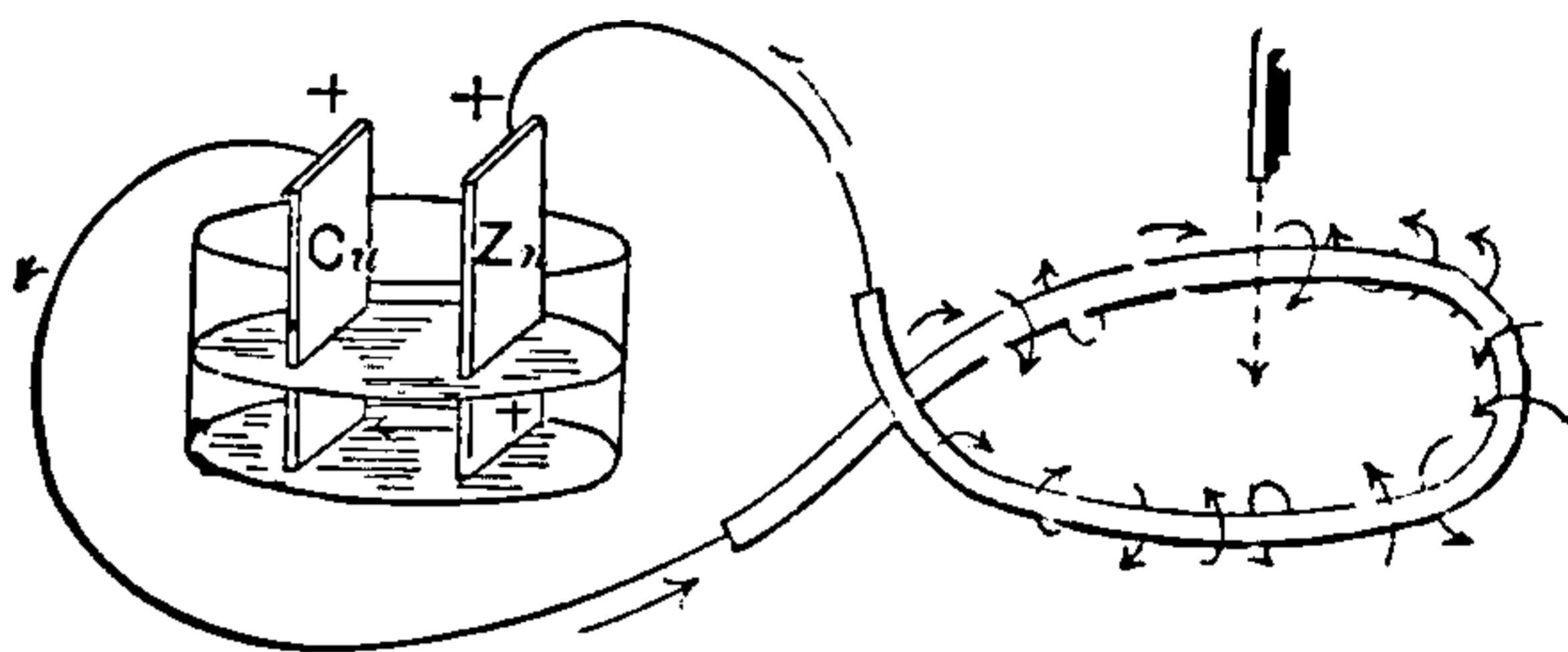
Fig. 373. Direction of Lines of Force.
