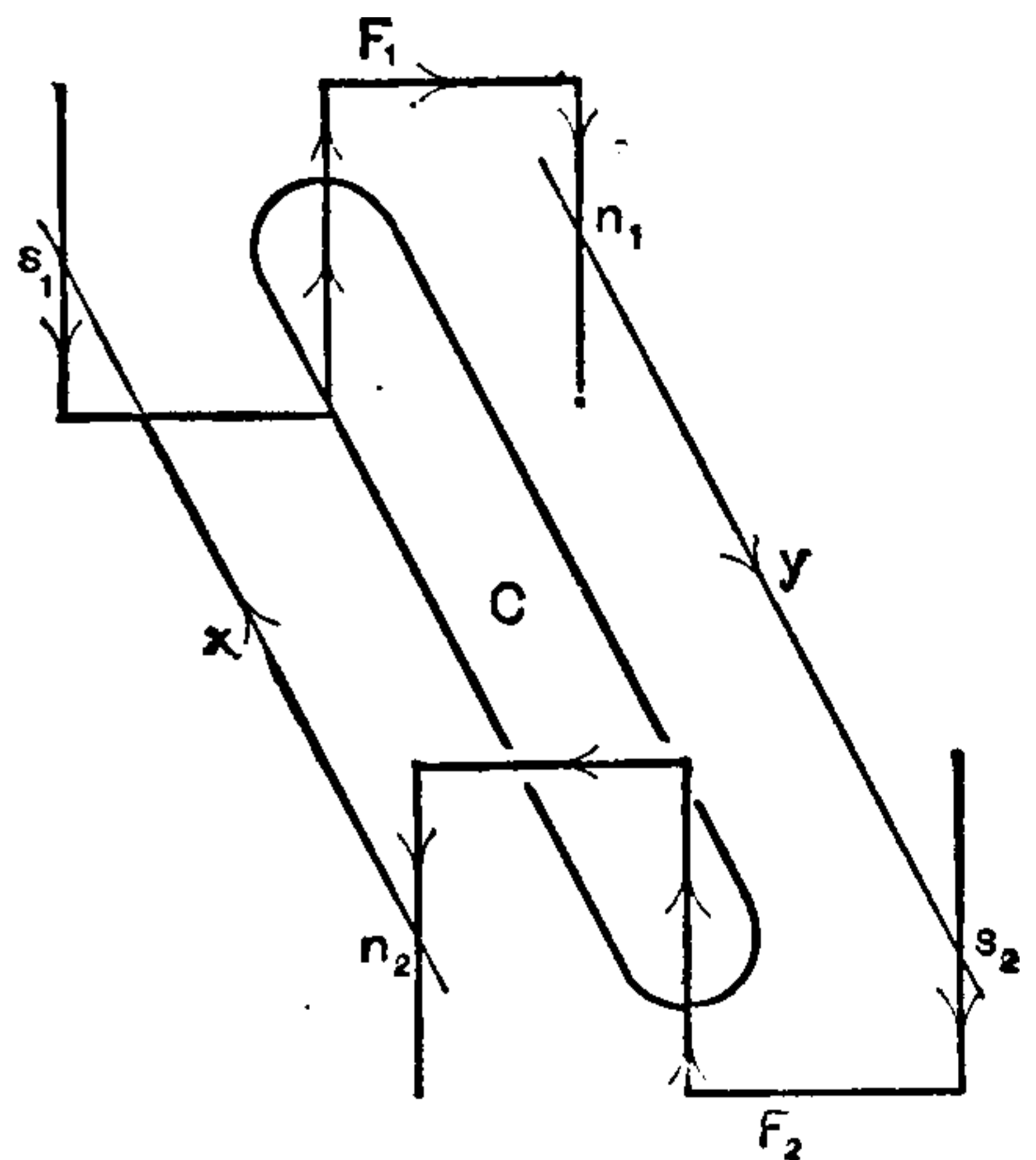
Fig. 390. Eickemeyer's Differential Magnetometer.
