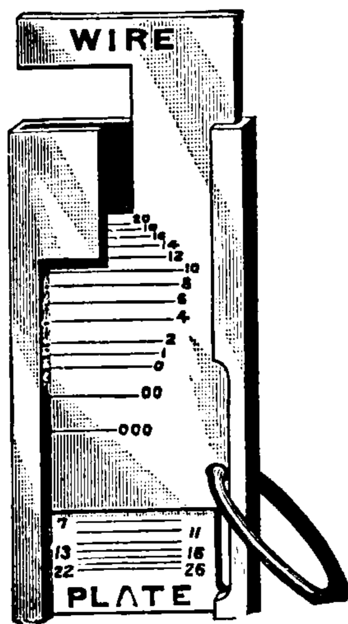
Fig 285. Wire and Plate Gauge.
