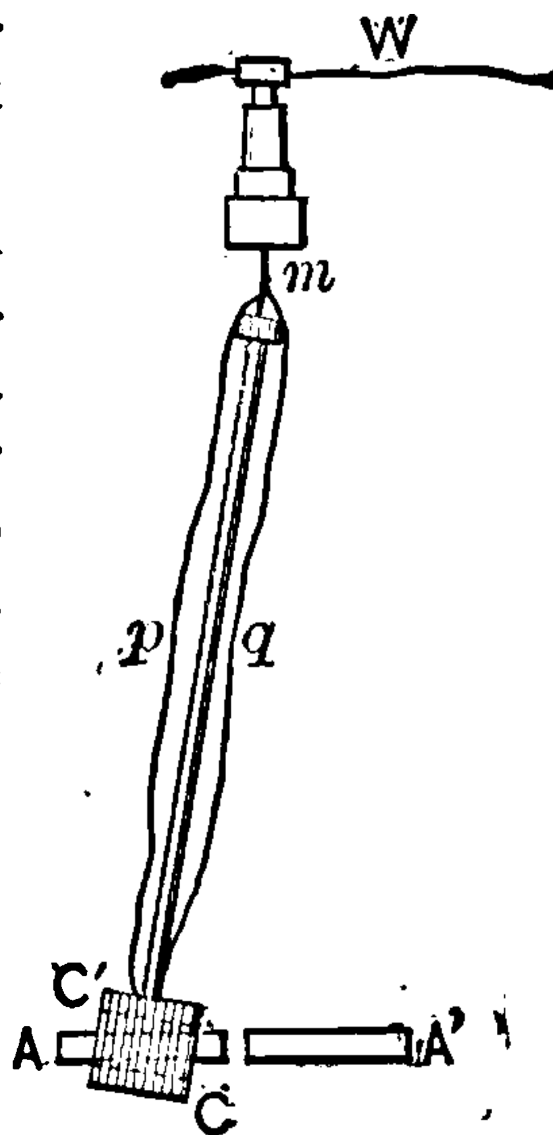
Fig. 138. Controlled Clock.
