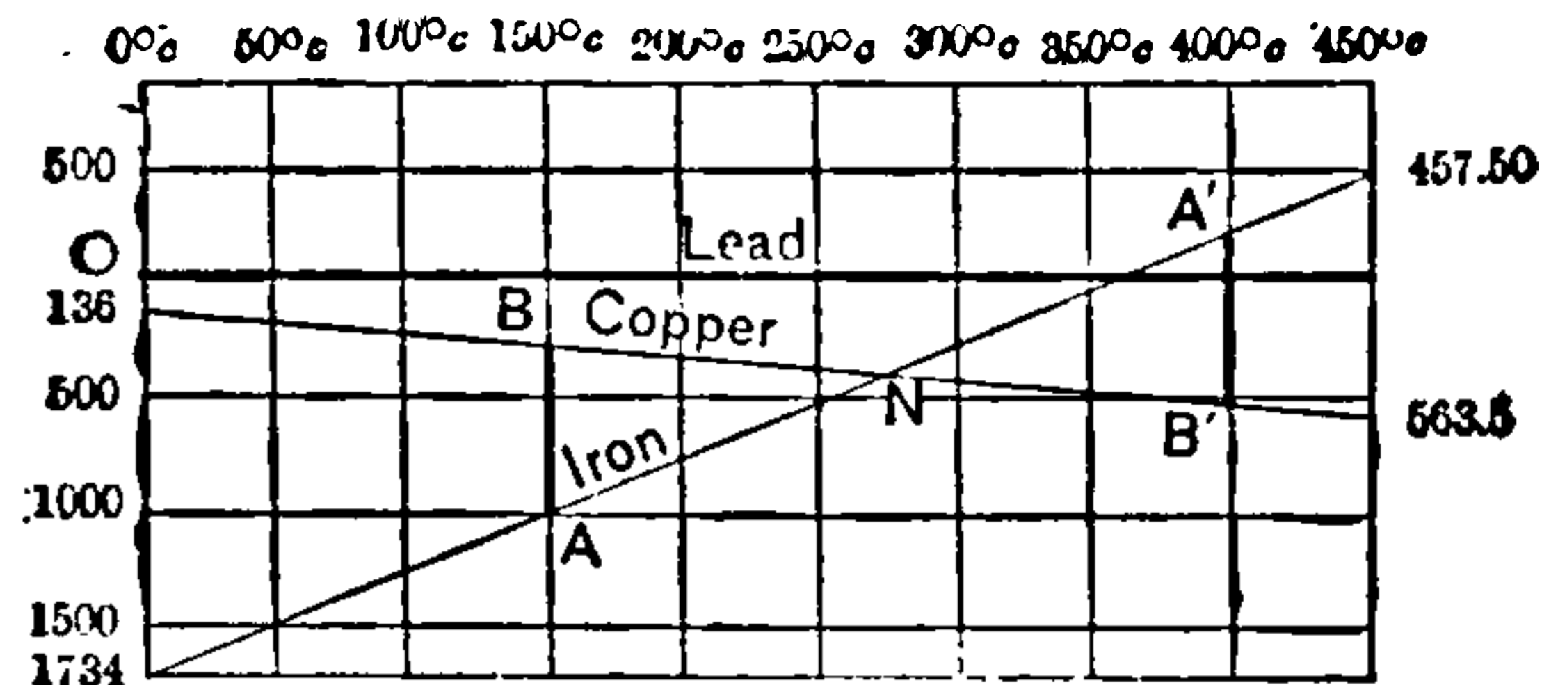
Fig. 198. Thermo-Electric Diagram.
