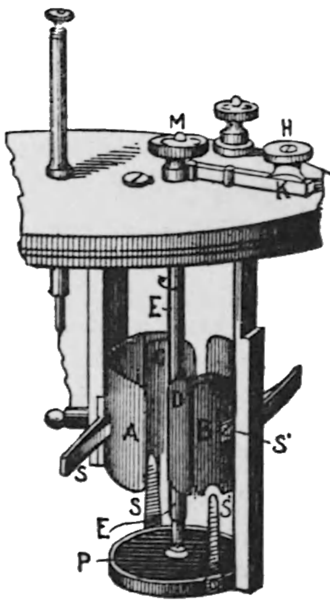
Fig. 486. The Replenisher.
