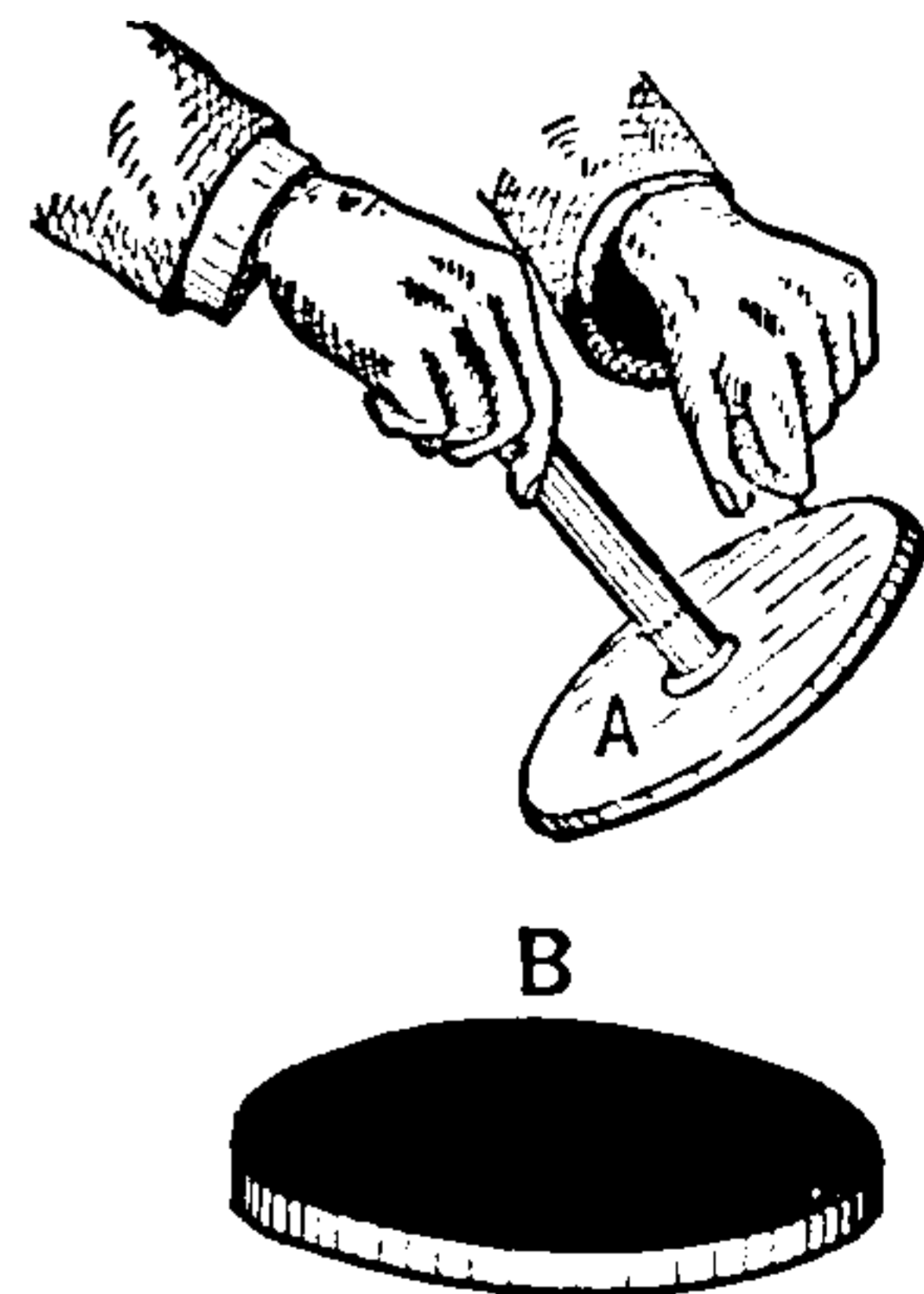
Fig. 236. Electrophorus, Discharging.
