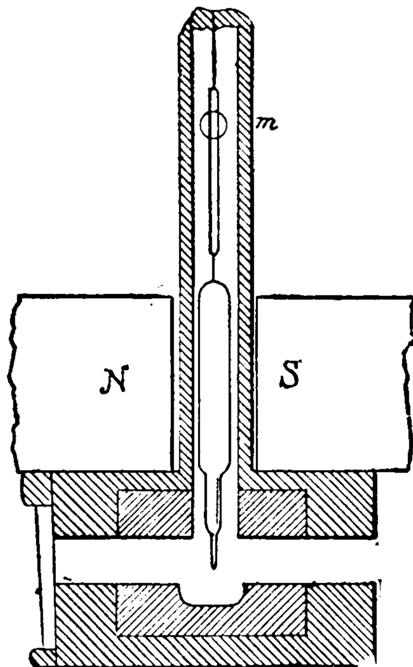
Fig. 457. Boys' Radio-Micrometer.
