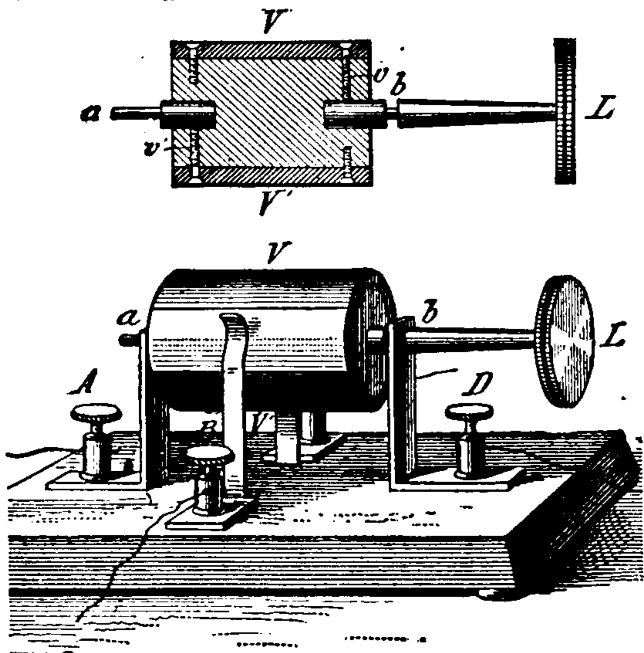
Fig. 160. Ruhmkorff's Commutator.
