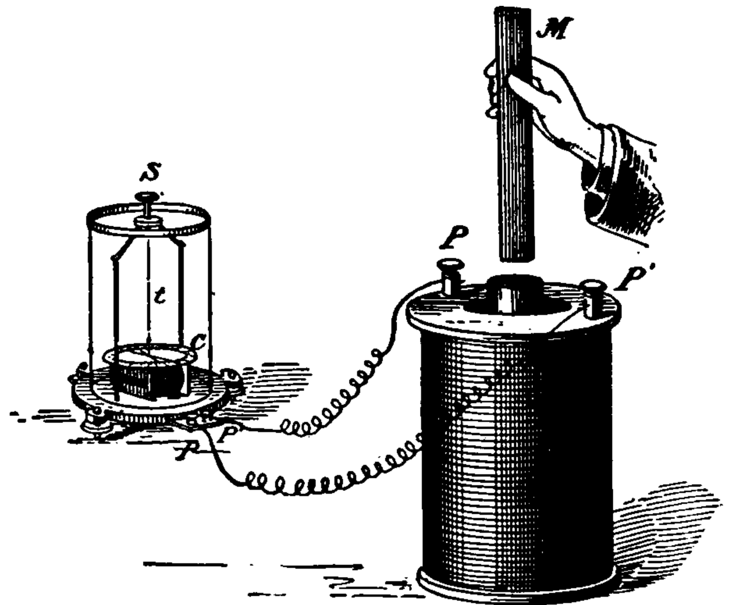
Fig. 302. Magneto-Electric Induction.
