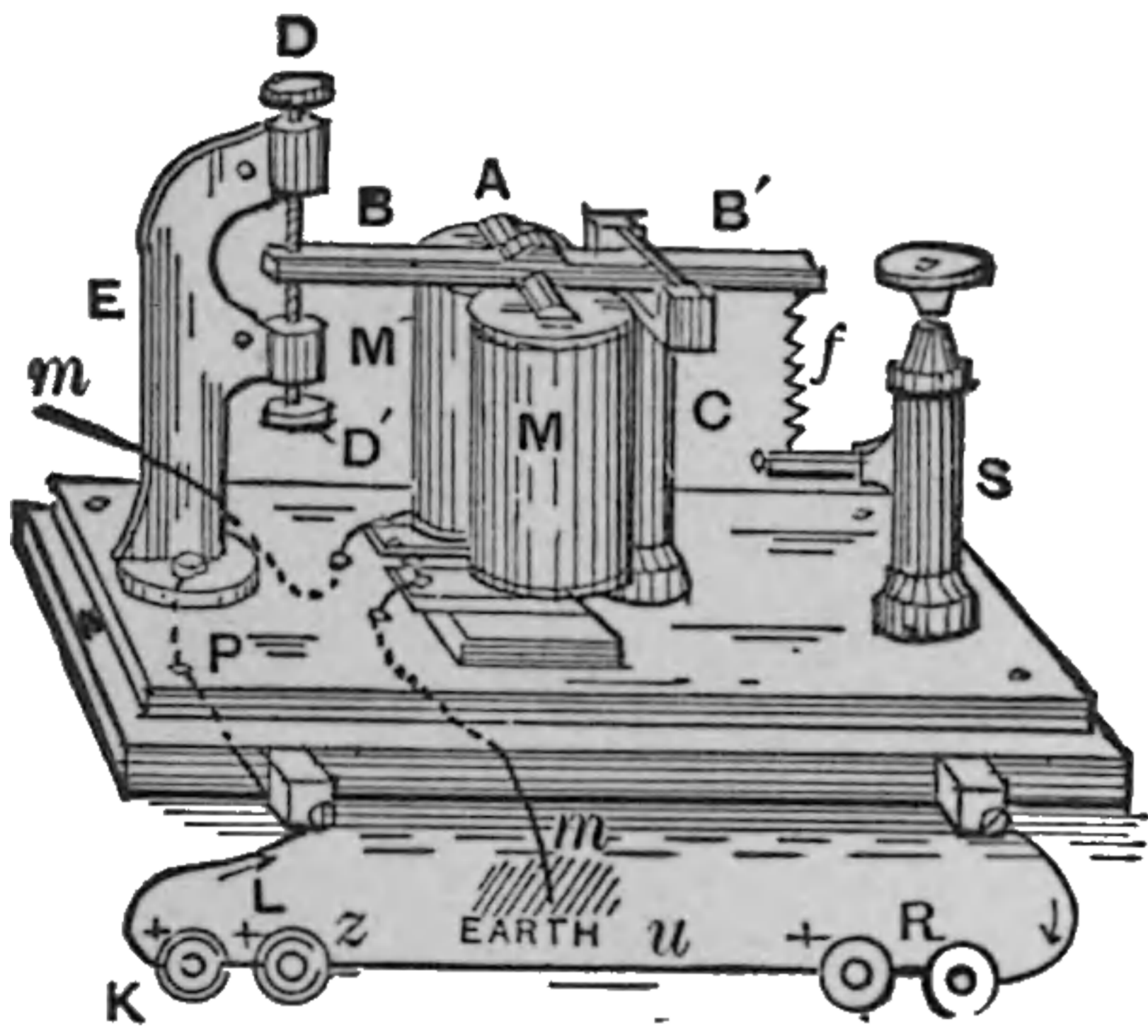
Fig. 478. Telegraphic Relay, German Pattern.
