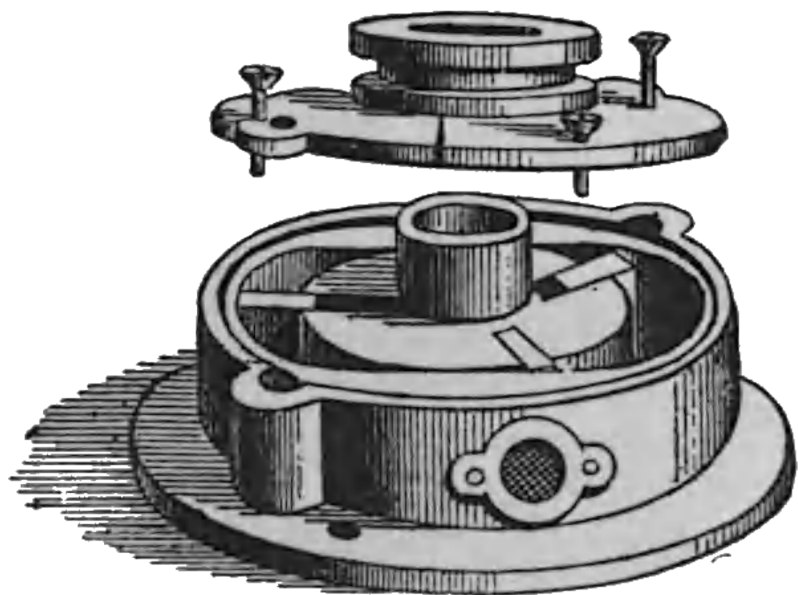
Fig. 5. The Thomson Blower.
