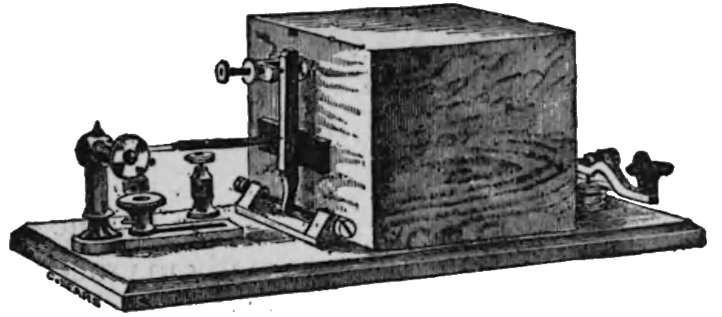
Fig. 479. Box-Sounding Relay
