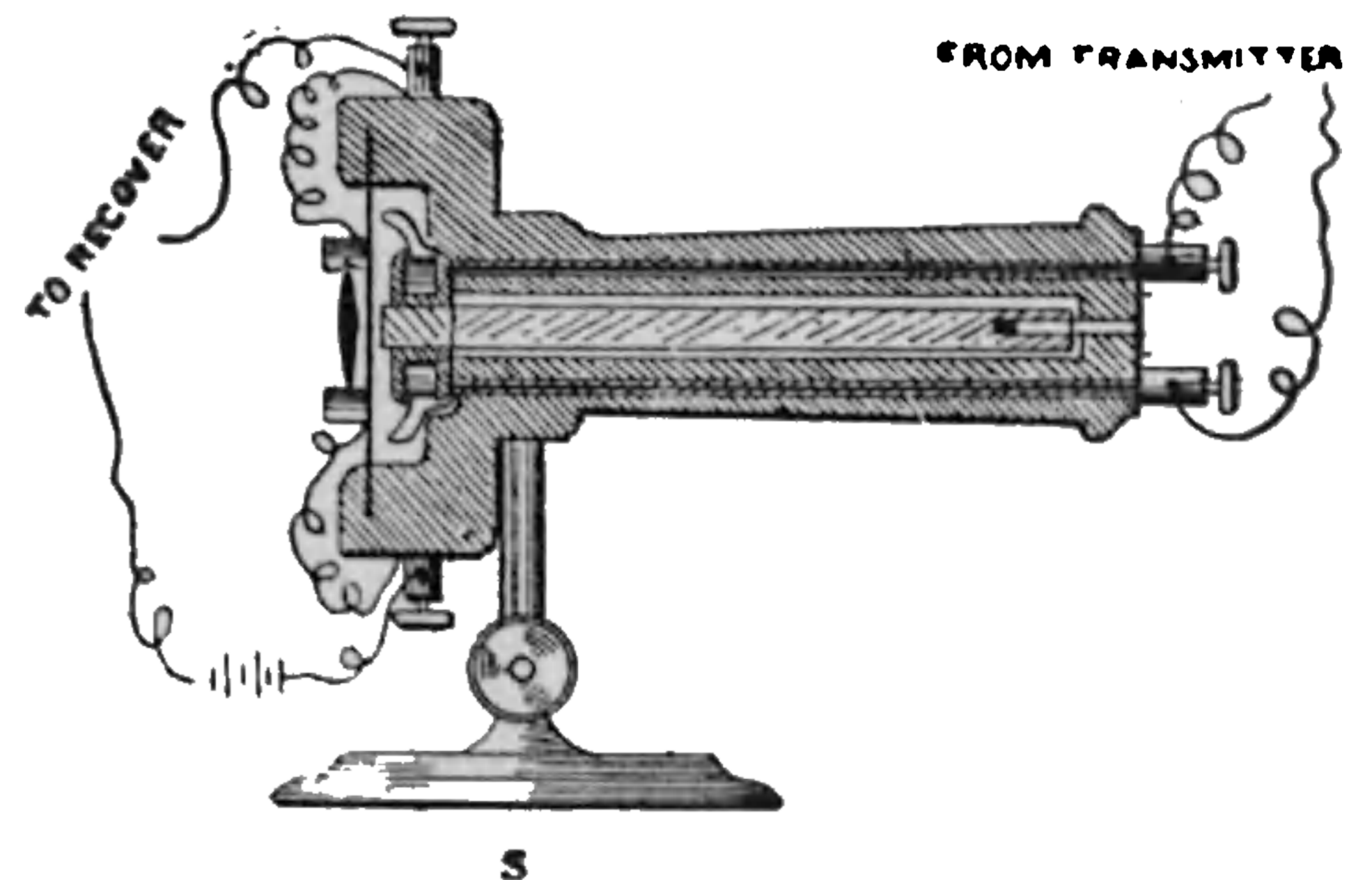
Fig. 481. Microphone Relay.
