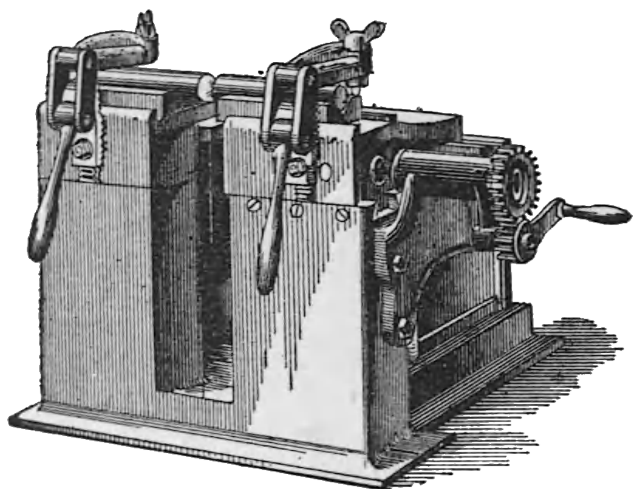
Fig. 567. The Thomson Indirect Welder.
