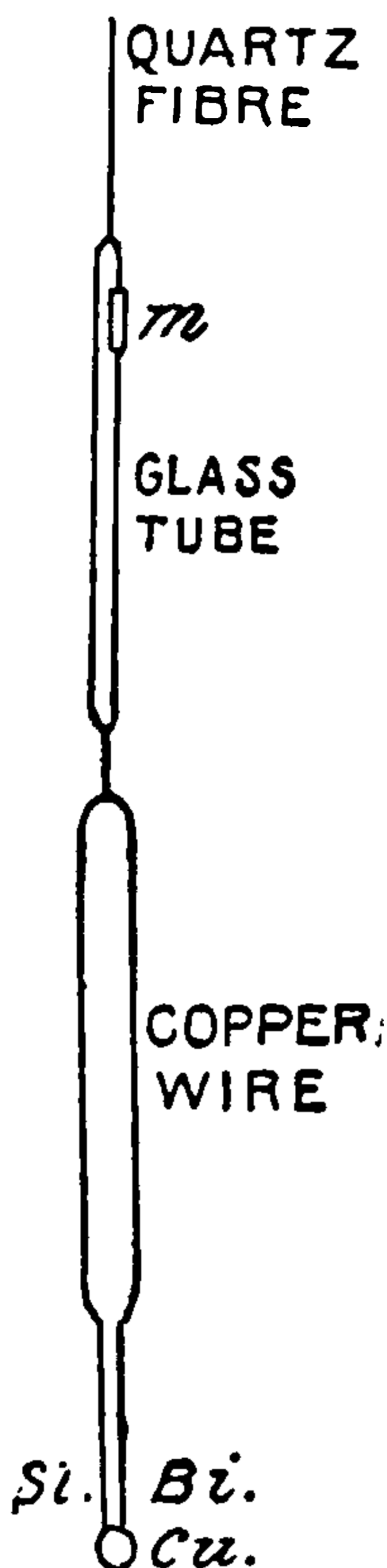
Fig. 458. Boys' Radio-Micrometer.
