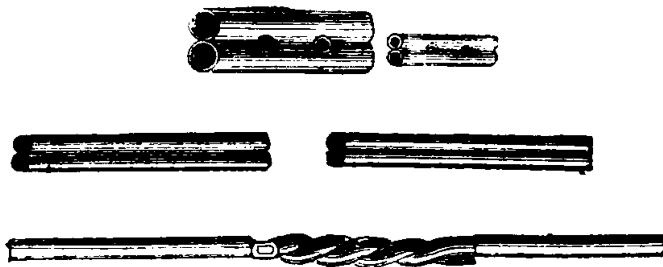
Fig. 320. McIntire's Parallel Sleeve Joint.
