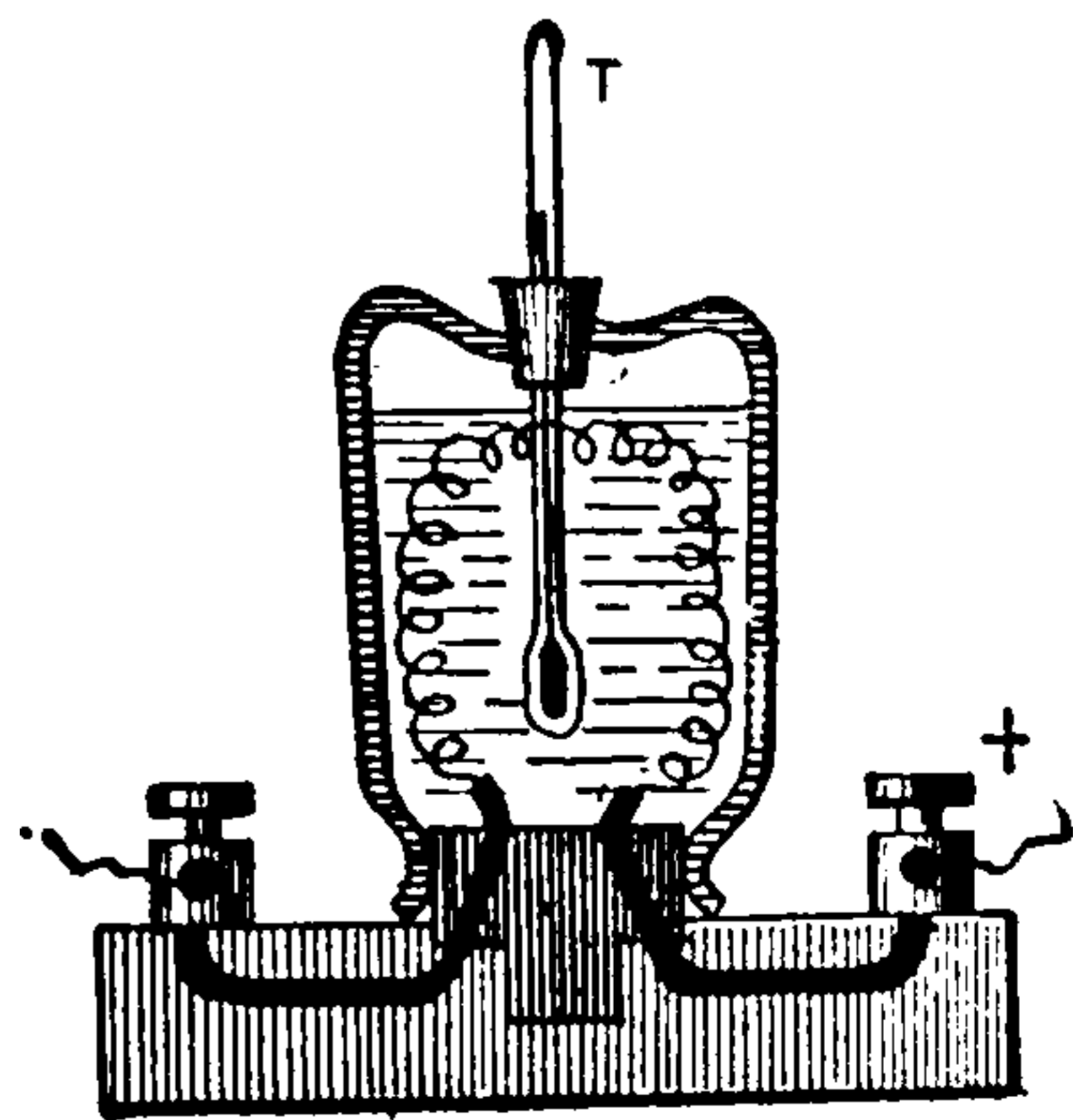
Fig. 97. Electric Calorimeter.
