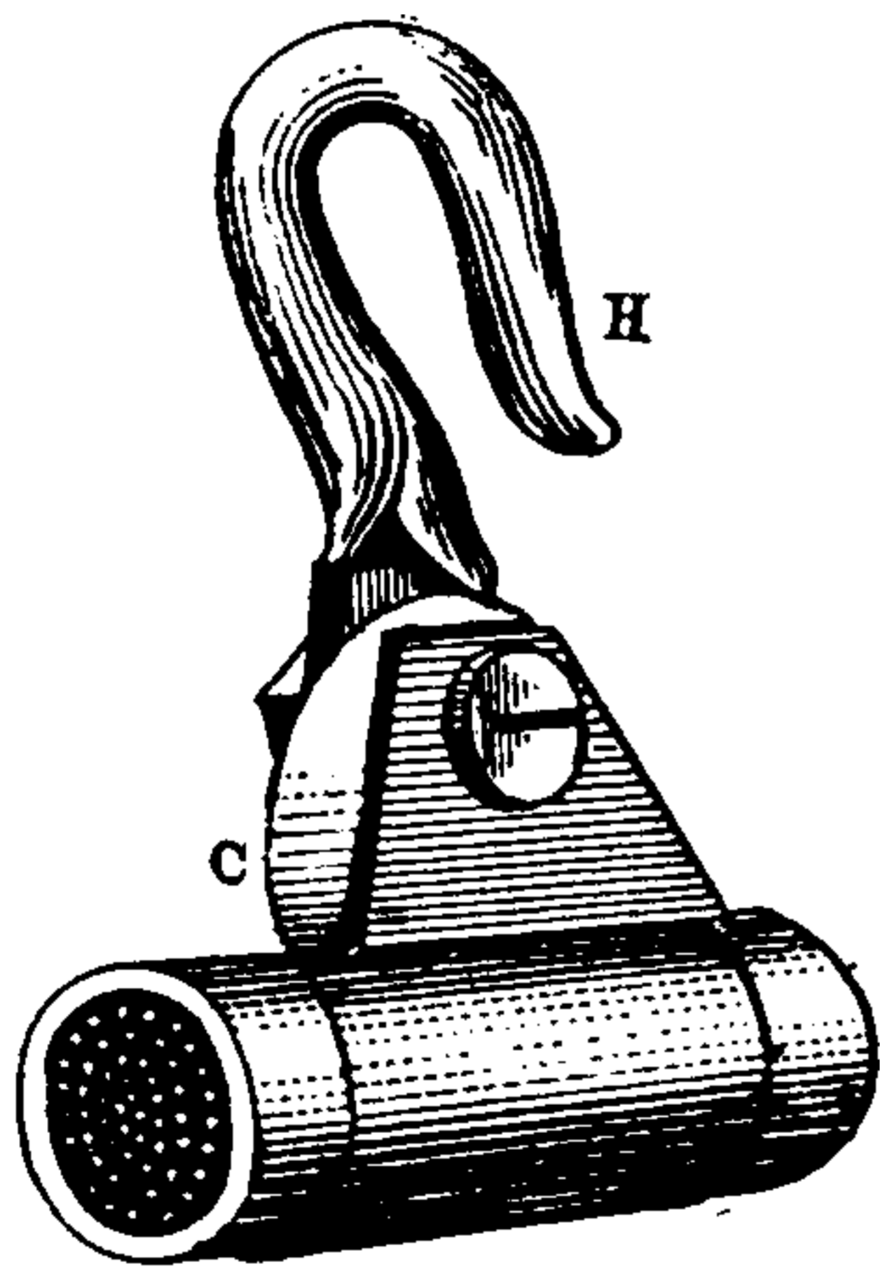
Fig. 290. Cable Hanger.
