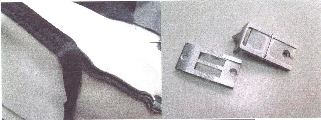
FCS 00054 Needle plate for tape attachment plus open stitch guide for PLC 1660 / PLC 1660L (Specify needle gauge and width of the tape)
