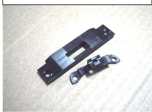
FCS 00006 Needle plate & feed dog with a height of 3mm (LU2210)
