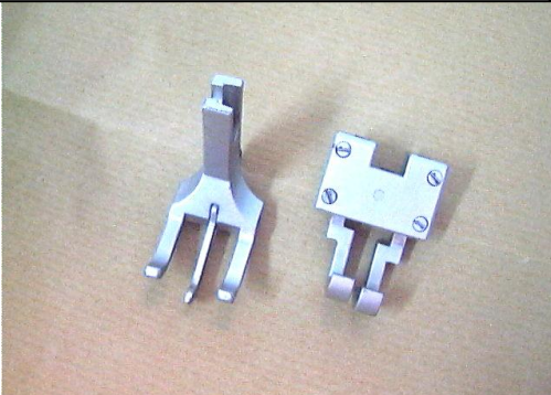
FCS 00016 Compensating presser foot PLC1660 (specify needle gauge)
