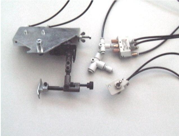
FCS 00063 Pneumatic Base For Micrometric Guide with 2 Quick Adjustable Positions LU 2210/2260
