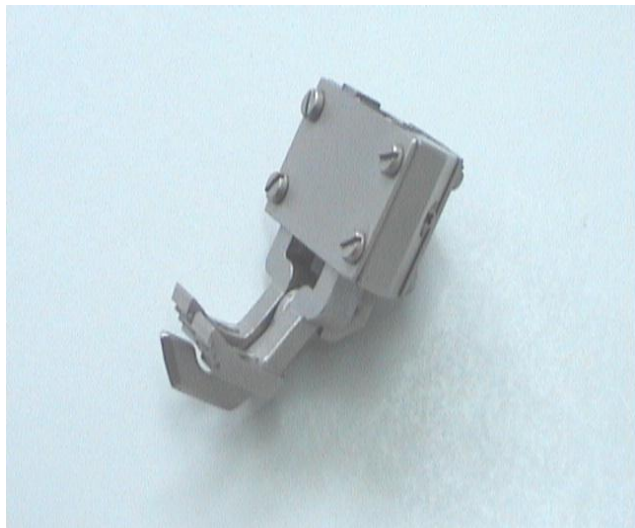
FCS 00088 Compensating Foot with Narrow Middle Guide LU-2260 / PLC-1760
