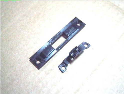
FCS 00005 Needle plate & feed dog with 3mm higher in center (LU2210)
