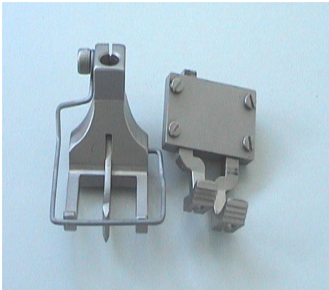
FCS 00075 Compensating Footh PLC-1760 Specify Needle Gauge
