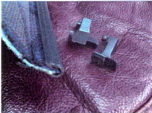
FCS 00050 Complete presser foots for plastics LU 2210 Ref: 2696/02 – 16mm
