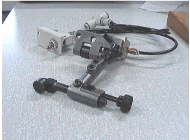
FCS 00070 PNEUMATIC UP & DOWN AJUSTABLE GUIDE
