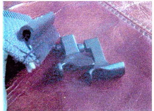
FCS 00051 Complete presser foots for plastics LU 2210 Ref: A158/01 – 8mm
