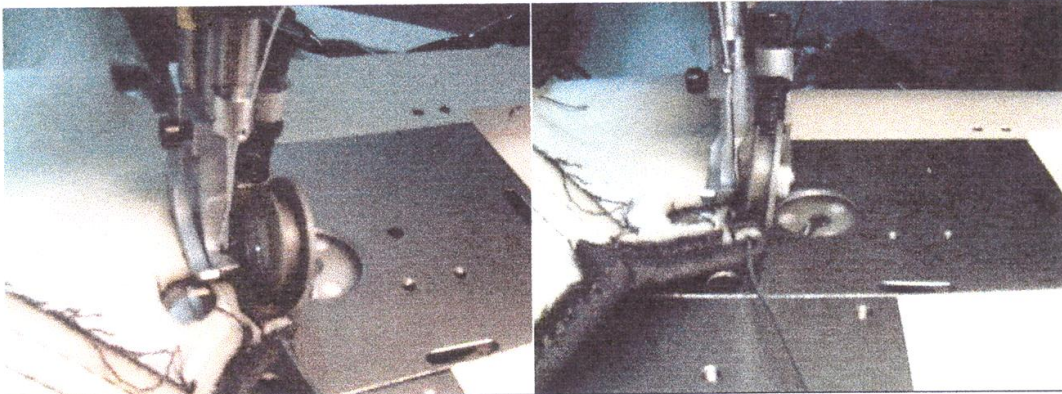
FCS 00055 ERGONOMIC PRESSER AND ROLLER GIUDE FOR SEWING WIRE ON EDGE SEAMS LU 2210
