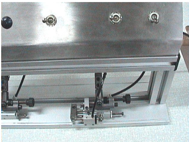
FCS 00071 PNEUMATIC 3 POSITION AJUSTABLE GUIDE WITH PNEUMATIC UP & DOWN POSITION
