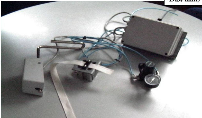
FCS 00059 Complete Presser Foot Set For Open Stitch with Pneumatic Middle Guide (Specify Edge Guide Left/Dir. Dist mm)
