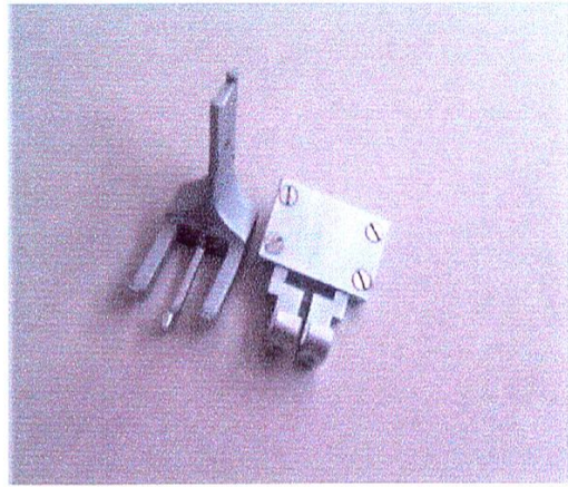
FCS 00043 Compensating presser feet LU 1560 ( specify needle gauge )
