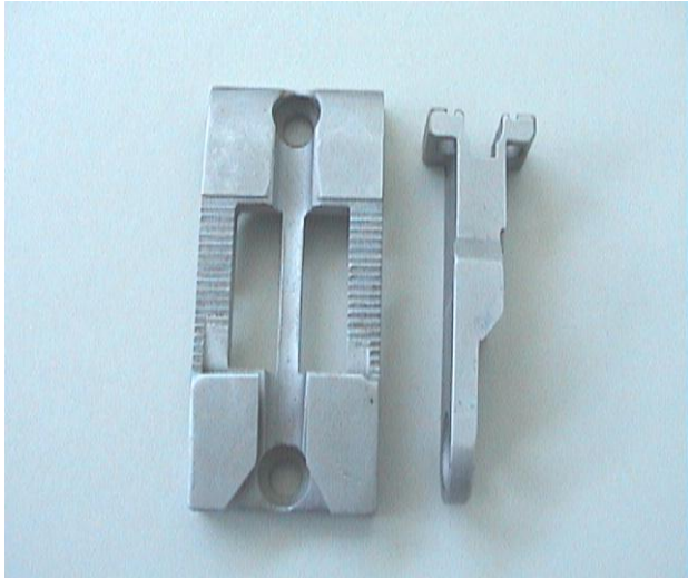
FCS 00081 Needle Plate with Narrow Feed Dog For Tape Attachment PLC-1760
