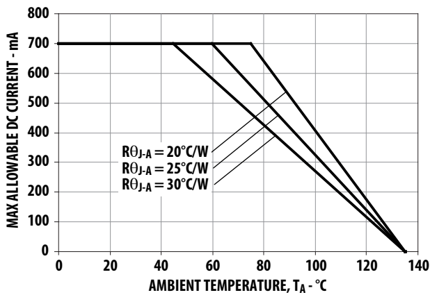
Figure 21. Maximum Forward Current vs. Ambient Temperature. Derated based on T_{JMAX} = 135^\circ\text{C} , R_{\theta J-A} = 20^\circ\text{C/W} , 25^\circ\text{C/W} and 30^\circ\text{C/W} .
