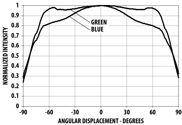
Figure 15. Radiation Pattern for Blue and Green.
