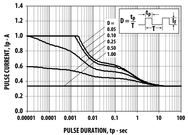
Figure 6. Maximum pulse current vs. ambient temperature. Derated based on T_A = 85^\circ\text{C} , R\theta_{J-A} = 30^\circ\text{C/W} .
