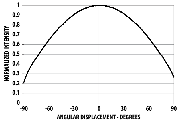
Figure 16. Radiation Pattern for Cool White and Warm White.
