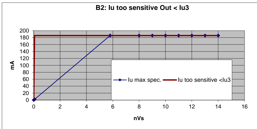
Figure 56: Reduced Size, Failure Mode B2
