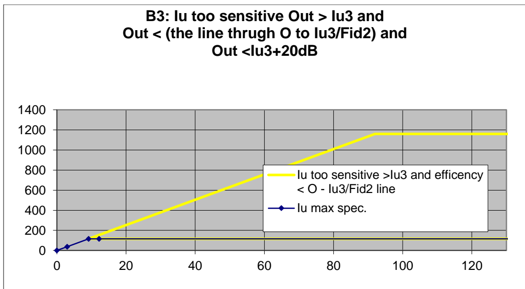
Figure 60: Standard Size, Failure Mode B3
