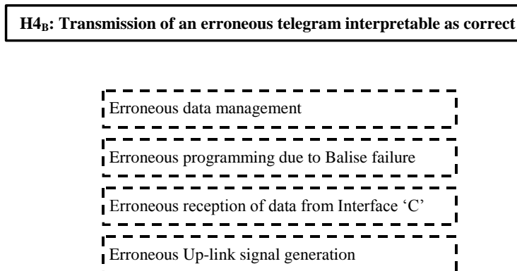
Figure 21: Erroneous telegram interpretable as correct
