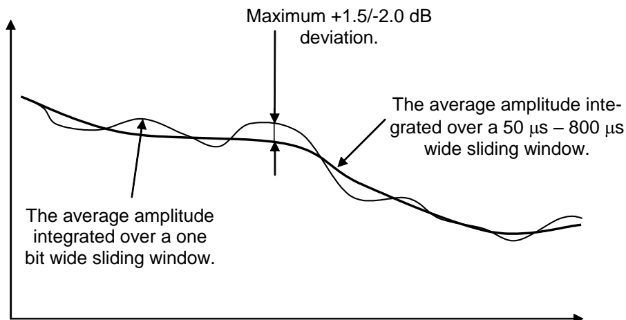
Figure 11: Amplitude jitter
