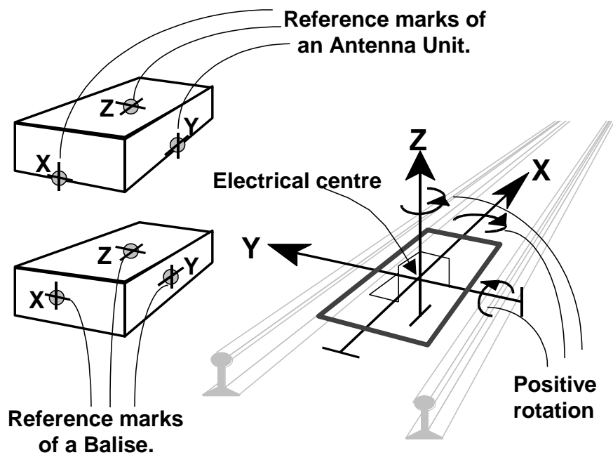
Figure 7: Reference Axes
