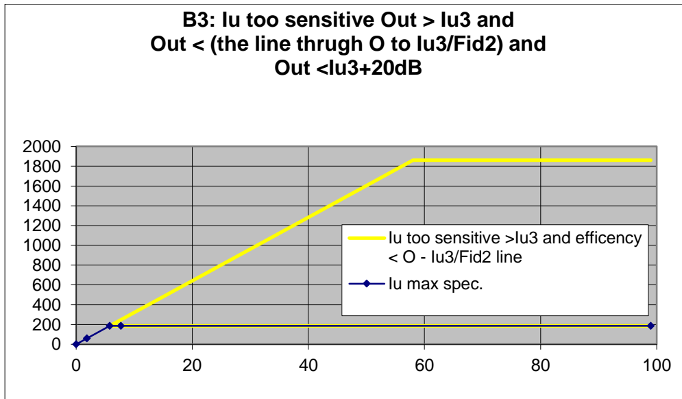
Figure 57: Reduced Size, Failure Mode B3
