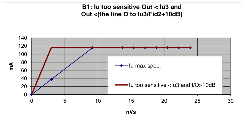
Figure 58: Standard Size, Failure Mode B1
