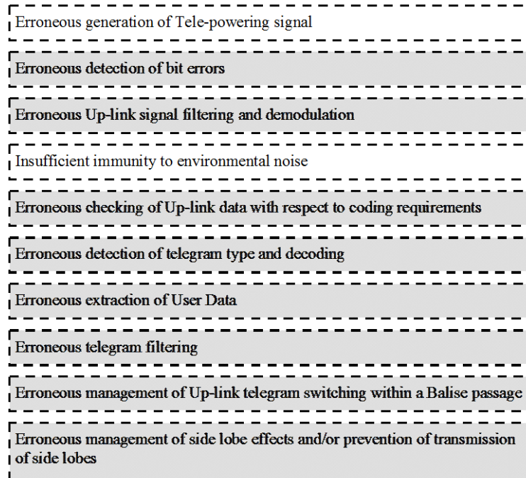
Figure 46: Loss of telegram for full performance
