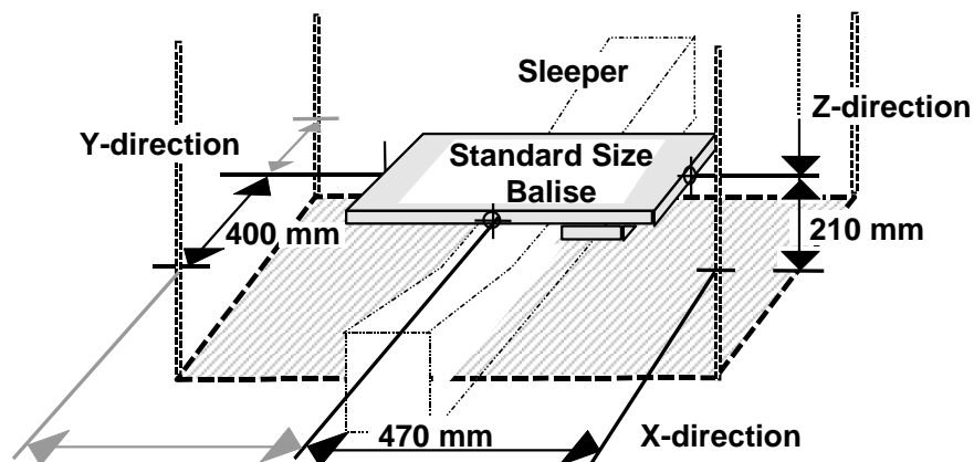
Figure 29: Metal free volume for Standard Size Balise
