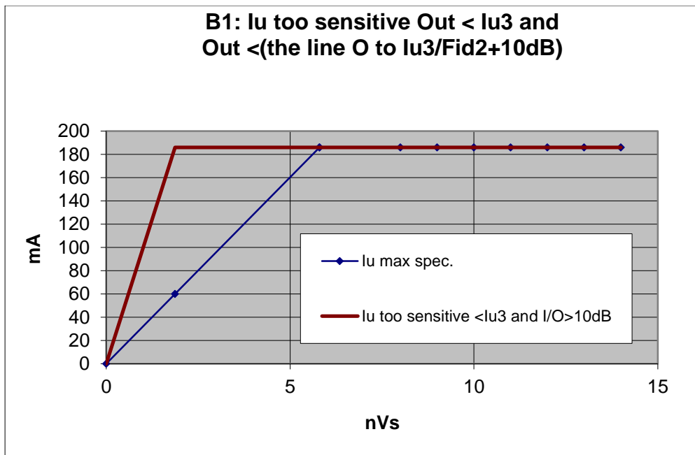
Figure 55: Reduced Size, Failure Mode B1
