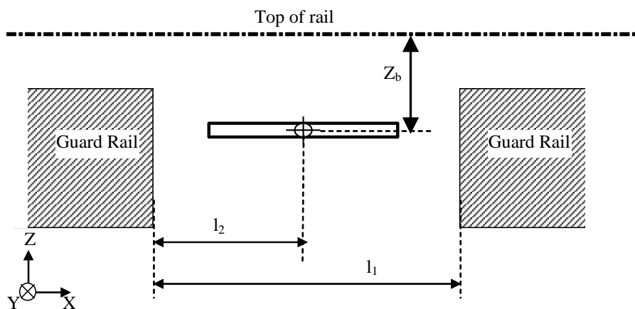
Figure 33: Centrally positioned Guard Rails
