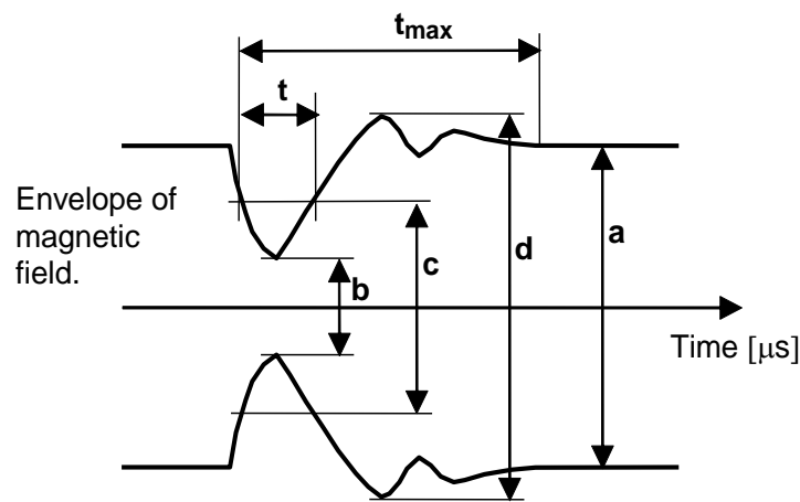
Figure 53: Definition of AM pulse parameters, toggling Tele-powering
