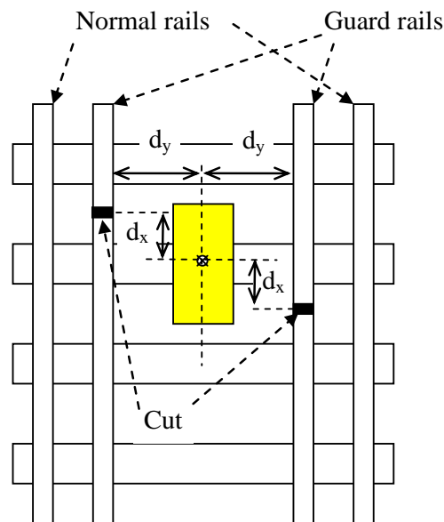
Figure 32: Laterally Displaced Guard Rails
