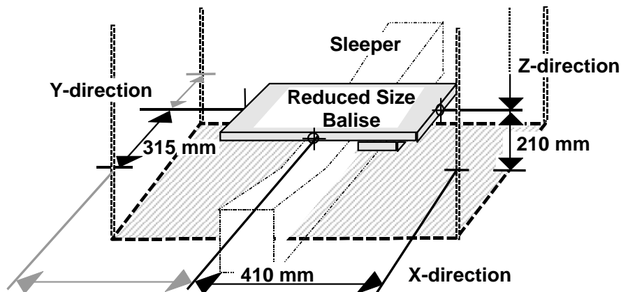
Figure 30: Metal free volume for Reduced Size Balise
