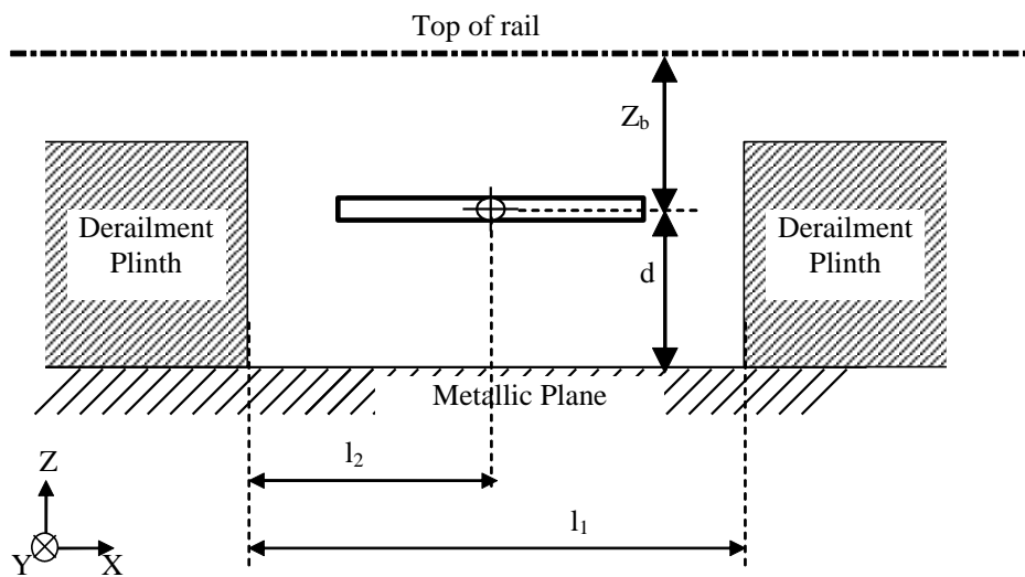
Figure 34: Derailment Plinth
