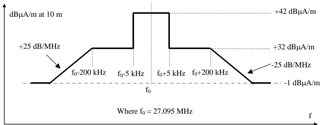
Figure 54: Requirements for interoperable mode
