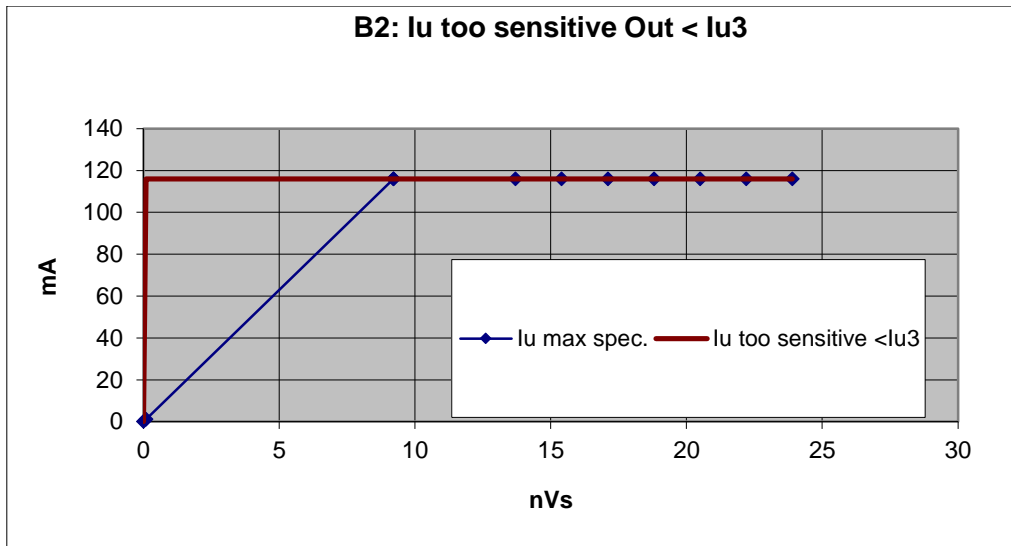
Figure 59: Standard Size, Failure Mode B2
