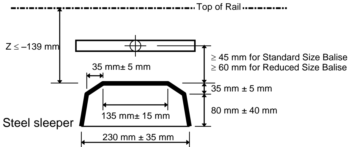
Figure 31: Balise mounted to a steel sleeper
