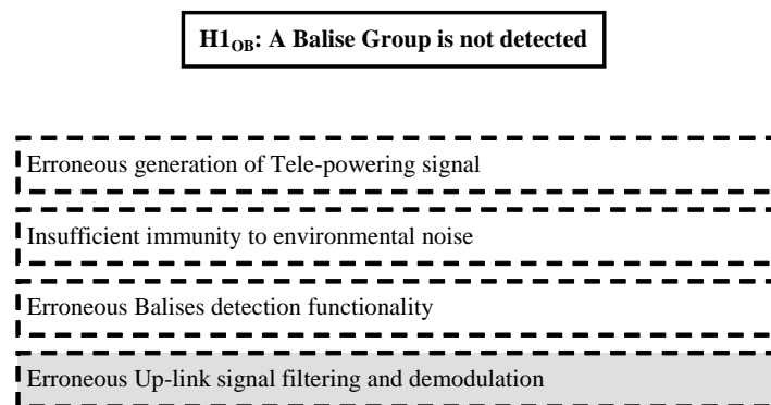
Figure 42: Balise Group Detection
