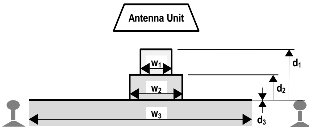
Figure 51: Metal masses in the track
