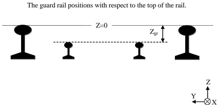
Balise positioning and gap in guard rails
