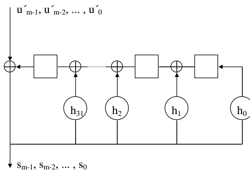
Figure 5: Scrambling
