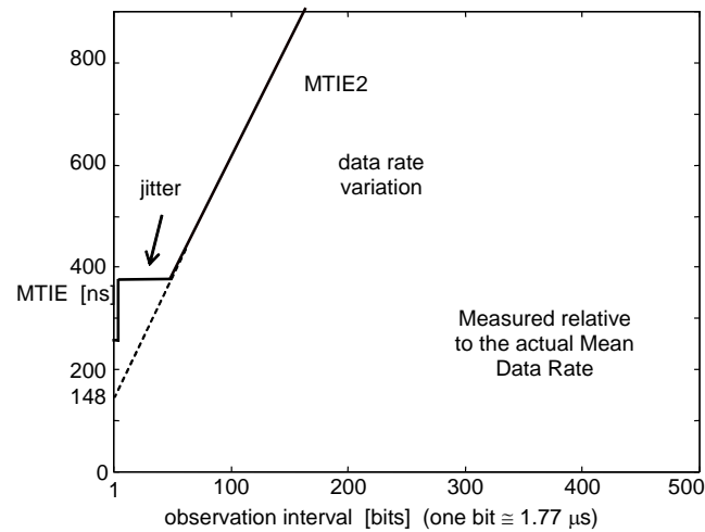
Figure 10: MTIE requirement 2
