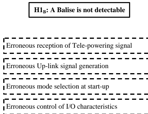
Figure 20: Balise Detectability
