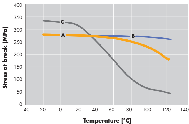
Strength of Grivory HT in comparison to die-cast alloys
