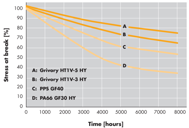
Resistance to hot water, 110°C
