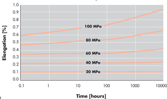
Creep curves Grivory HT2V-5H at 23°C / 50 % rel. humidity
