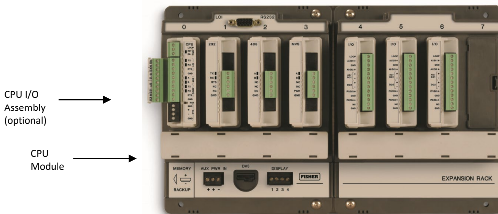
FloBoss 107 with optional Expansion Rack
