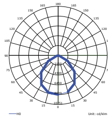
LUMINOUS INTENSITY DISTRIBUTION DIAGRAM
