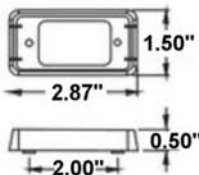
vsm9381 Chrome ABS Surface Mount Bracket
