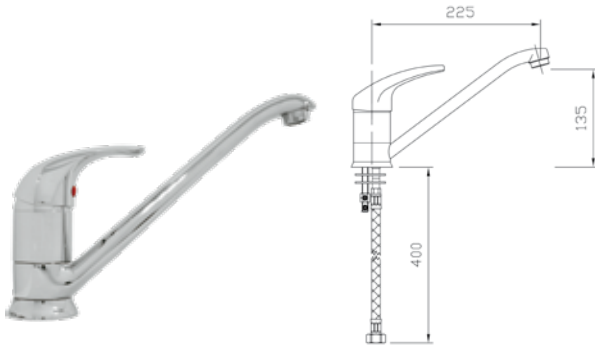
Model Code Low spout tap with short handle • R0020221
