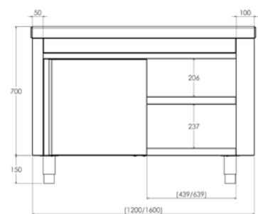
NEUTRAL SELF-SERVICE WITH SLIDING DOORS DIMENSIONS
