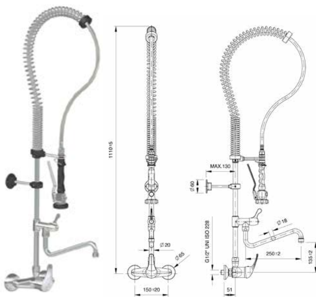
Model Code Wall-mounted spraying tap with extra tap • R0020218
