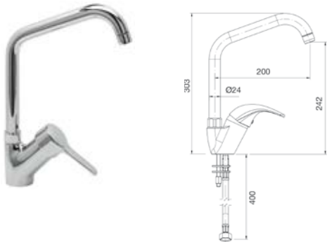
Model Code Single-handle high spout tap • R0020202
