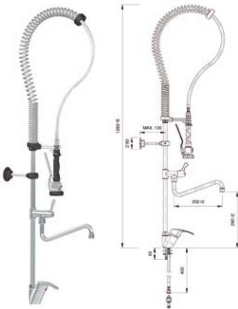
Model Single-handle Spraying tap with extra tap Code • R0020302
