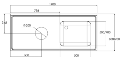
INDUSTRIAL SINK DIMENSIONS 1400 MM
