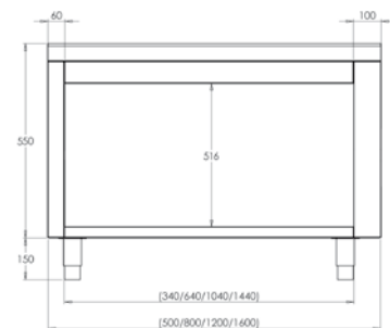
NEUTRAL CHILDREN'S SELF-SERVICE UNIT DIMENSIONS
