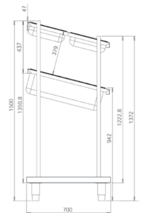
DISPENSER DIMENSIONS
