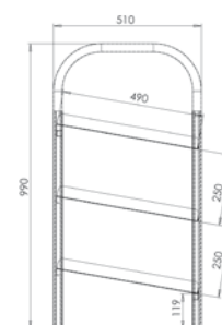
TROLLEY DIMENSIONS
