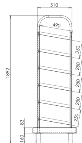
TROLLEY DIMENSIONS
