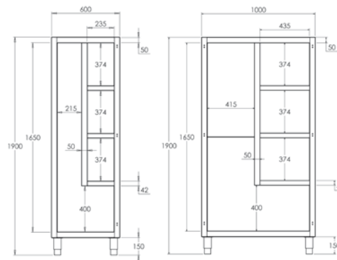
FREESTANDING CABINET DIMENSIONS
