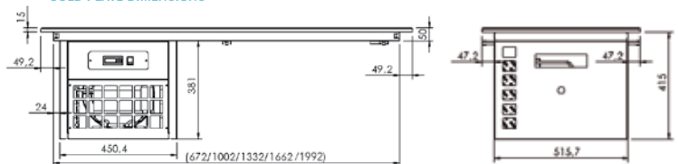
COLD PLATE DIMENSIONS
