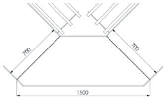
MODEL S1000401 DIMENSIONS
