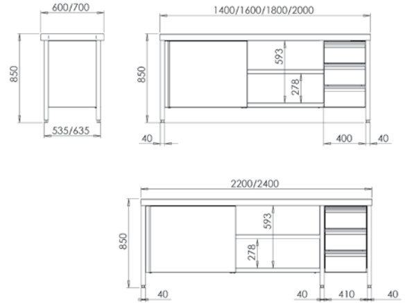
CENTER TABLE WITH DOORS AND DRAWERS DIMENSIONS
