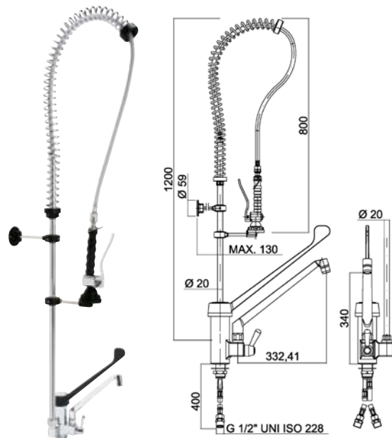
Model Spraying tap with hot/cold controls and extra tap Code • R0020301
