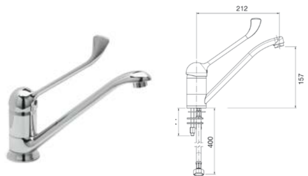
Model Code Low spout tap with long handle • R0020304
