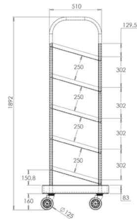
TROLLEY DIMENSIONS
