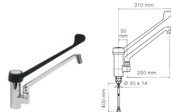
Model Code Easy elbow lever tap • R0020215
