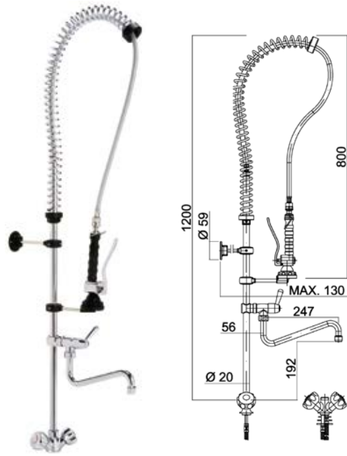
Model Spraying tap with hot/cold controls and extra tap Code • R0020301
