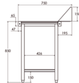
WALL-FACING TABLE DIMENSIONS
