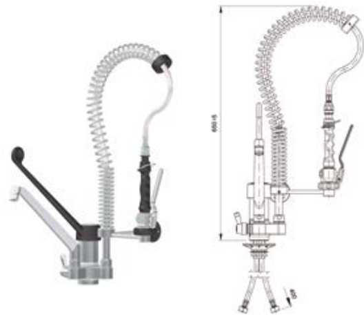
Model Code 600-mm-high easy-open spraying tap with hot/cold controls • R0020306
