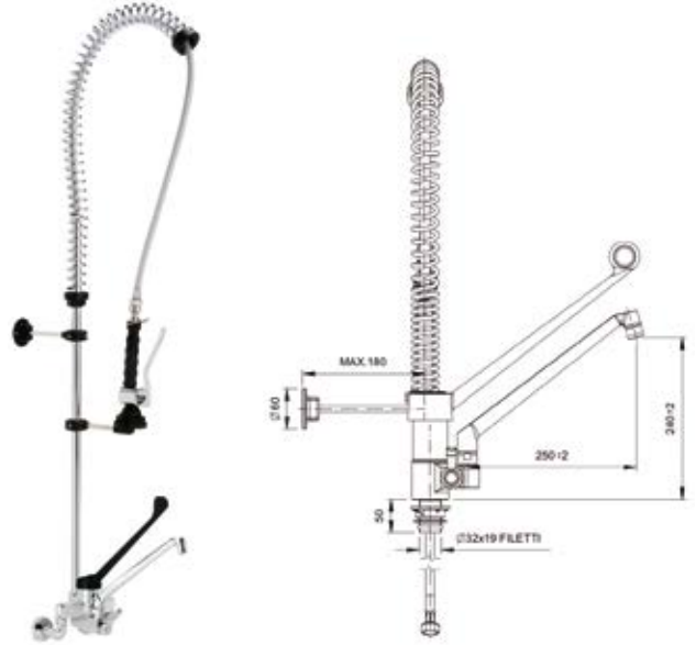
Model Code Easy-open wall-mounted spraying tap • R0020234
