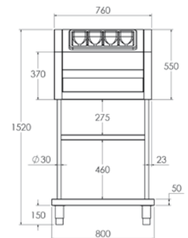
DISPENSER DIMENSIONS
