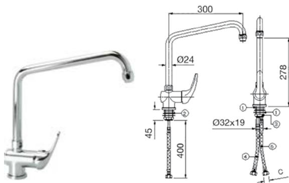
Model Code High spout filled tap • R0020238
