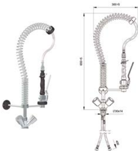
Model Code 600-mm-high hot/cold spray tap • R0020303
