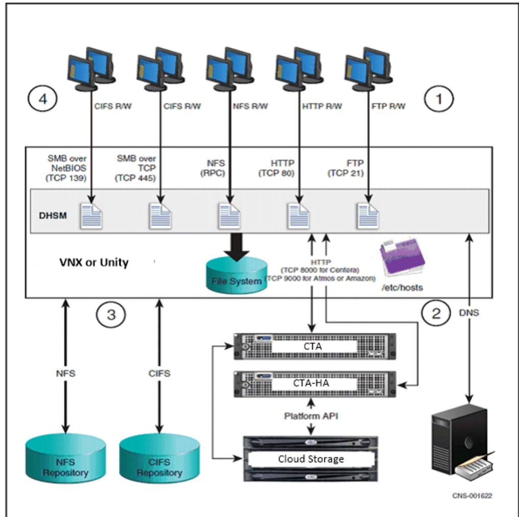
Figure 1. VNX or Unity file implementation
