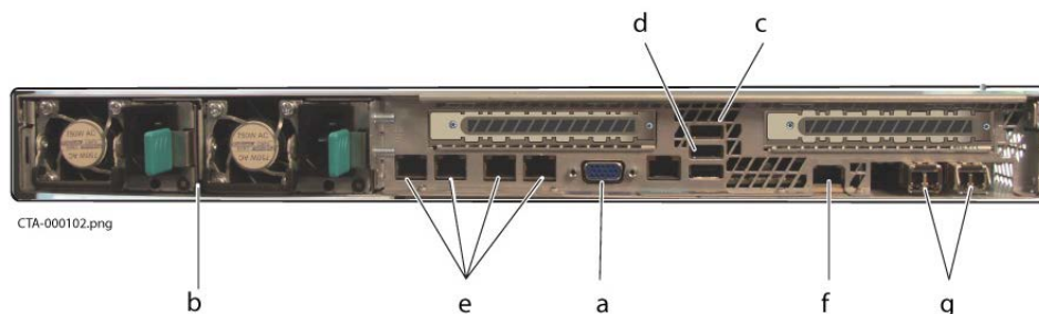
Figure 4. Rear view of Gen 8 appliance
