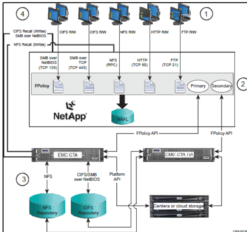
Figure 2. NetApp implementation
