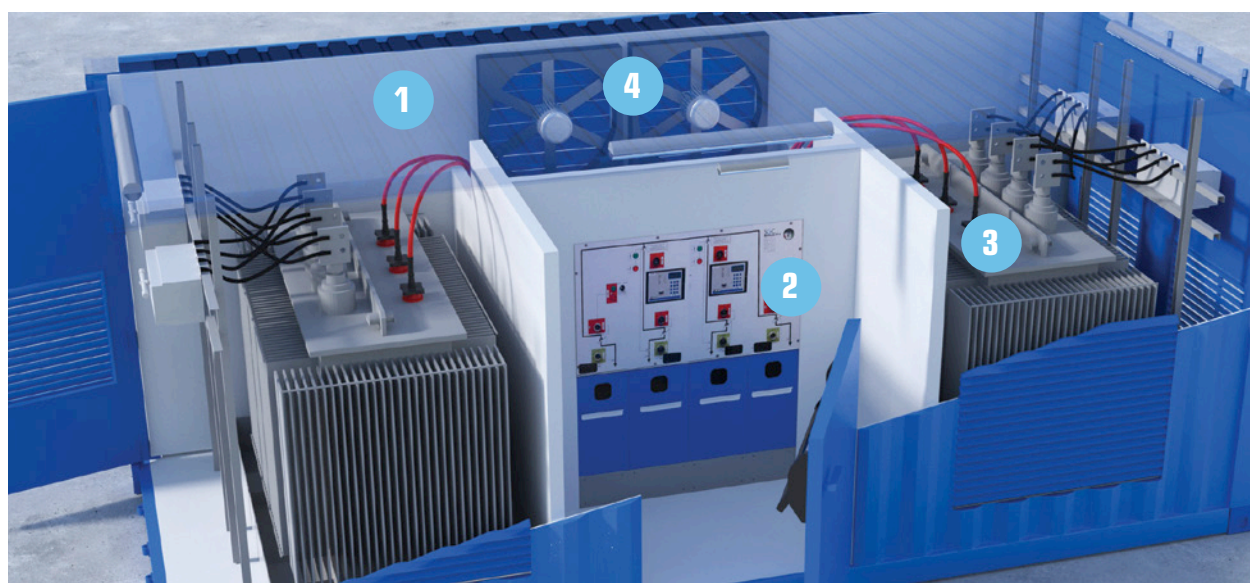
Standard Power Container: typical lay-out, other lay-outs by request.
