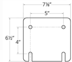
Mounting Plate
