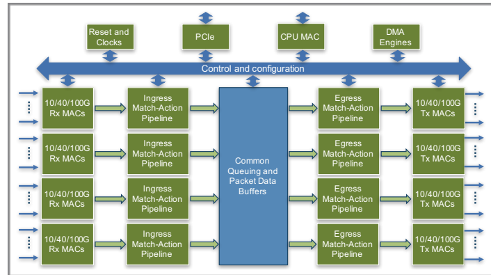
Arista 7170 Series Packet Pipeline Architecture
