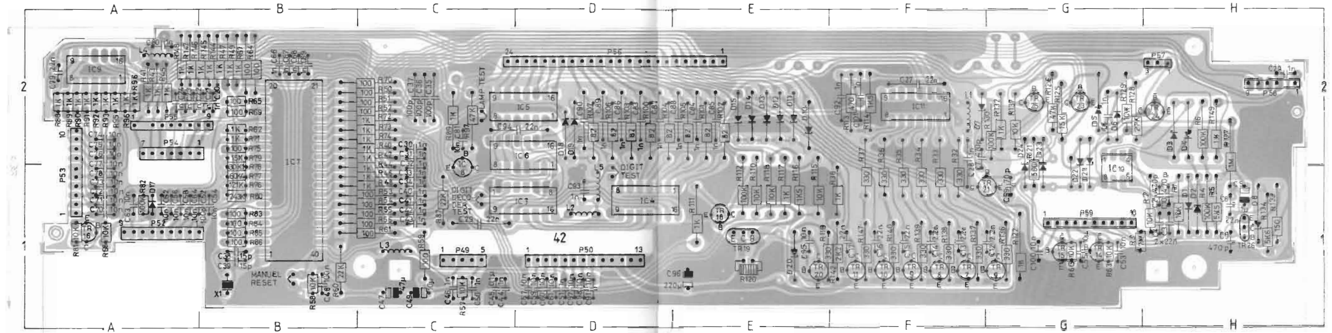
Microcomputer, 8002588, PC42
