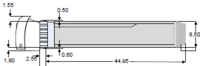
Rear View of Module with Pin Placement
