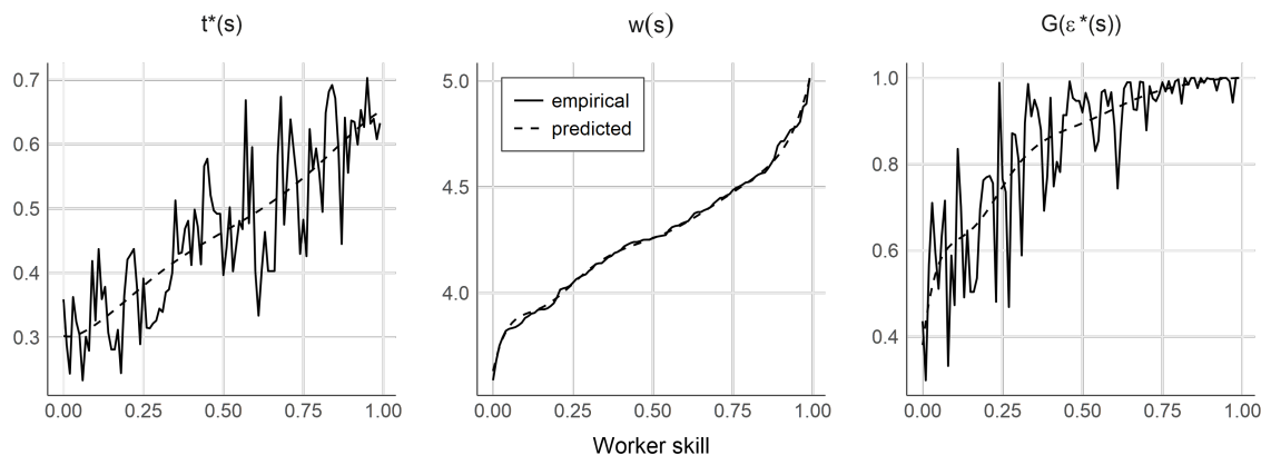
Figure 3.9: Model Goodness-of-Fit
