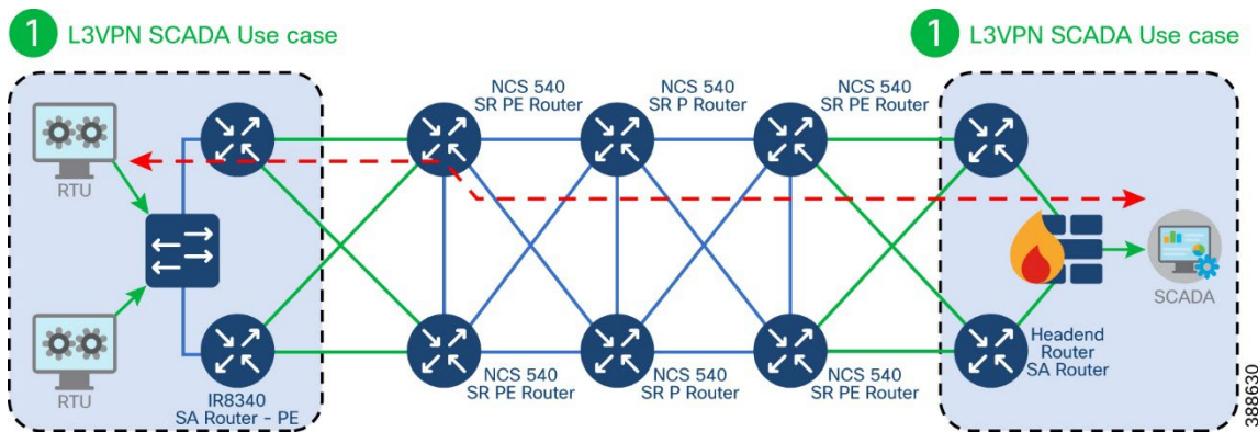
Figure 12 IR8340 Substation Router as PE over SR
