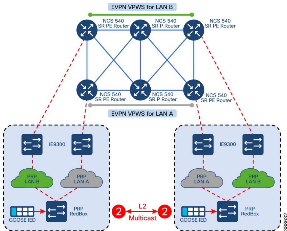
Figure 13 Dual IE9300 as L2 Gateway for L2 Teleprotection services with CS - SR
