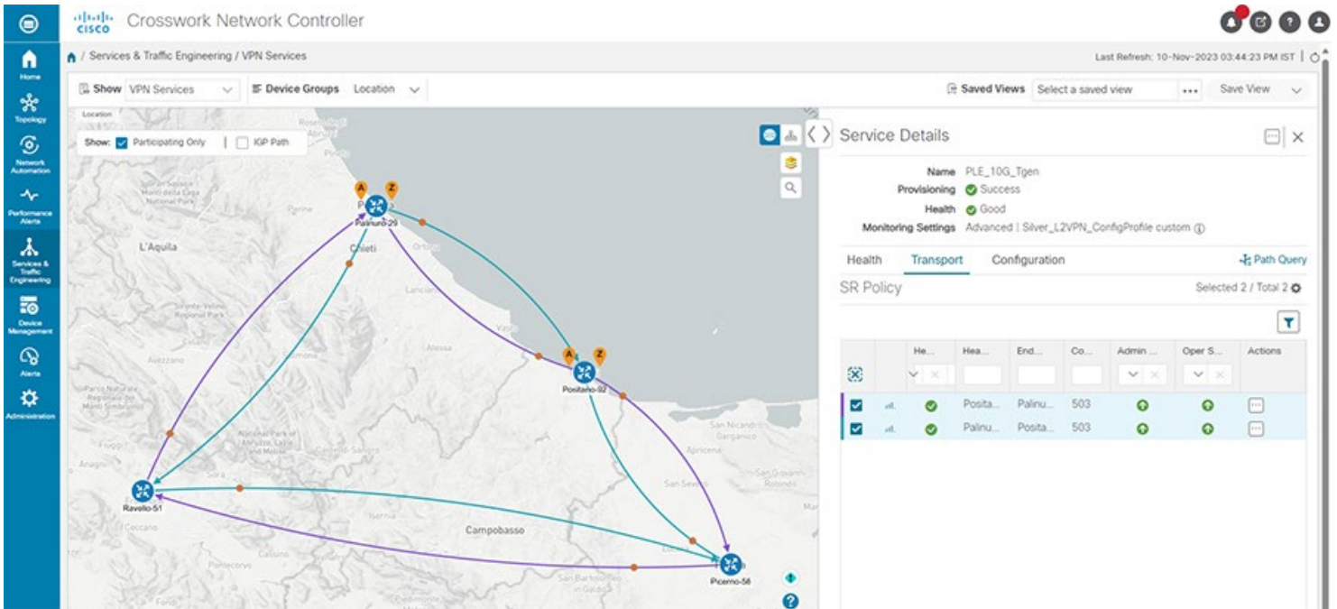
Figure 87 Visualization of the bi-directional nature (depicted in two different colors purple and blue) of CS SR-TE policies between the endpoints
