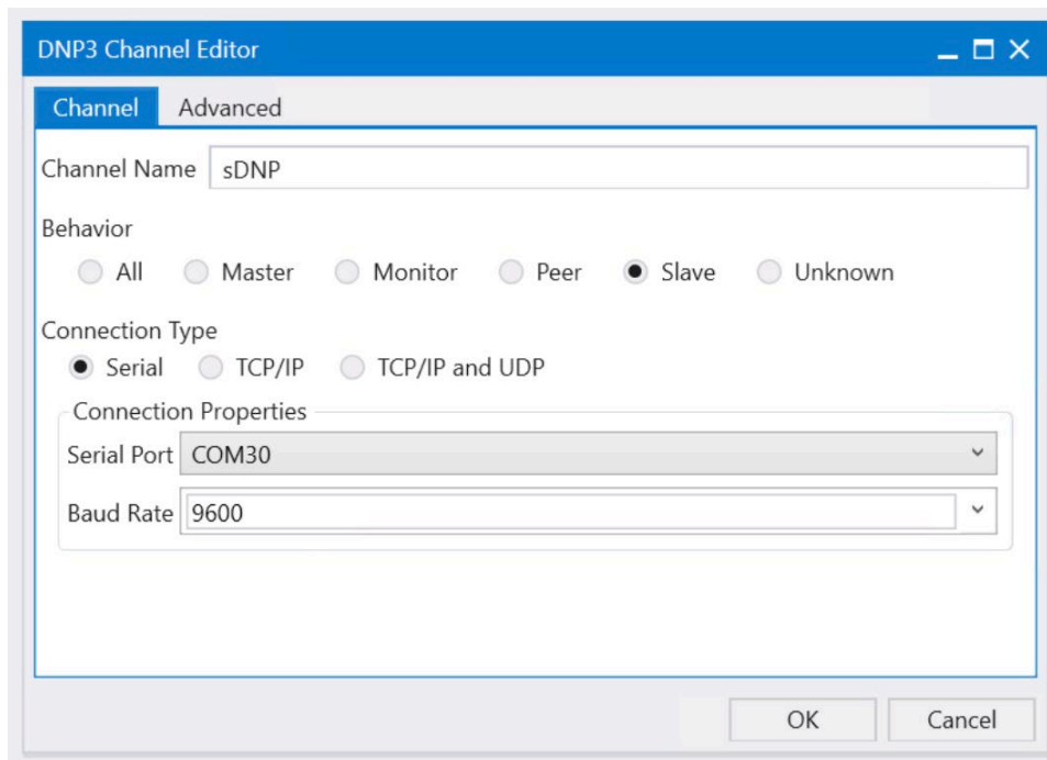
Figure 40 DNP3 IED Channel Configuration
