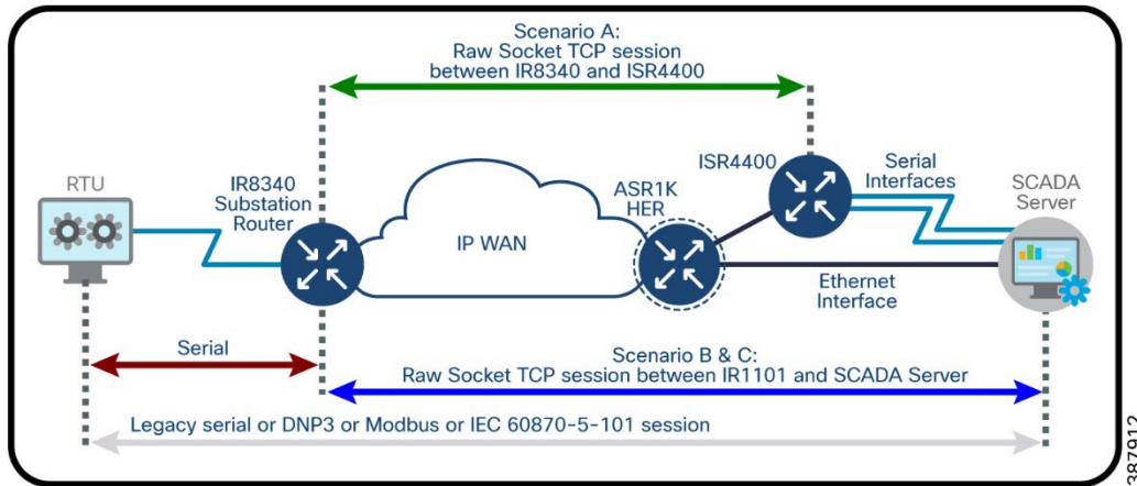
Figure 22 SCADA Raw Socket Implementation diagram
