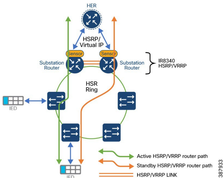
Figure 10 HSRP/VRRP LAN Traffic Flow
