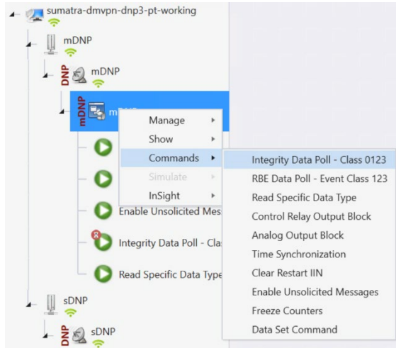
Figure 46 DNP3 Integrity Data Poll
