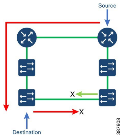
Figure 15 Rapid Per VLAN Spanning Tree
