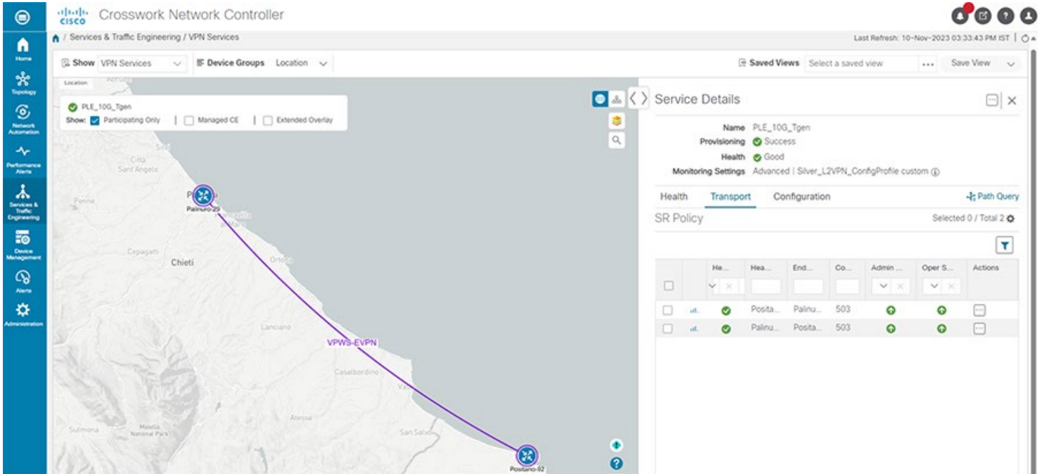
Figure 86 EVPN-VPWS service stitched to CS SR-TE policy
