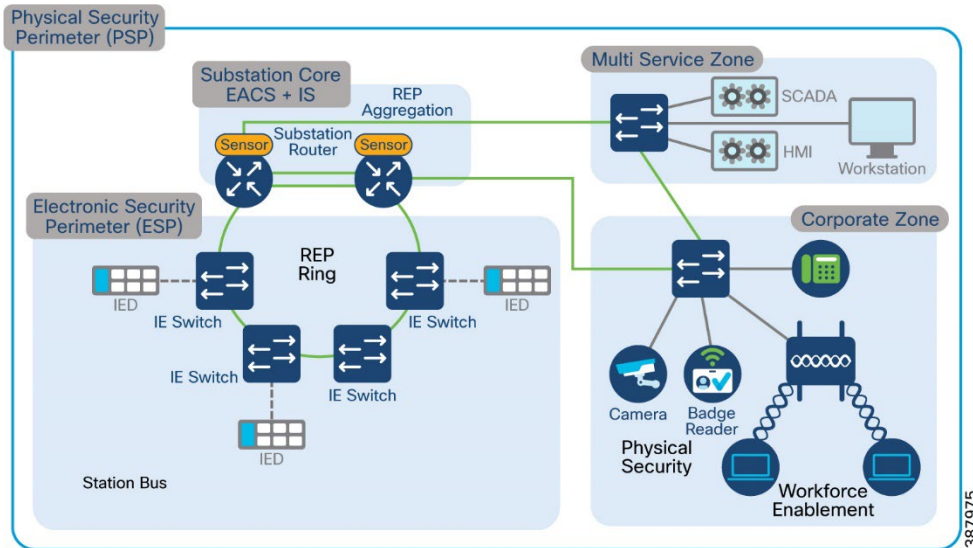
Figure 16 Substation Router with multiple REP rings for different zones
