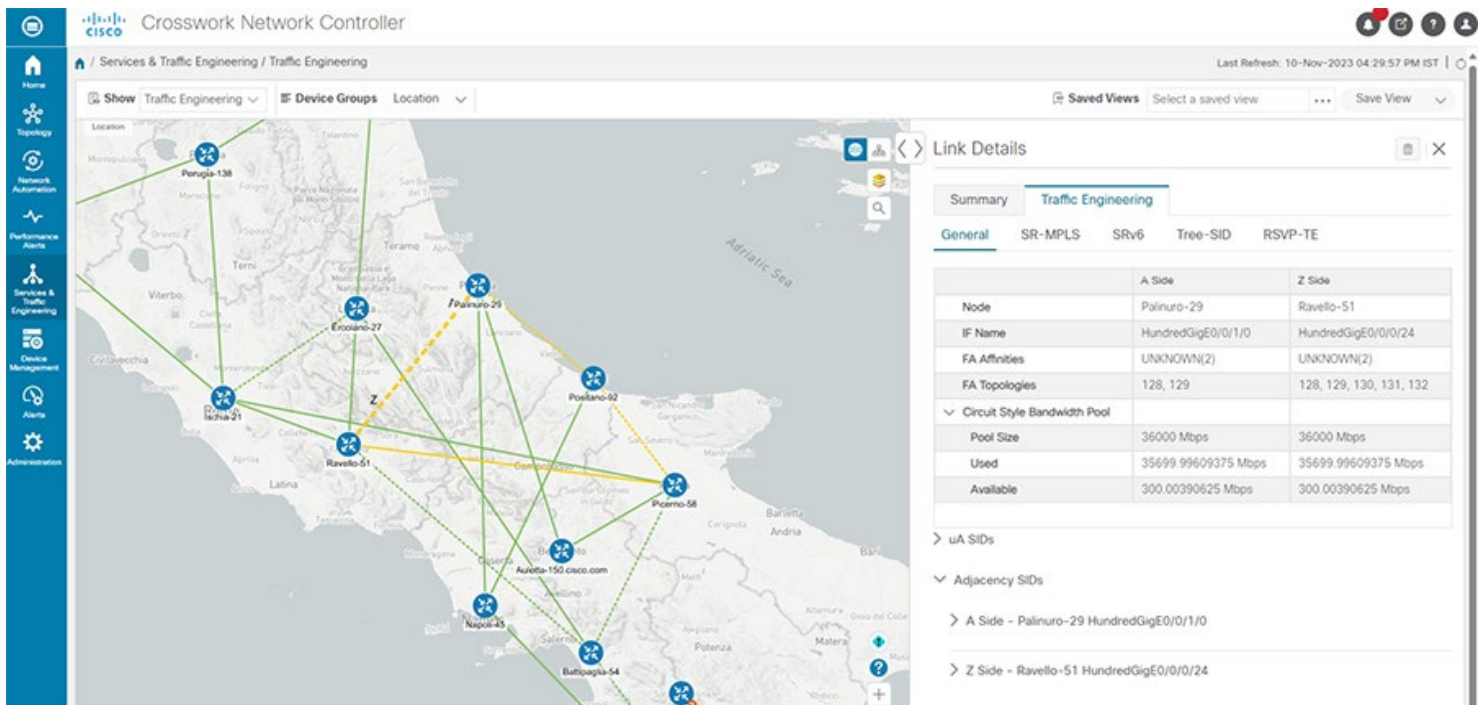
Figure 91 Bandwidth monitoring on the Working Path
