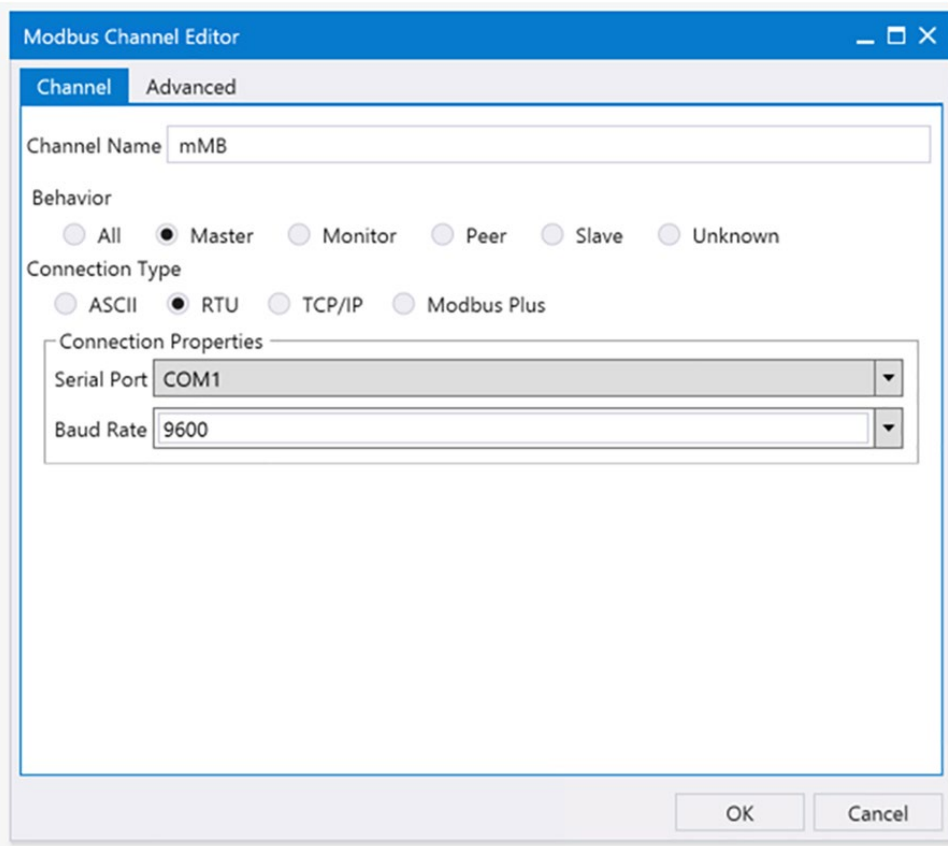
Figure 24 Modbus FEP Channel Configuration
