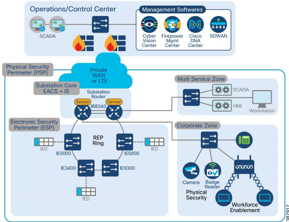
Figure 19 NTP in a Substation
