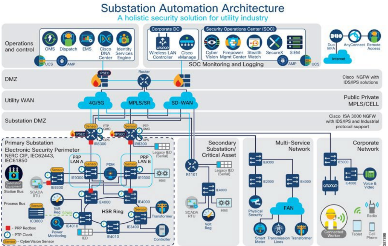
Figure 21 Substation Automation validation topology with SCADA
