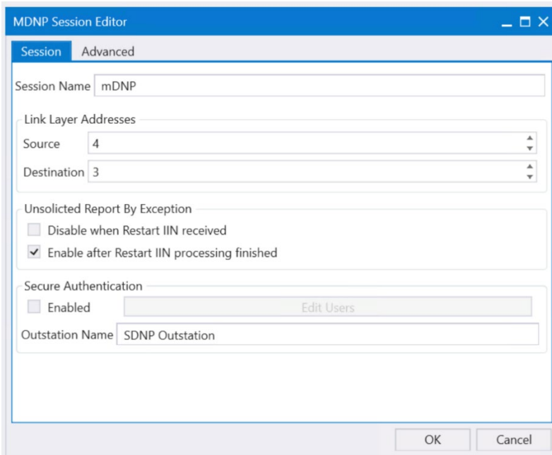
Figure 44 DNP3 FEP session configuration
