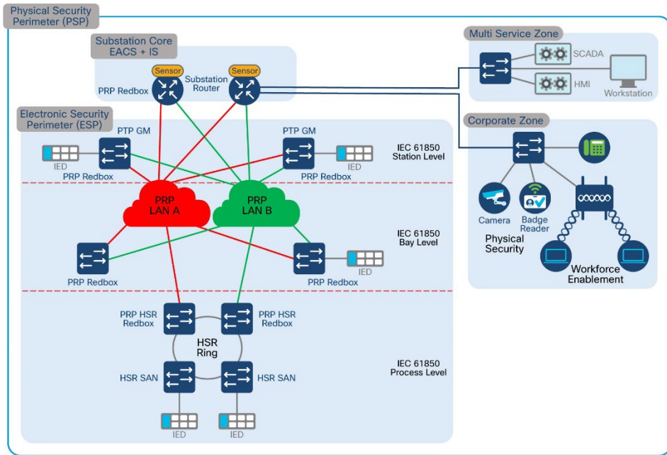
Figure 20 PTP in Substation LAN
