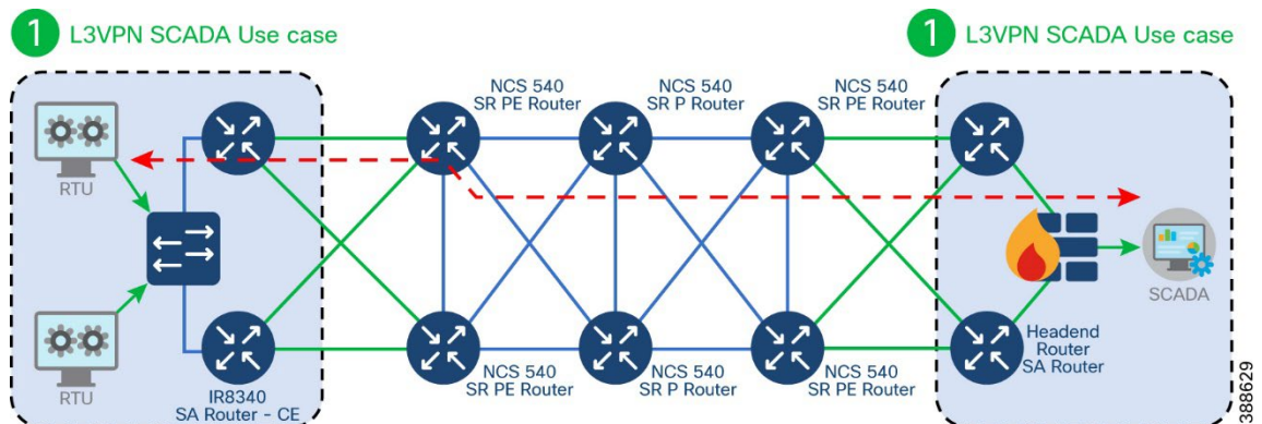
Figure 11 IR8340 Substation Router as CE over SR
