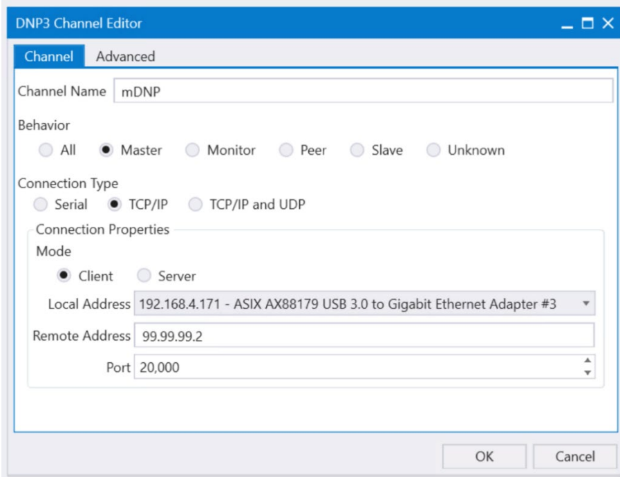
Figure 43 DNP3 FEP Channel configuration
