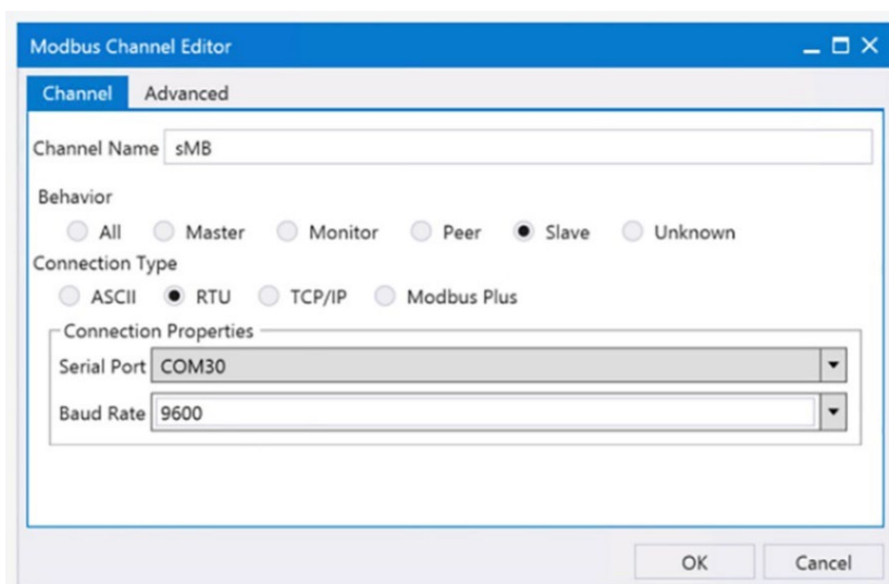
Figure 29 Modbus IED Channel configuration
