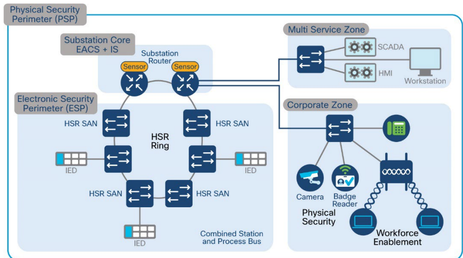
Figure 3 HSR on Substation Router
