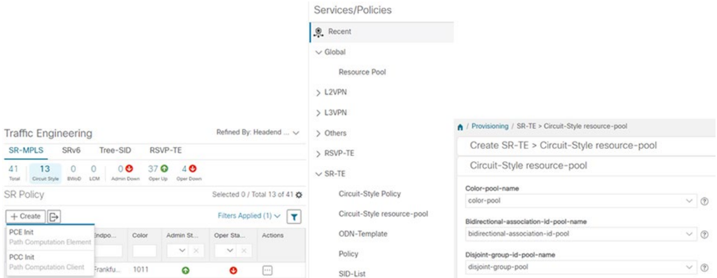
Figure 76 CS SR-TE policy initiation; CS resource-pool definition
