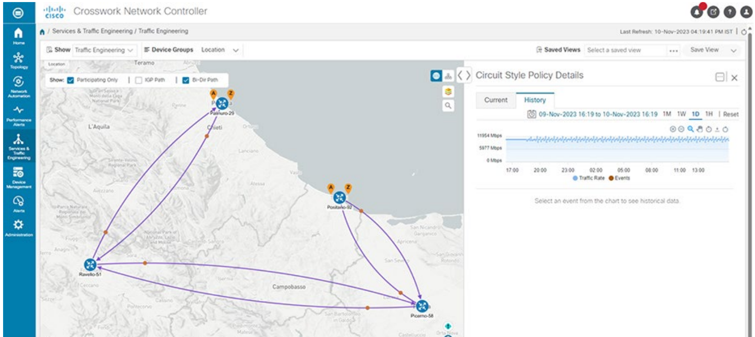
Figure 90 Steady traffic running over the working path between endpoints
