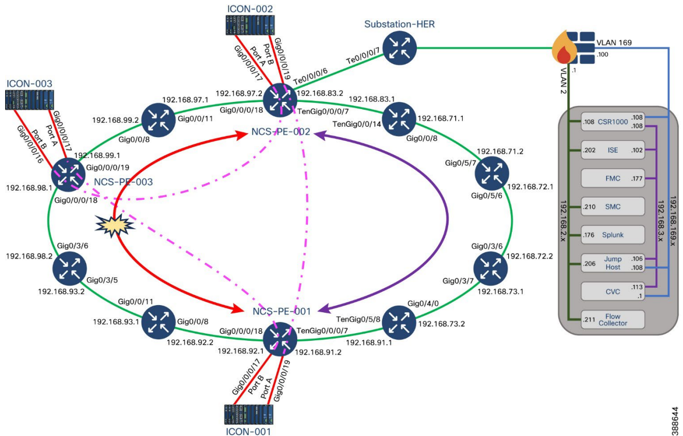
Figure 8 Teleprotection over Segment Routed Core using SEL ICON
