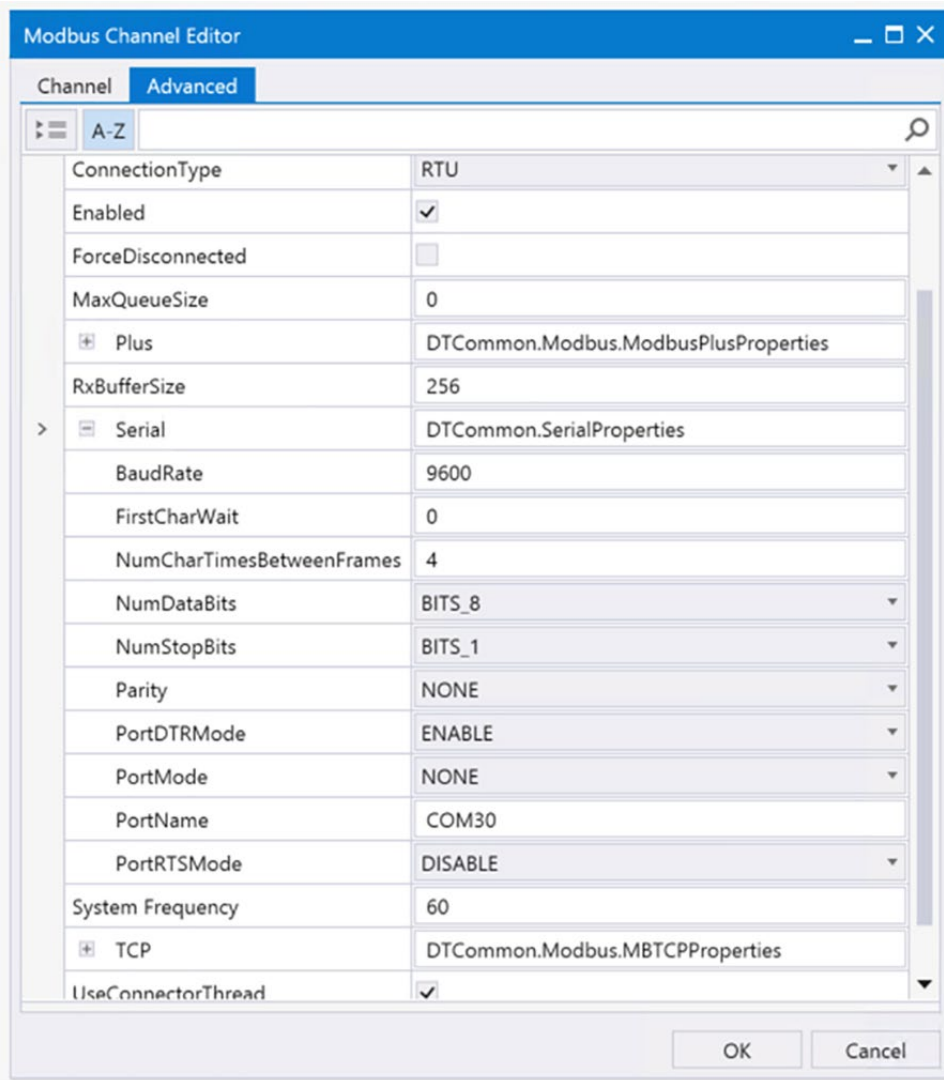
Figure 25 Modbus FEP advance Channel configuration
