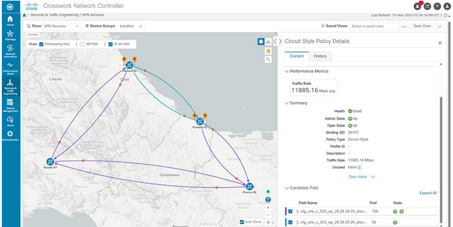
Figure 88 Visualization of bi-directional CS SR-TE policy showcasing working path (purple; higher preference 100) and protect path (blue; preference 50) between endpoints A and Z
