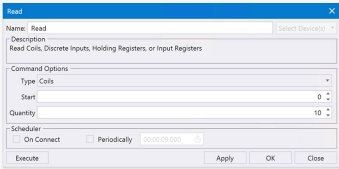
Figure 34 Modbus Read command config window
