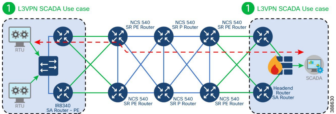
Figure 6 IR8340 Substation Router as PE over SR
