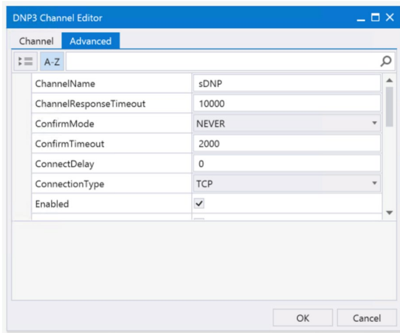
Figure 58 DNP3 IP IED Advance Channel configuration
