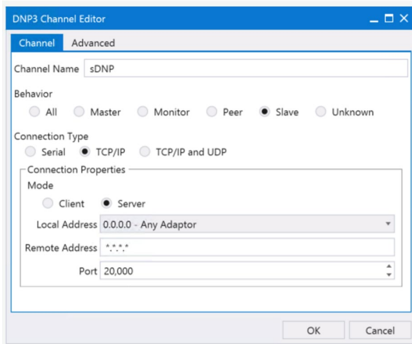
Figure 57 DNP3 IP IED Channel Configuration
