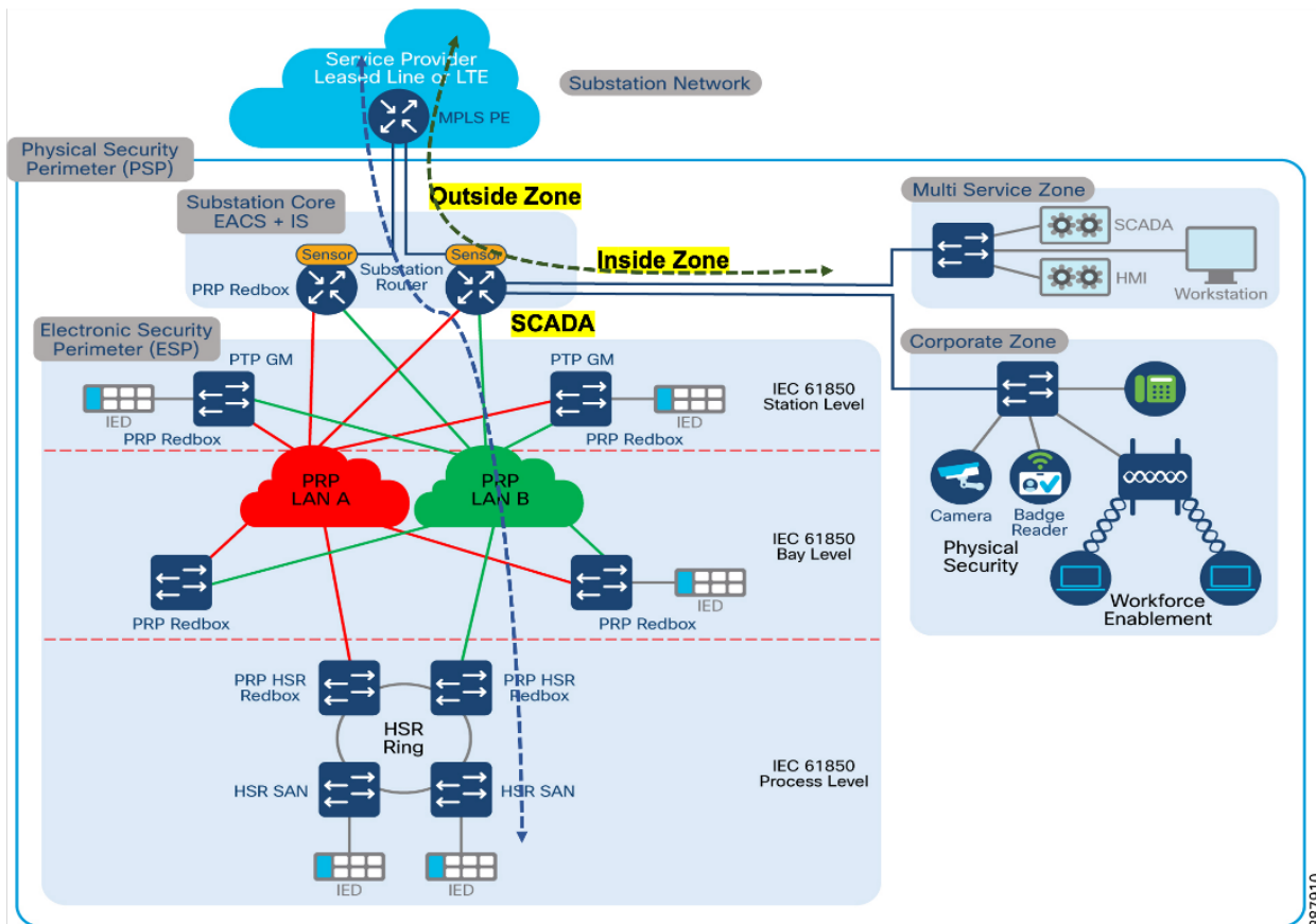
Figure 60 Zone Based Firewall in a Substation
