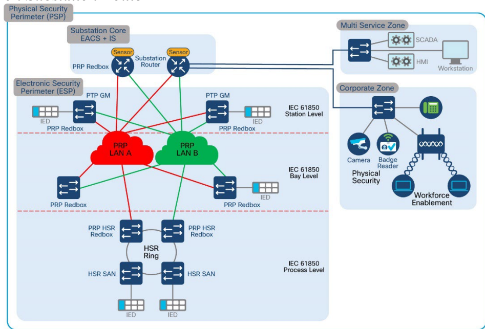
Figure 2 PRP on Substation Router
