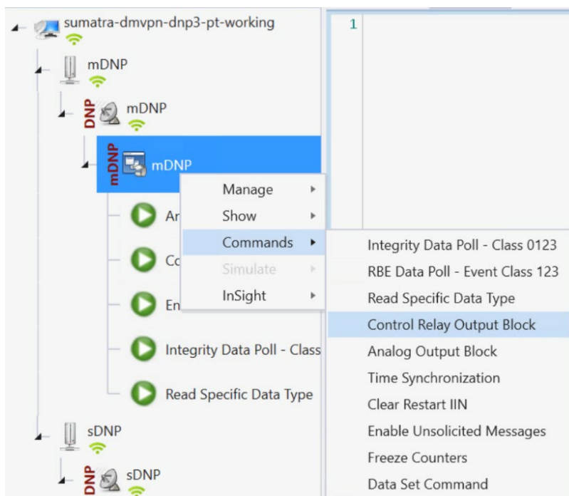
Figure 54 DNP3 CROB control command
