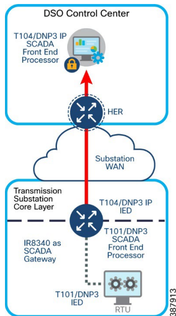
Figure 39 Protocol Translation implementation diagram
