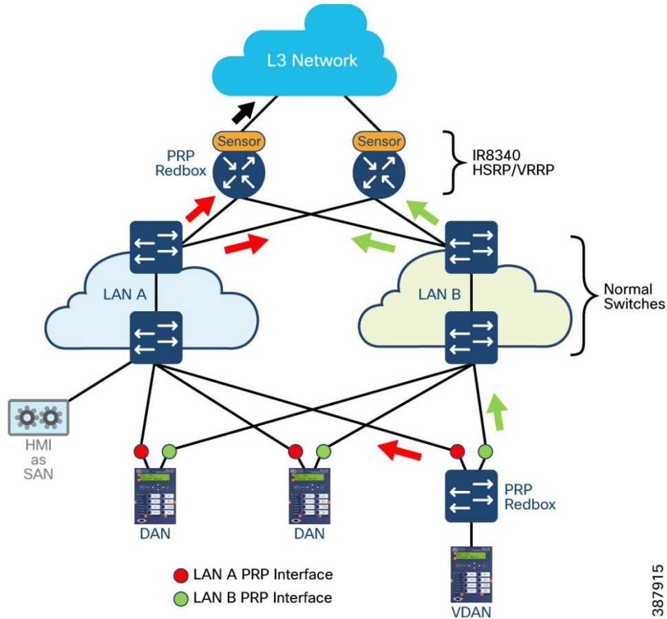
Figure 17 PRP Redbox with L3 Gateway Redundancy
