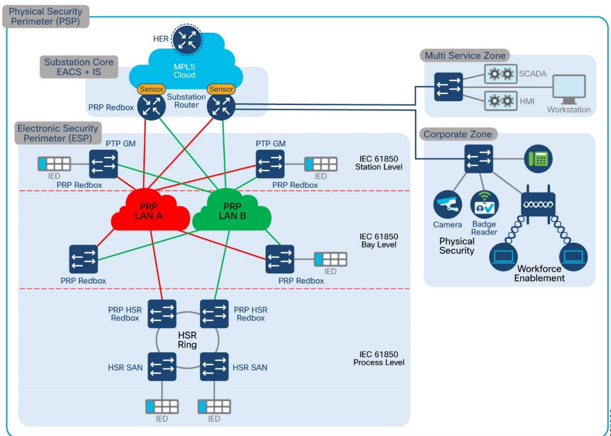
Figure 9 Substation Router with MPLS Backhaul
