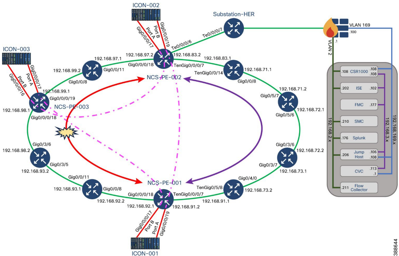
Figure 14 Teleprotection over Segment Router core using SEL ICON
