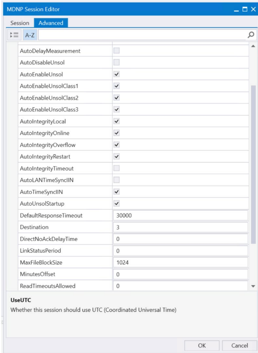
Figure 45 DNP3 FEP Advanced session configuration
